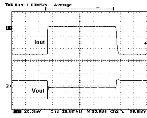
Figure 28 : Load Transient
