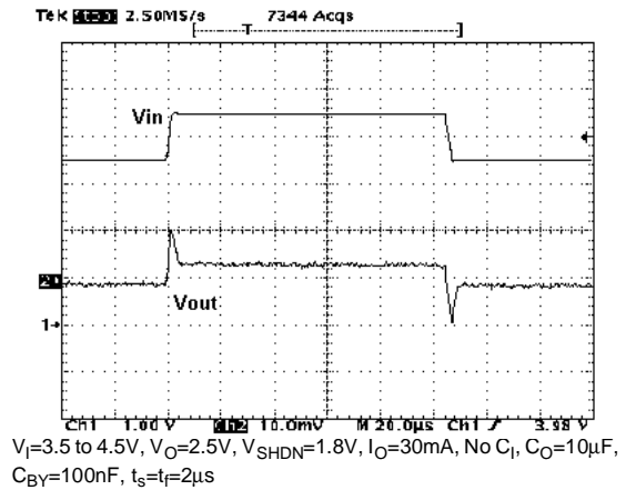
Figure 24 : Line Transient
