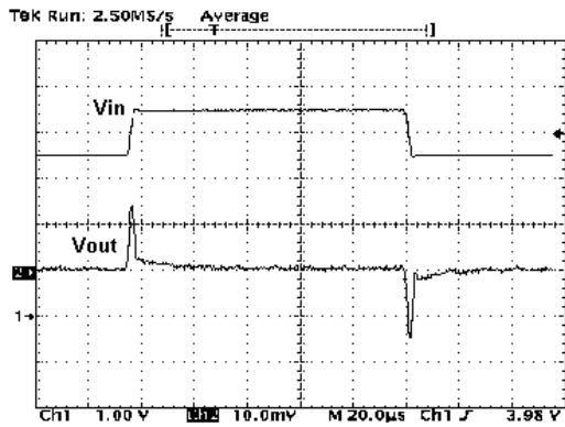
Figure 25 : Line Transient
