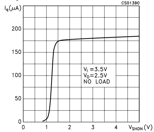
Figure 16 : Quiescent Current vs Shutdown Voltage
