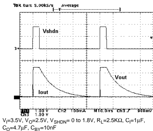
Figure 21 : Start-up Transient
