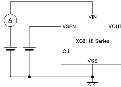
Circuit 4
