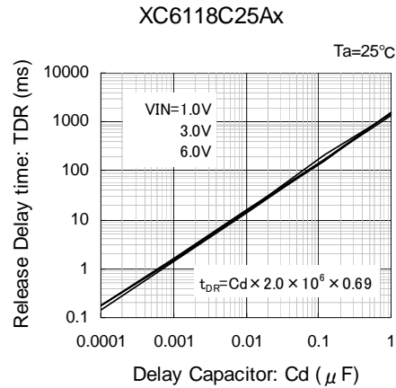
(11) Release Delay Time vs. Delay Capacitance
