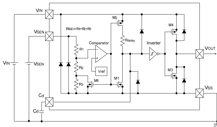
Figure 1: Typical application circuit example
