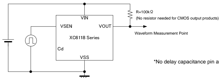
Circuit 9
