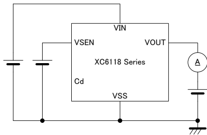
Circuit 5
