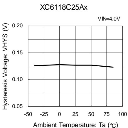
(5) Hysteresis Voltage vs. Ambient Temperature
