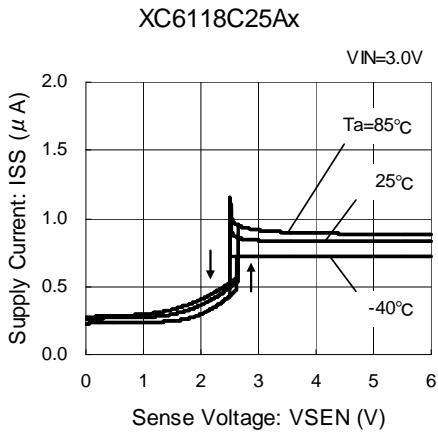
(2) Supply Current vs. Input Voltage
