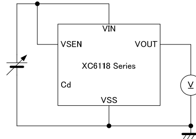
Circuit 8
