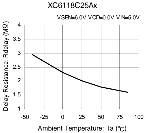
(10) Delay Resistance vs. Ambient Temperature
