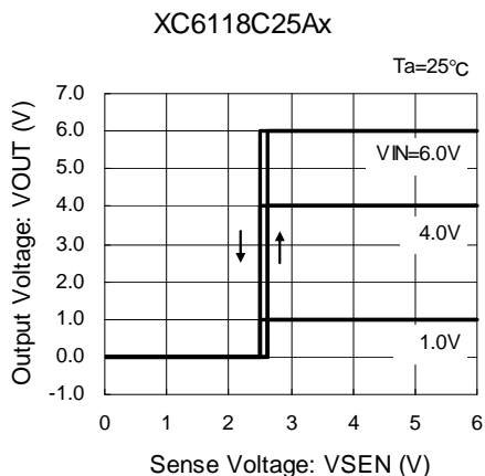
(7) Output Voltage vs. Sense Voltage
