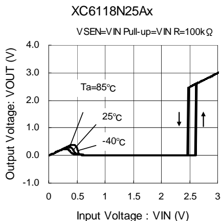
(8) Output Voltage vs. Input Voltage
