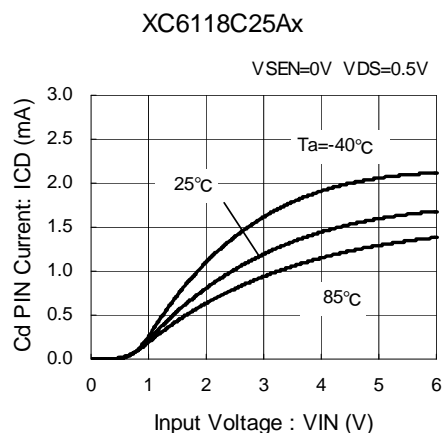
(6) CD Pin Sink Current vs. Input Voltage
