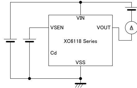
Circuit 6
