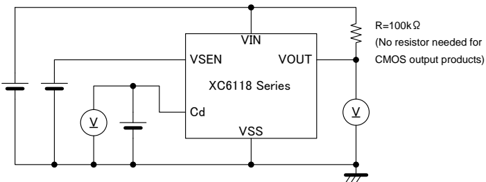
Circuit 9
