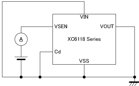
Circuit 7
