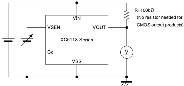
Circuit 3
