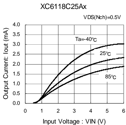
(9) Output Current vs. Input Voltage
