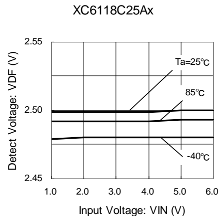
(4) Detect Voltage vs. Input Voltage
