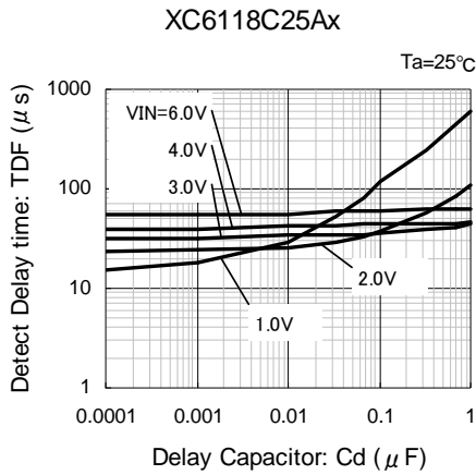
(12) Detect Delay Time vs. Delay Capacitance
