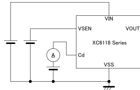
Circuit 8
