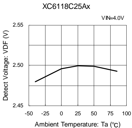
(3) Detect Voltage vs. Ambient Temperature
