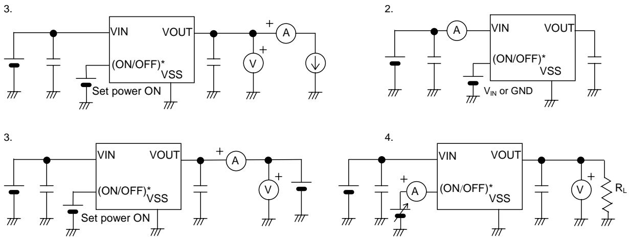
Figure 6 Test Circuits
