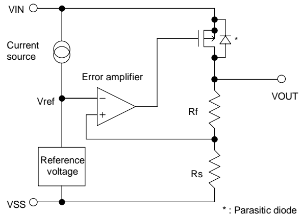
Figure 9 Block Diagram
