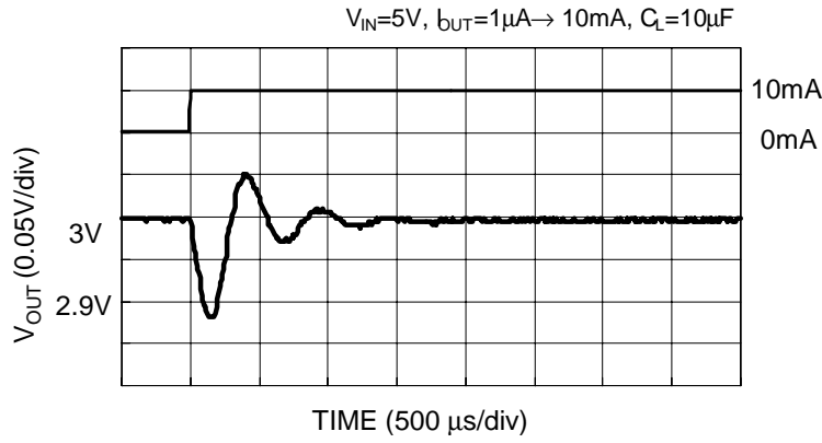
Load dependence of undershoot at load transient
