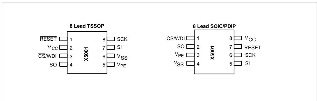
Figure 1. PIN CONFIGURATION
