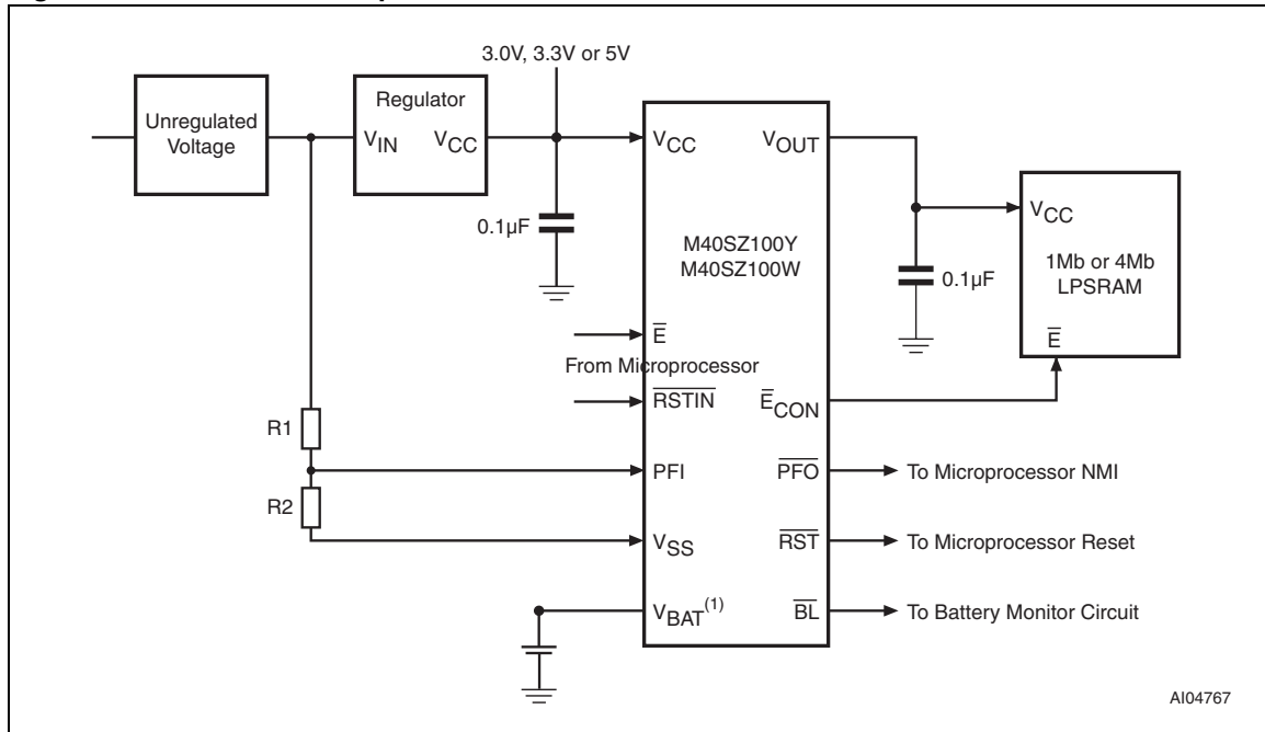
Figure 5. Hardware hookup
