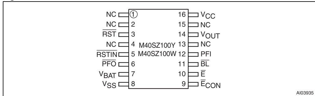
Figure 2. SOIC16 connections
