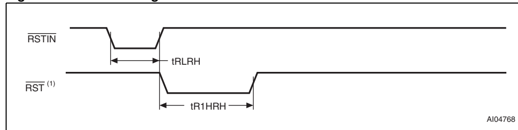
Figure 8. \overline{RSTIN} timing waveform
