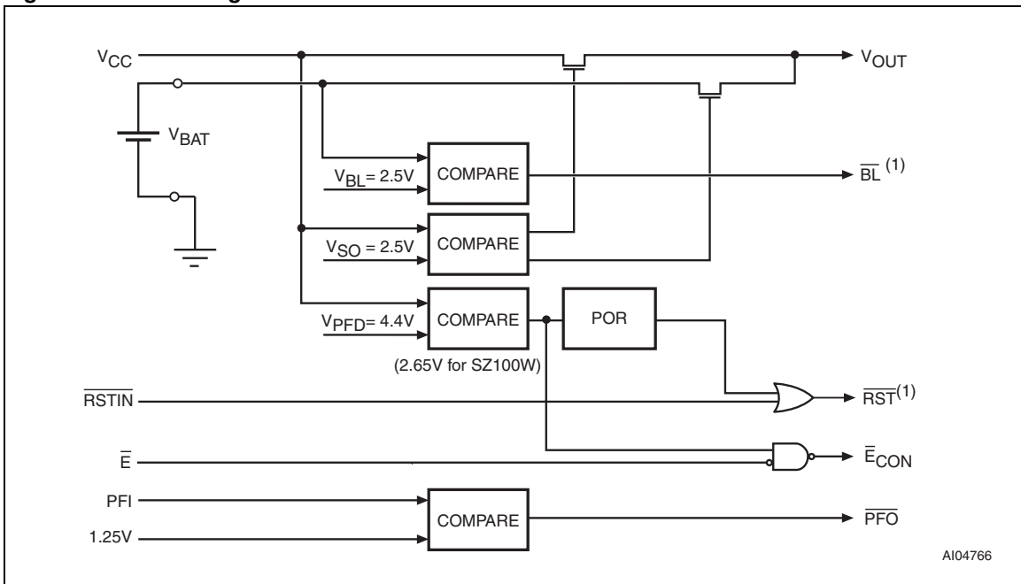
Figure 4. Block diagram
