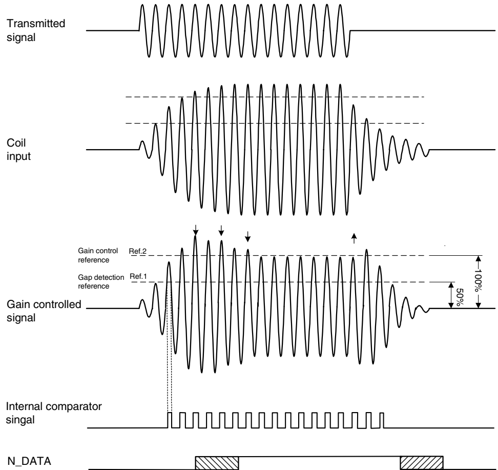
Figure 4. Automatic Gain Control
