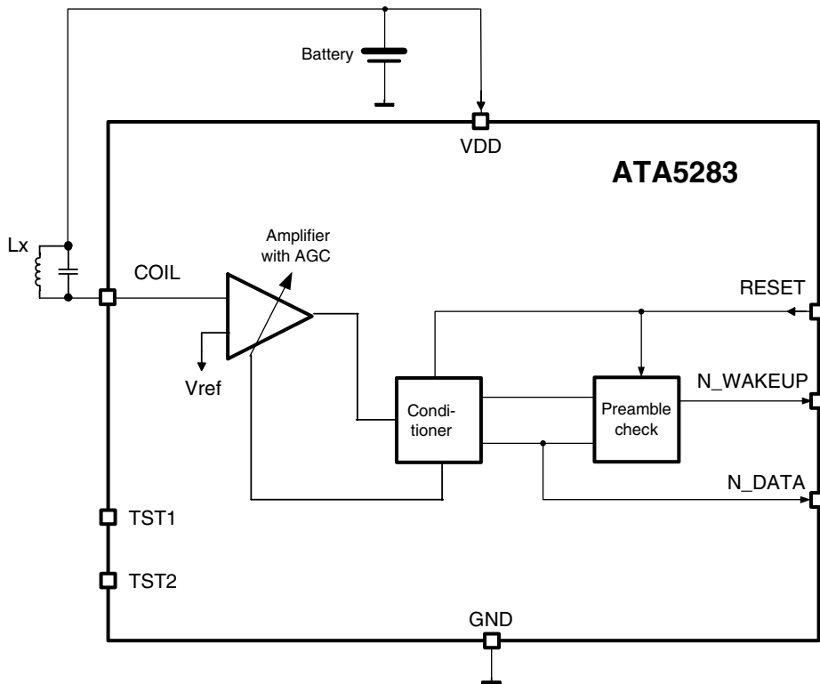
Figure 1. Block Diagram
