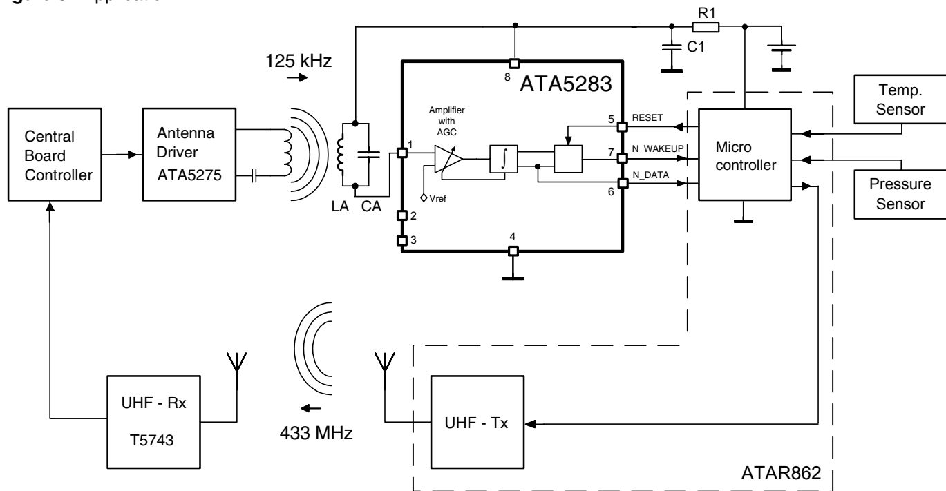
Figure 8. Application
