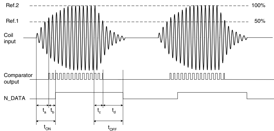
Figure 5. Output Timing
