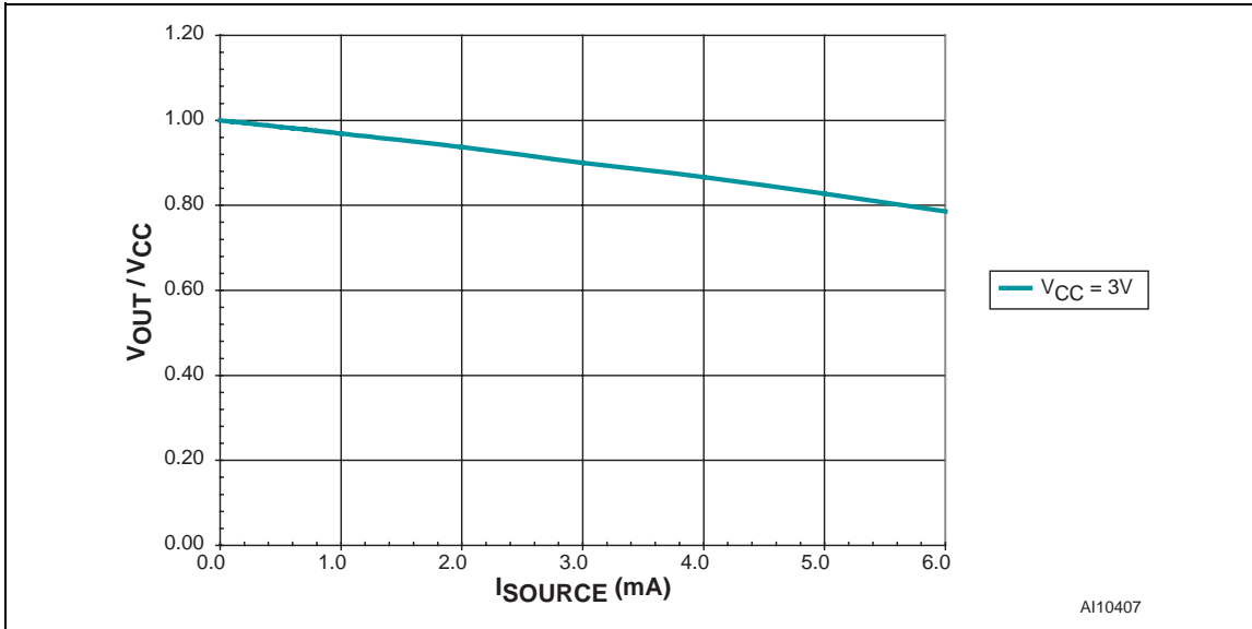
Figure 18. Voltage Output High vs. I SOURCE
