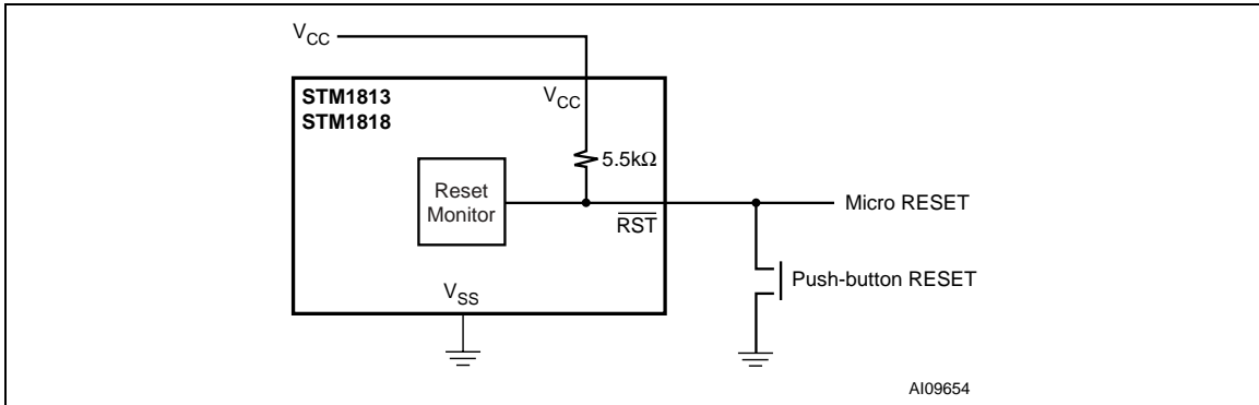
Figure 9. Push-Button Manual Reset with \overline{\text{MR}} Detect (STM1813/1818)
