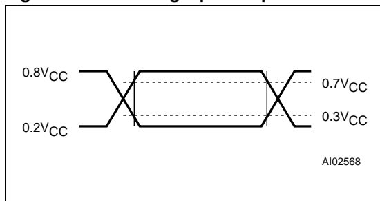
Figure 21. AC Testing Input/Output Waveforms
