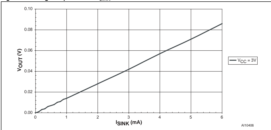
Figure 17. Voltage Output Low vs. I_{SINK}
