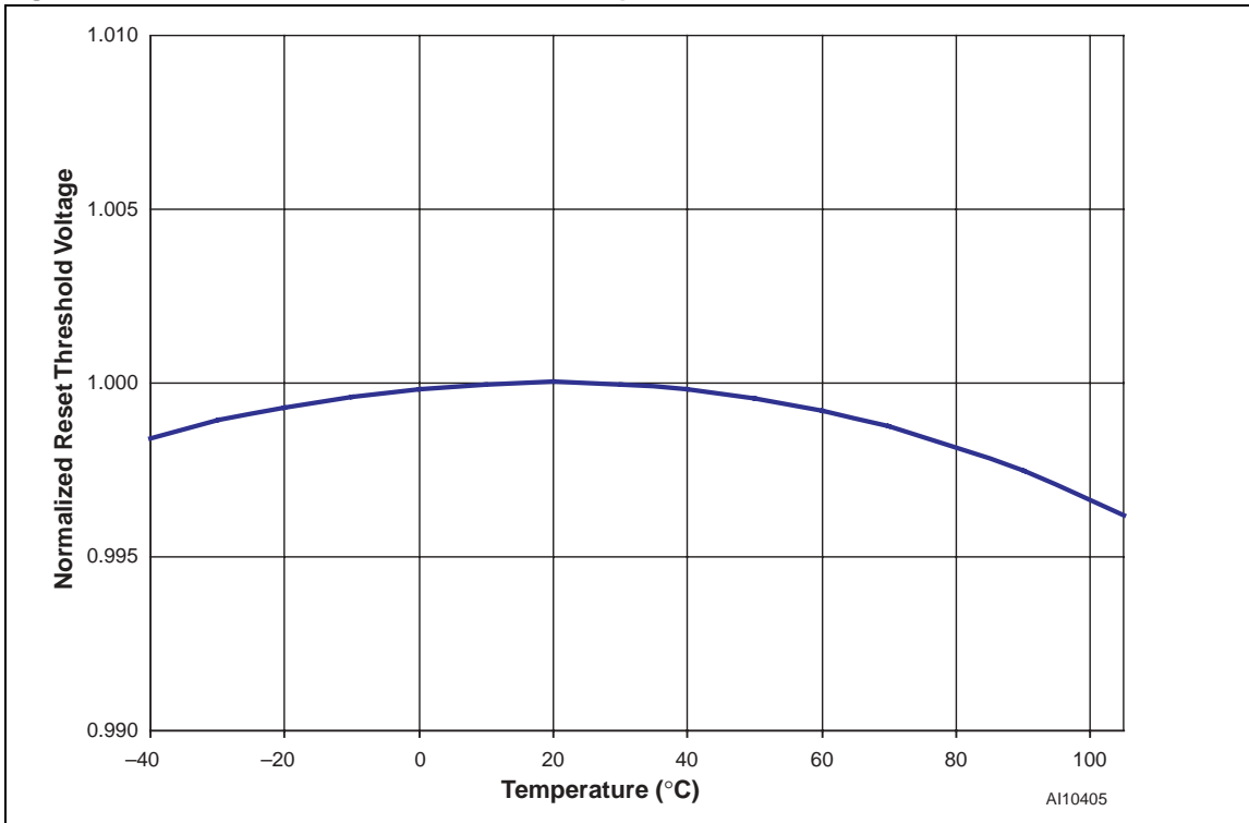
Figure 19. Normalized Reset Threshold vs. Temperature
