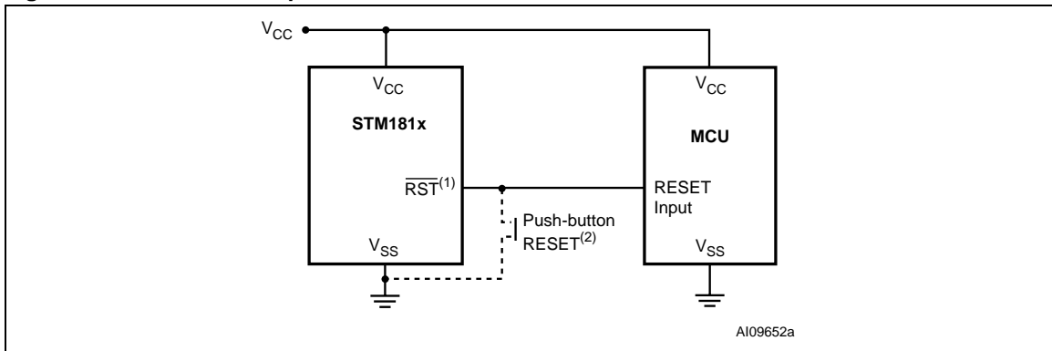
Figure 4. Hardware Hookup
