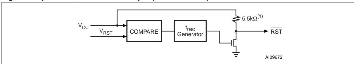
Figure 6. Open Drain, Active-Low Output (STM1811/1816)
