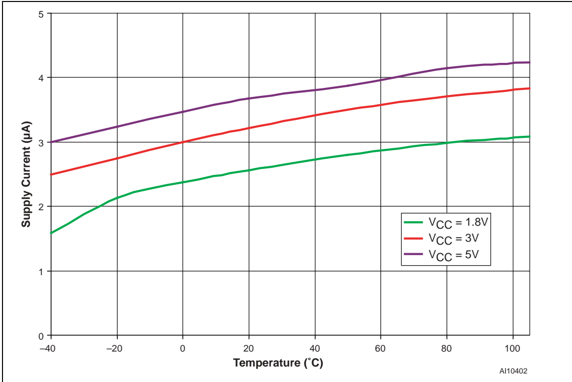
Figure 14. Supply Current vs. Temperature (no load)
