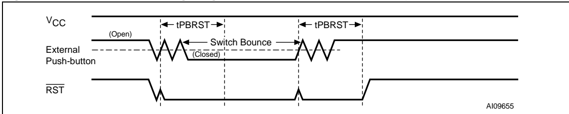
Figure 10. Manual Reset Timing Diagram, Switch Bounce/Debounce (STM1813/1818)
