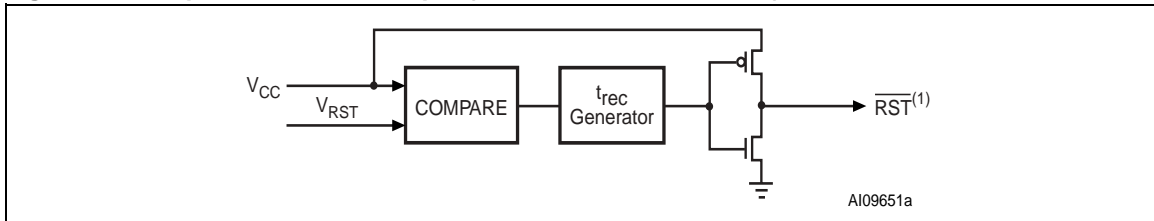
Figure 5. Push-pull Active-Low Output (STM1810/1812/1815/1817)
