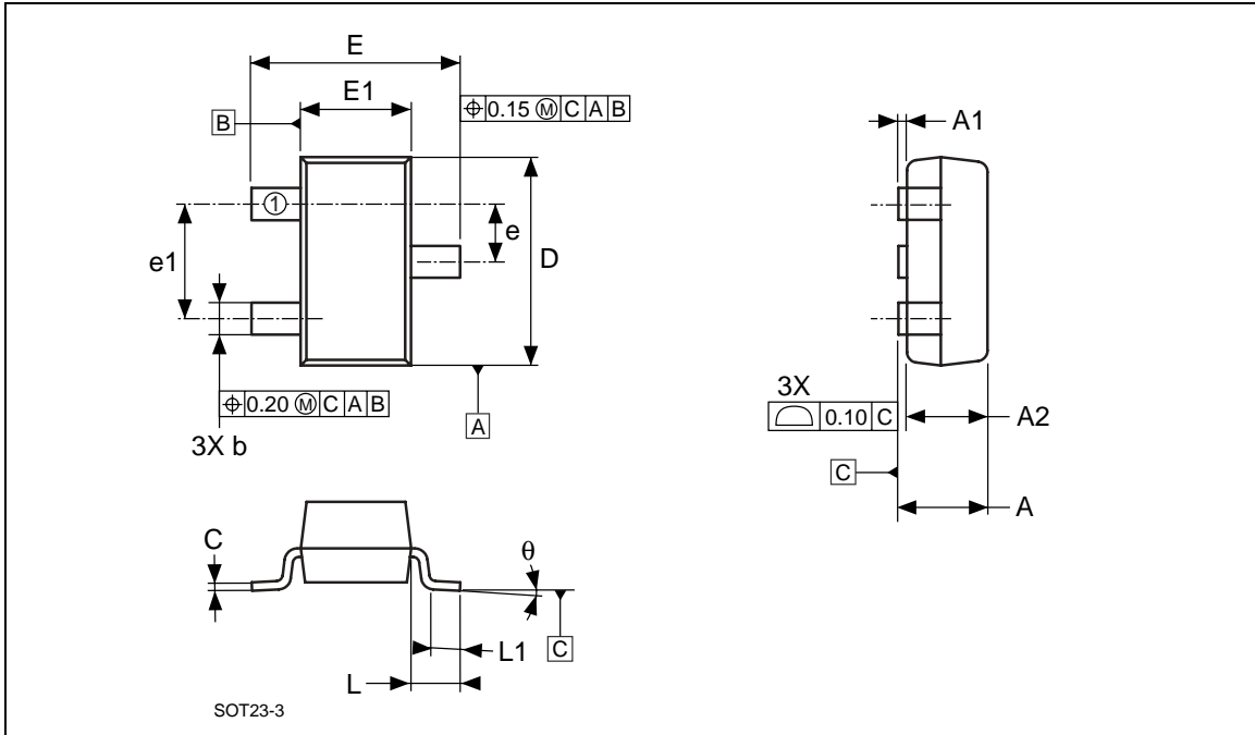
Figure 22. SOT23-3 – 3-lead Small Outline Transistor Package Outline
