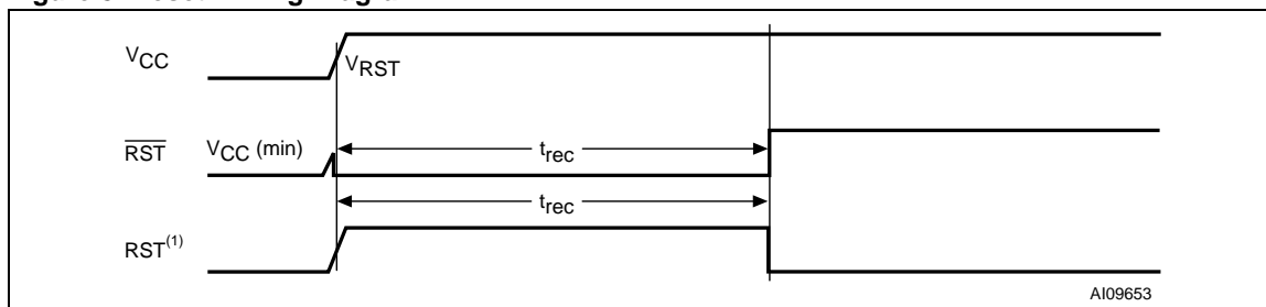
Figure 8. Reset Timing Diagram
