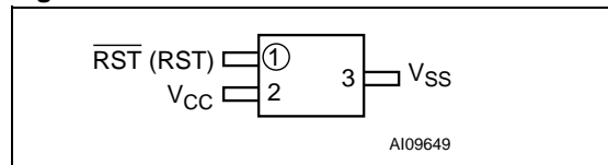
Figure 3. SOT23-3 Connections
