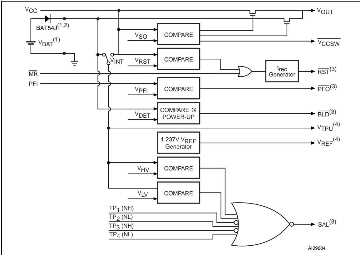
Figure 4. Block Diagram
