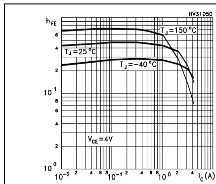
Figure 6. DC current gain (NPN)
