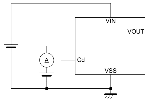
Circuit 4
