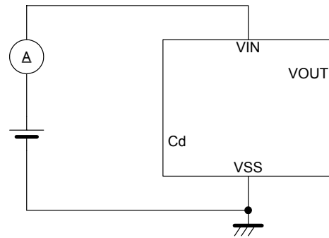
Circuit 4
