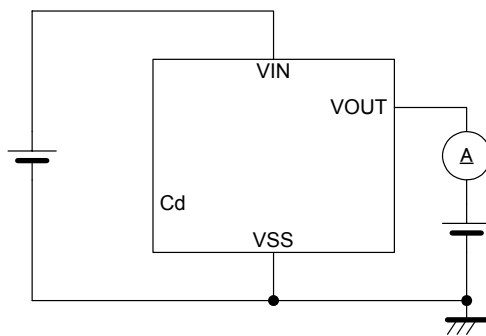
Circuit 3
