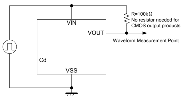
Circuit 7
