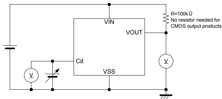
Circuit 5
