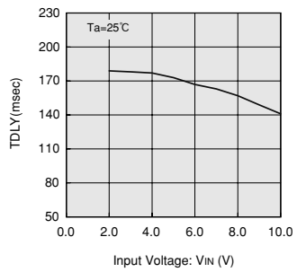
(8) INPUT vs. TRANSIENT DELAY TIME
