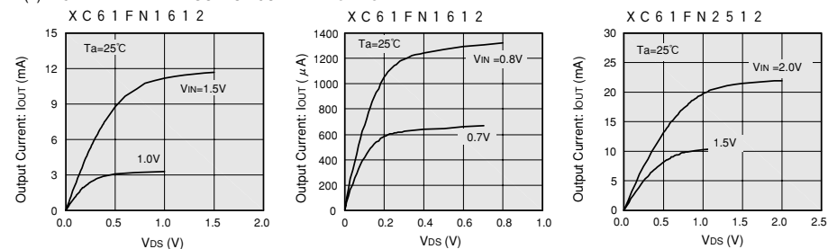
(4) N-CHANNEL DRIVER OUTPUT CURRENT vs. Vds
