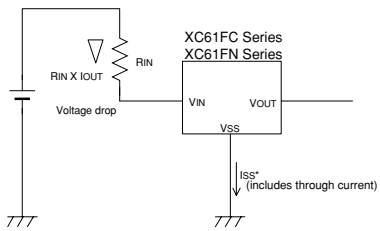
Diagram 3. Oscillation in relation to through current
