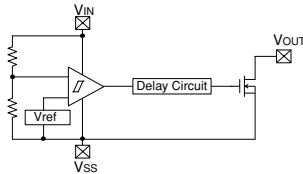
(2) N-channel open drain output
