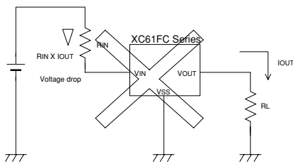
Diagram 2. Oscillation in relation to output current
