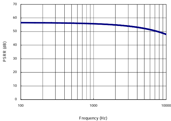
PSRR (VOUT = 3.3) (VIN = 5V, VPP = 1V)
