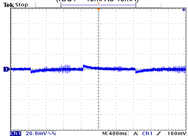
Transient Response (VOUT = 3.3V) (IOOUT = 10mA to 40mA)
