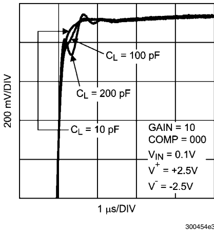
Positive Overshoot vs. C_{LOAD}
