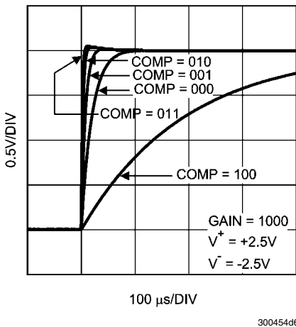
Large Signal Step Response for Various COMP Settings
