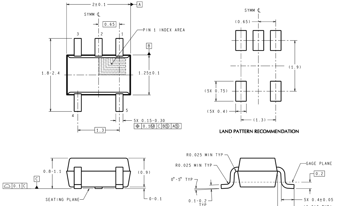
5-Pin SC70 NS Package Number MAA05A
