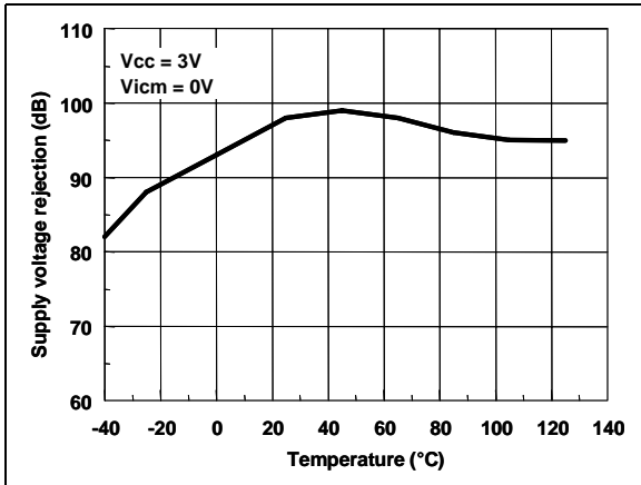
Figure 9. Supply voltage rejection vs. temperature
