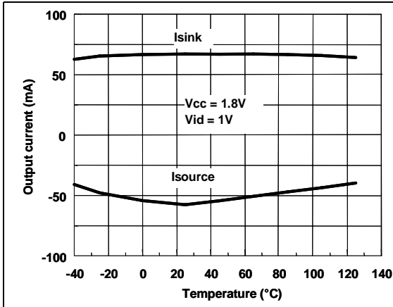
Figure 19. Output current vs. temperature
