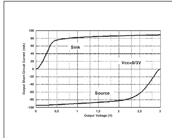
OUTPUT SHORT CIRCUIT CURRENT vs OUTPUT VOLTAGE
