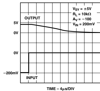
TPC 33. Negative Overvoltage Recovery
