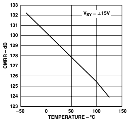
TPC 22. CMRR vs. Temperature
