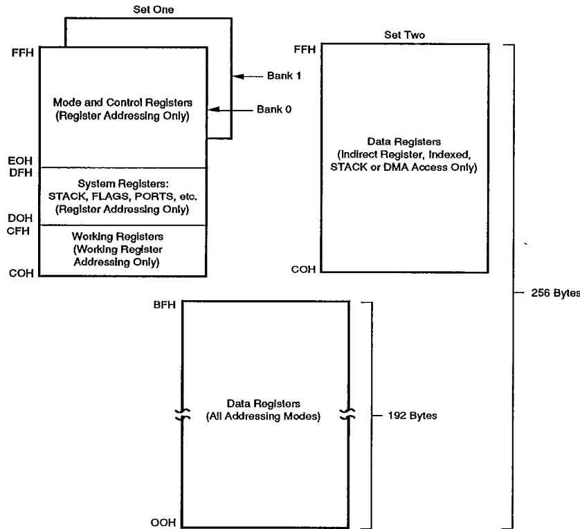
Figure 6. Super8 Registers
