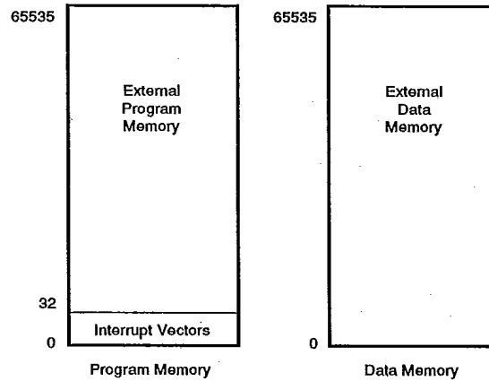
Figure 9. Program and Data Memory Address Space
