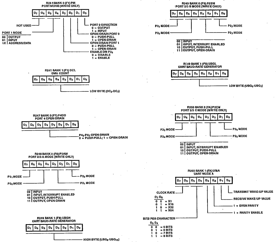
Figure 8. Mode and Control Registers (Continued)
