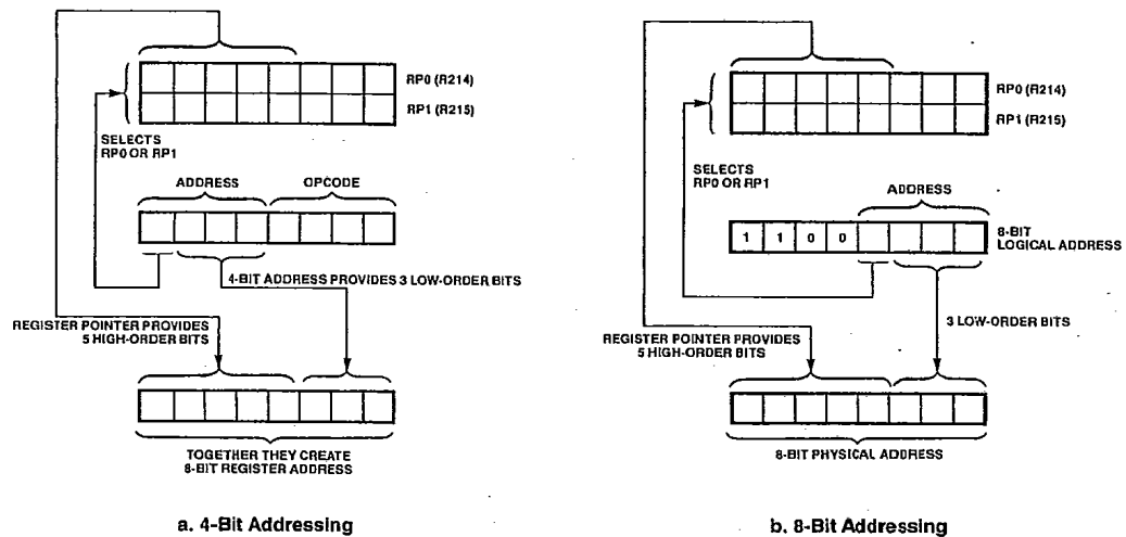
Figure 7. Working Register Window
