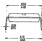
48-Lead DIP Package
