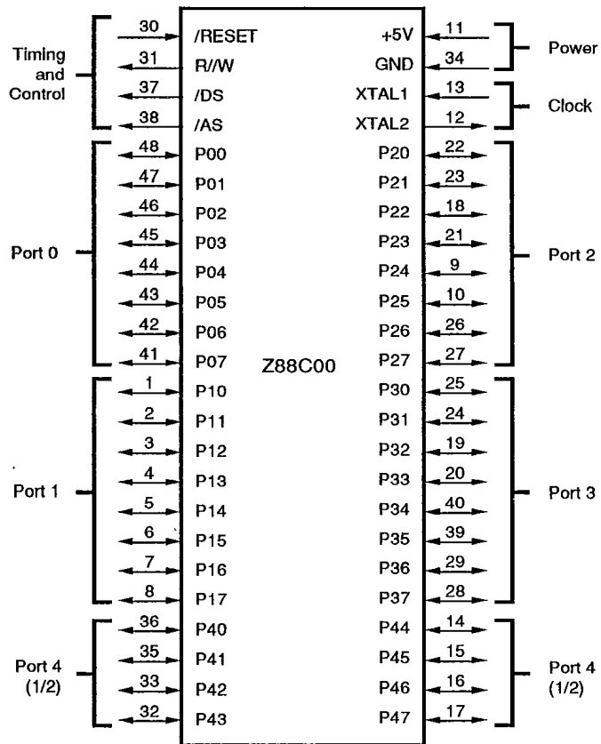
Figure 5. Pin Functions
