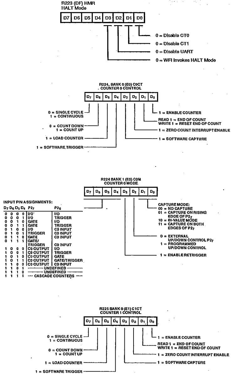
Figure 8. Mode and Control Registers (Continued)
