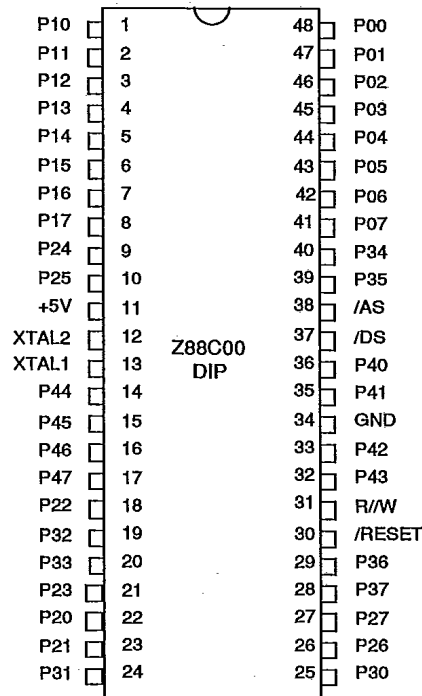
Figure 2. 48-Lead DIP Package
