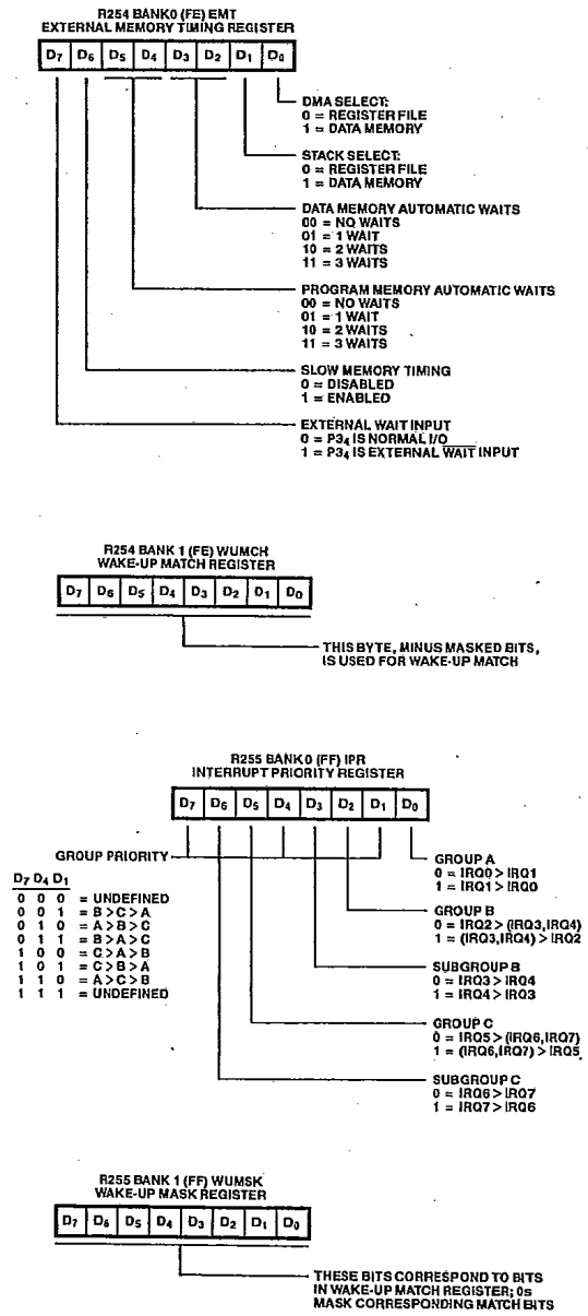
Figure 8. Mode and Control Registers (Continued)
