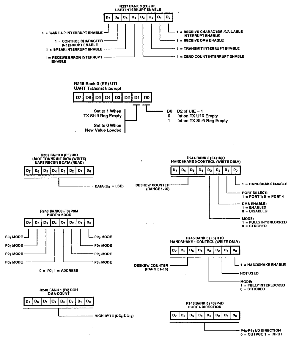
Figure 8. Mode and Control Registers
