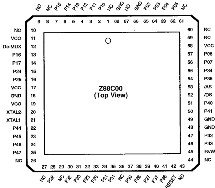
Figure 3. 68-Lead PLCC Package
