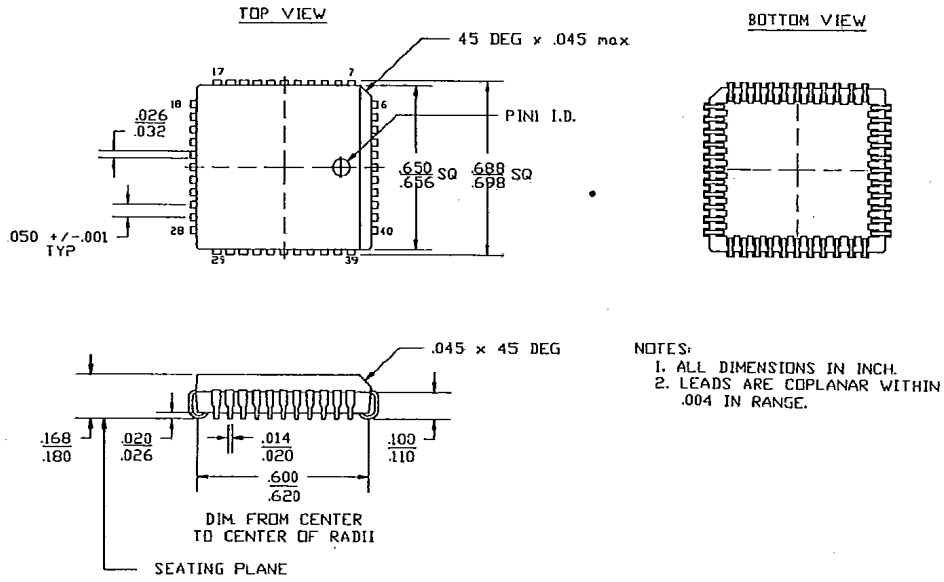
44-Lead PLCC Package
