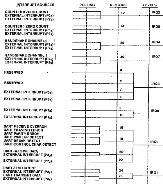
Figure 12. Interrupt Levels and Vectors
