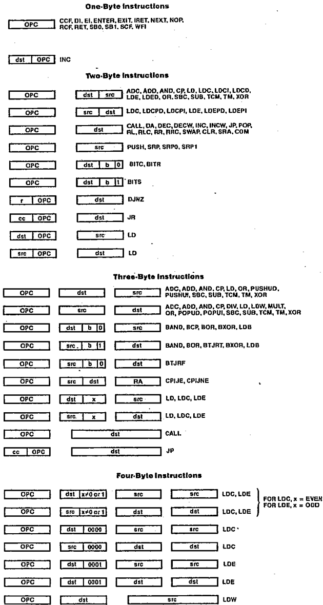
Figure 10. Instruction Formats
