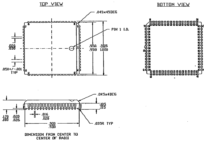
68-Lead PLCC Package
