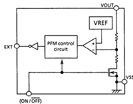
(2) S-8322 Series
