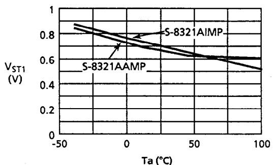
V_{ST1} vs. T_a
