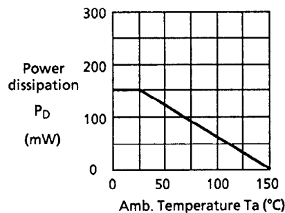
Figure 12 Power dissipation of the package (before mounting)
