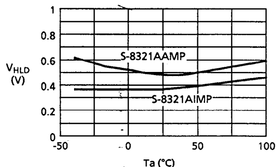
V_{HLD} vs. T_a
