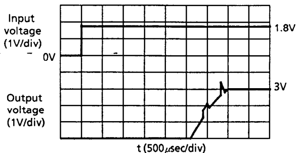
S-8322AI V_{IN} = 0 \rightarrow 1.8\text{V} , R_L = 250\Omega
