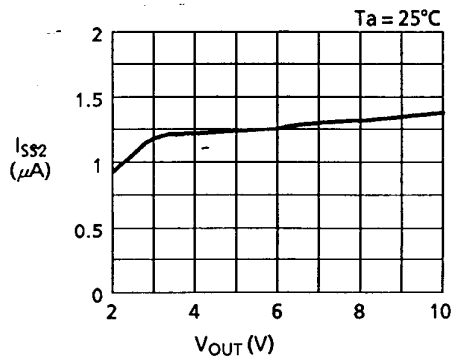
I_{SS2} vs. V_{OUT} , T_a
