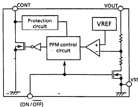
(1) S-8321 Series
