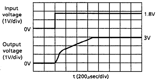
S-8321AI V_{IN} = 0 \rightarrow 1.8\text{V} , R_L = 250\Omega
