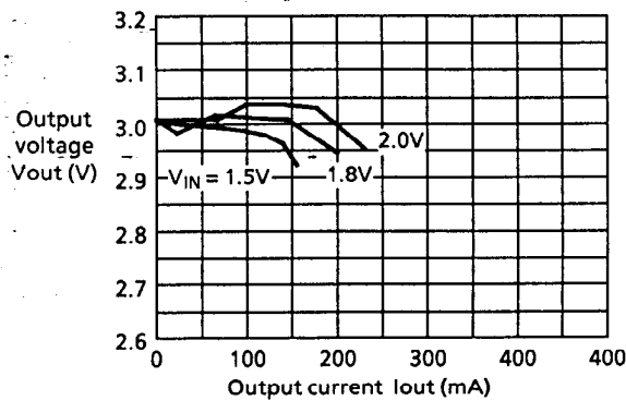
(c) Output current - Output voltage characteristics
