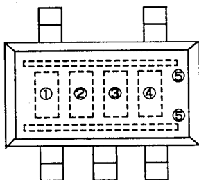
(1) S-8321/22AXMP
