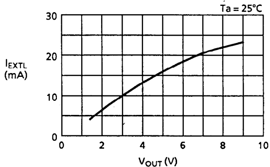
I_{EXTL} vs. V_{OUT} , T_a
