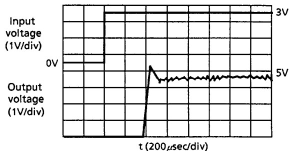
S-8321AA V_{IN} = 0 \rightarrow 3\text{V} , R_L = 250\Omega
