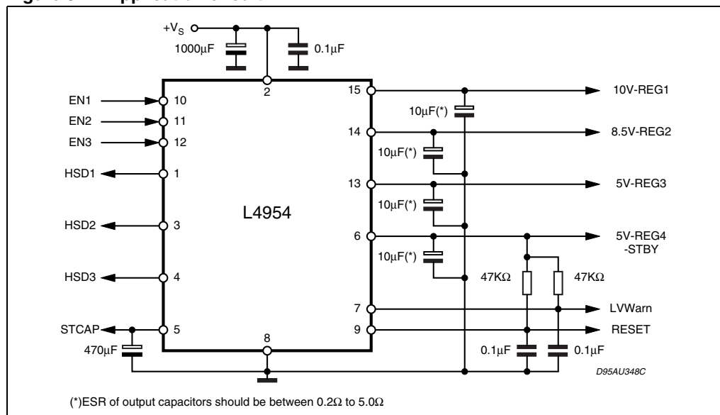
Figure 3. Application circuit
