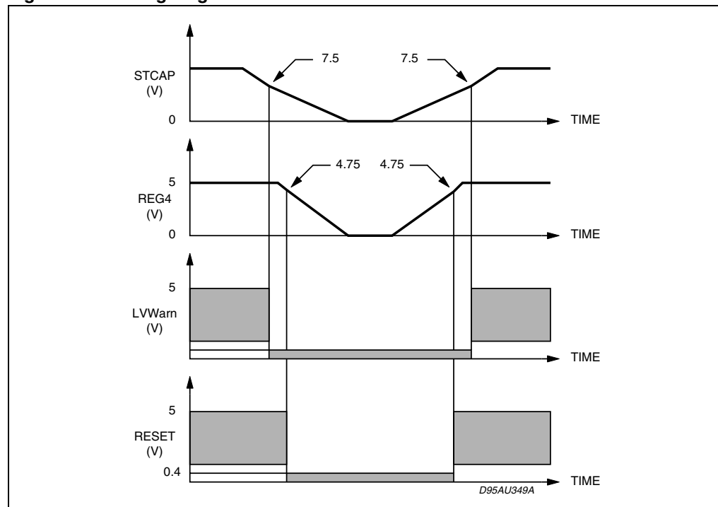
Figure 4. Timing diagram
