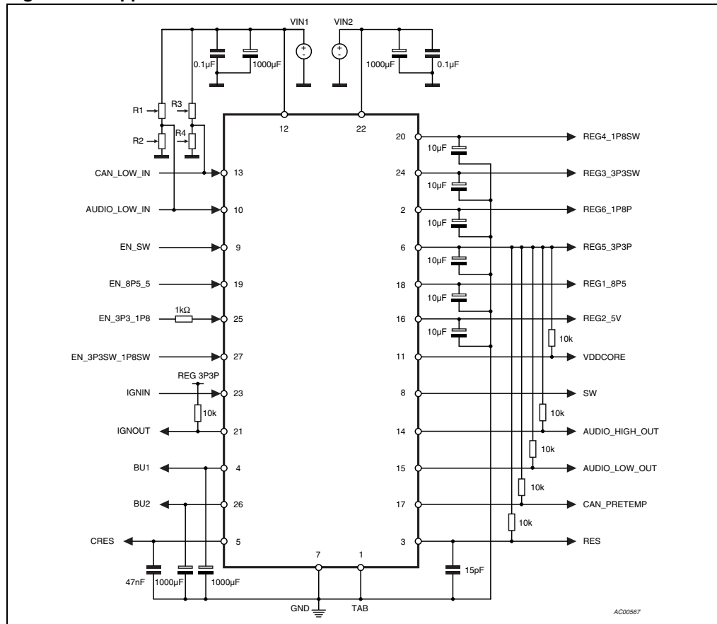
Figure 3. Application circuit
