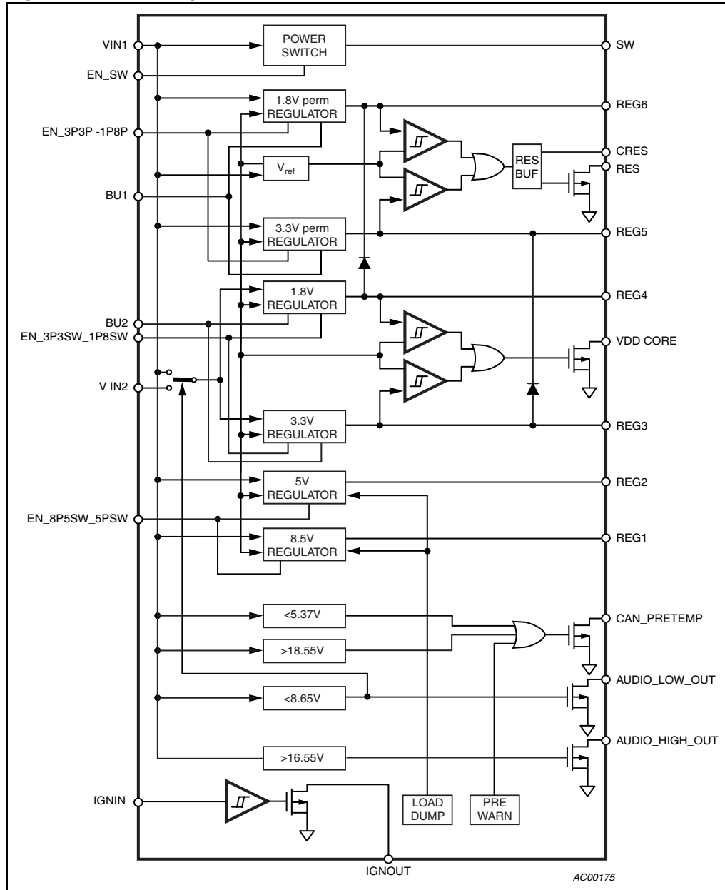
Figure 1. Block diagram
