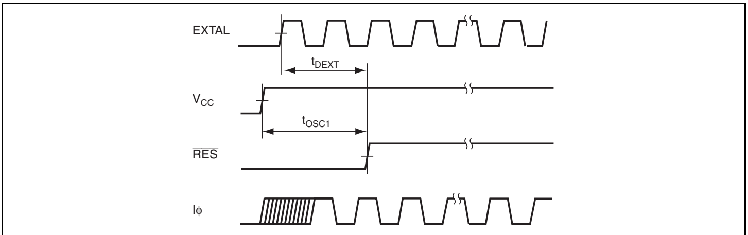
Figure 21.4 Oscillation Settling Timing
