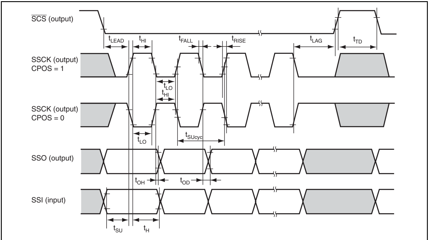
Figure 21.17 SSU Timing (Master, CPHS = 1)
