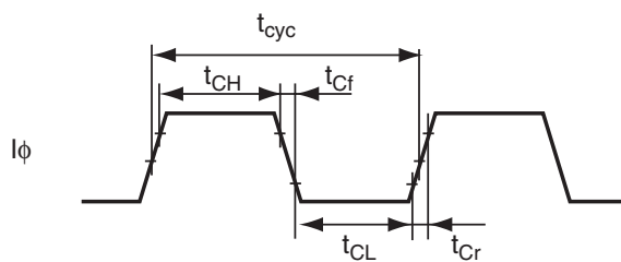
Figure 21.2 System Bus Clock Timing
