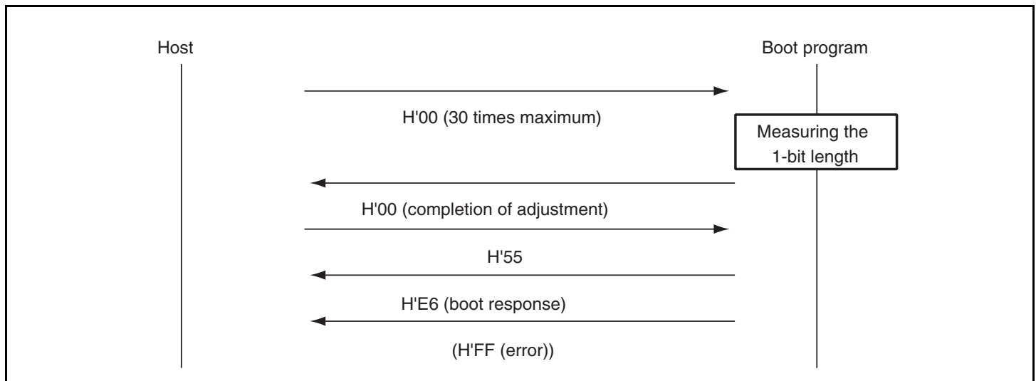
Figure 17.22 Bit-Rate-Adjustment Sequence
