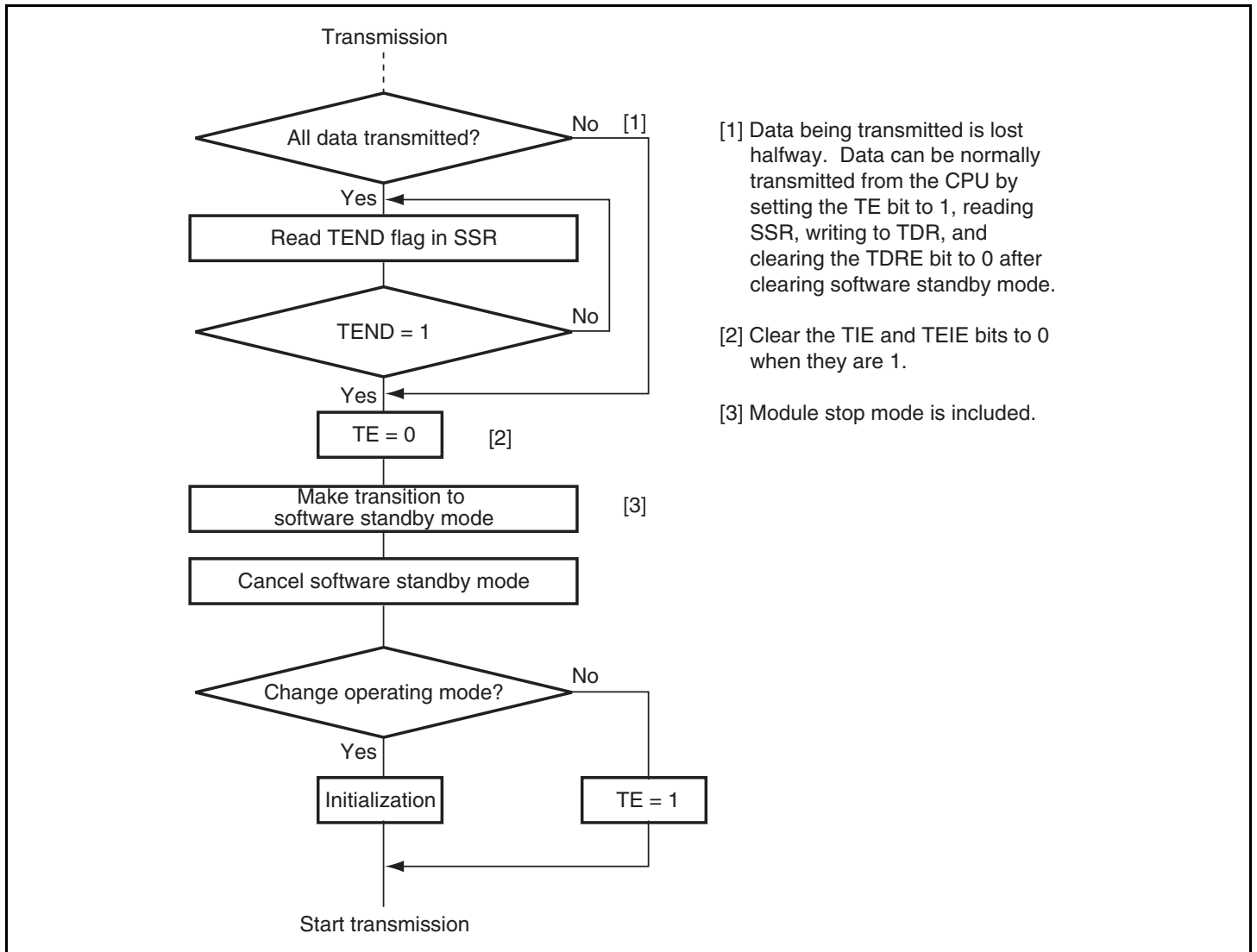
Figure 12.34 Sample Flowchart for Mode Transition during Transmission
