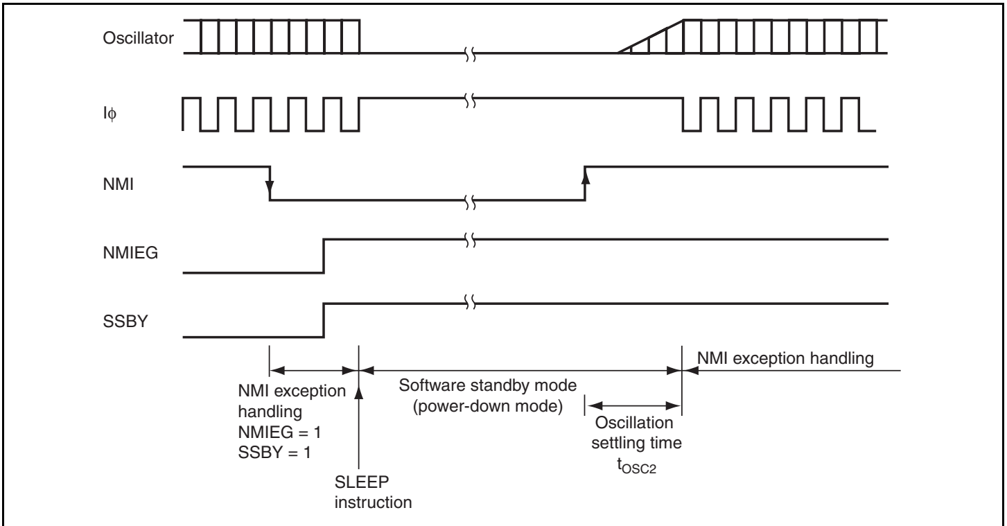
Figure 21.3 Oscillation Settling Timing after Software Standby Mode
