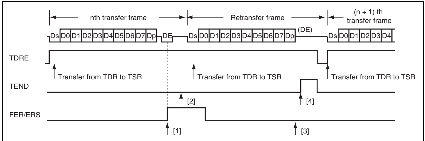
Figure 12.26 Data Re-Transfer Operation in SCI Transmission Mode
