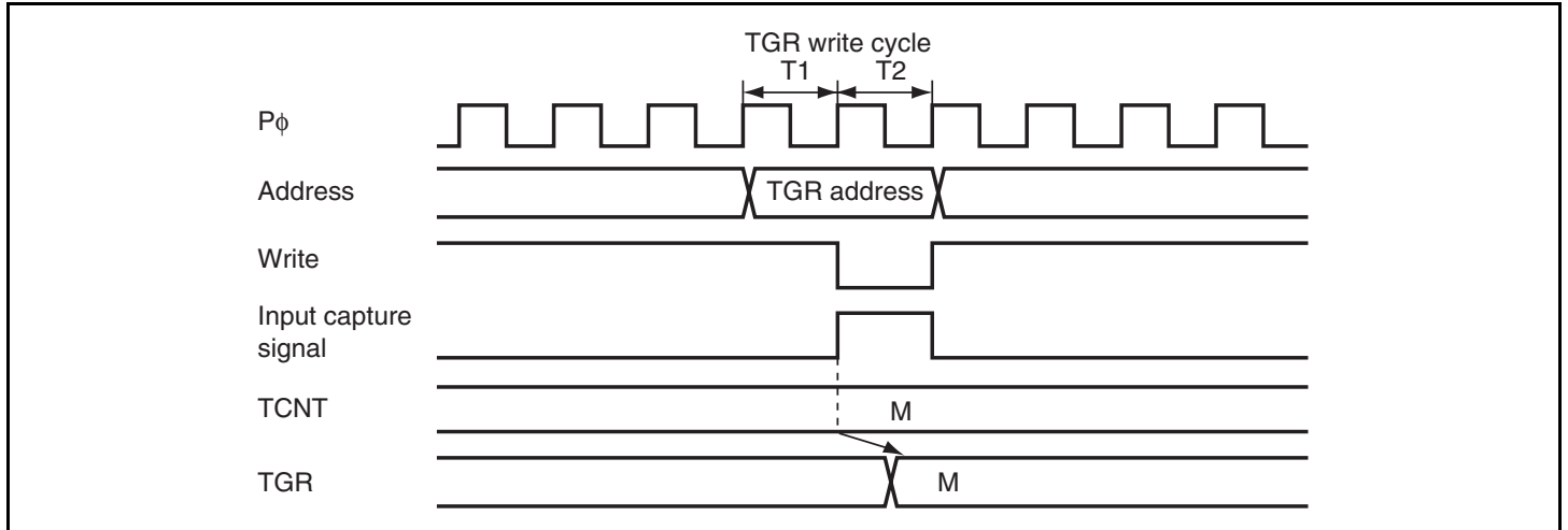
Figure 9.52 Conflict between TGR Write and Input Capture
