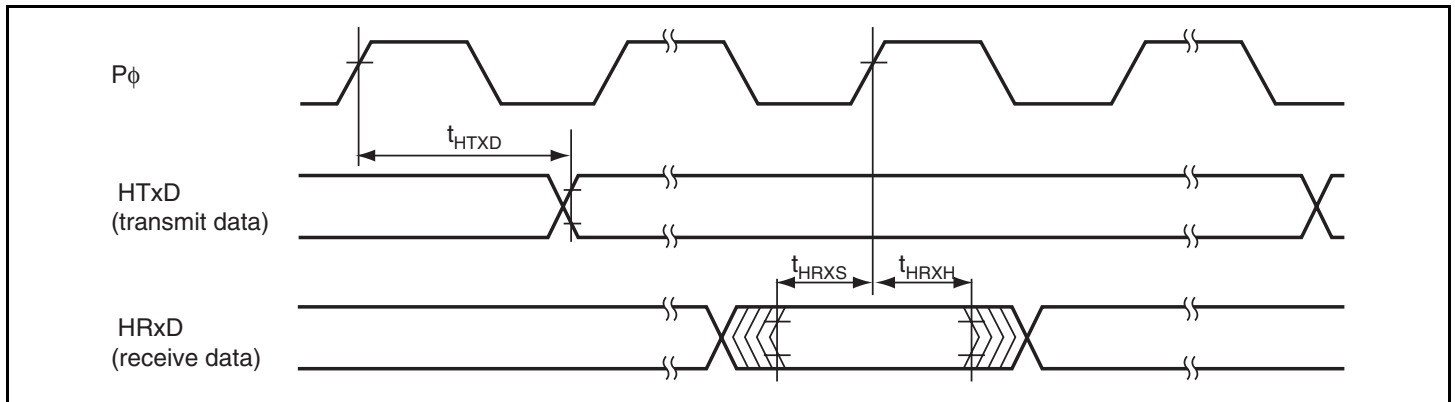
Figure 21.16 HCAN Input/Output Timing
