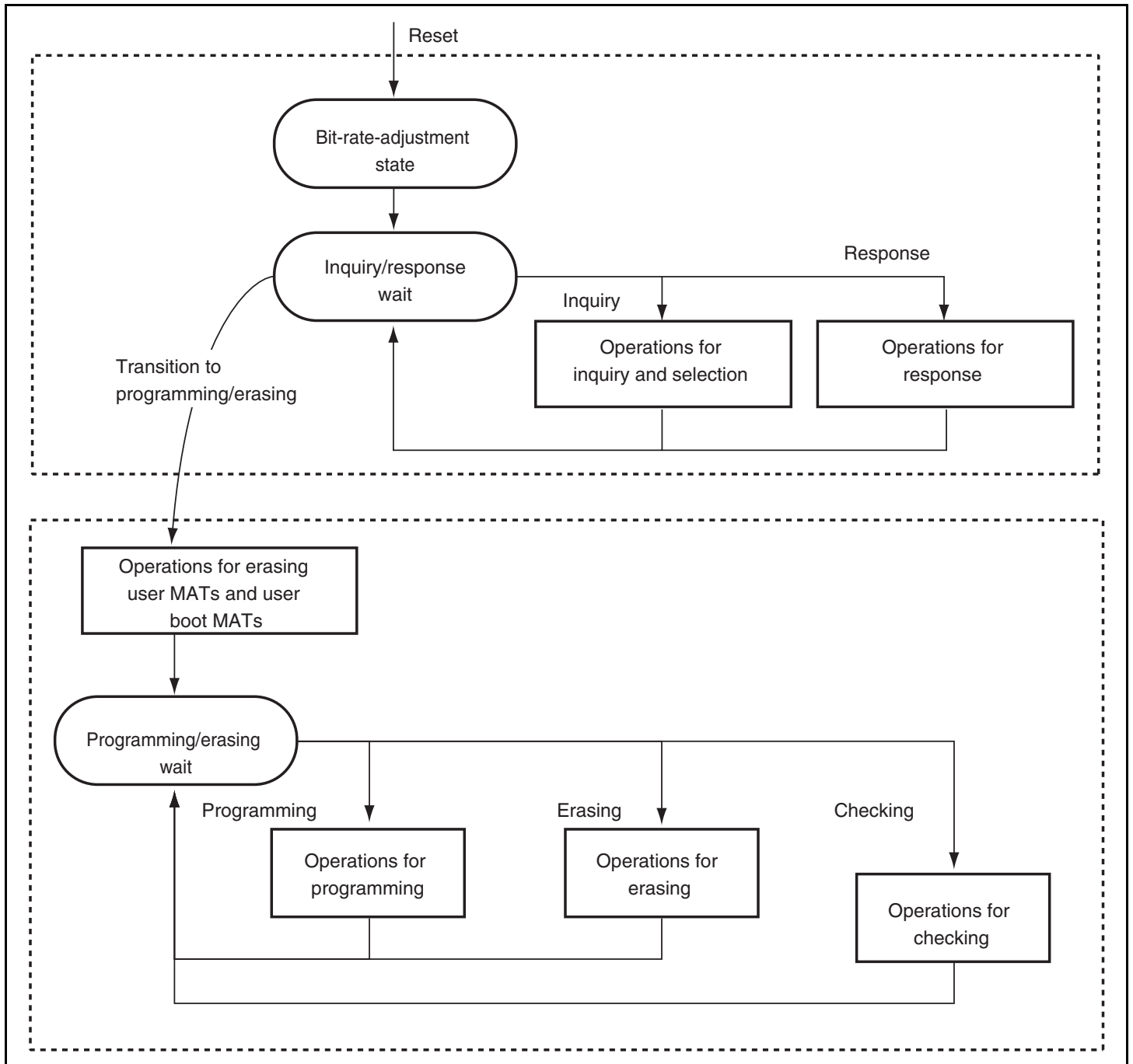
Figure 17.21 Boot Program States
