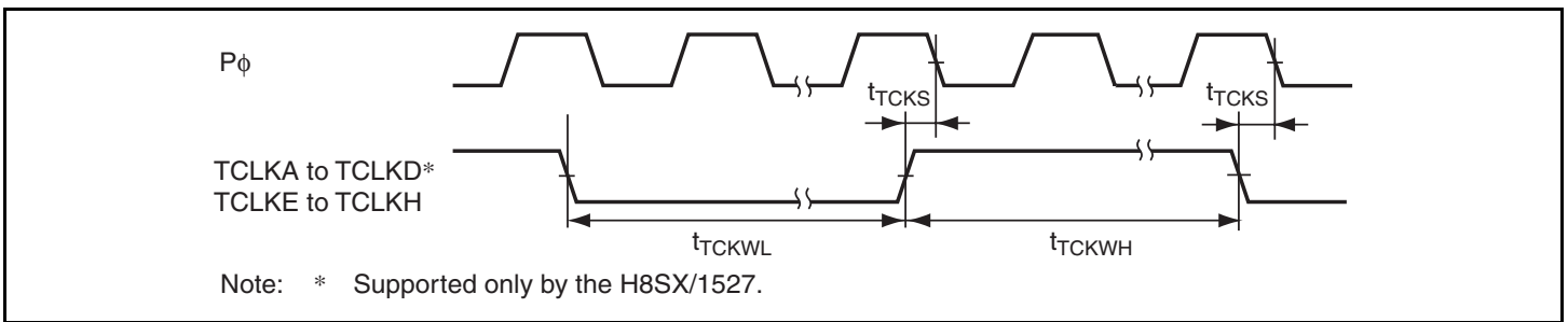
Figure 21.11 TPU Clock Input Timing
