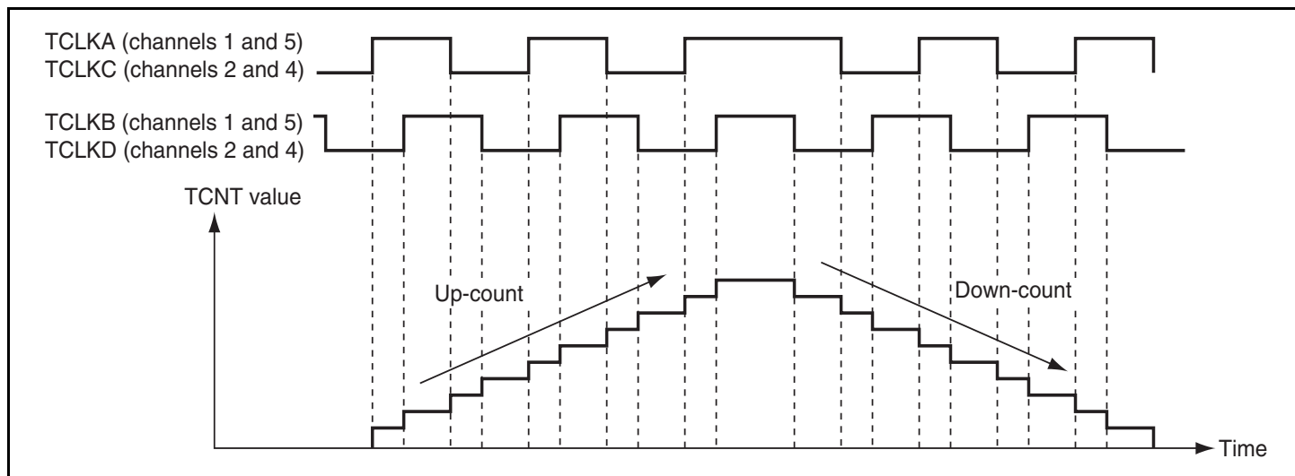
Figure 9.26 Example of Phase Counting Mode 1 Operation
