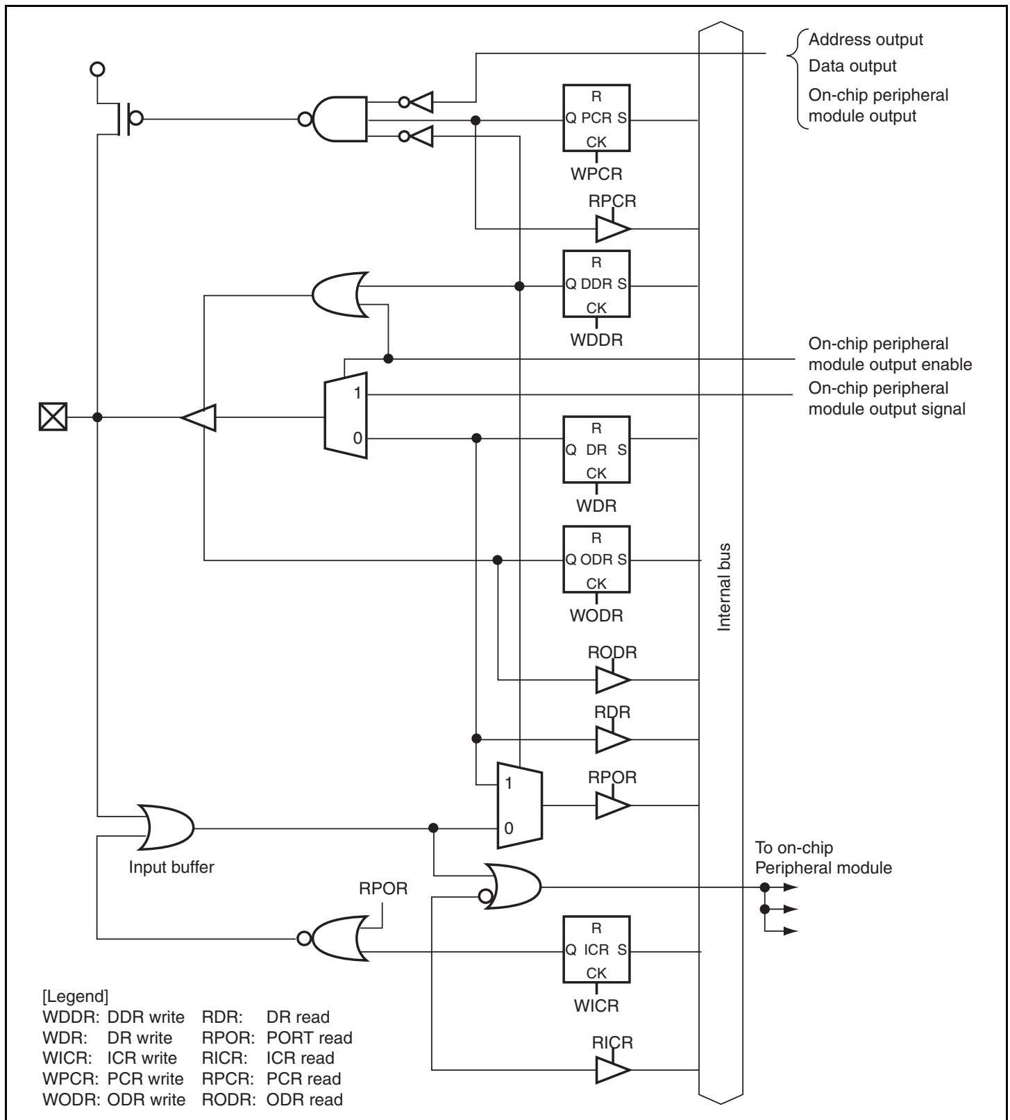
Figure 8.1 Port Block Diagram
