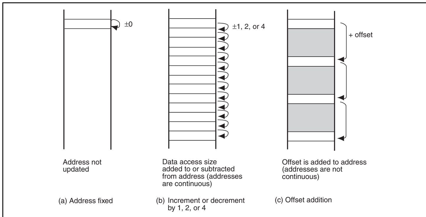
Figure 7.17 Address Update Method
