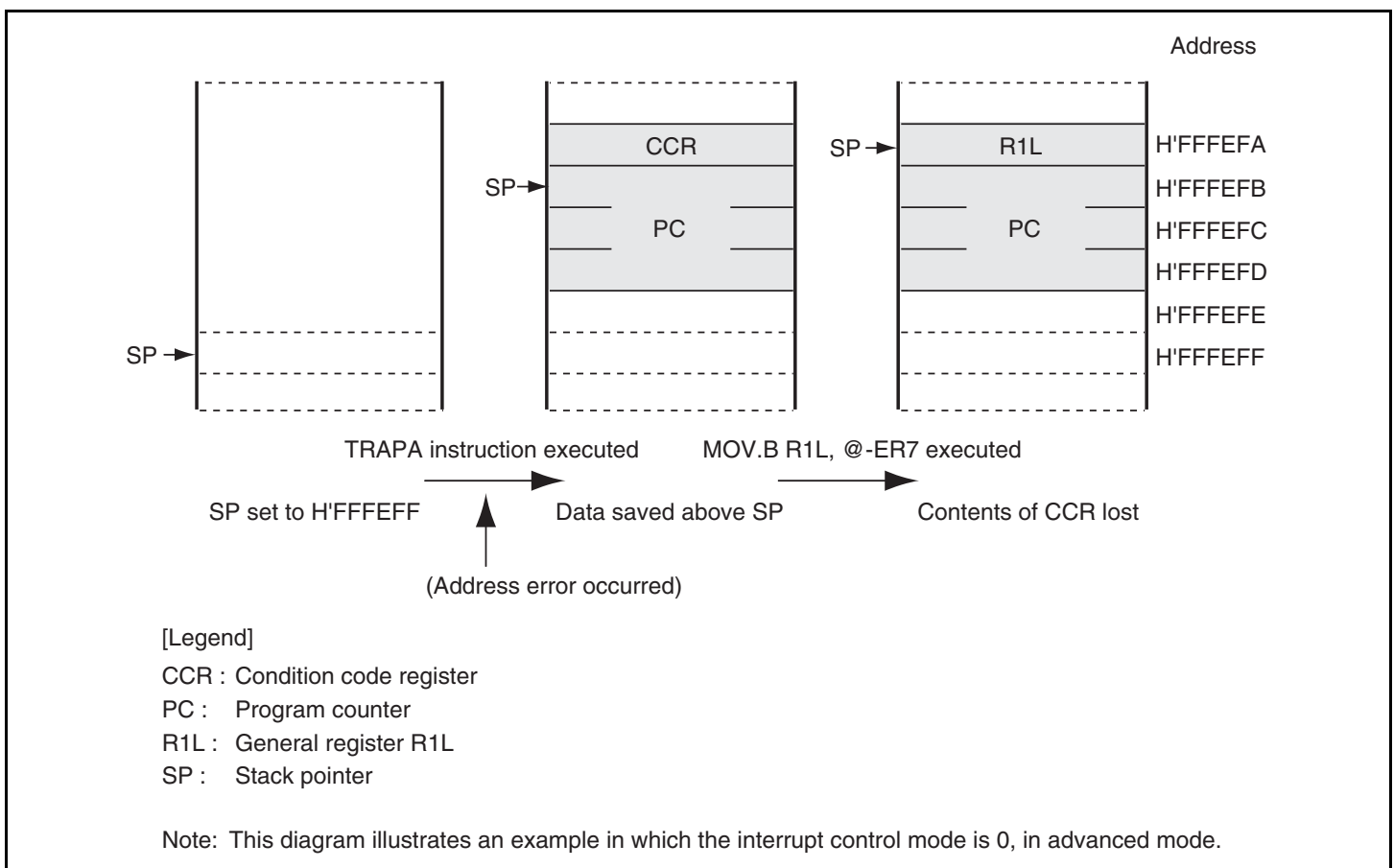
Figure 4.3 Operation when SP Value Is Odd
