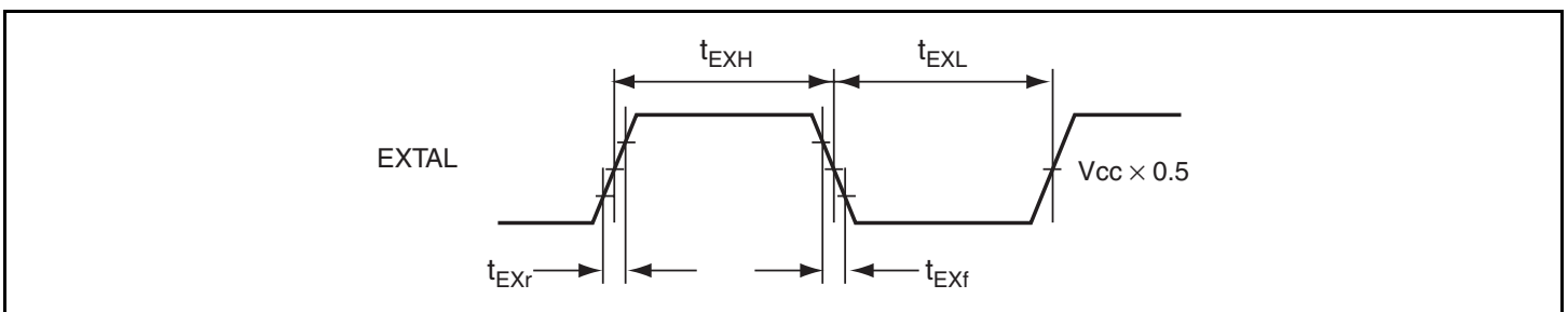
Figure 21.5 External Input Clock Timing
