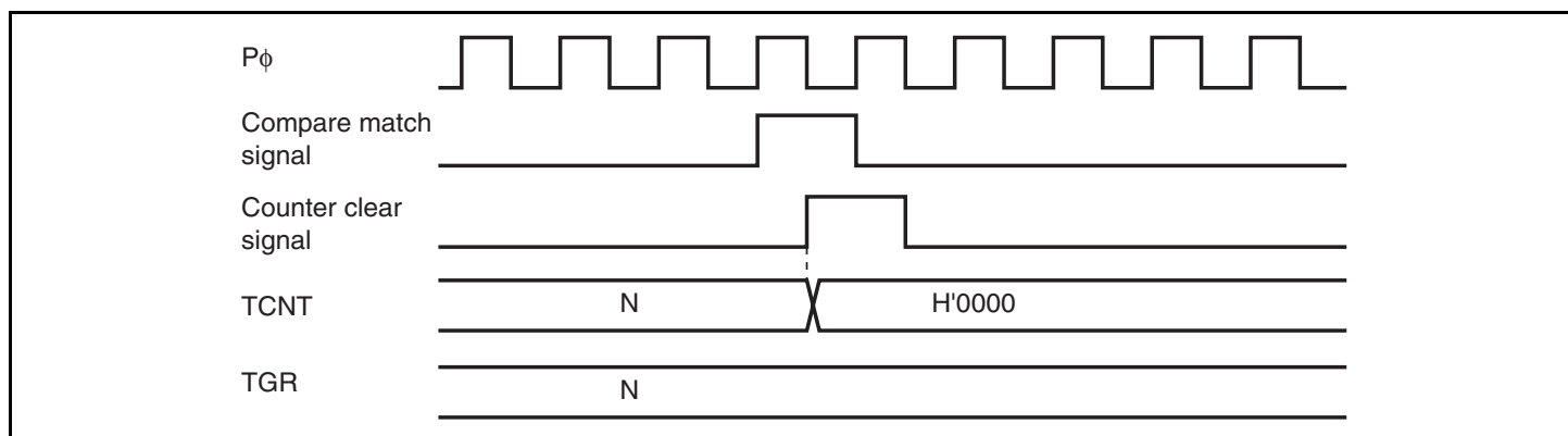
Figure 9.35 Counter Clear Timing (Compare Match)
