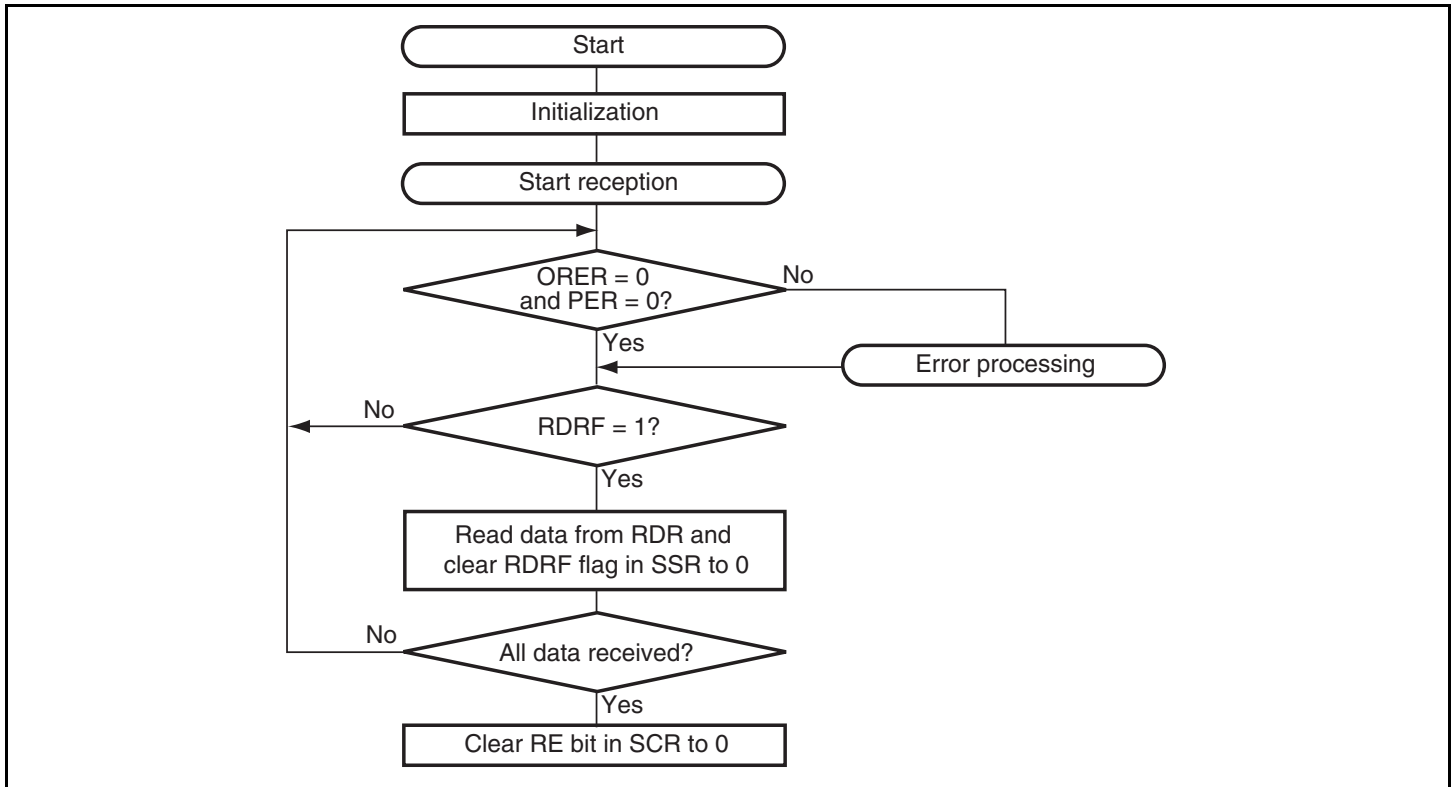
Figure 12.30 Sample Reception Flowchart
