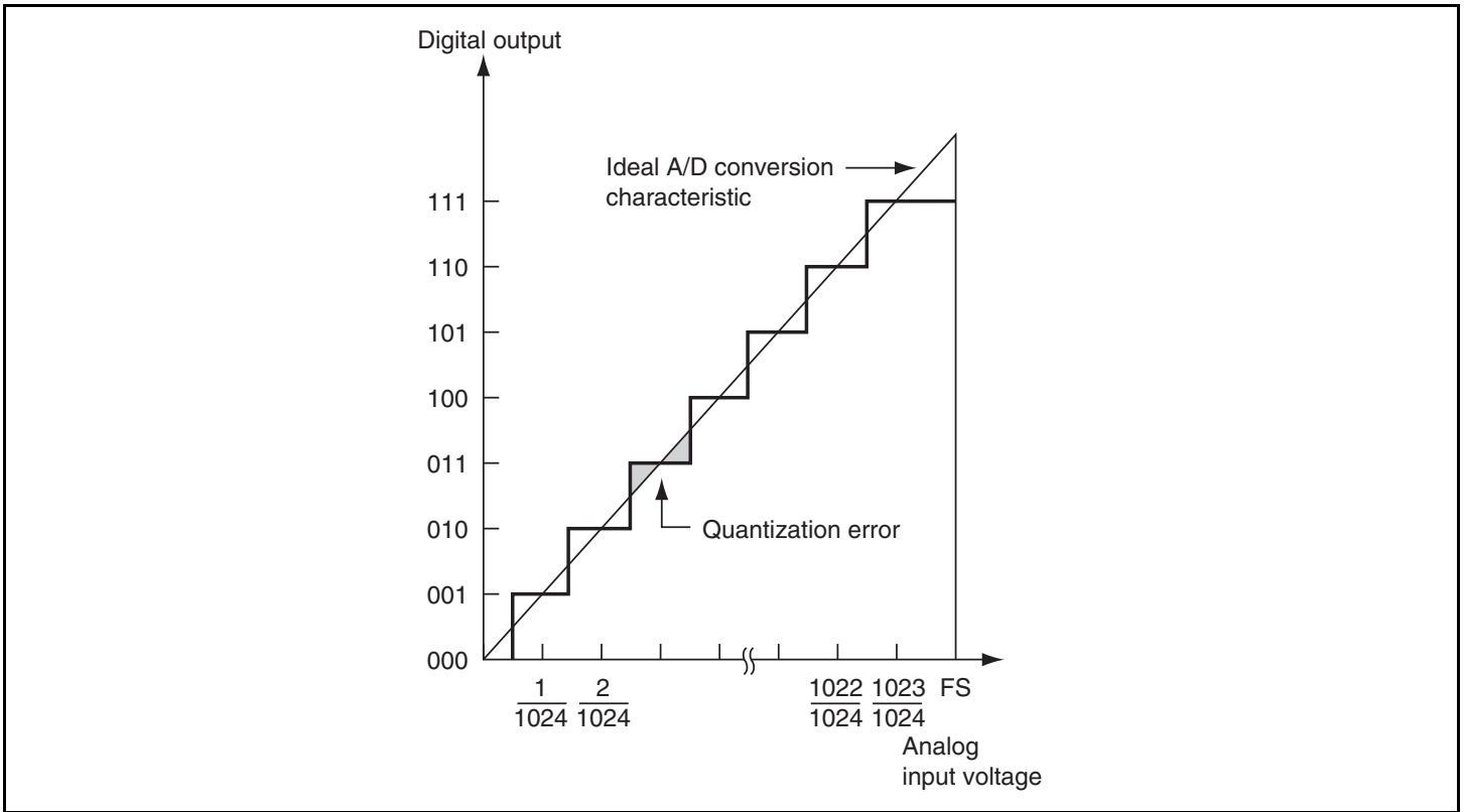
Figure 15.7 A/D Conversion Accuracy Definitions
