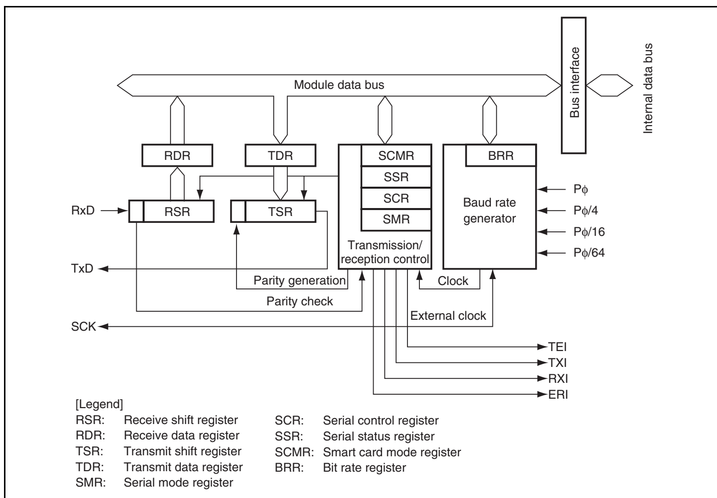
Figure 12.1 Block Diagram of SCI
