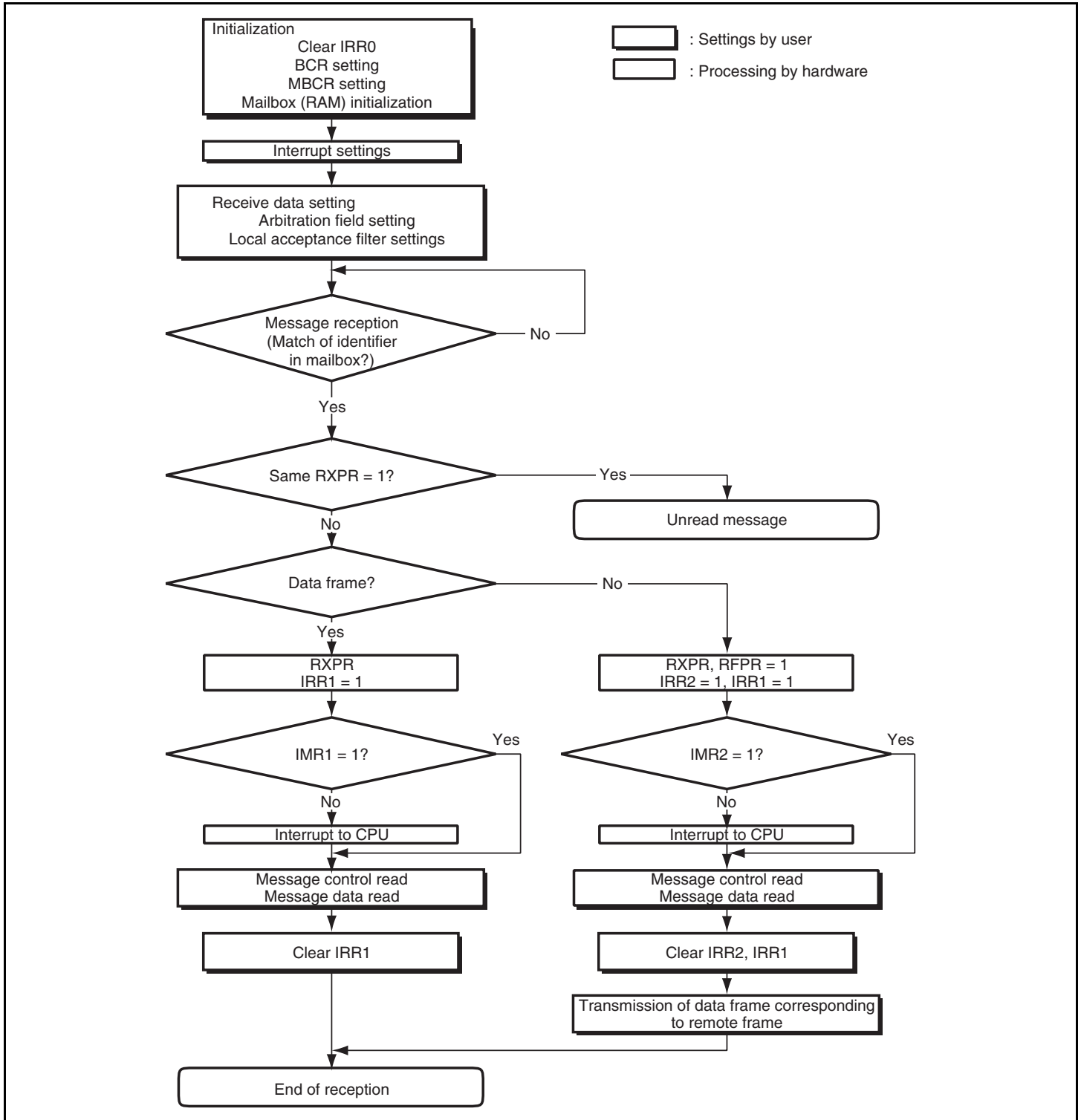
Figure 13.11 Reception Flowchart
