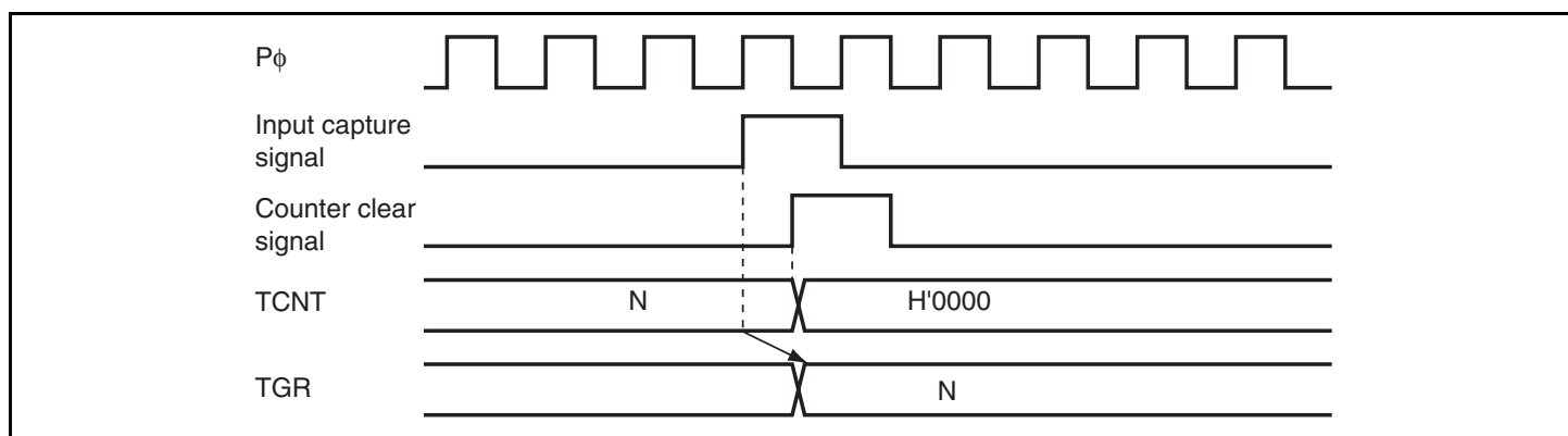
Figure 9.36 Counter Clear Timing (Input Capture)
