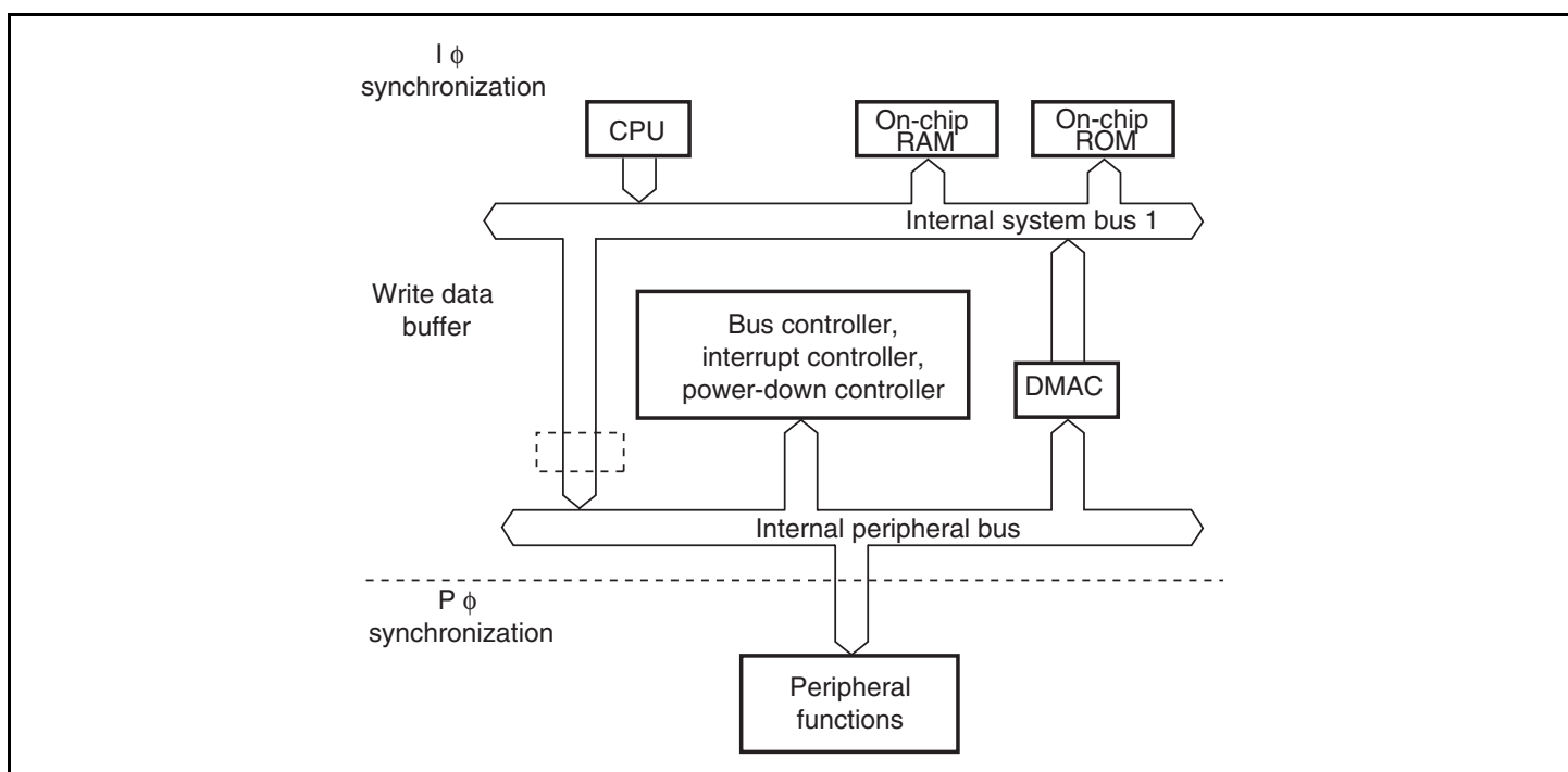
Figure 6.2 Internal Bus Configuration
