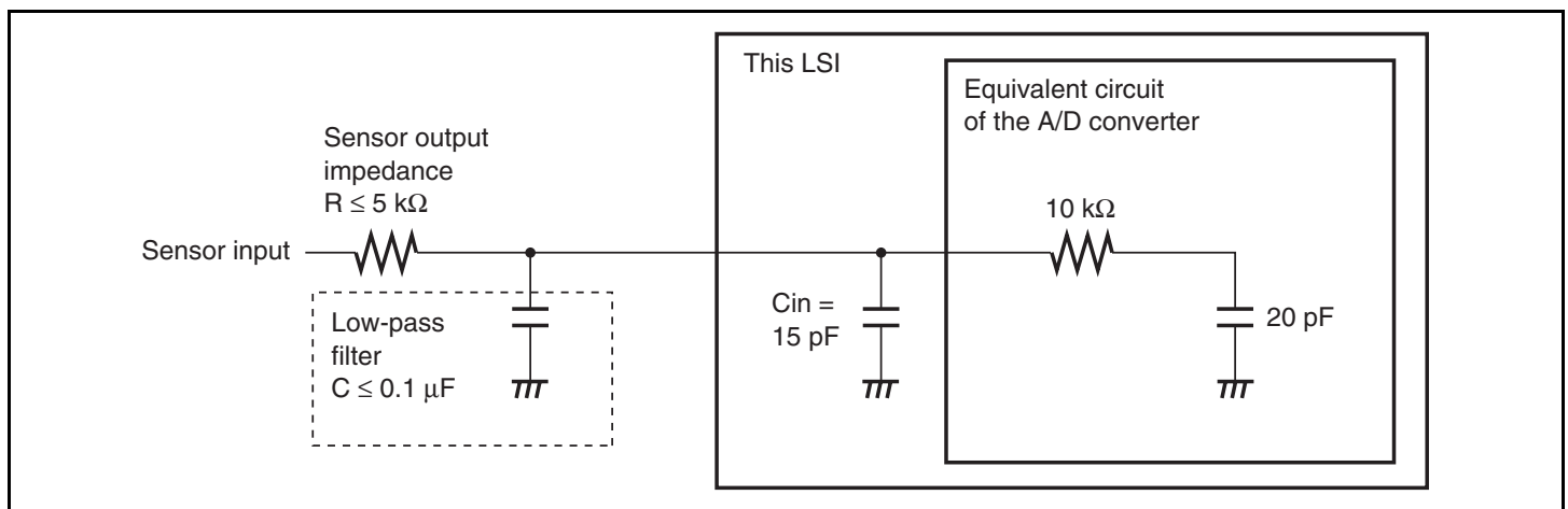
Figure 15.9 Example of Analog Input Circuit
