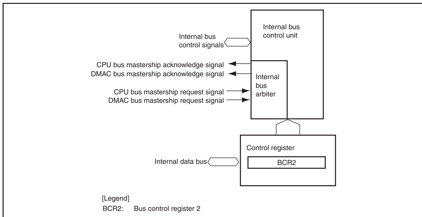
Figure 6.1 Block Diagram of Bus Controller
