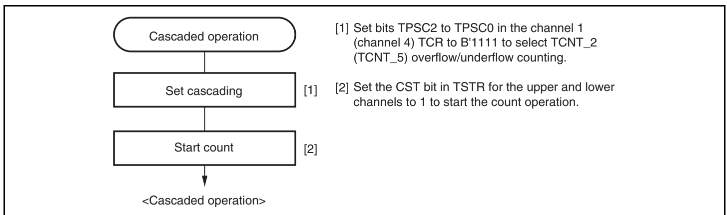
Figure 9.18 Example of Cascaded Operation Setting Procedure
