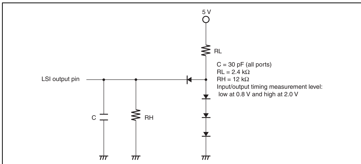
Figure 21.1 Output Load Circuit
