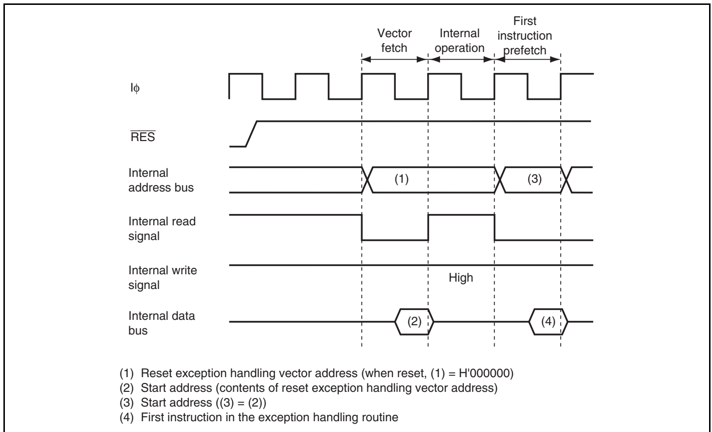
Figure 4.1 Reset Sequence (On-Chip ROM Enabled Advanced Mode)
