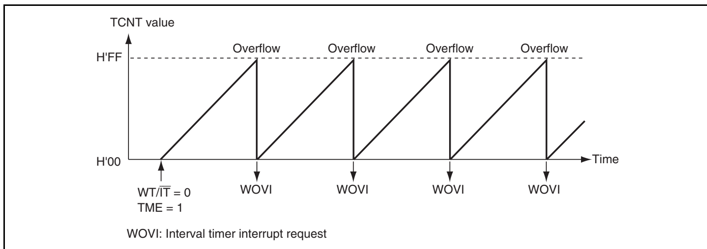
Figure 11.3 Operation in Interval Timer Mode
