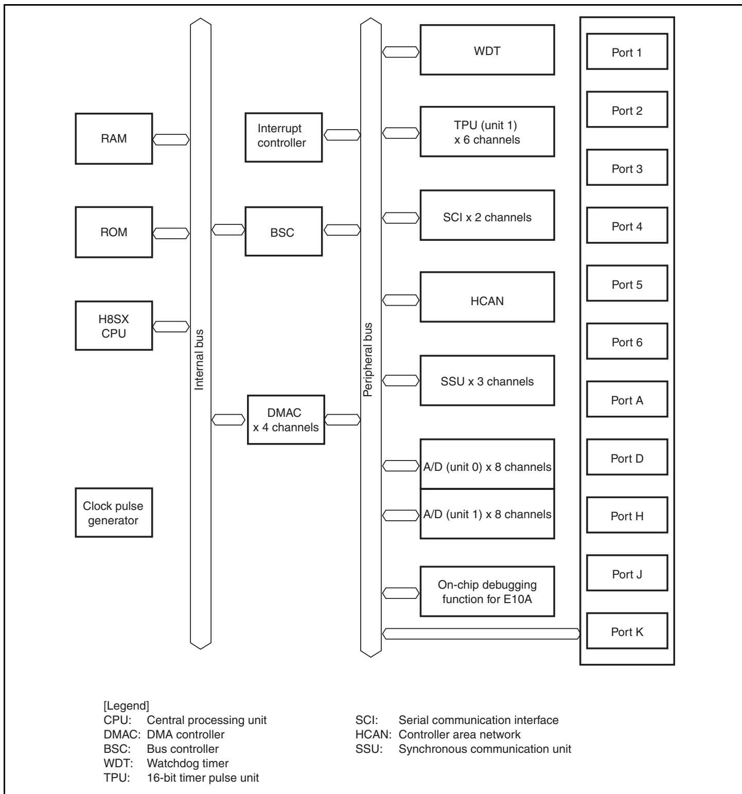
Figure 1.2 Block Diagram of H8SX/1525
