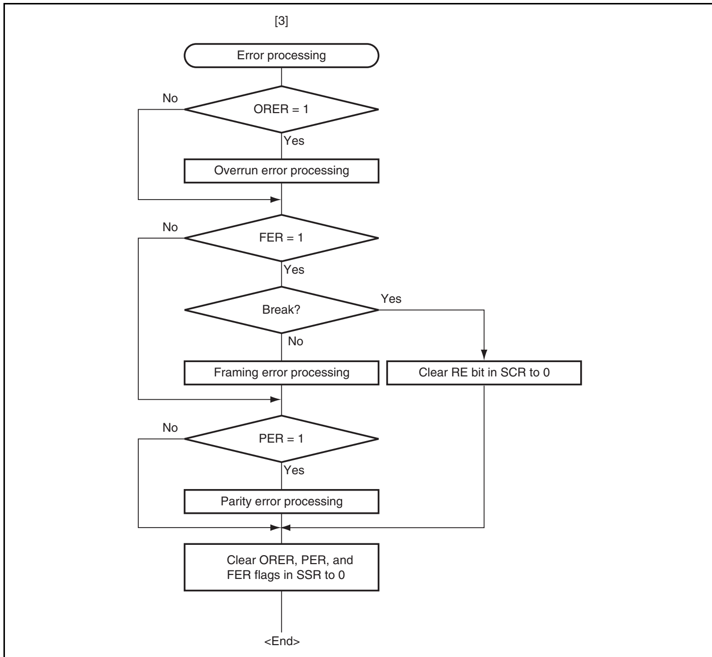
Figure 12.9 Sample Serial Reception Flowchart (2)
