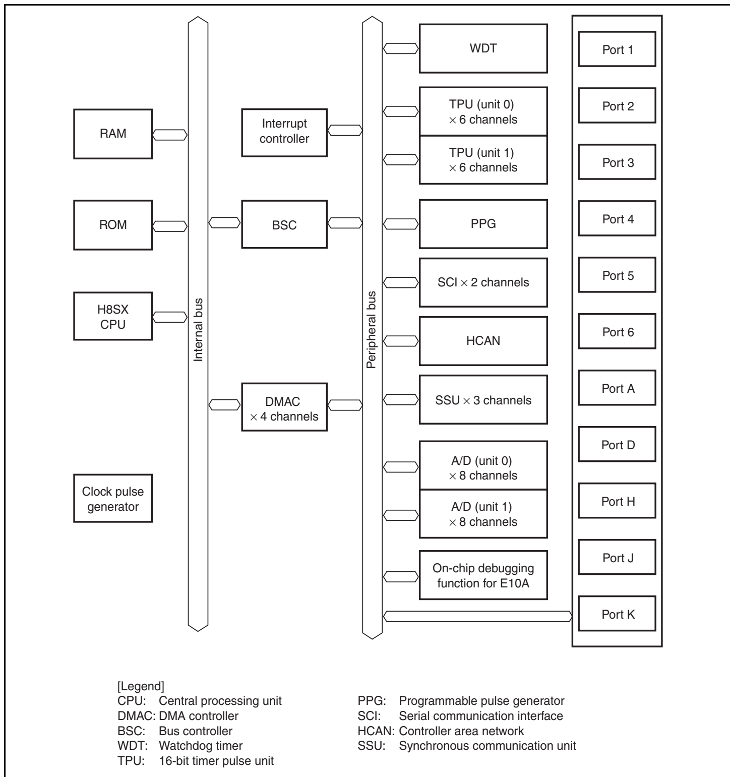
Figure 1.1 Block Diagram of H8SX/1527
