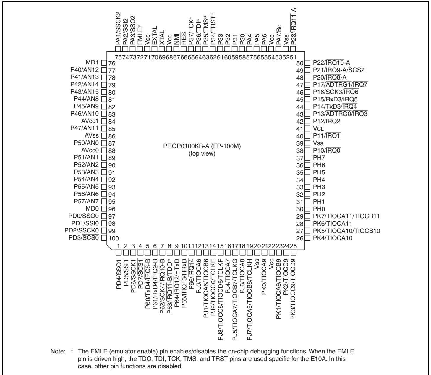
Figure 1.4 Pin Assignments of H8SX/1525
