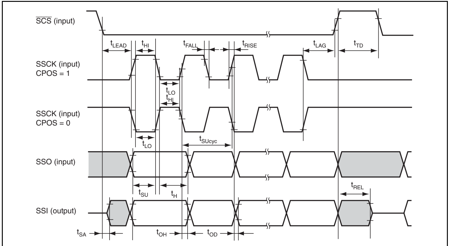
Figure 21.20 SSU Timing (Slave, CPHS = 0)
