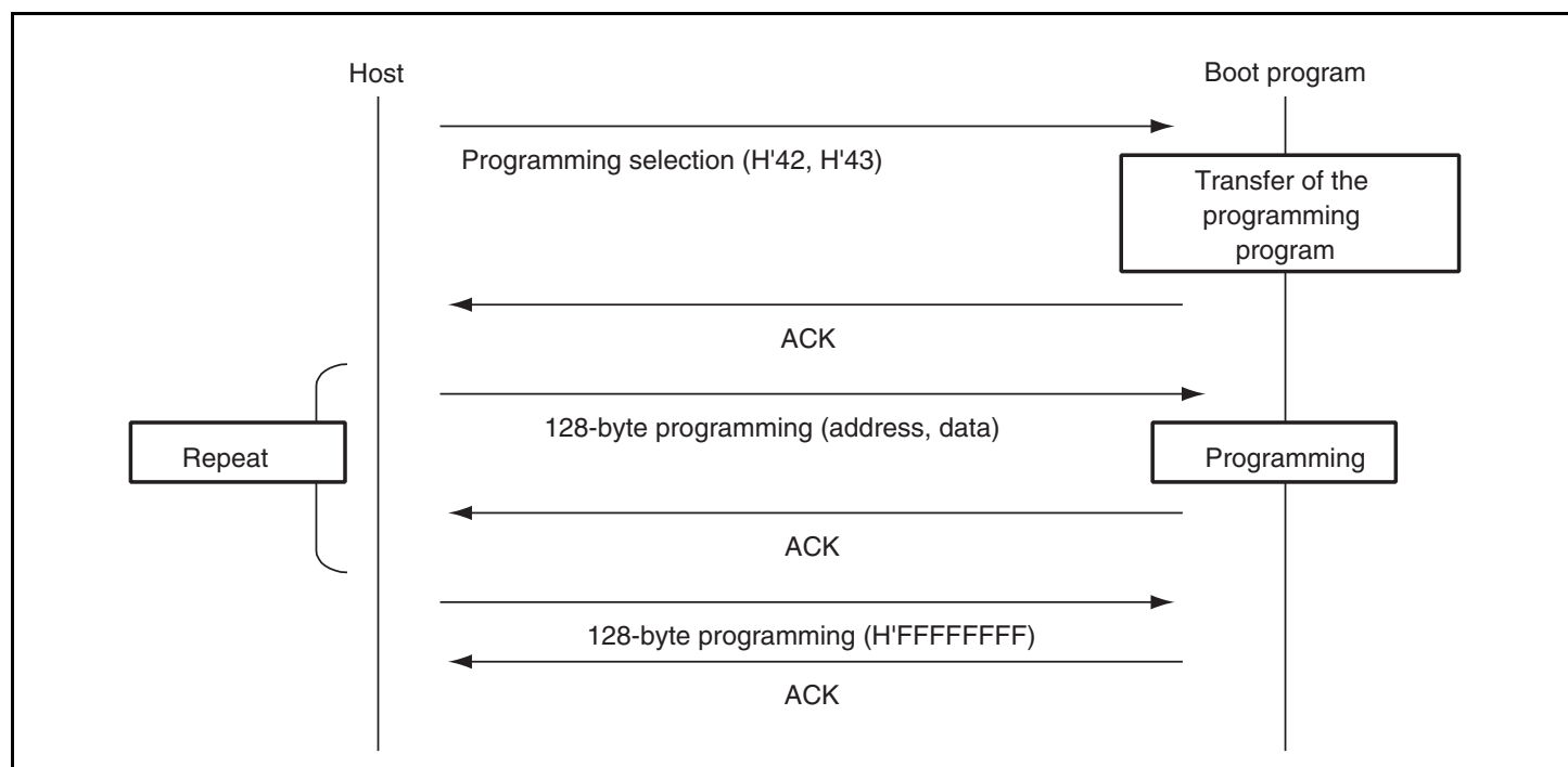
Figure 17.25 Programming Sequence
