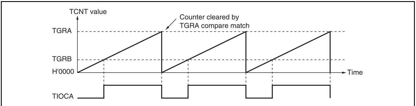
Figure 9.22 Example of PWM Mode Operation (1)
