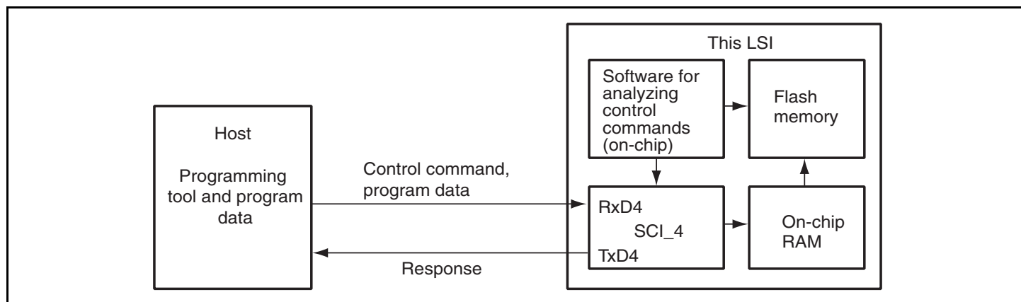
Figure 17.6 System Configuration in Boot Mode
