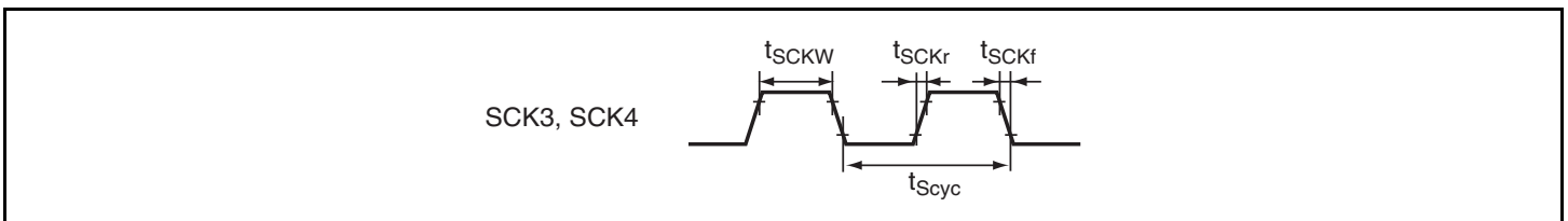
Figure 21.13 SCK Clock Input/Output Timing
