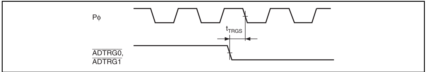
Figure 21.15 A/D Converter External Trigger Input Timing
