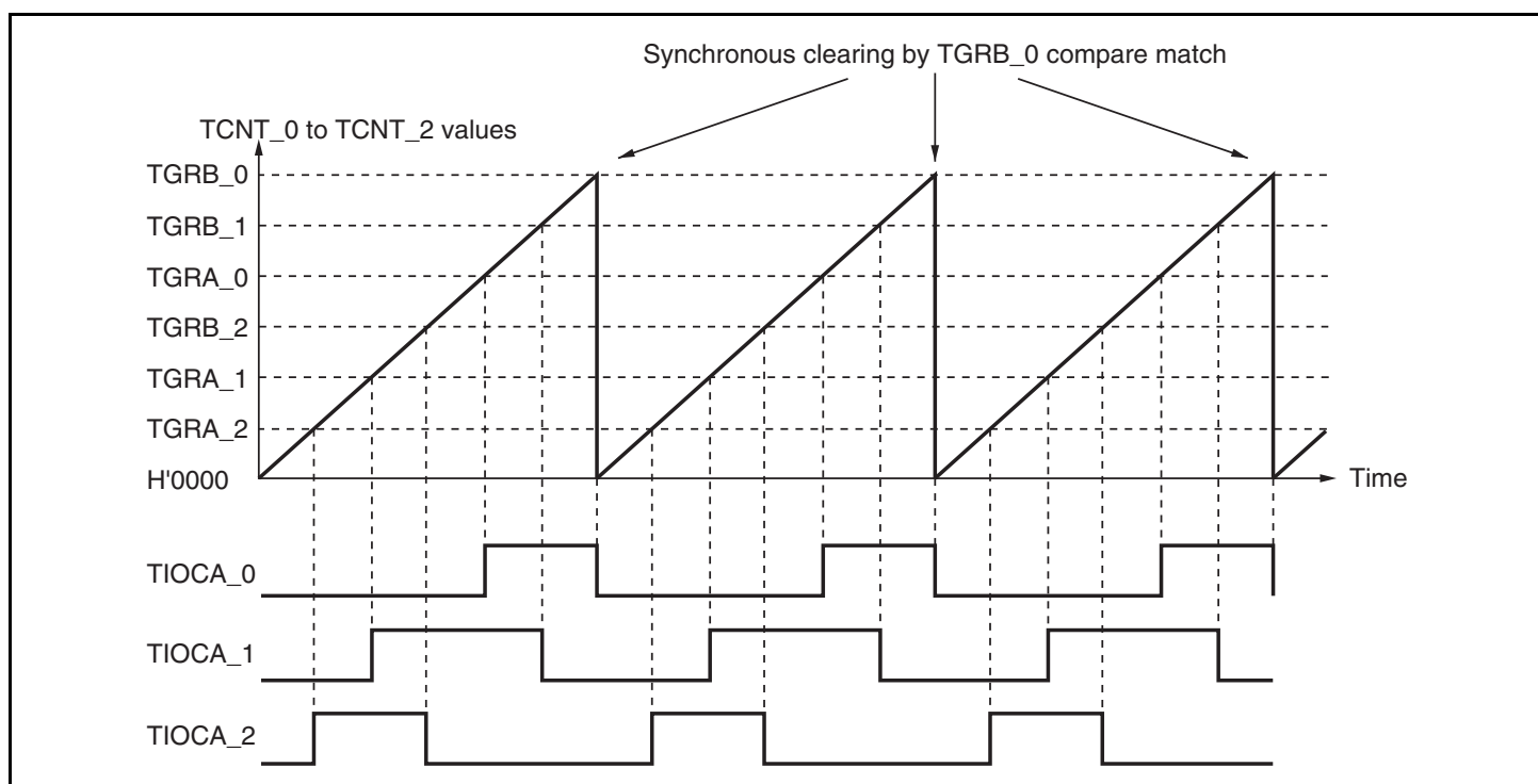
Figure 9.12 Example of Synchronous Operation
