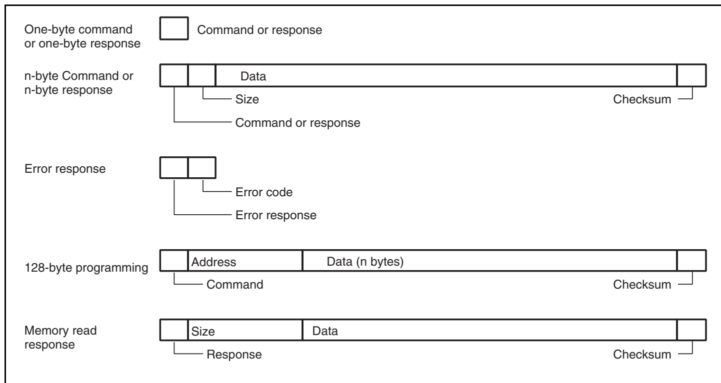
Figure 17.23 Communication Protocol Format
