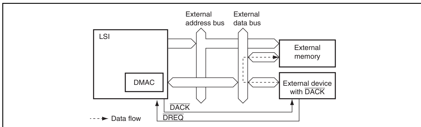
Figure 7.4 Data Flow in Single Address Mode
