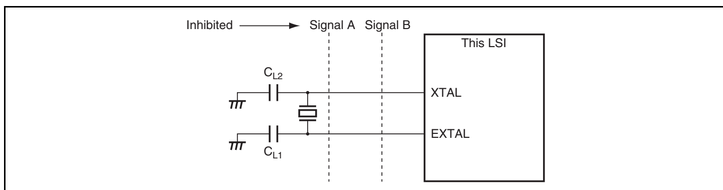
Figure 18.6 Note on Board Design for Oscillation Circuit
