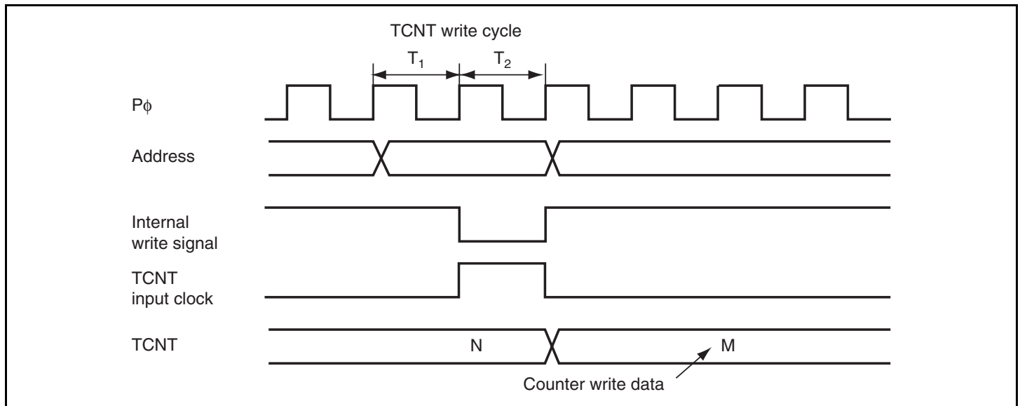
Figure 11.5 Conflict between TCNT Write and Increment
