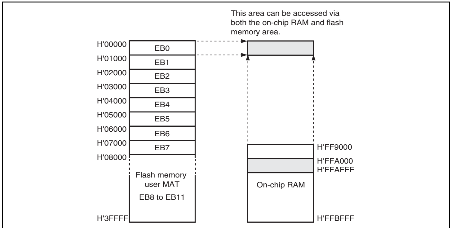
Figure 17.18 Address Map of Overlaid RAM Area
