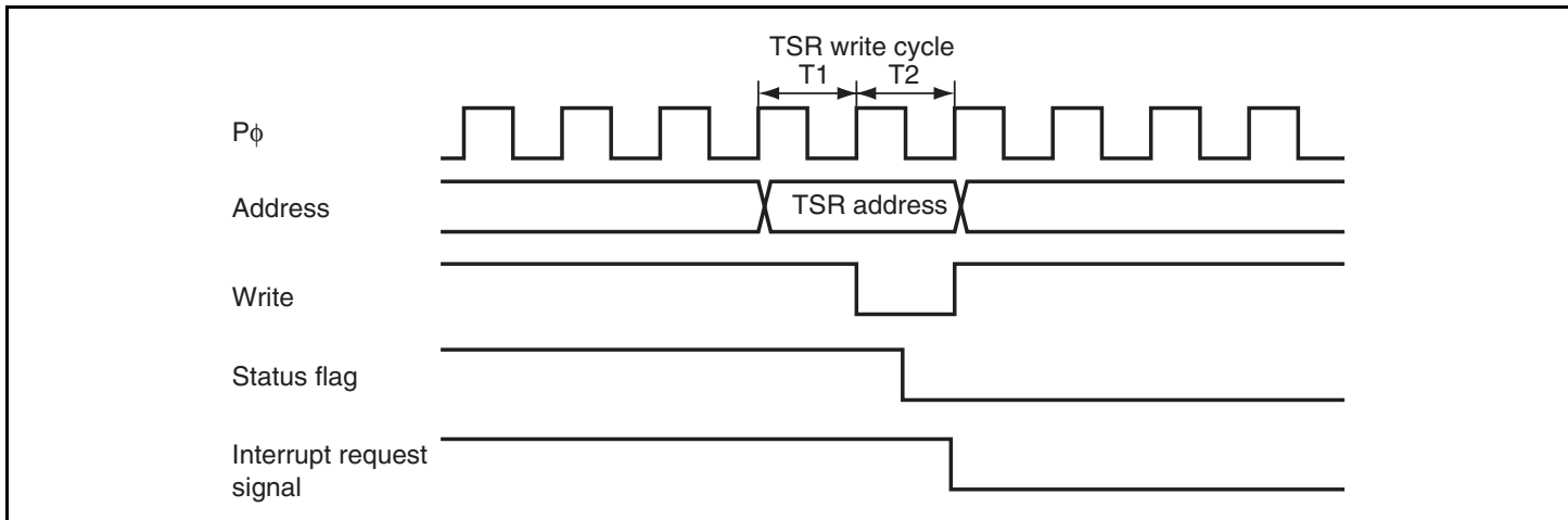
Figure 9.43 Timing for Status Flag Clearing by CPU
