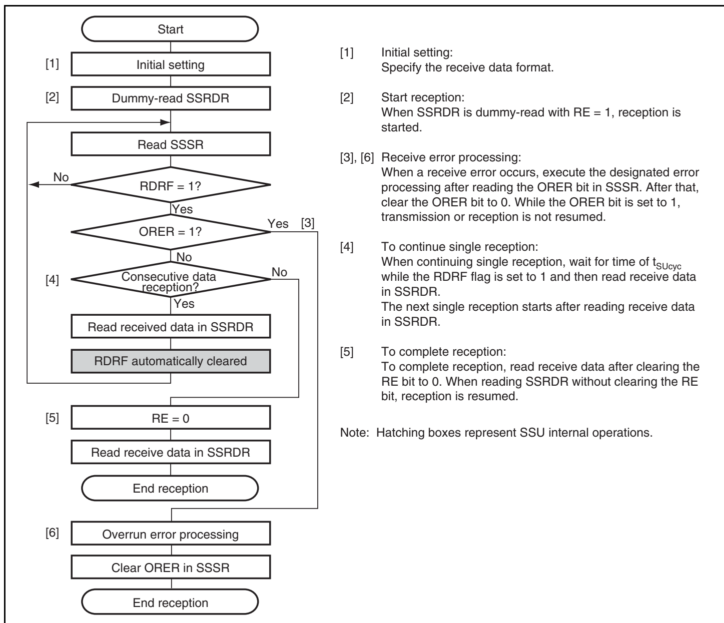
Figure 14.8 Flowchart Example of Data Reception (SSU Mode)
