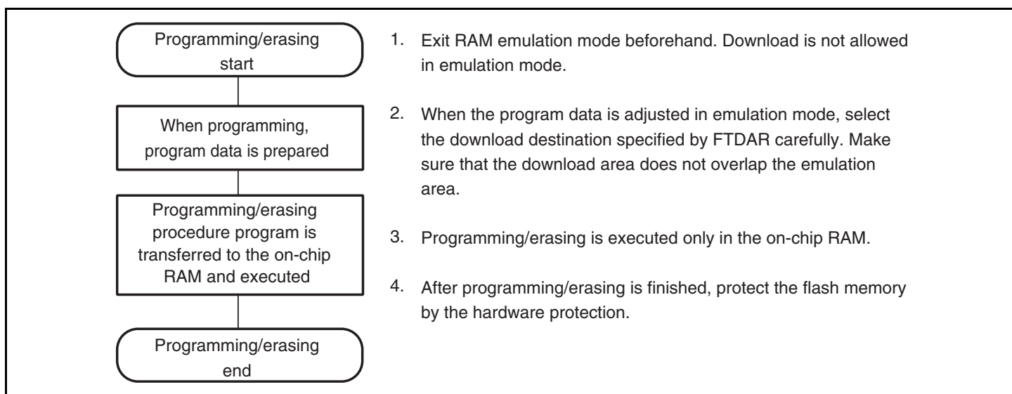
Figure 17.9 Programming/Erasing Flow
