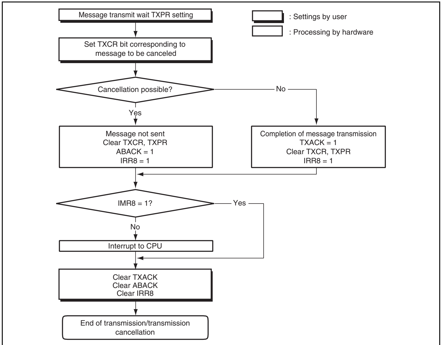
Figure 13.10 Transmit Message Cancellation Flowchart
