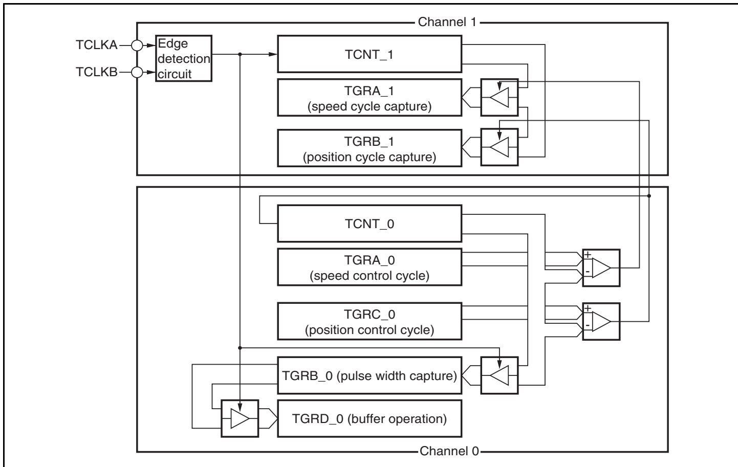
Figure 9.30 Phase Counting Mode Application Example
