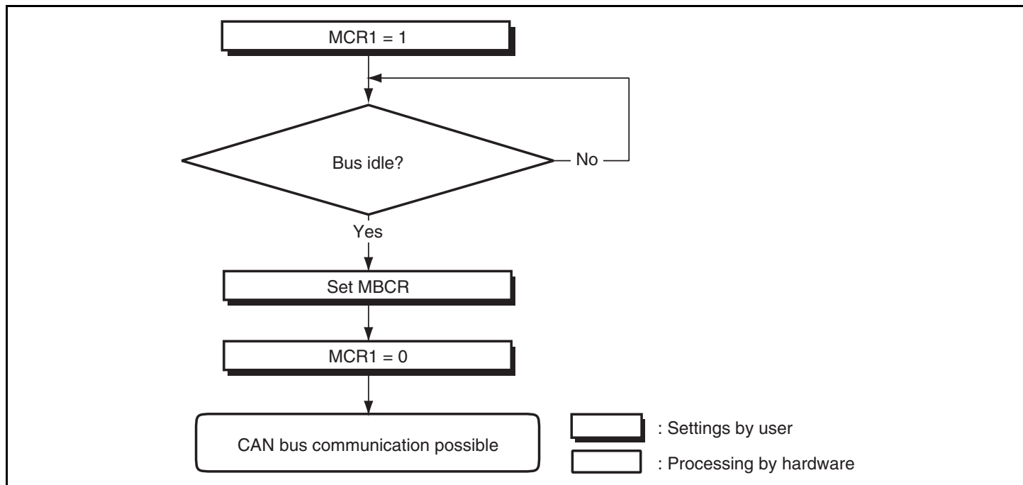
Figure 13.14 HCAN Halt Mode Flowchart
