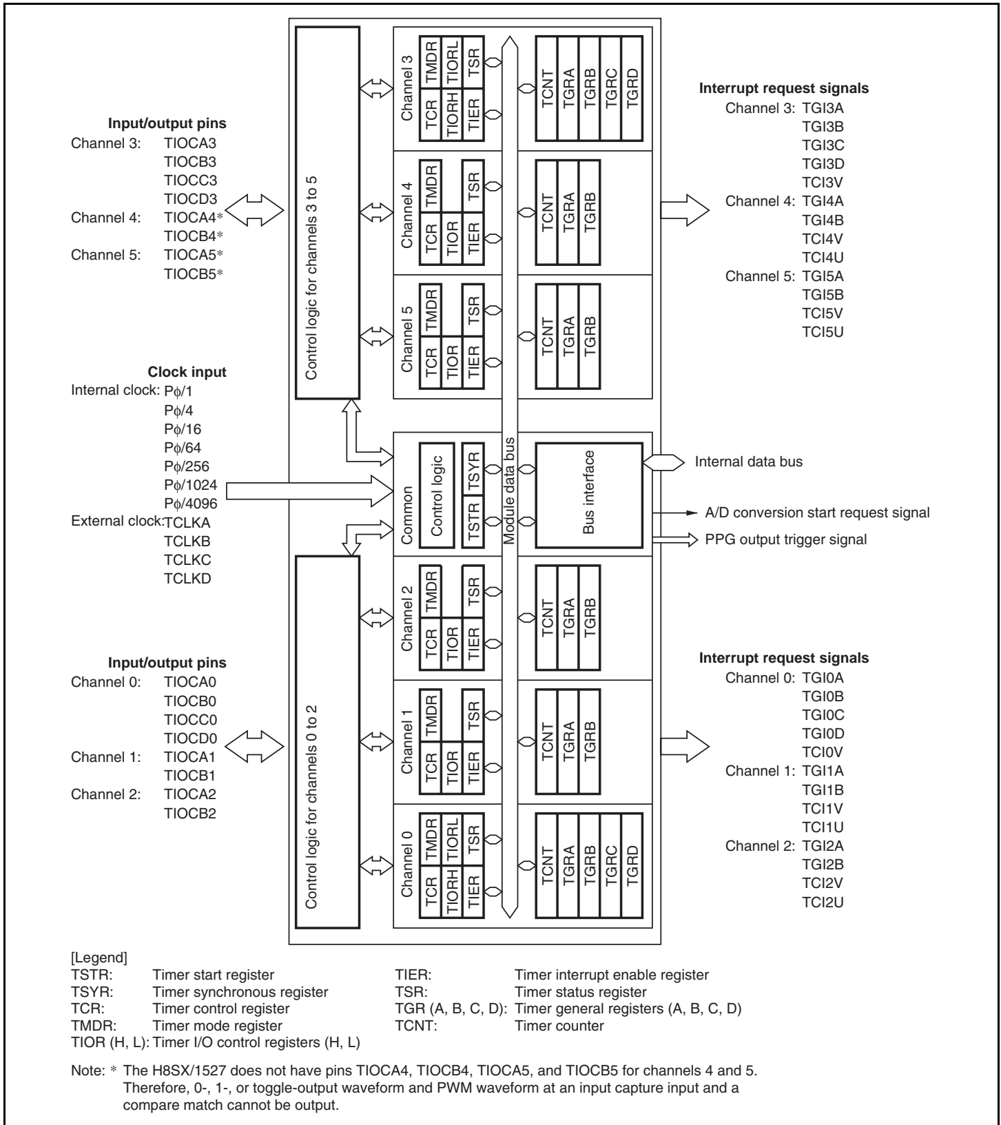
Figure 9.1 Block Diagram of TPU (Unit 0)
