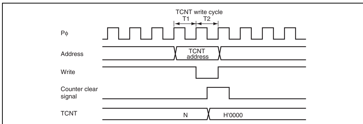
Figure 9.47 Conflict between TCNT Write and Clear Operations
