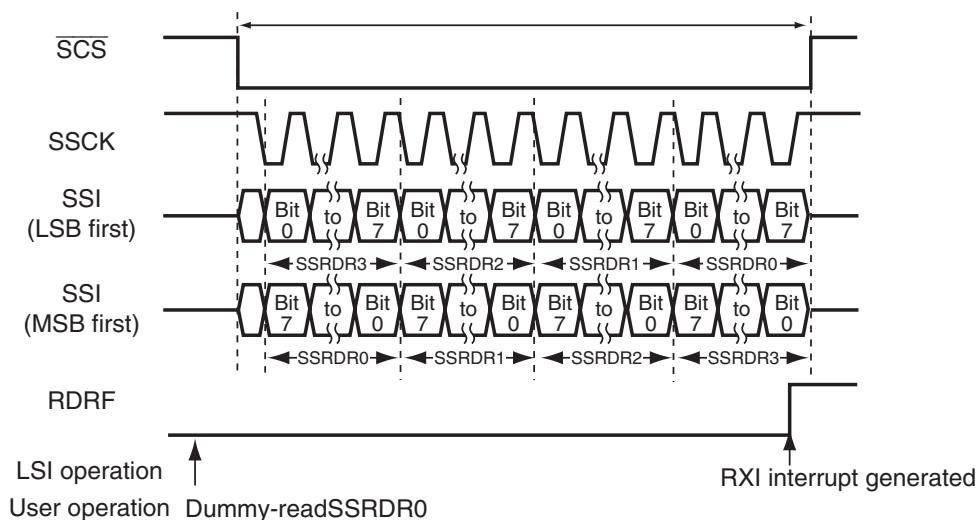
Figure 14.7 Example of Reception Operation (SSU Mode)
