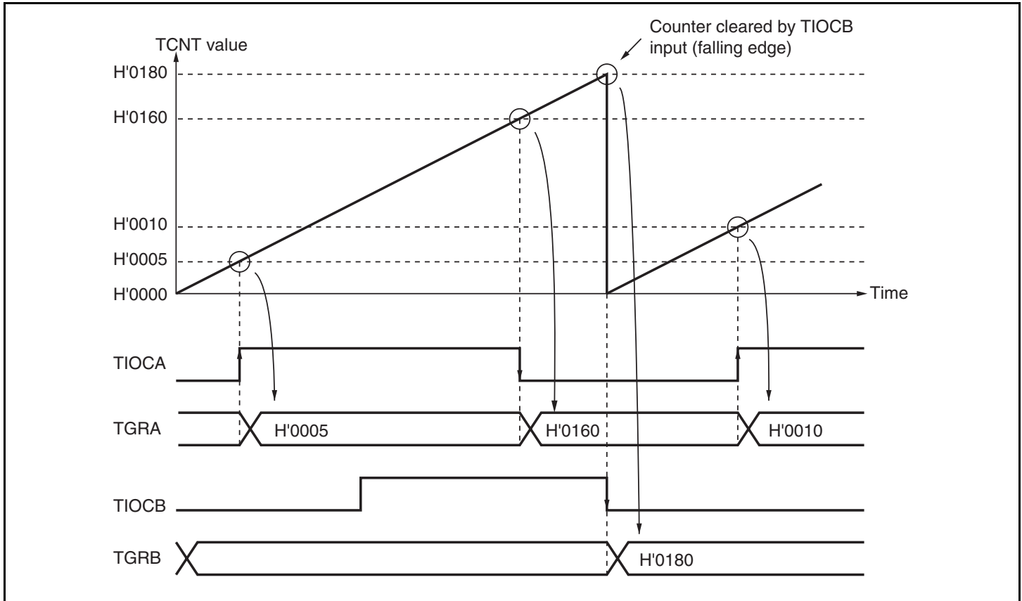
Figure 9.10 Example of Input Capture Operation
