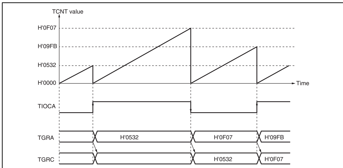
Figure 9.17 Example of Buffer Operation (2)
