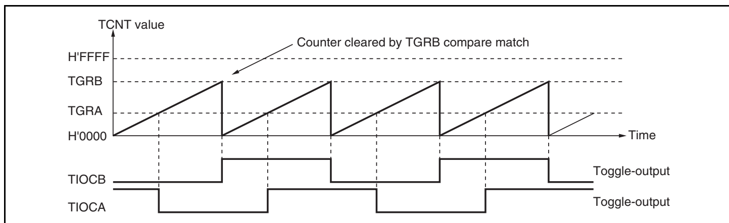
Figure 9.8 Example of Toggle Output Operation
