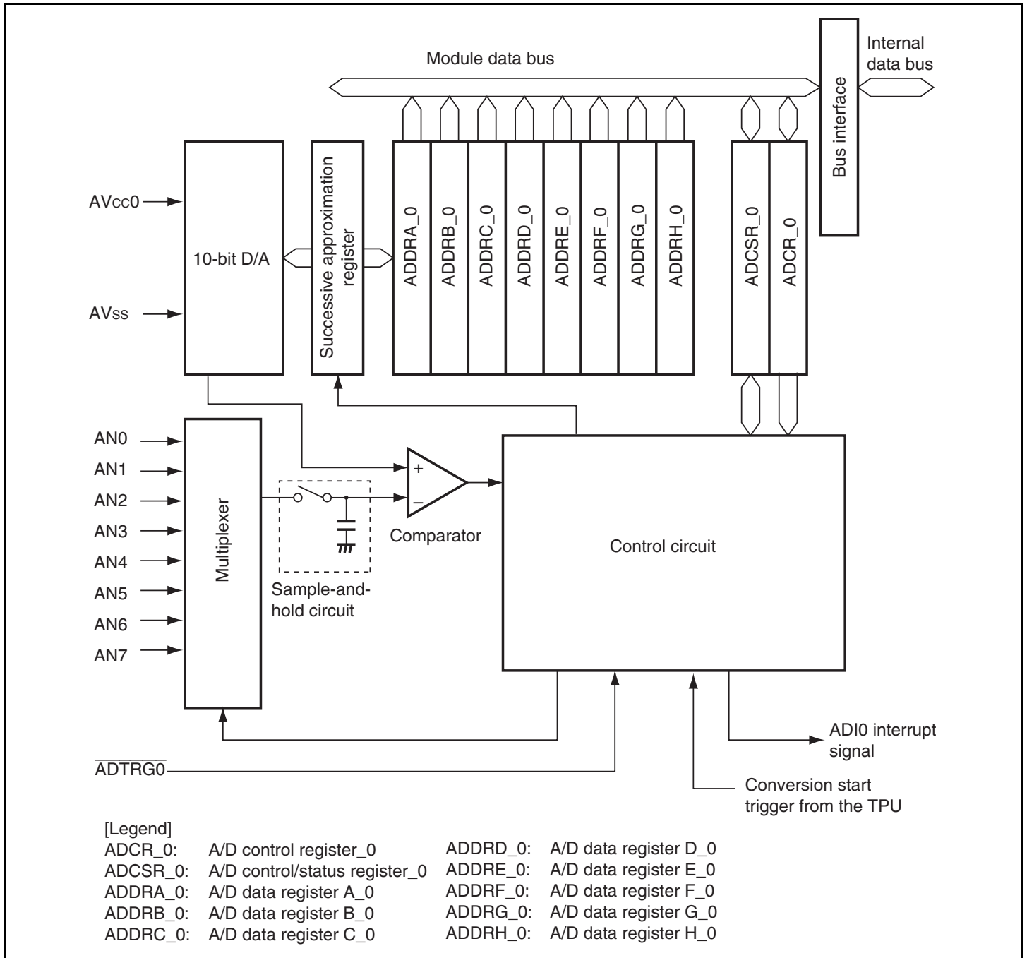
Figure 15.1 Block Diagram of A/D Converter (Unit 0/AD_0)
