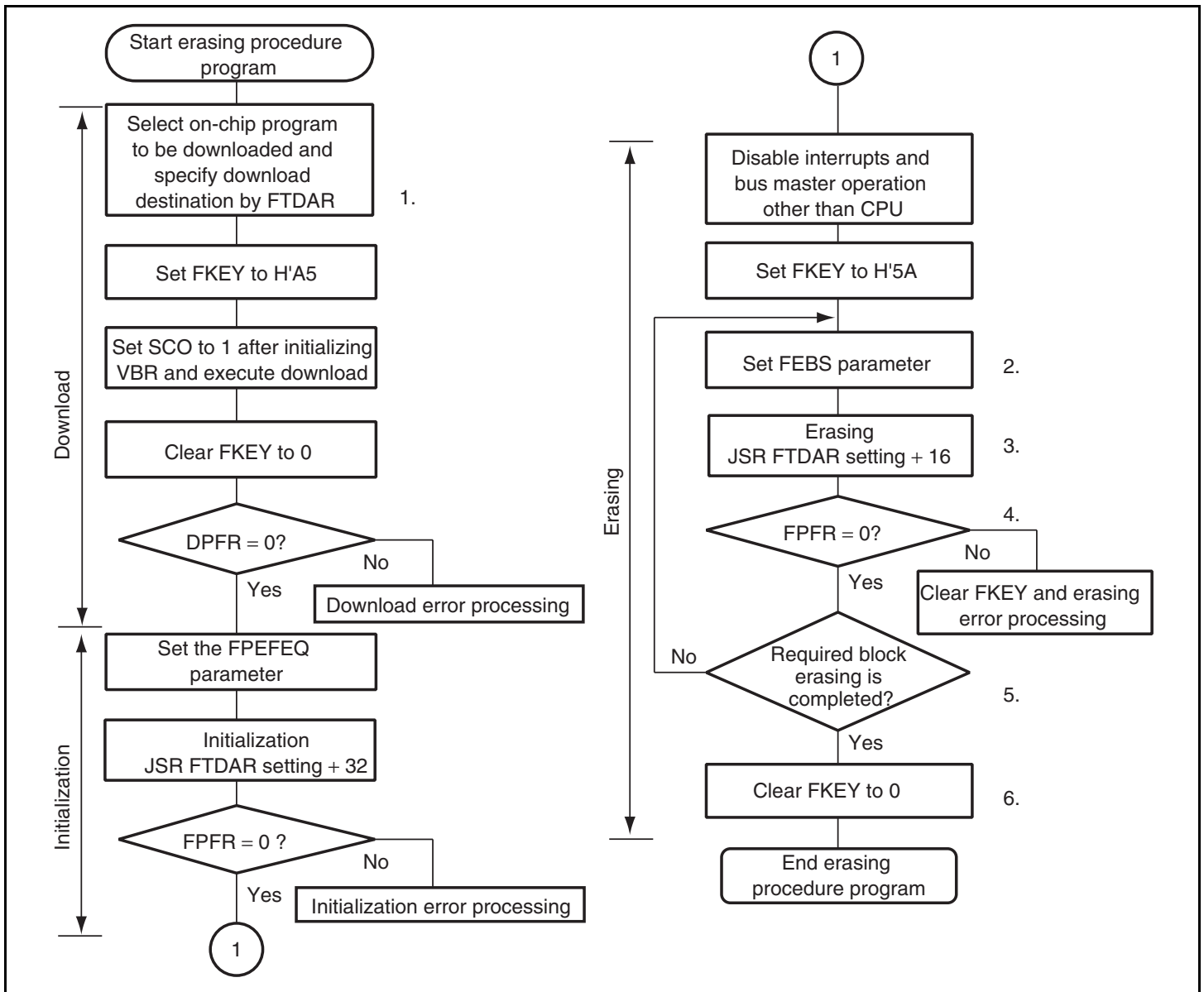
Figure 17.12 Erasing Procedure in User Program Mode
