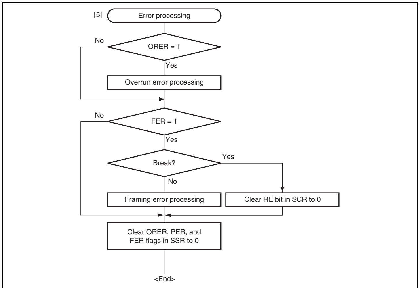
Figure 12.13 Sample Multiprocessor Serial Reception Flowchart (2)
