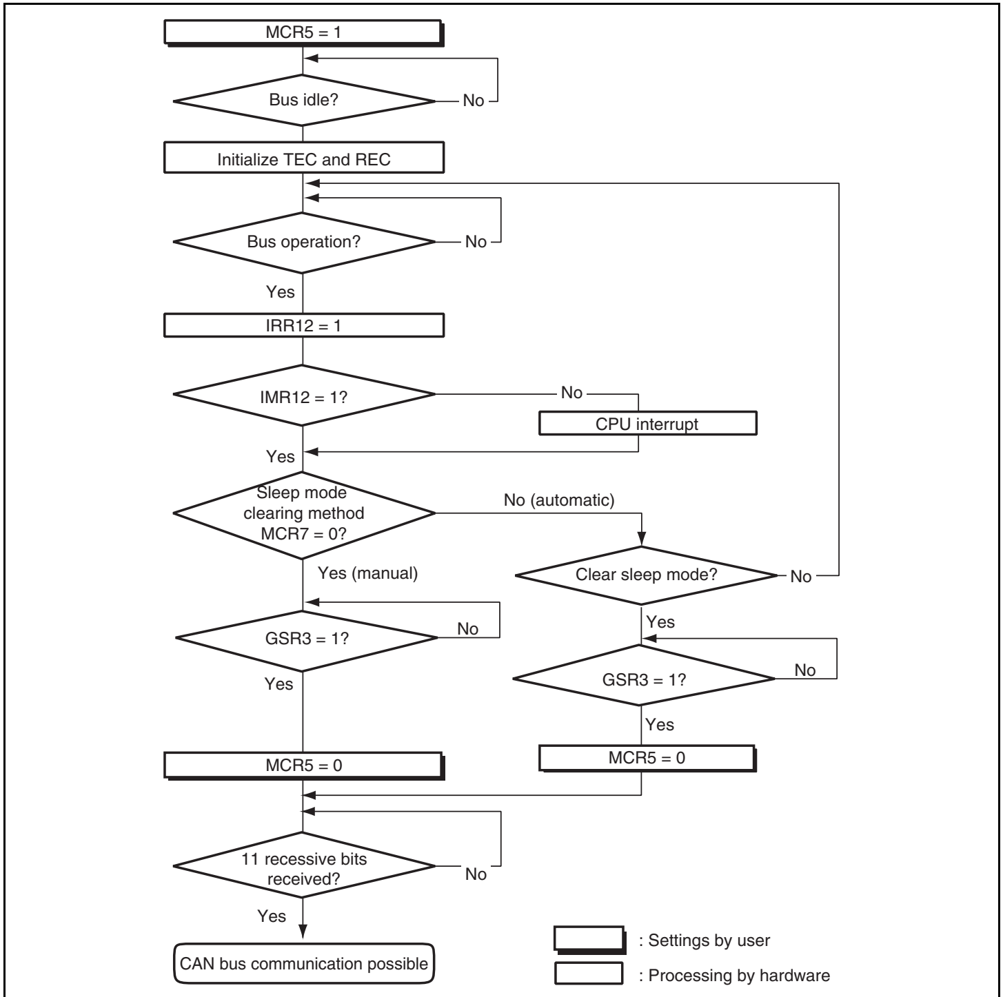
Figure 13.13 HCAN Sleep Mode Flowchart
