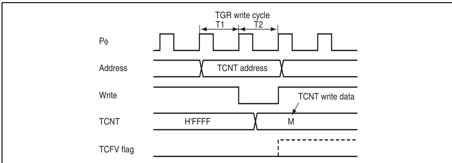
Figure 9.55 Conflict between TCNT Write and Overflow
