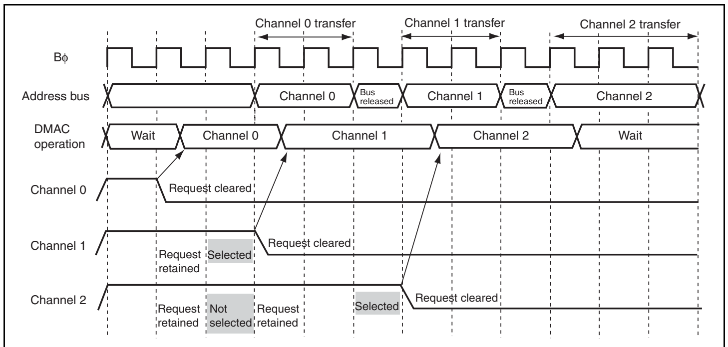
Figure 7.22 Example of Timing for Channel Priority
