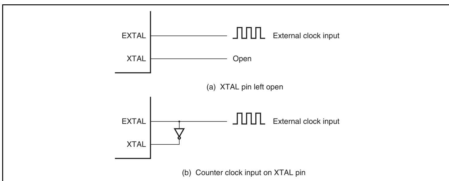
Figure 18.4 External Clock Input (Examples)
