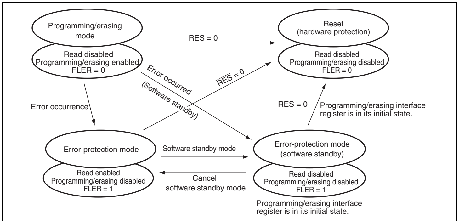
Figure 17.16 Transitions to Error Protection State
