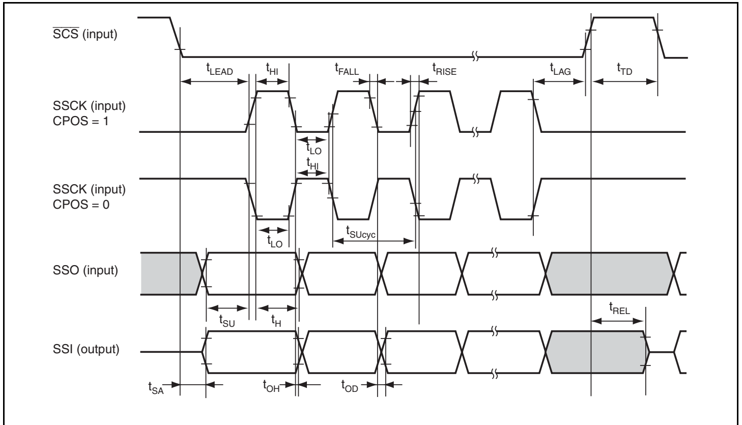
Figure 21.19 SSU Timing (Slave, CPHS = 1)
