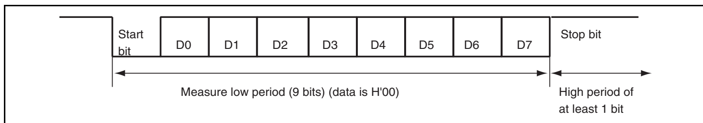
Figure 17.7 Automatic-Bit-Rate Adjustment Operation
