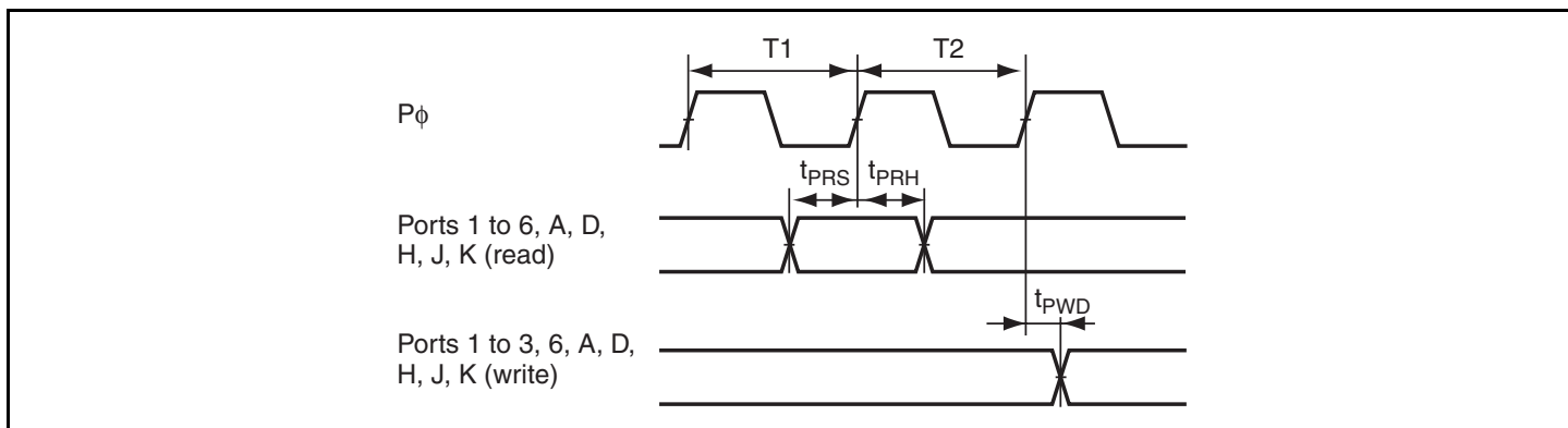
Figure 21.8 I/O Port Input/Output Timing
