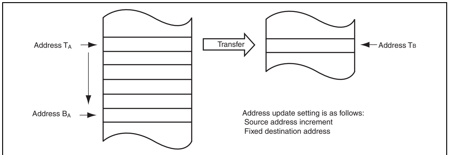
Figure 7.3 Operations in Dual Address Mode
