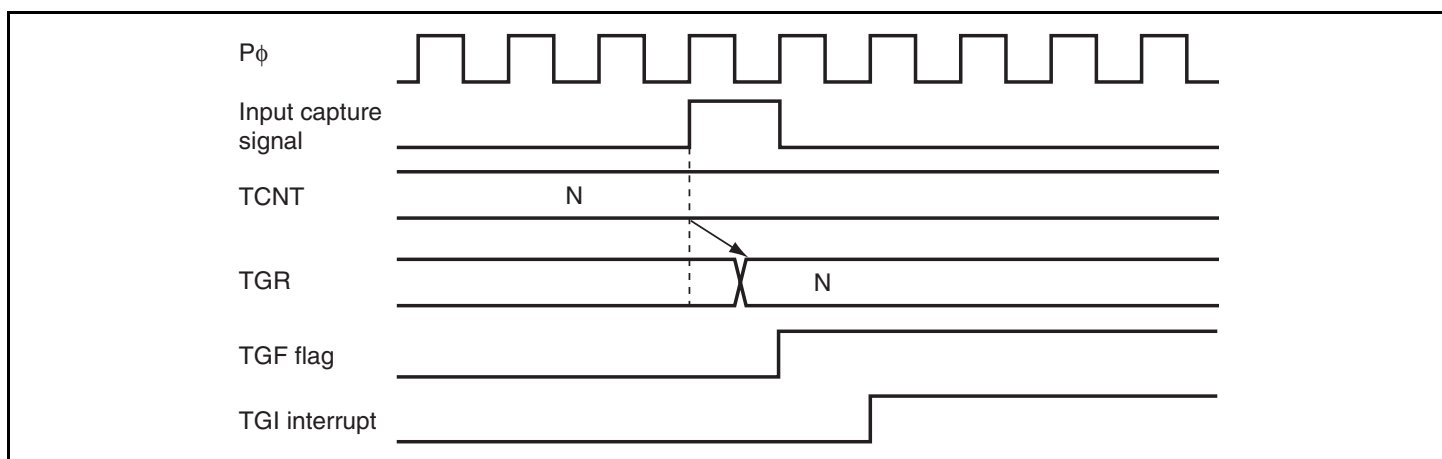
Figure 9.40 TGI Interrupt Timing (Input Capture)
