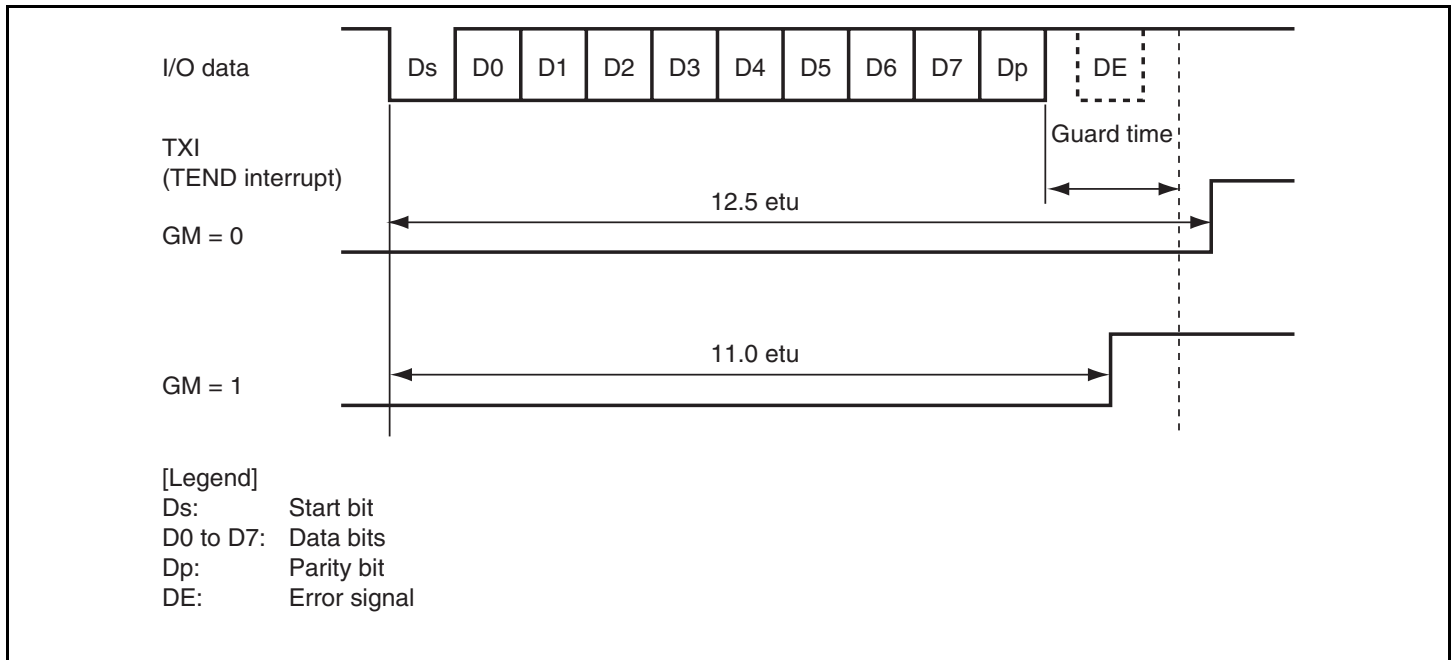
Figure 12.27 TEND Flag Set Timing during Transmission
