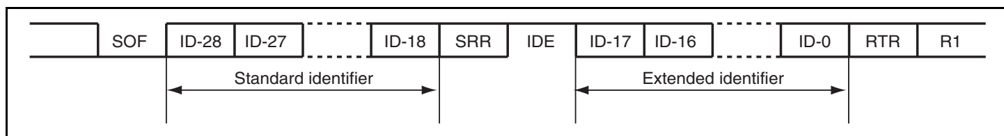
Figure 13.4 Extended Format
