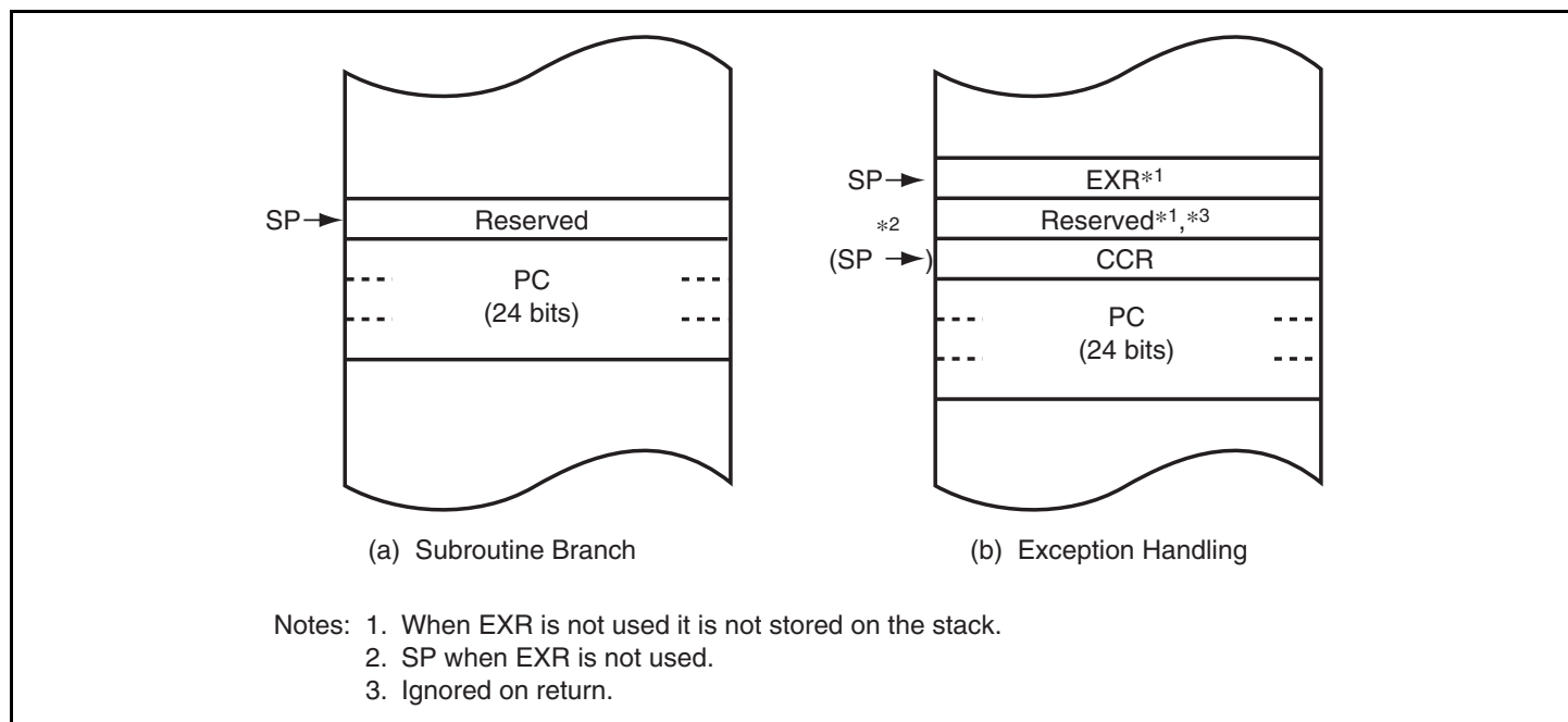
Figure 2.5 Stack Structure (Middle and Advanced Modes)
