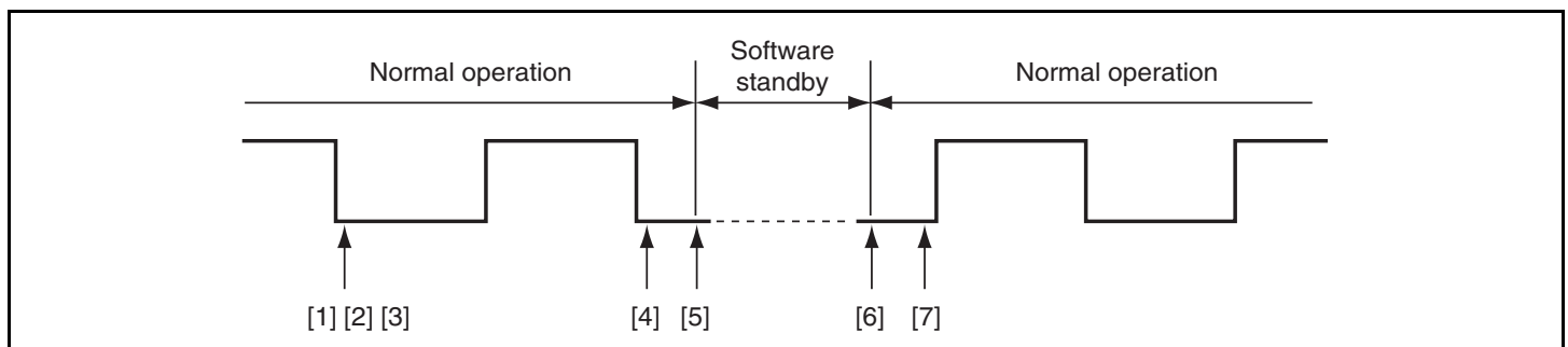
Figure 12.32 Clock Stop and Restart Procedure
