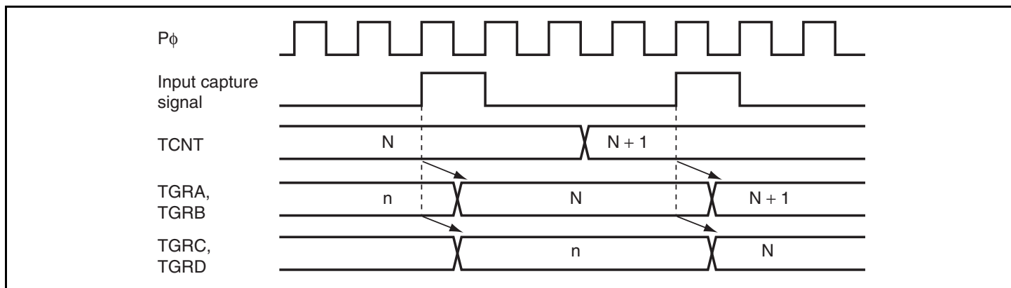
Figure 9.38 Buffer Operation Timing (Input Capture)
