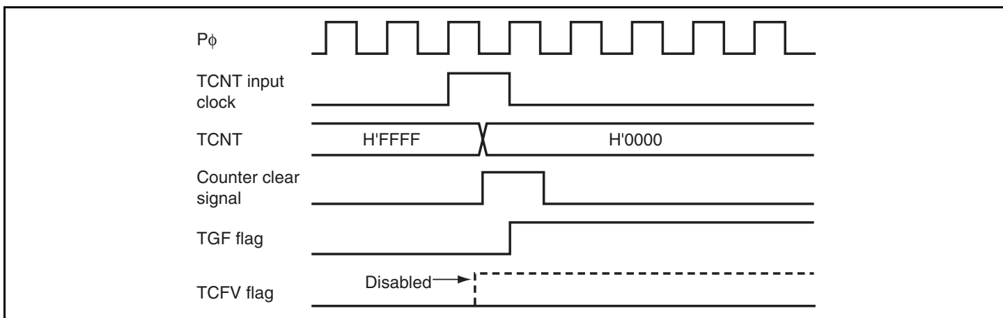
Figure 9.54 Conflict between Overflow and Counter Clearing
