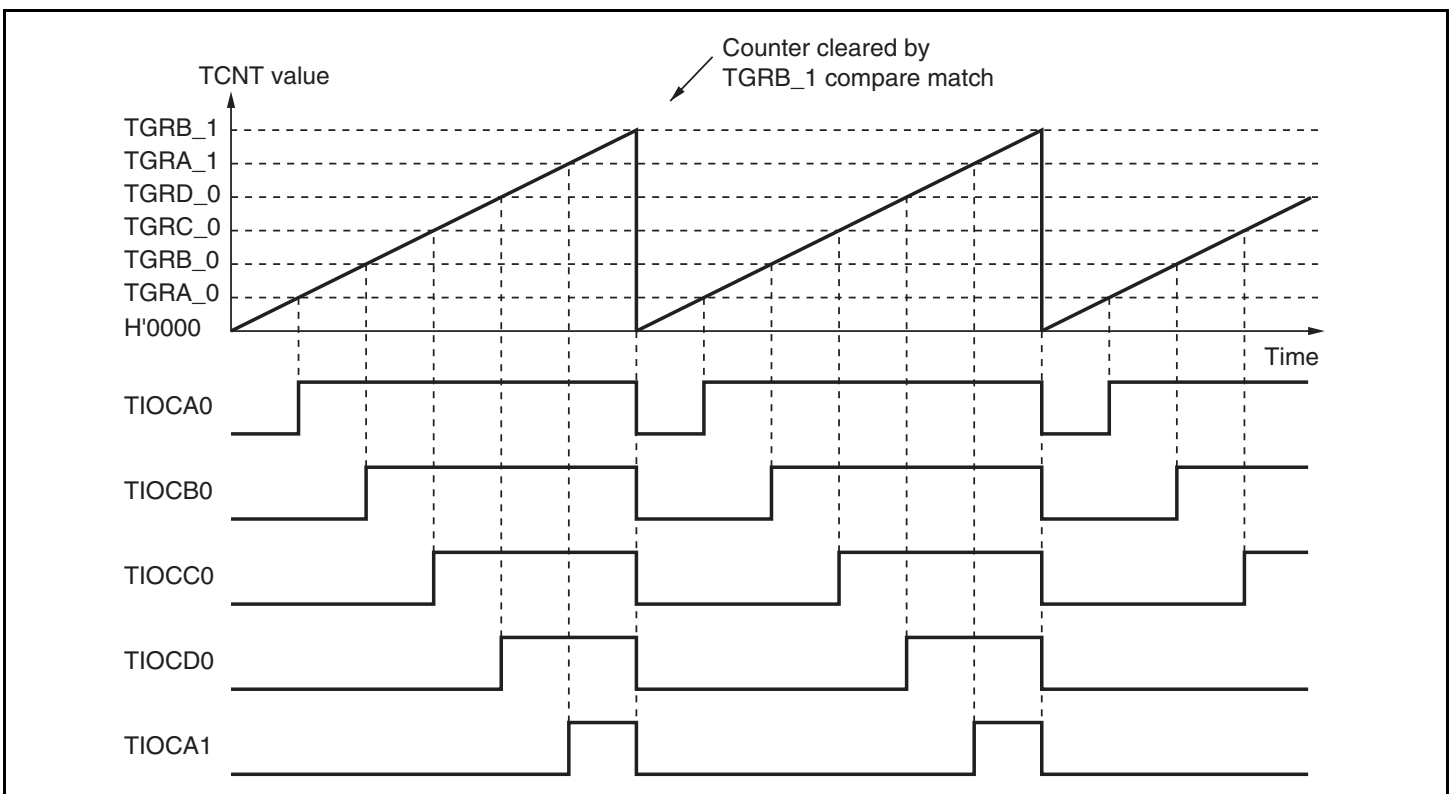
Figure 9.23 Example of PWM Mode Operation (2)
