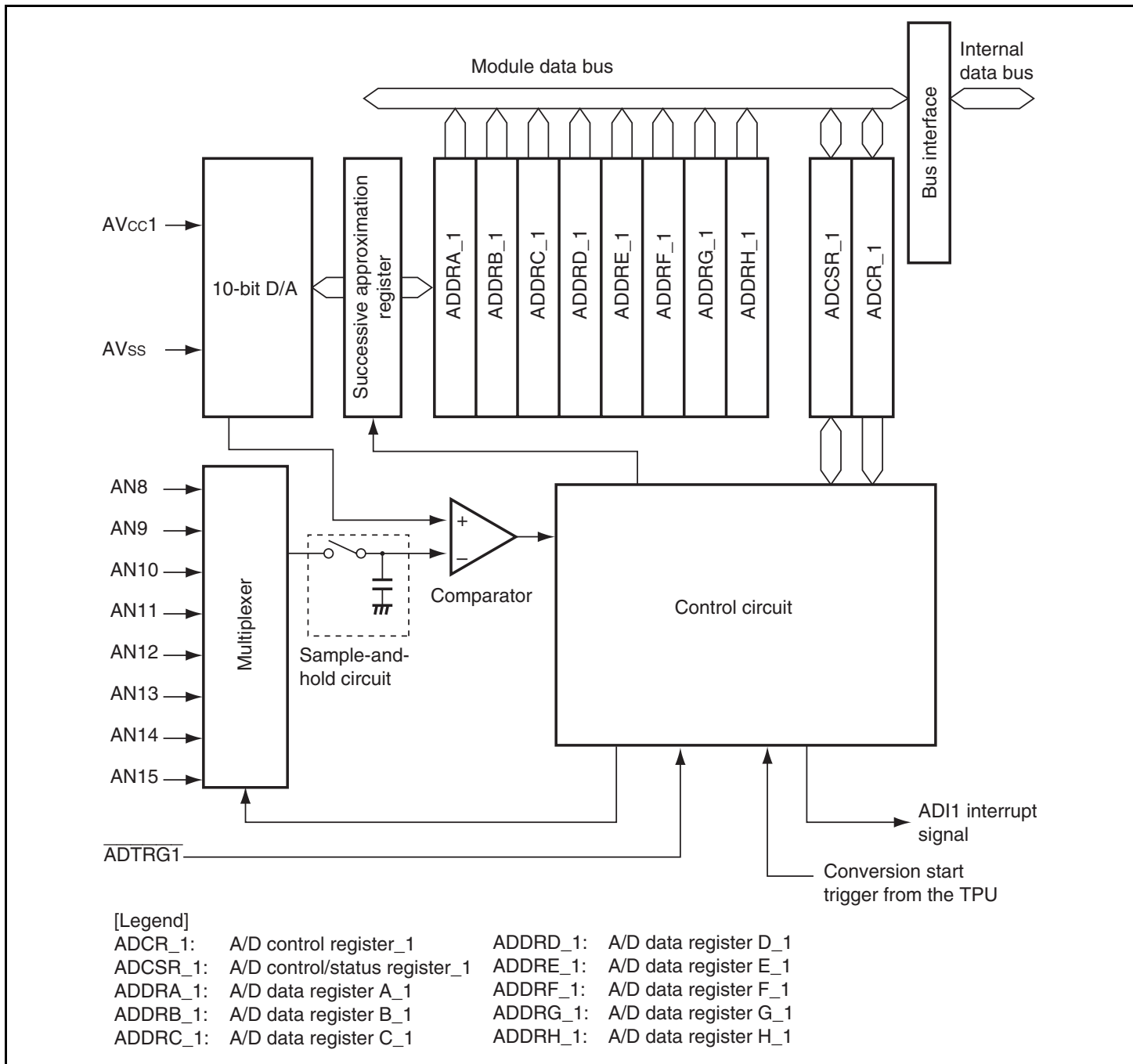
Figure 15.2 Block Diagram of A/D Converter (Unit 1/AD_1)
