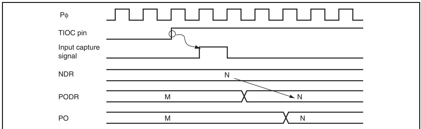
Figure 10.11 Pulse Output Triggered by Input Capture (Example)
