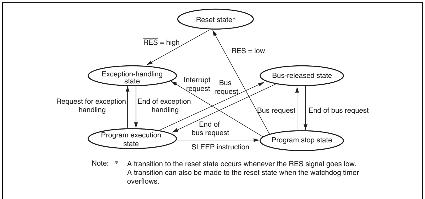
Figure 2.16 State Transitions
