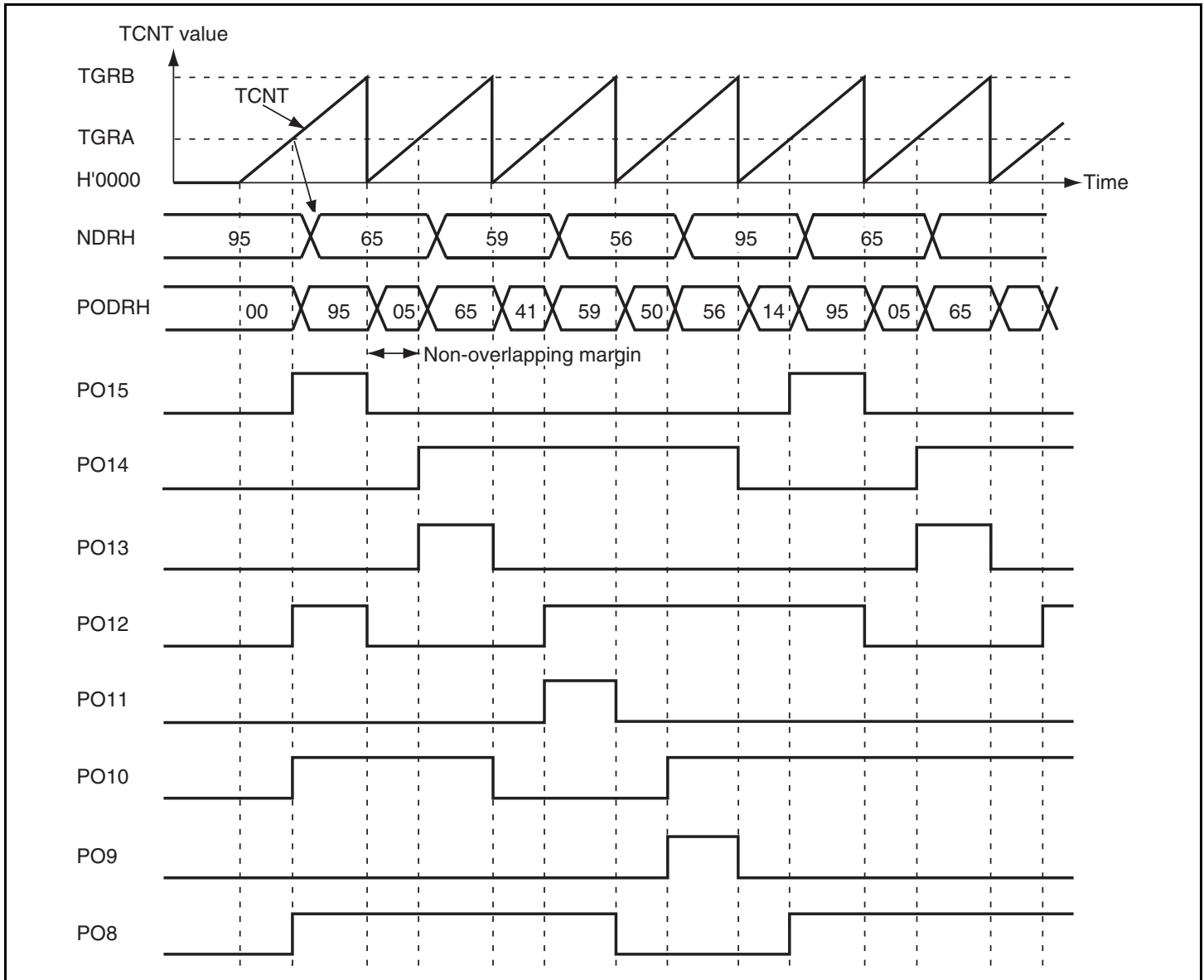
Figure 10.9 Non-Overlapping Pulse Output Example (4-Phase Complementary)
