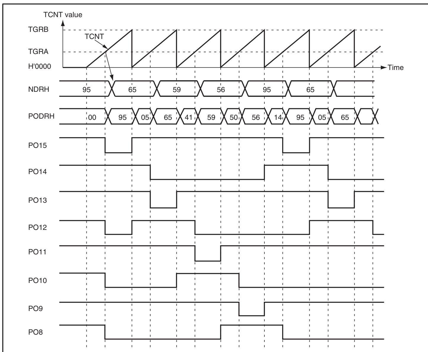
Figure 10.10 Inverted Pulse Output (Example)
