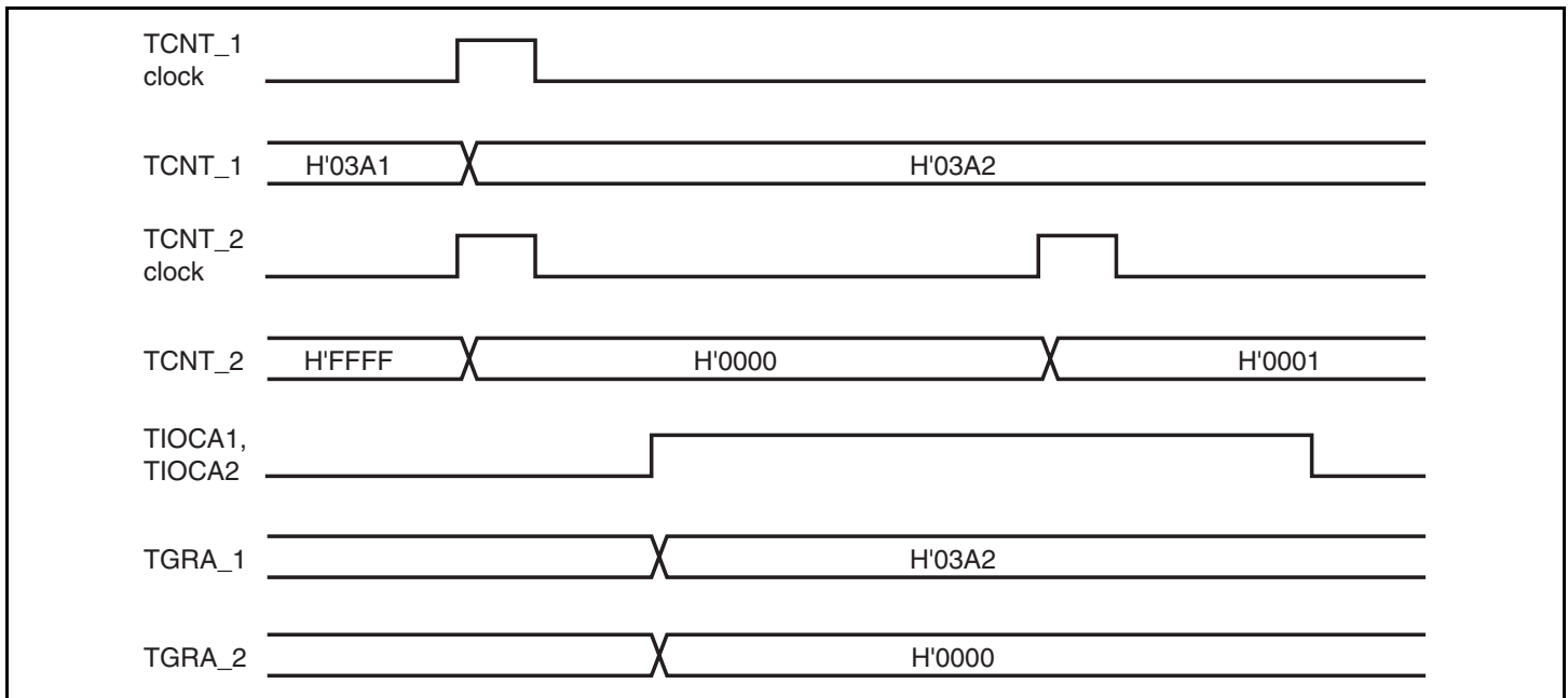
Figure 9.19 Example of Cascaded Operation (1)
