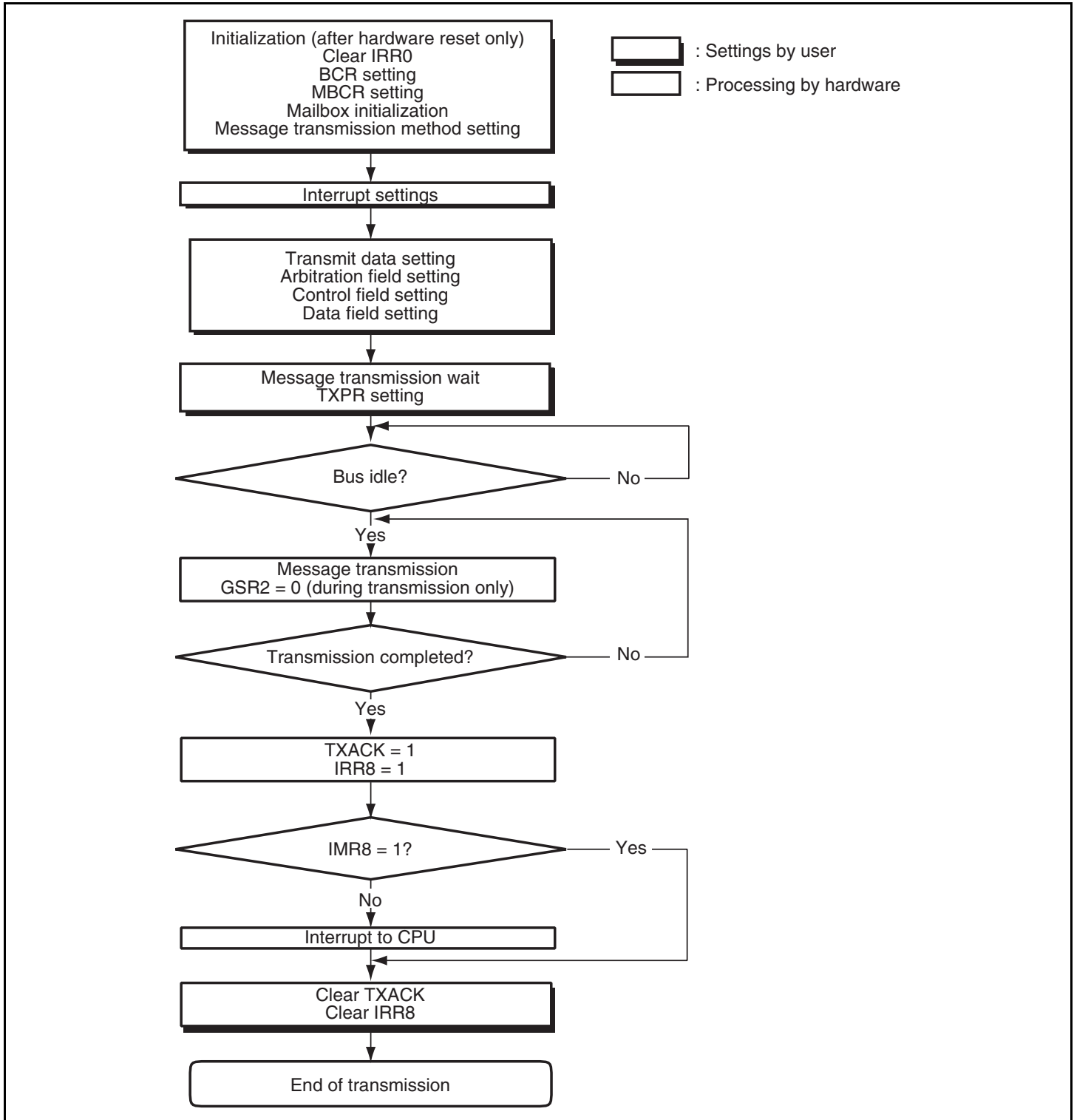
Figure 13.9 Transmission Flowchart
