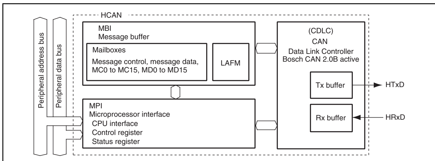
Figure 13.1 HCAN Block Diagram
