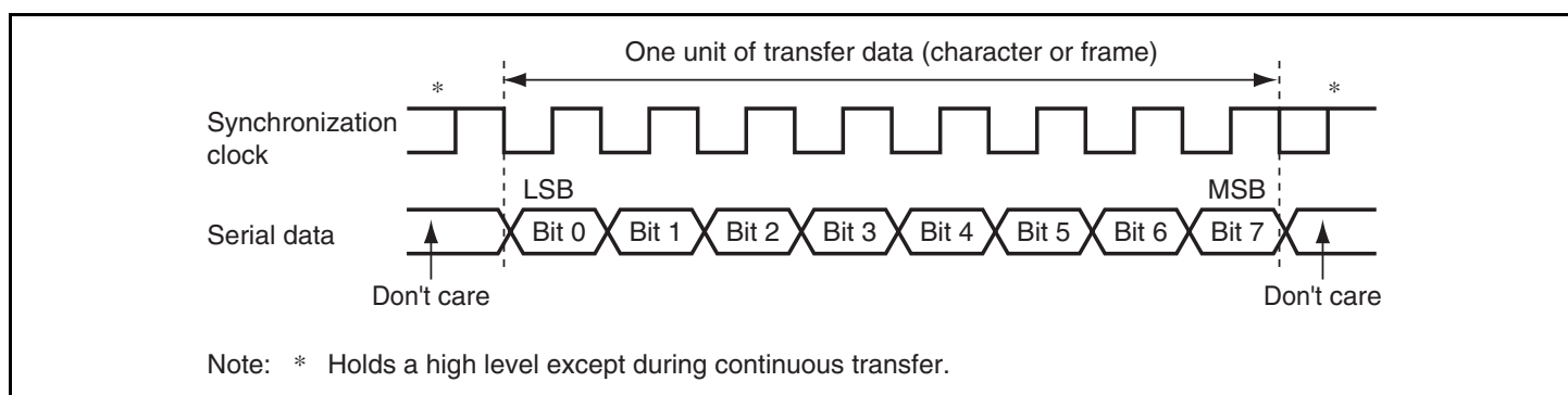
Figure 12.14 Data Format in Clocked Synchronous Communication (LSB-First)
