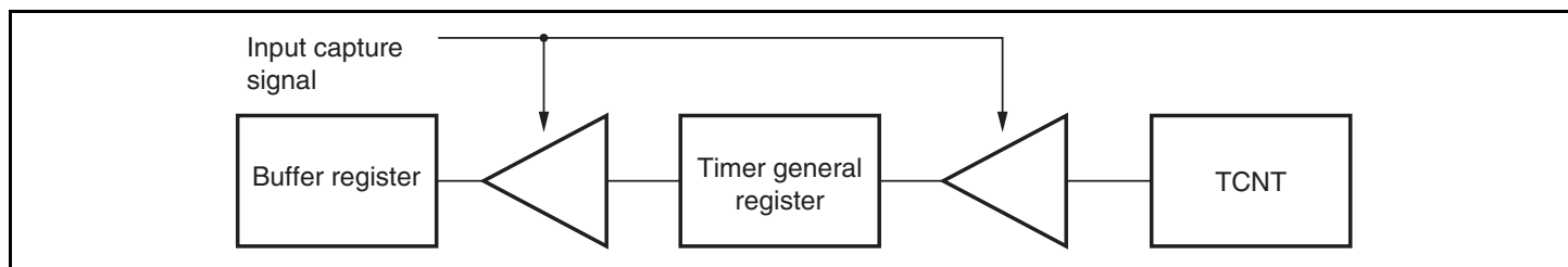
Figure 9.14 Input Capture Buffer Operation
