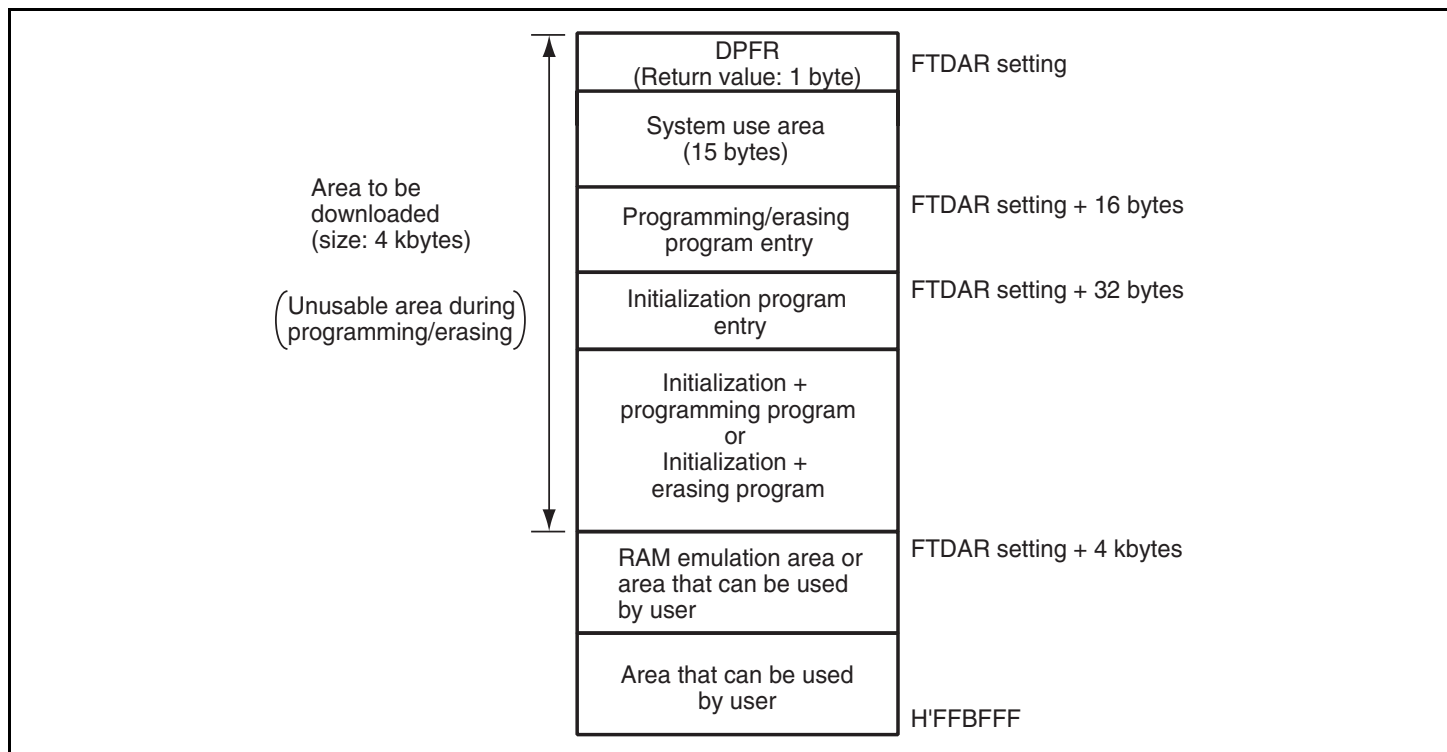
Figure 17.10 RAM Map when Programming/Erasing is Executed
