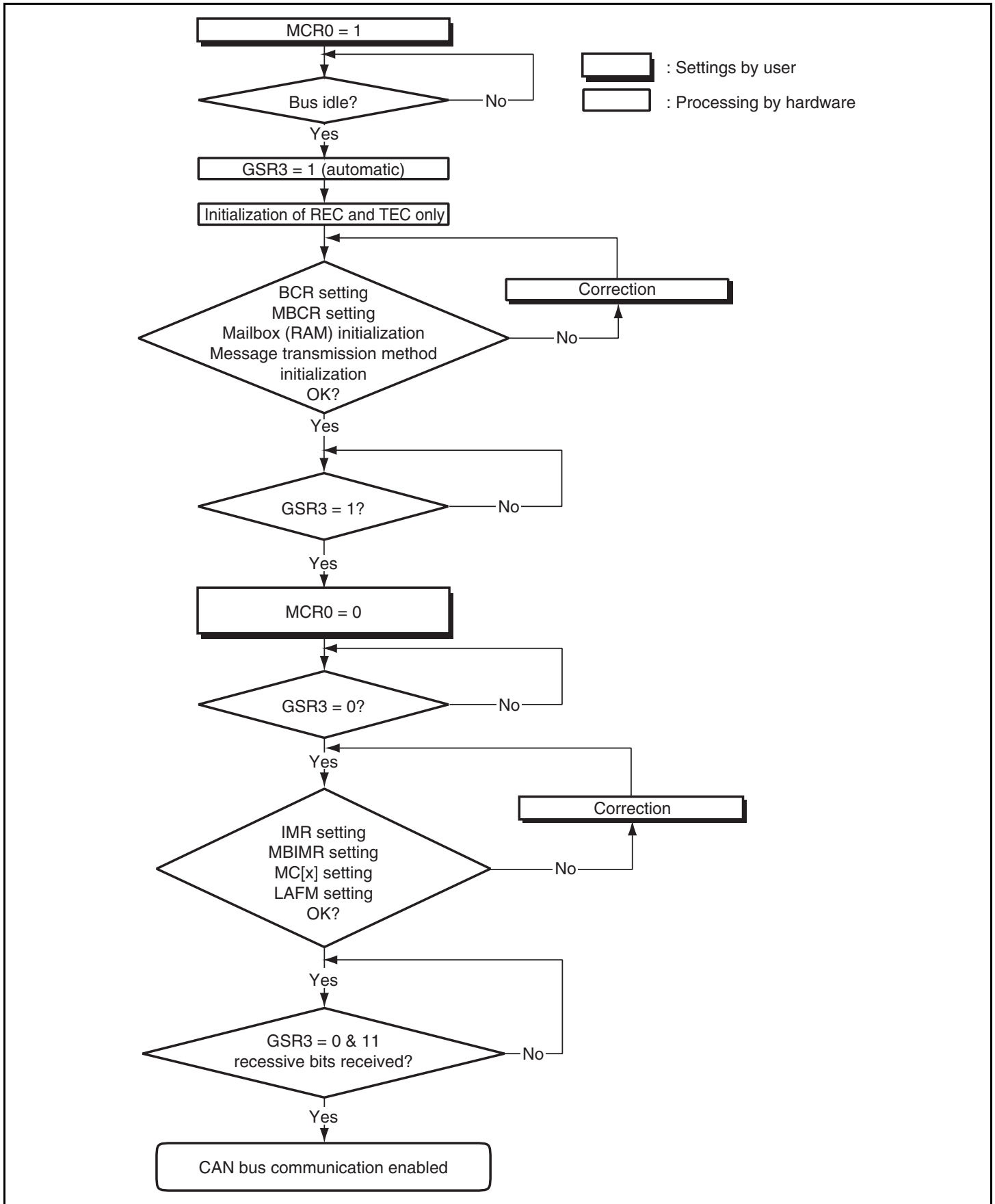
Figure 13.7 Software Reset Flowchart
