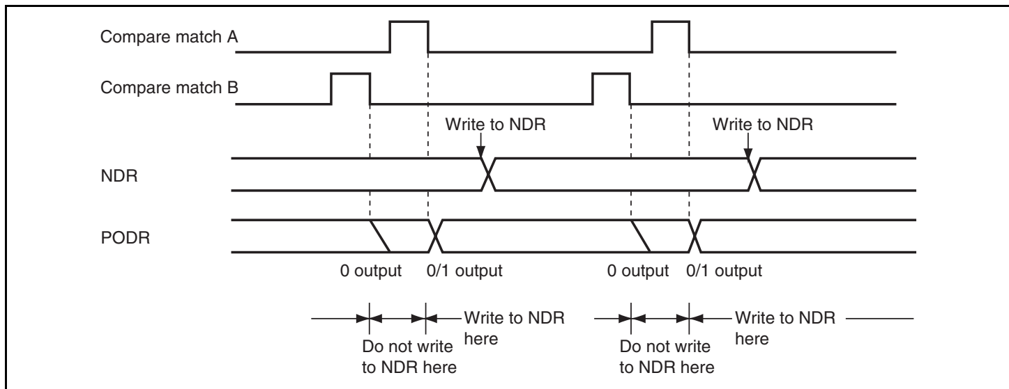
Figure 10.7 Non-Overlapping Operation and NDR Write Timing
