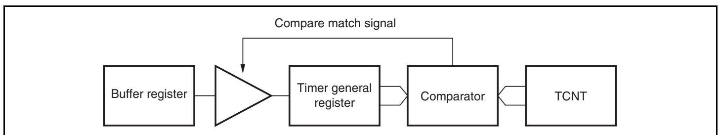
Figure 9.13 Compare Match Buffer Operation
