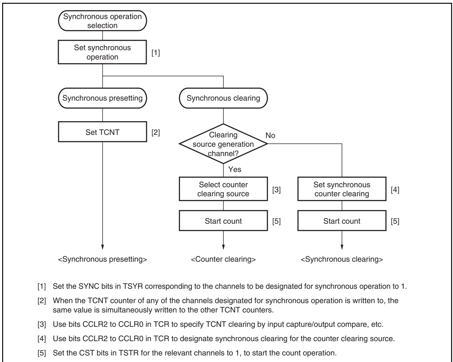
Figure 9.11 Example of Synchronous Operation Setting Procedure
