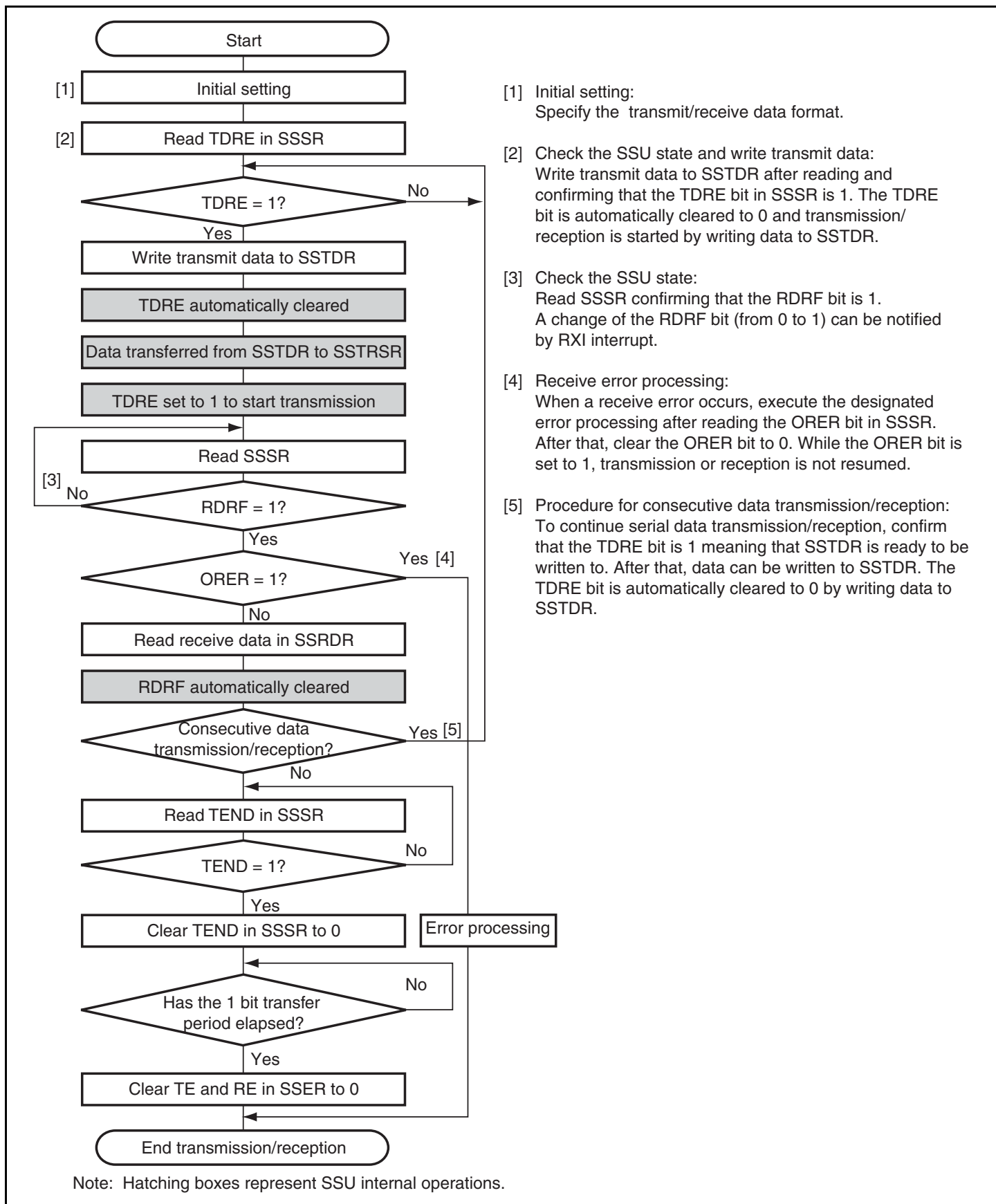
Figure 14.9 Flowchart Example of Simultaneous Transmission/Reception (SSU Mode)
