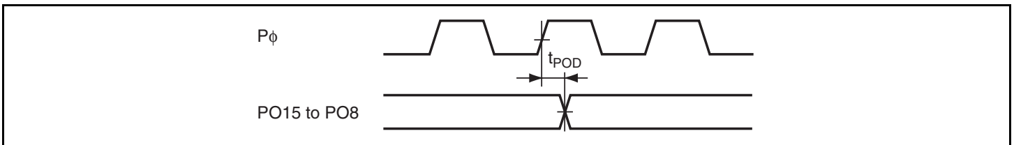
Figure 21.12 PPG Output Timing
