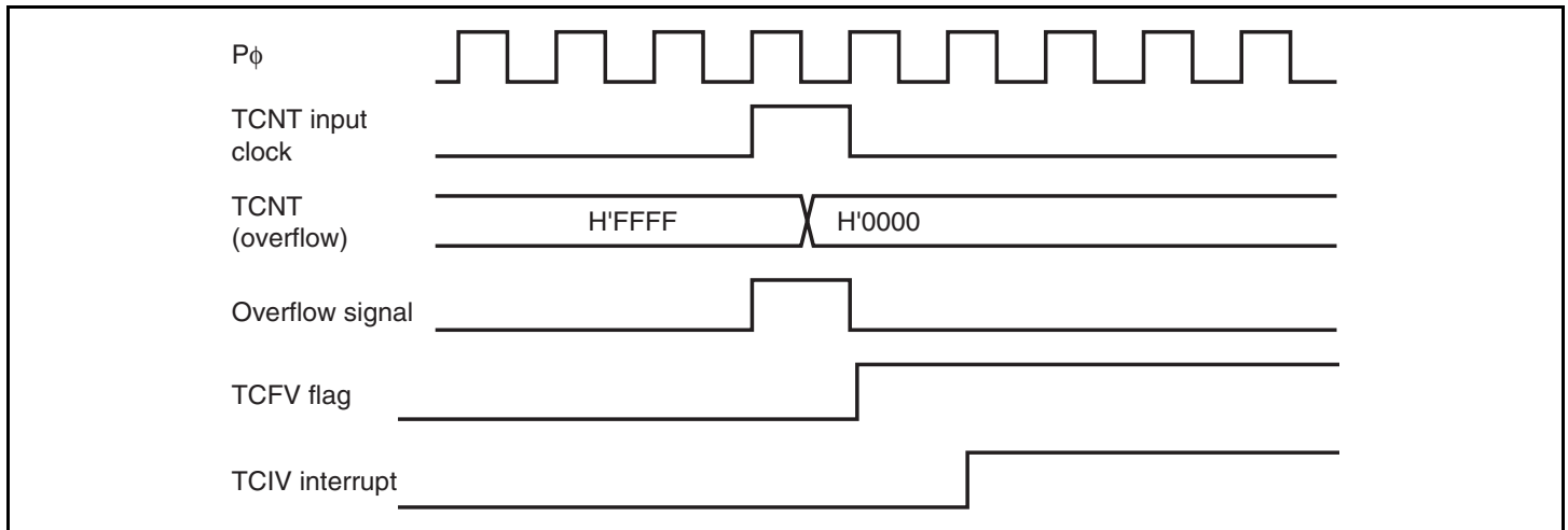
Figure 9.41 TCIV Interrupt Setting Timing
