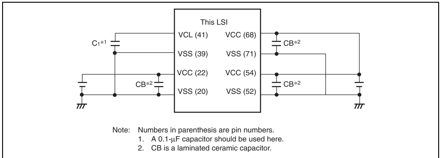
Figure 18.7 Connection Example of Bypass Capacitor
