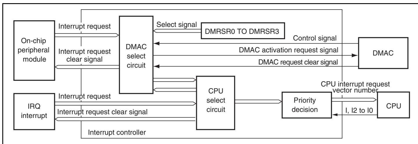
Figure 5.6 Block Diagram of DMAC and Interrupt Controller
