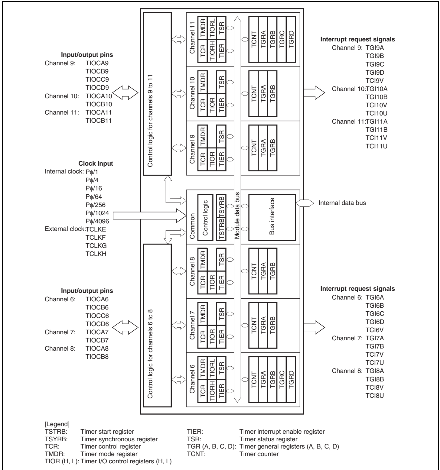
Figure 9.2 Block Diagram of TPU (Unit 1)
