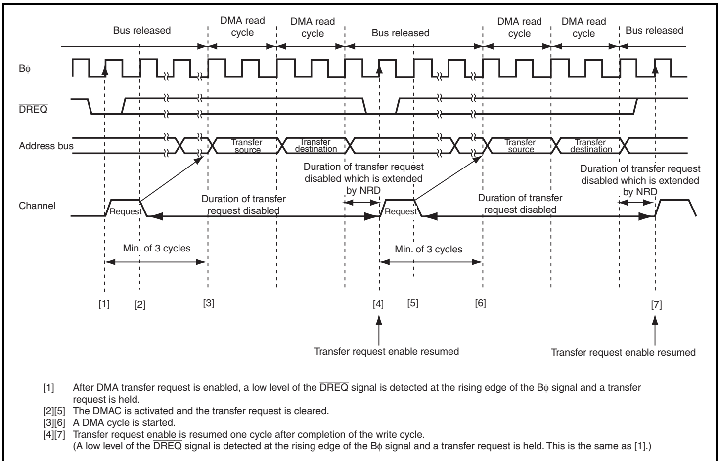
Figure 7.32 Example of Transfer in Normal Transfer Mode Activated by \overline{DREQ} Low Level with NRD = 1
