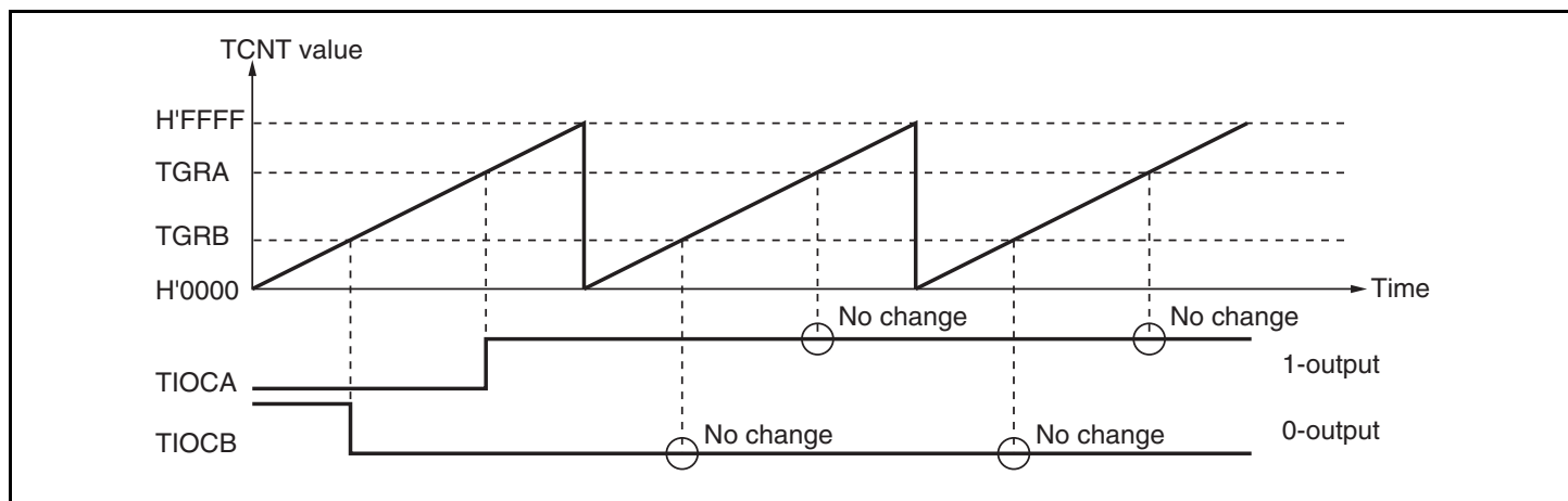
Figure 9.7 Example of 0-Output/1-Output Operation
