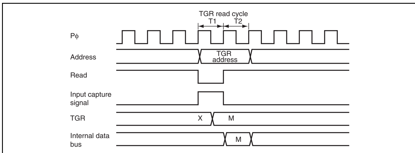
Figure 9.51 Conflict between TGR Read and Input Capture
