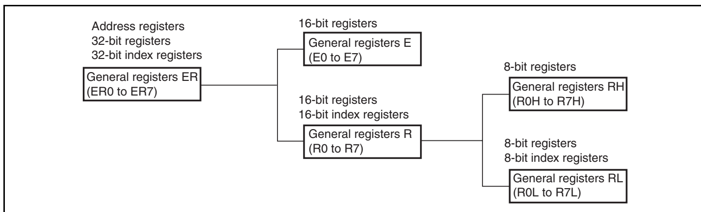
Figure 2.10 Usage of General Registers
