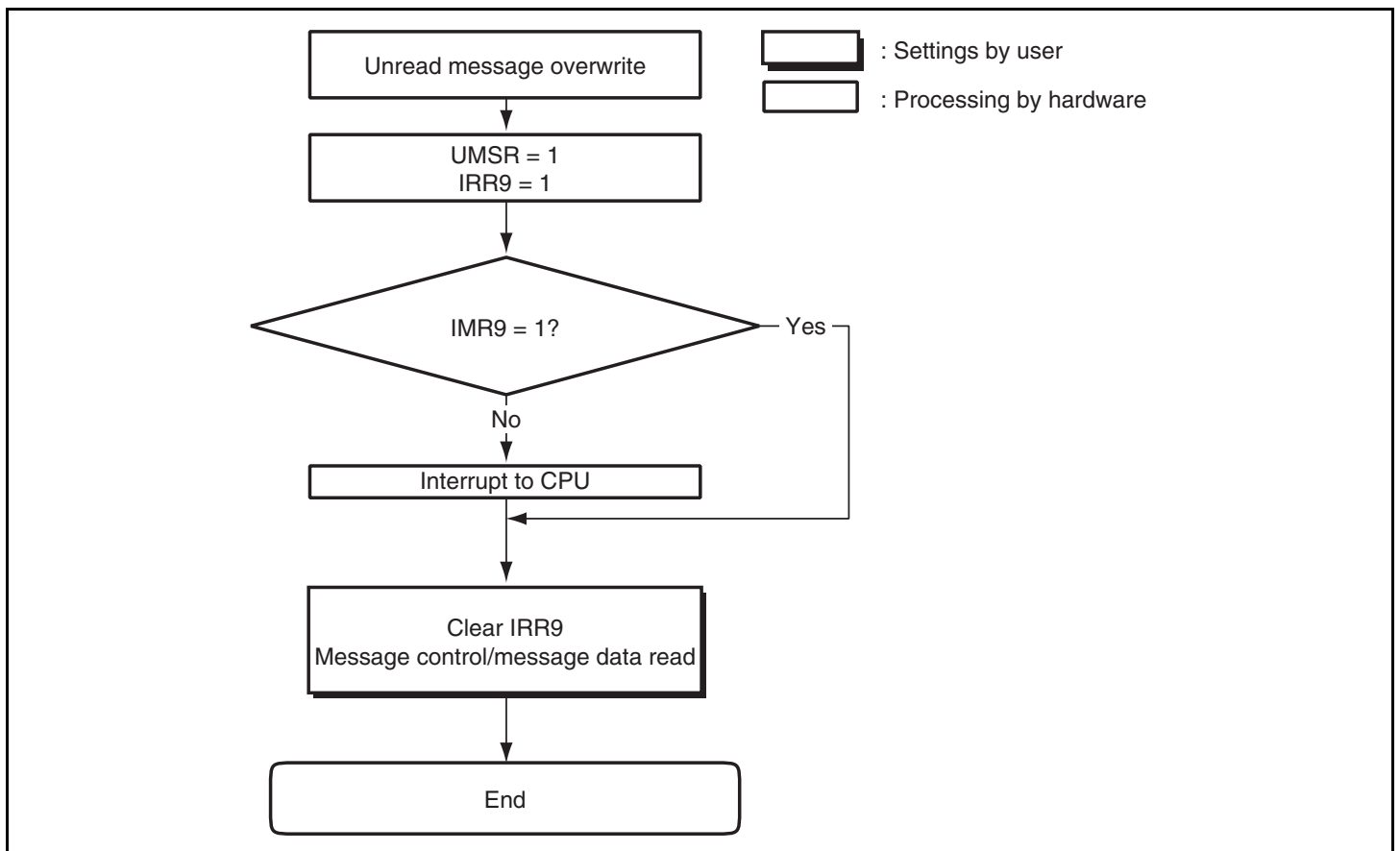
Figure 13.12 Unread Message Overwrite Flowchart
