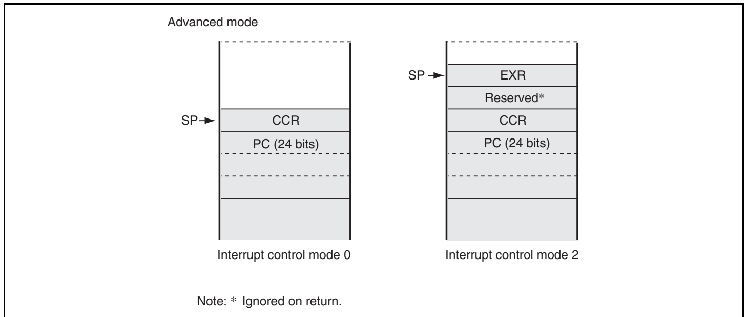
Figure 4.2 Stack Status after Exception Handling
