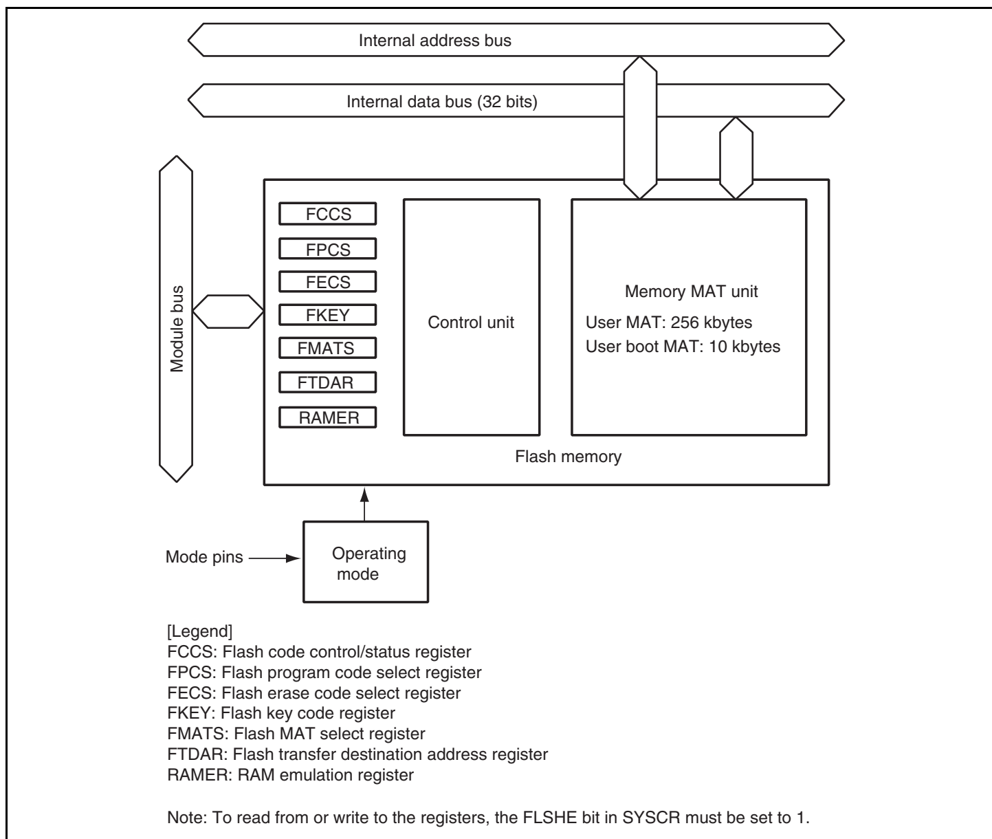
Figure 17.1 Block Diagram of Flash Memory
