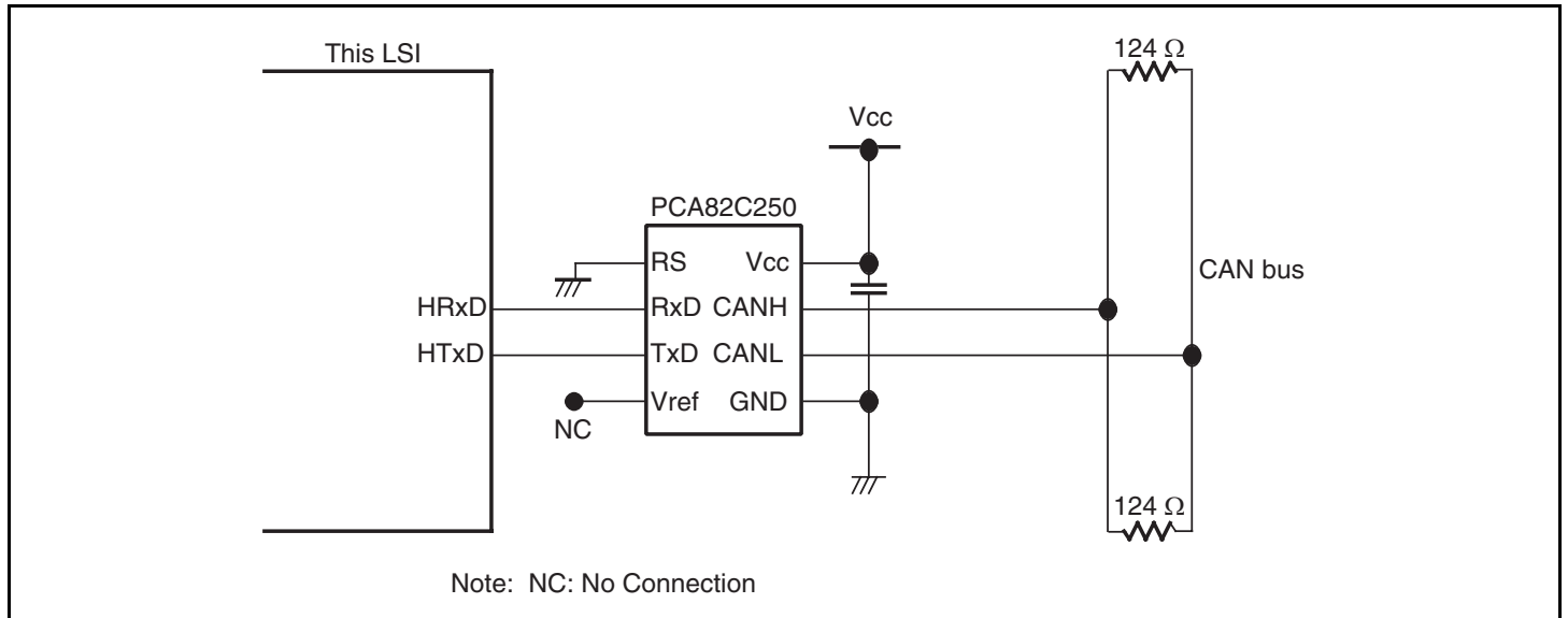
Figure 13.16 High-Speed Interface Using PCA82C250
