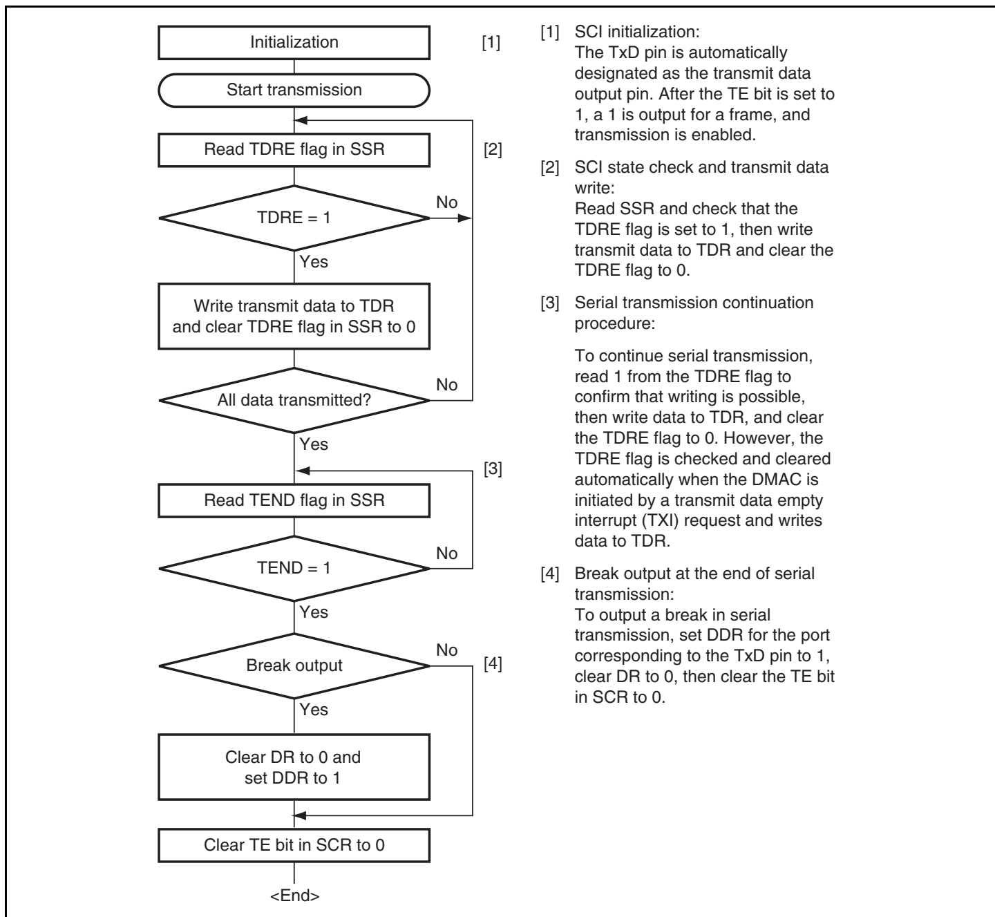
Figure 12.7 Sample Serial Transmission Flowchart
