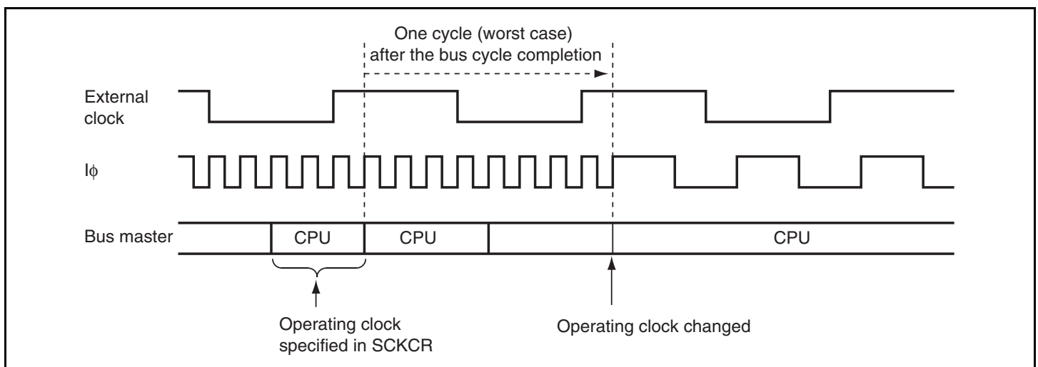
Figure 18.5 Clock Modification Timing
