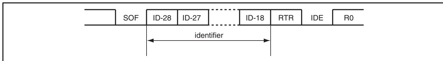
Figure 13.3 Standard Format
