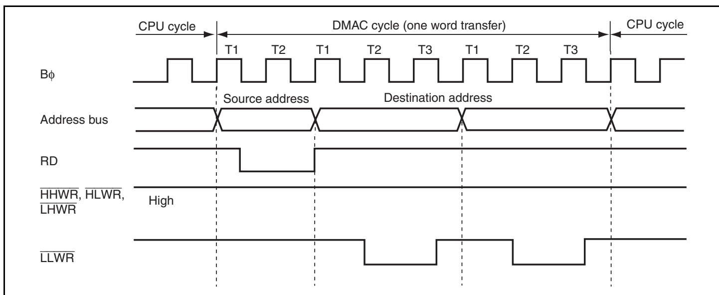
Figure 7.23 Example of Bus Timing of DMA Transfer
