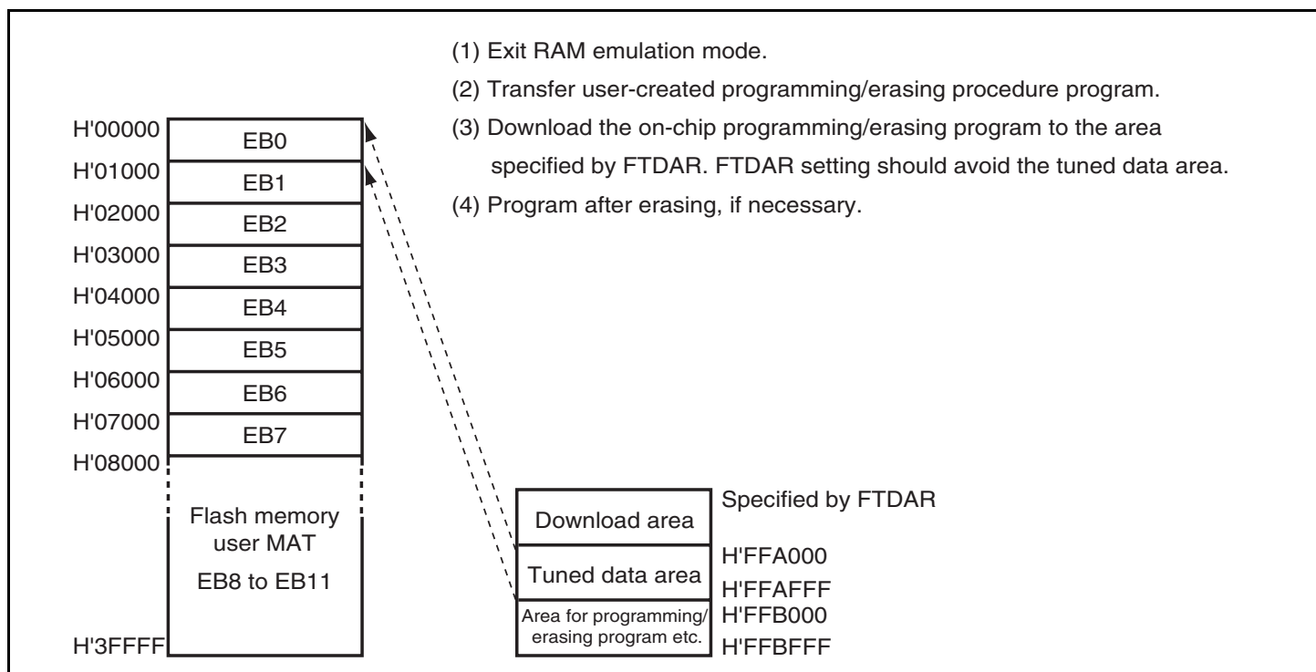
Figure 17.19 Programming Tuned Data
