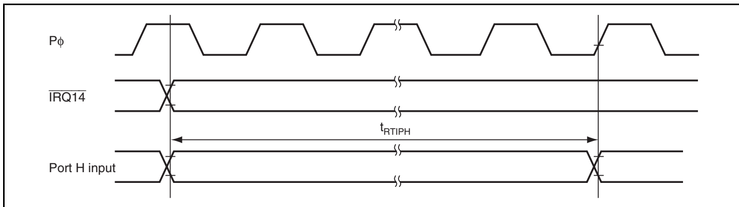
Figure 21.9 Data Input Timing for Realtime Input Port
