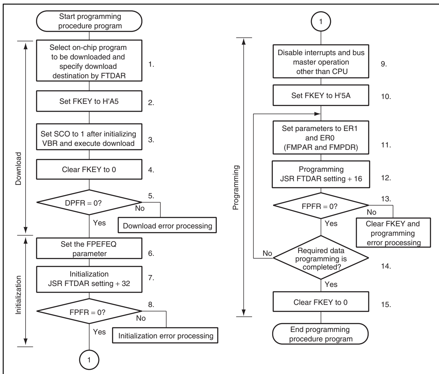
Figure 17.11 Programming Procedure in User Program Mode
