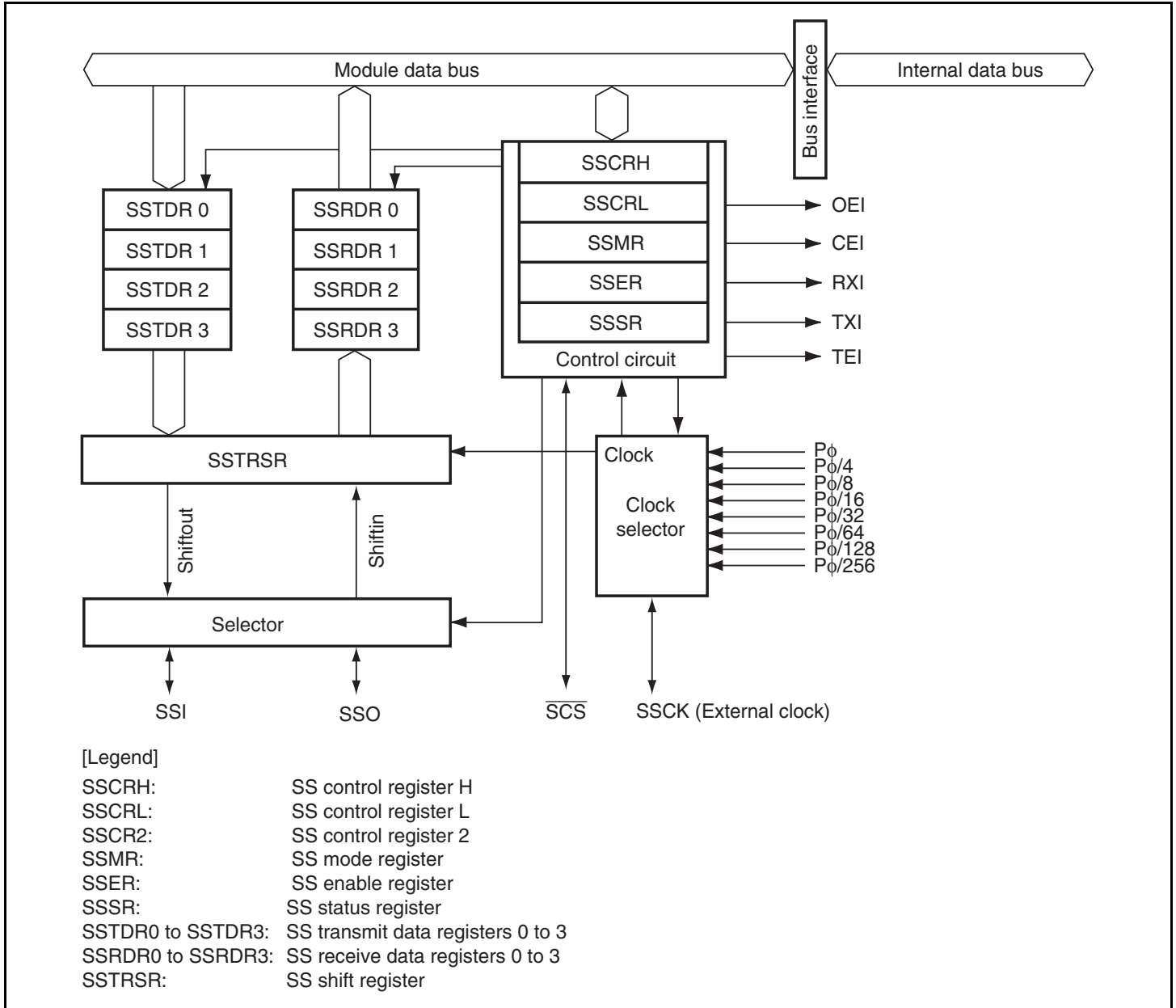
Figure 14.1 Block Diagram of SSU
