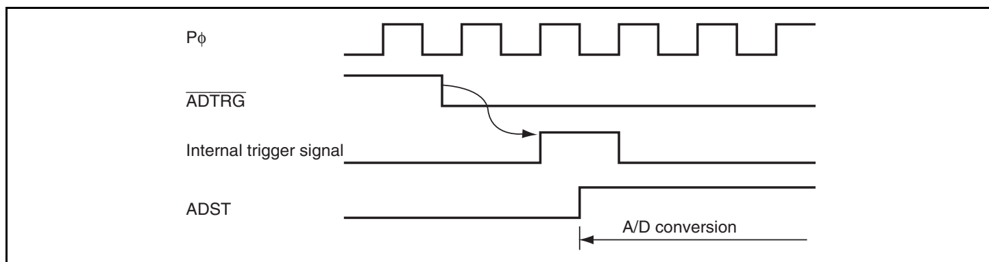
Figure 15.6 External Trigger Input Timing
