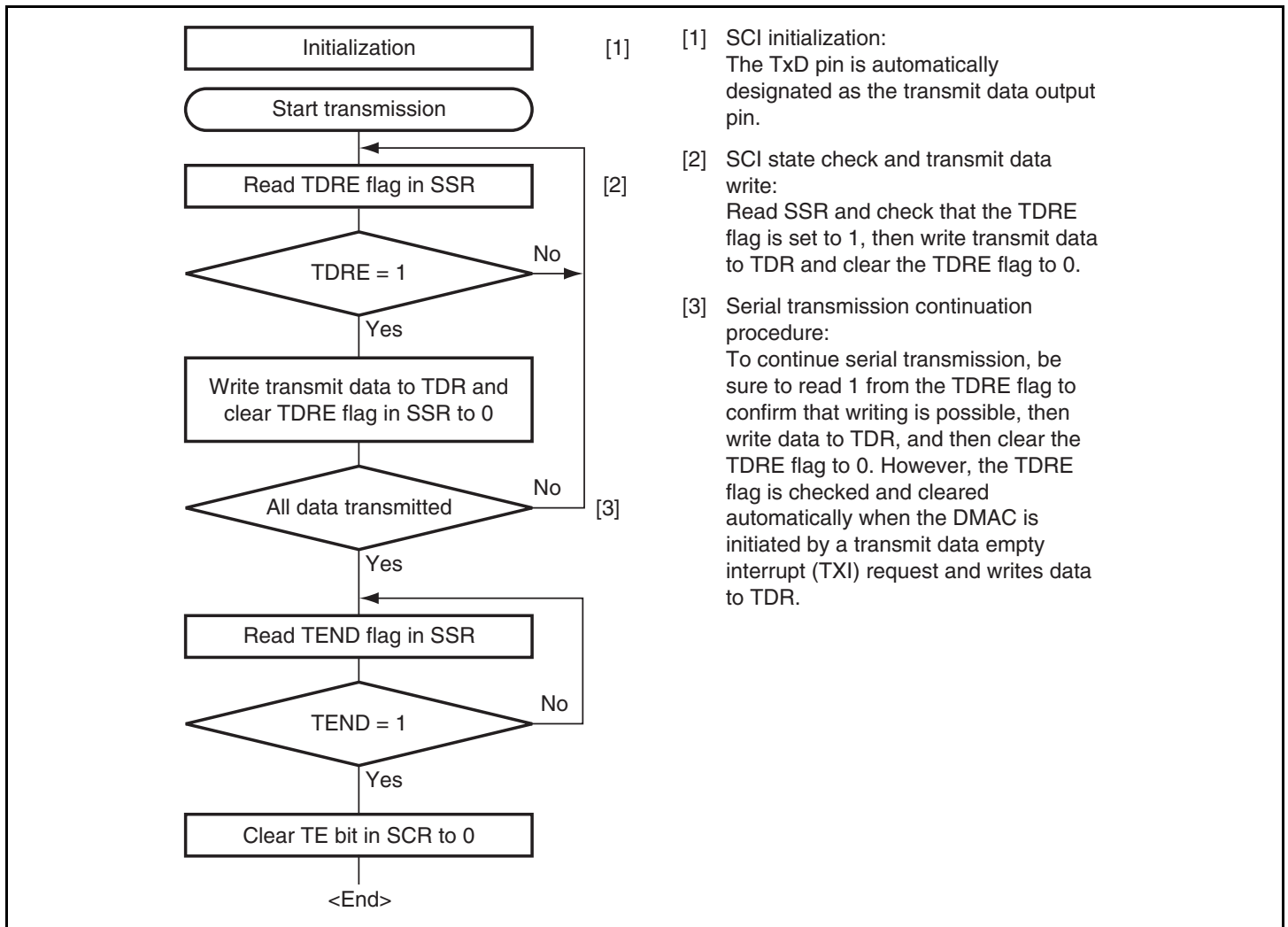
Figure 12.17 Sample Serial Transmission Flowchart
