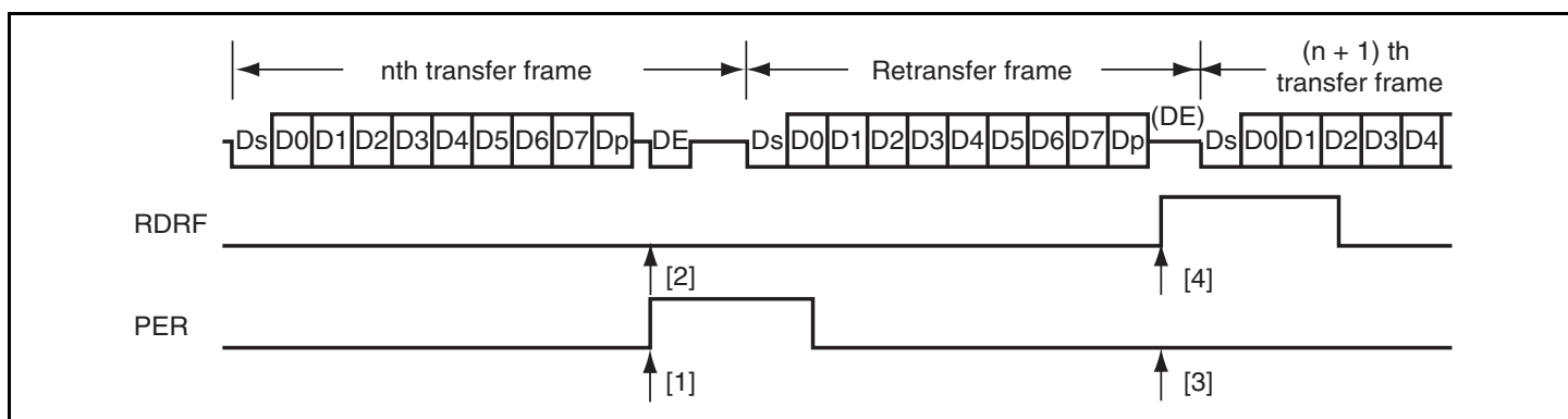
Figure 12.29 Data Re-Transfer Operation in SCI Reception Mode
