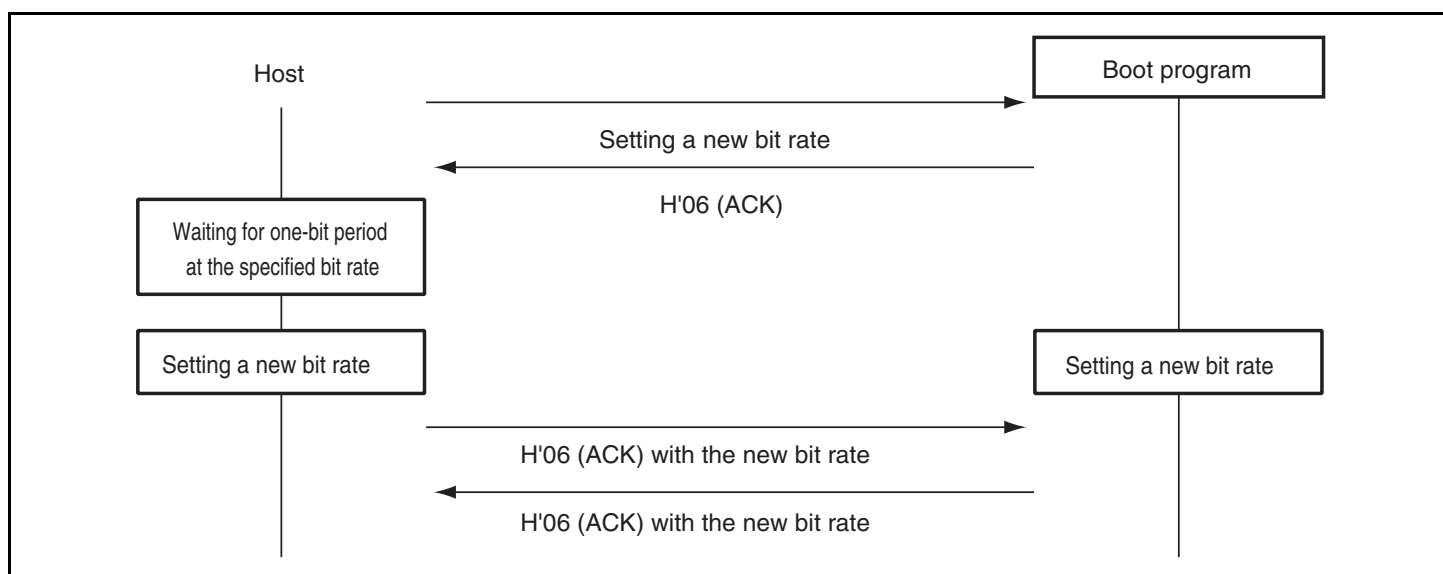
Figure 17.24 New Bit-Rate Selection Sequence
