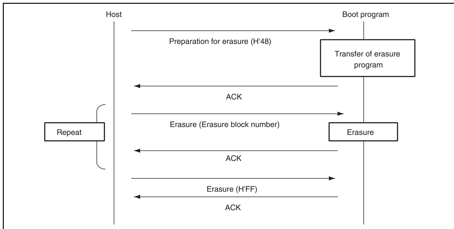
Figure 17.26 Erasure Sequence
