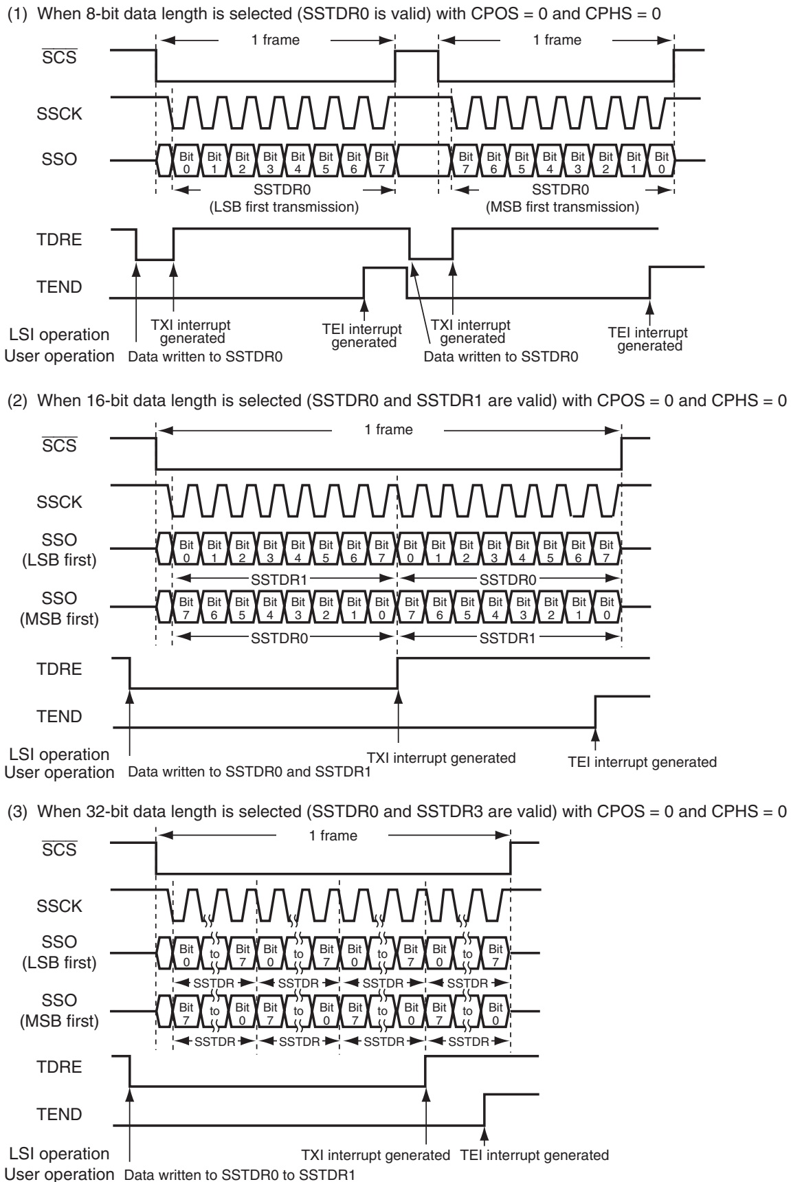
Figure 14.5 Example of Transmission Operation (SSU Mode)
