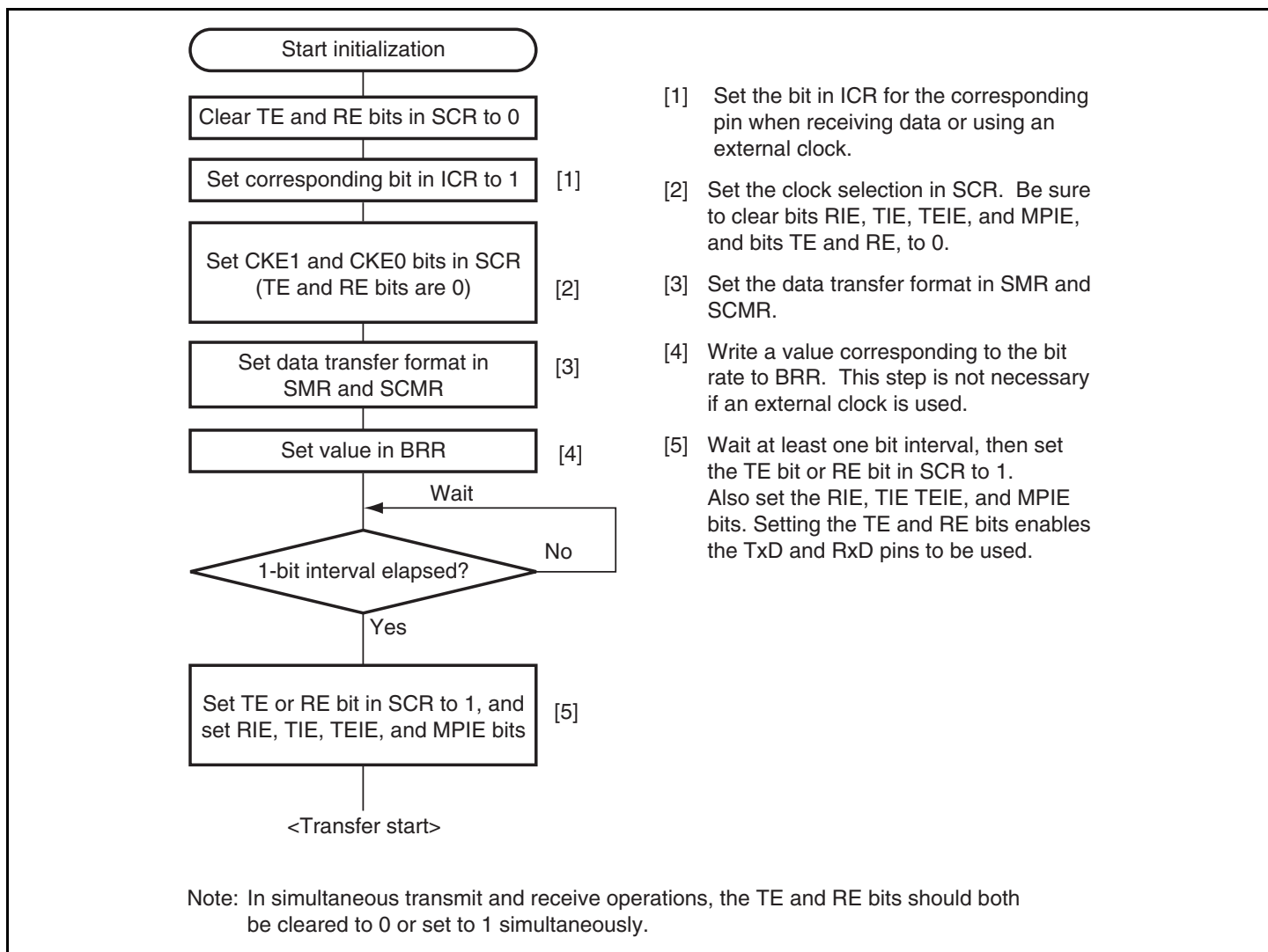
Figure 12.15 Sample SCI Initialization Flowchart
