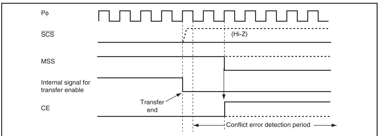
Figure 14.11 Conflict Error Detection Timing (After Transfer End)
