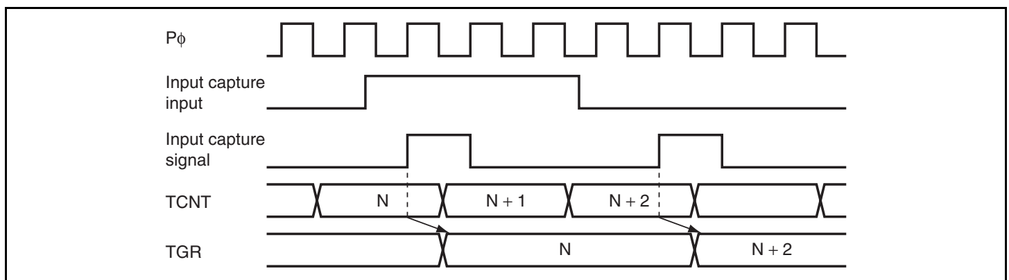
Figure 9.34 Input Capture Input Signal Timing
