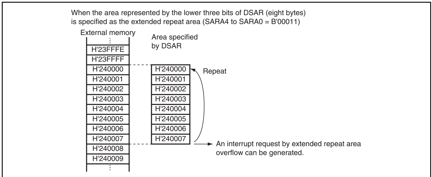
Figure 7.15 Example of Extended Repeat Area Operation
