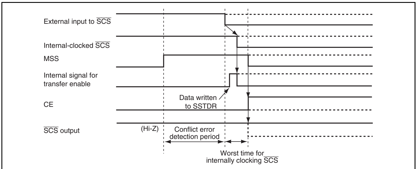
Figure 14.10 Conflict Error Detection Timing (Before Transfer)
