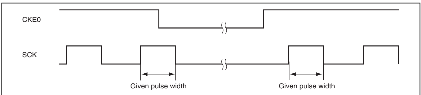
Figure 12.31 Clock Output Fixing Timing
