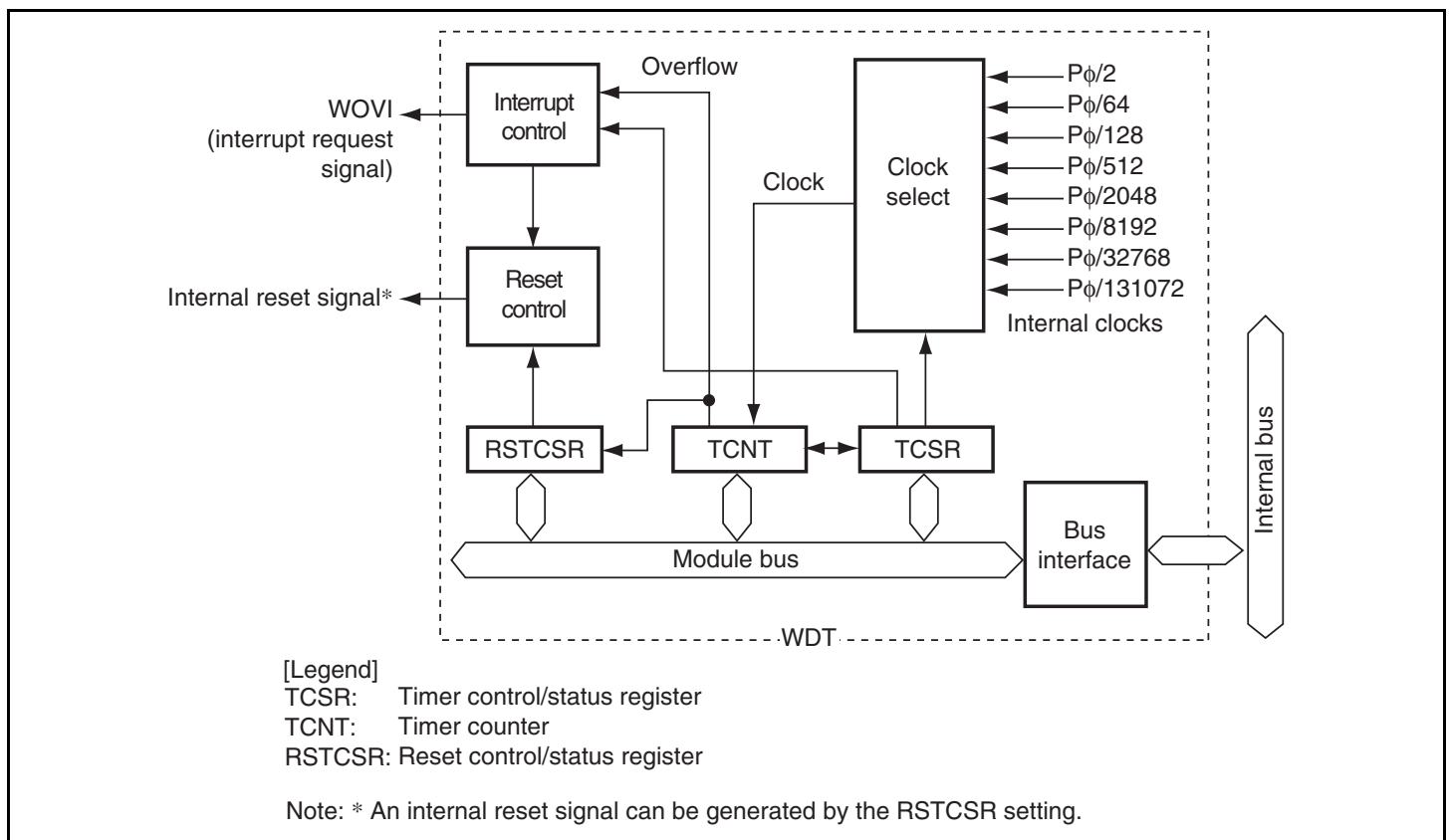
Figure 11.1 Block Diagram of WDT
