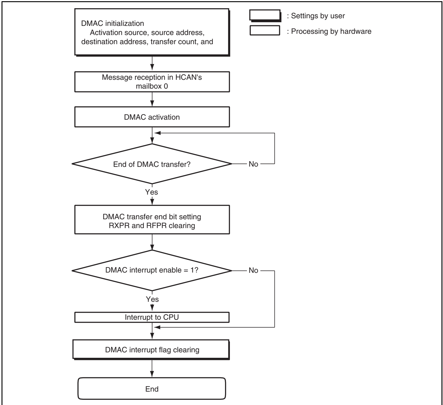
Figure 13.15 DMAC Transfer Flowchart
