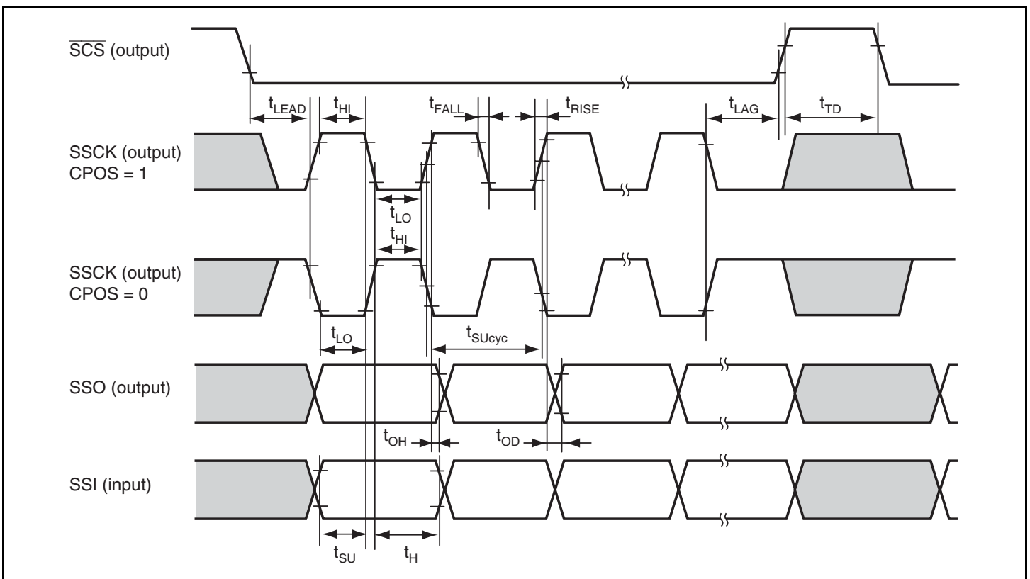
Figure 21.18 SSU Timing (Master, CPHS = 0)
