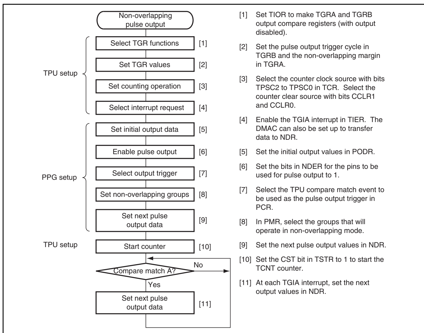
Figure 10.8 Setup Procedure for Non-Overlapping Pulse Output (Example)
