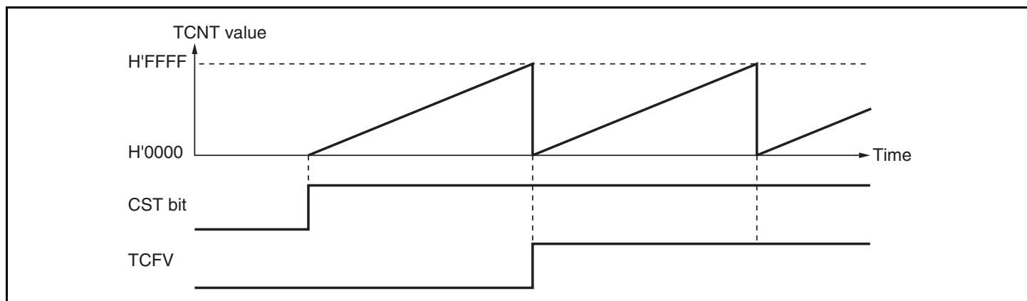
Figure 9.4 Free-Running Counter Operation
