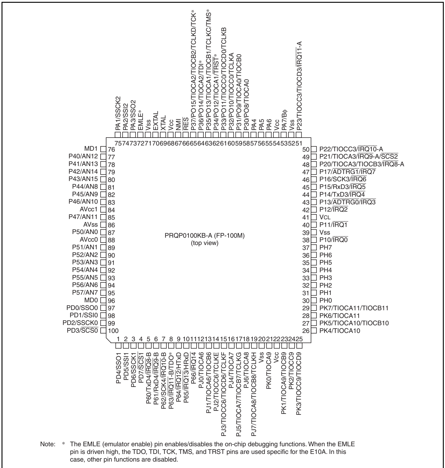
Figure 1.3 Pin Assignments of H8SX/1527
