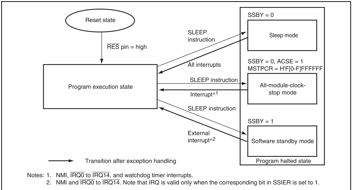
Figure 19.1 Mode Transitions
