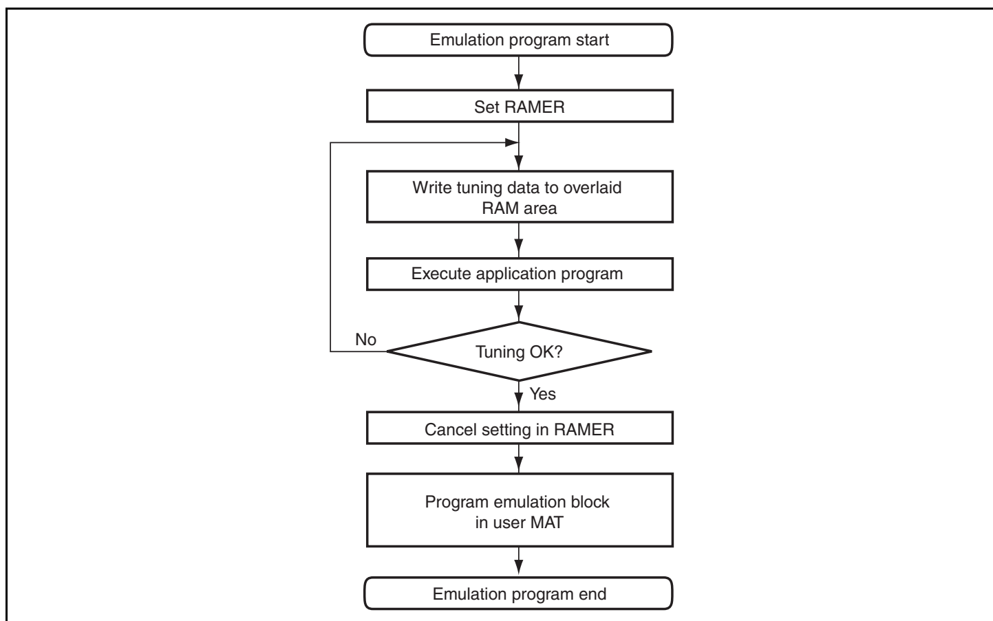
Figure 17.17 RAM Emulation Flow
