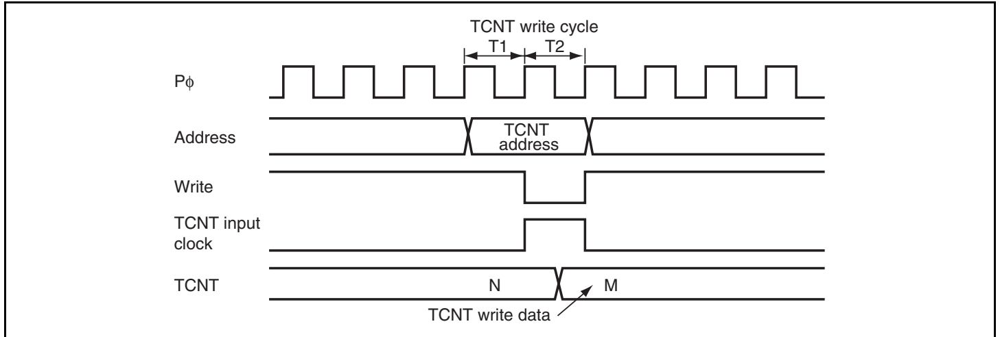
Figure 9.48 Conflict between TCNT Write and Increment Operations
