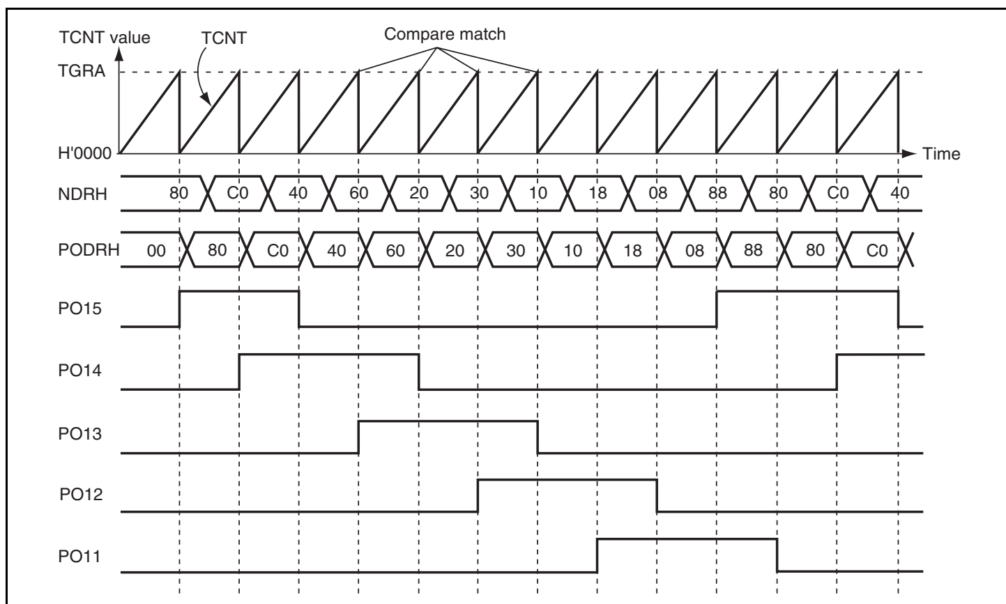
Figure 10.5 Normal Pulse Output Example (5-Phase Pulse Output)
