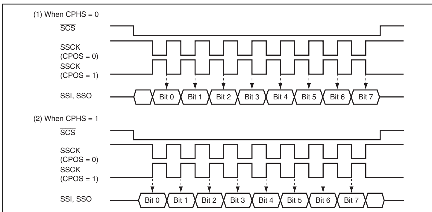
Figure 14.2 Relationship of Clock Phase, Polarity, and Data
