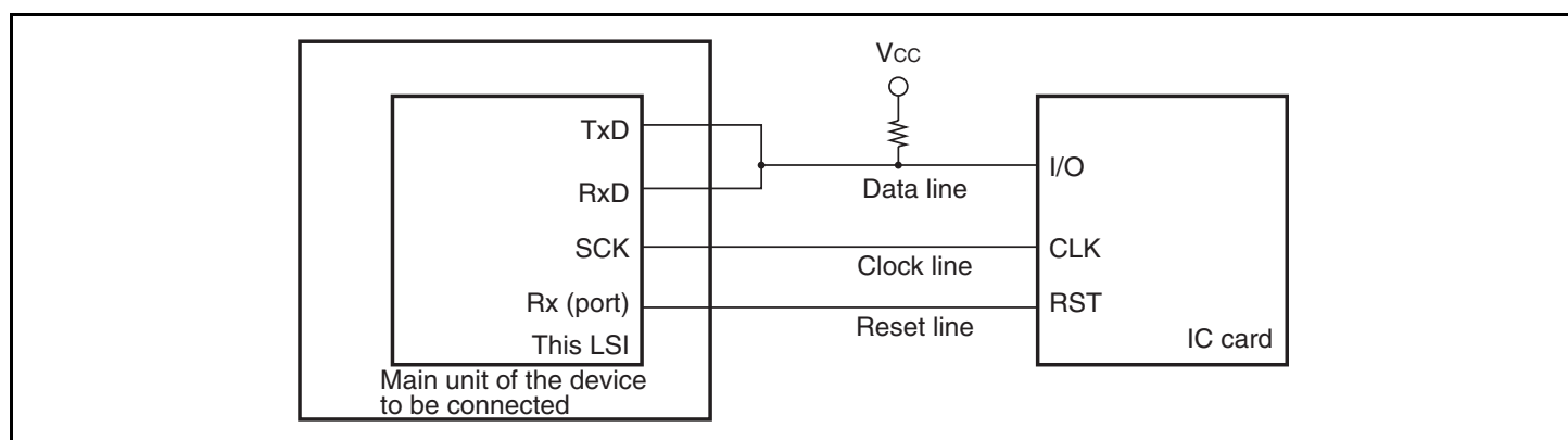
Figure 12.21 Pin Connection for Smart Card Interface
