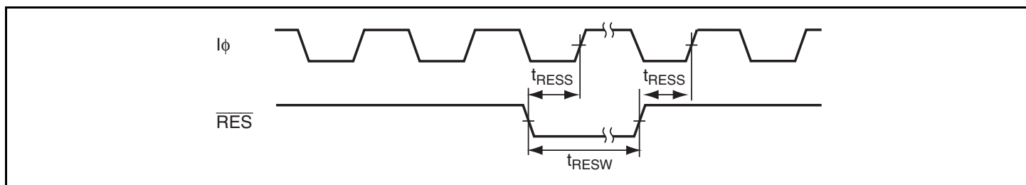
Figure 21.6 Reset Input Timing
