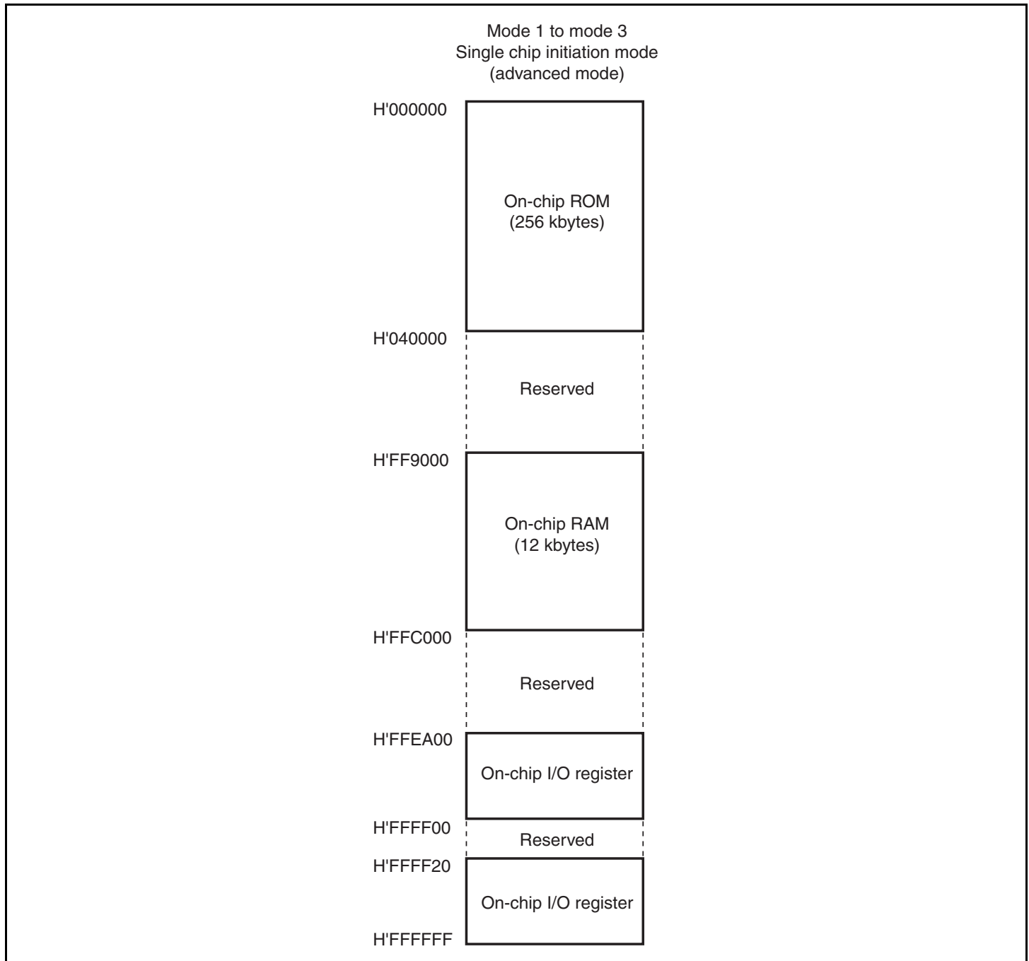
Figure 3.1 Address Map (Advanced Mode)
