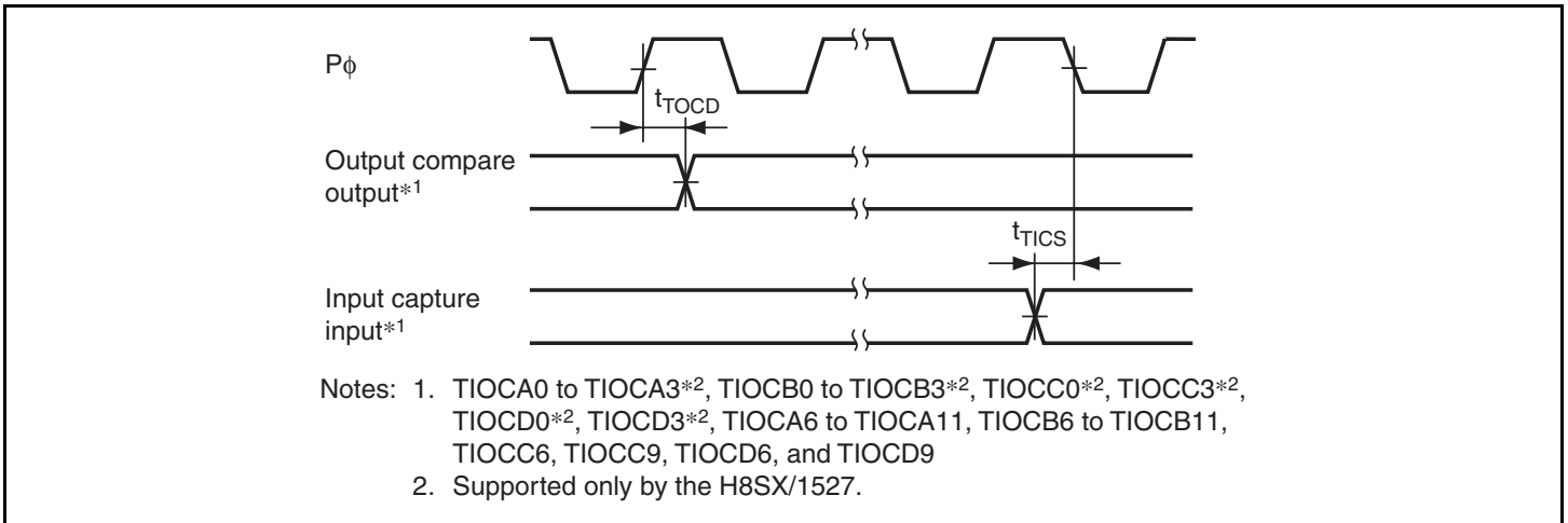
Figure 21.10 TPU Input/Output Timing
