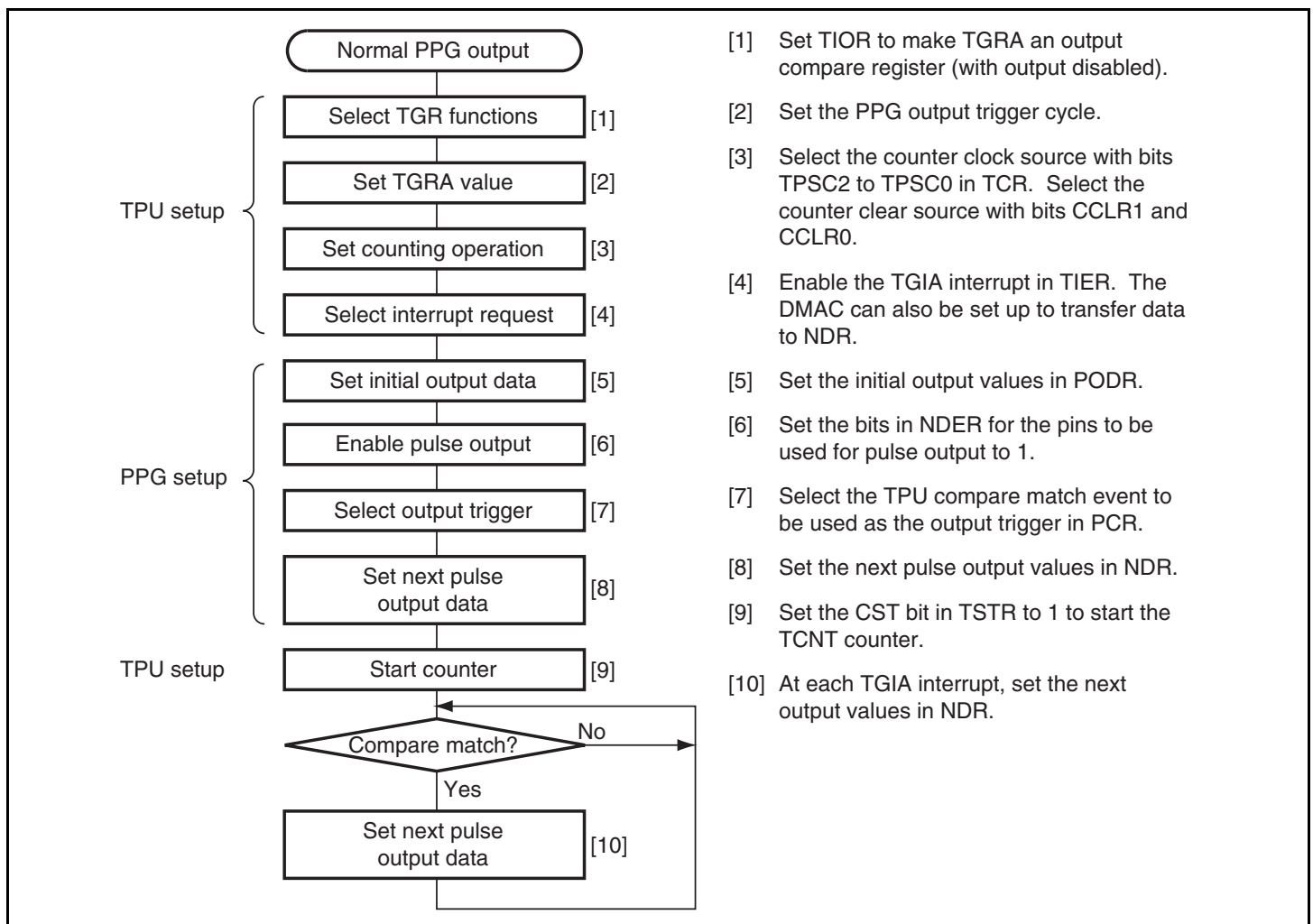
Figure 10.4 Setup Procedure for Normal Pulse Output (Example)
