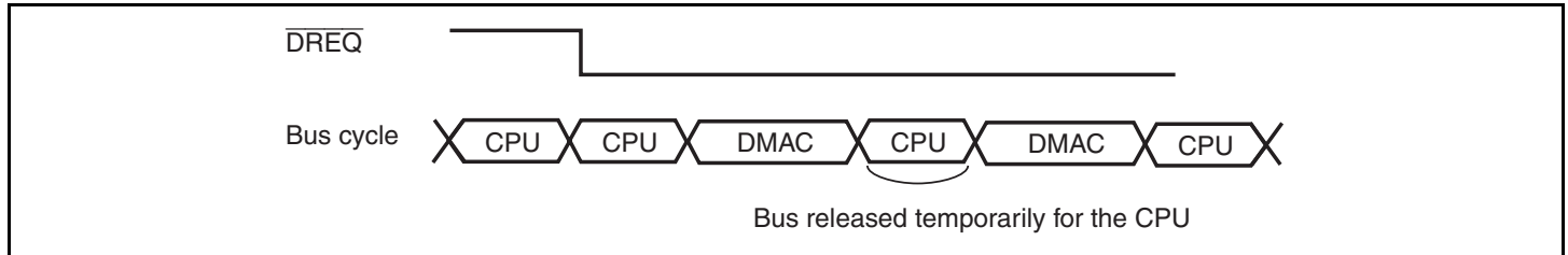
Figure 7.13 Example of Timing in Cycle Stealing Mode
