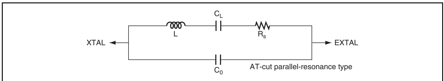
Figure 18.3 Crystal Resonator Equivalent Circuit
