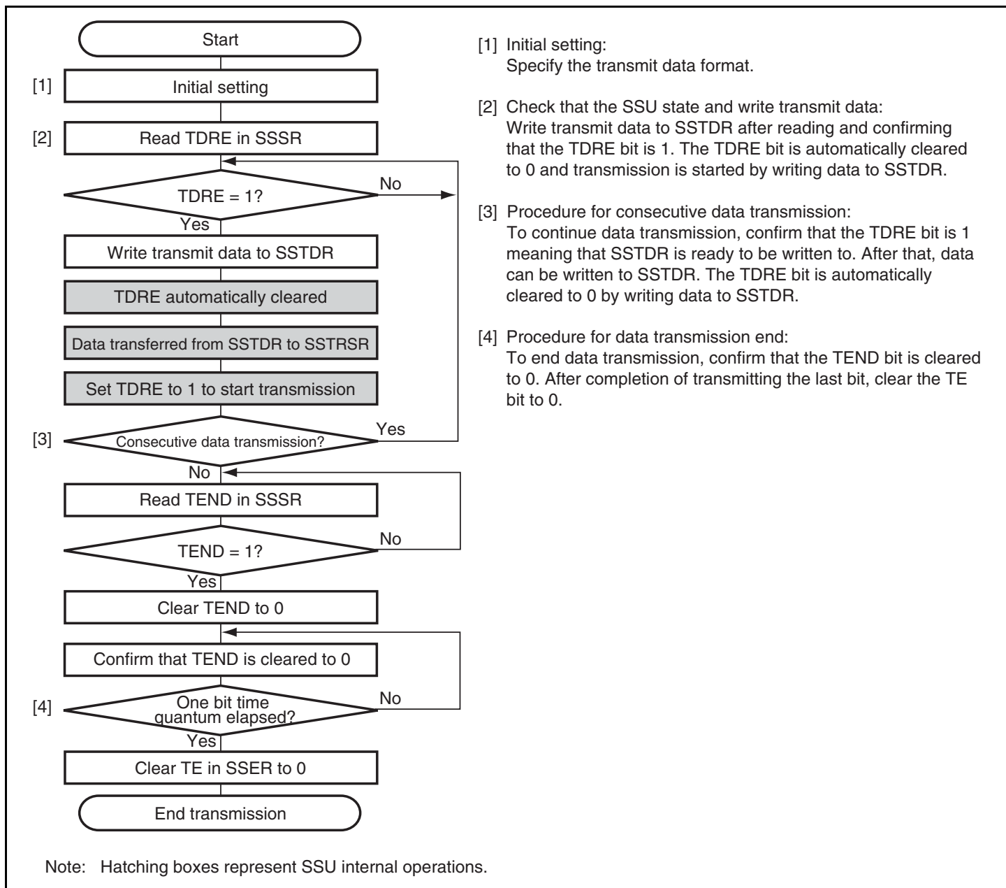
Figure 14.6 Flowchart Example of Data Transmission (SSU Mode)
