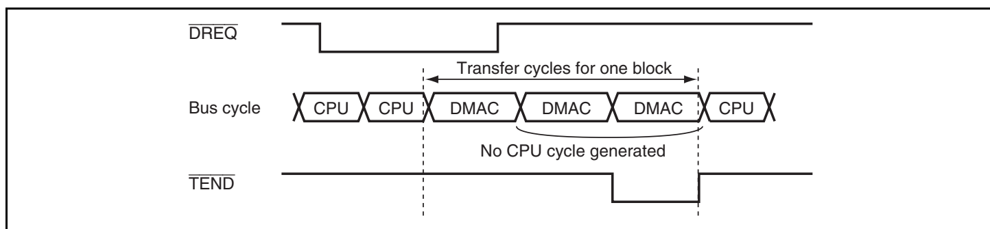
Figure 7.10 Operations in Block Transfer Mode
