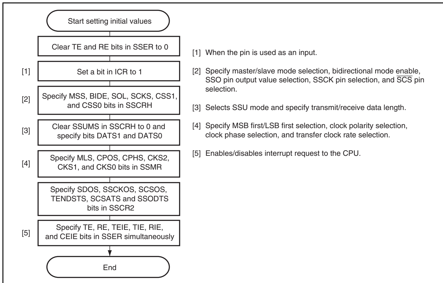
Figure 14.4 Example of Initial Settings in SSU Mode
