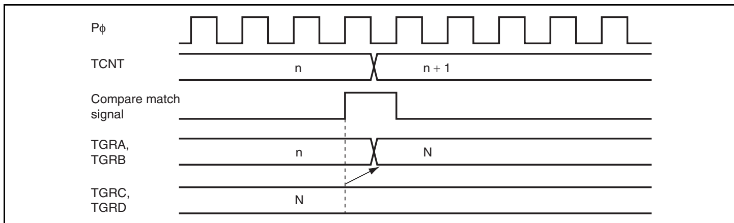
Figure 9.37 Buffer Operation Timing (Compare Match)
