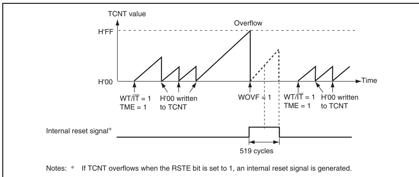
Figure 11.2 Operation in Watchdog Timer Mode
