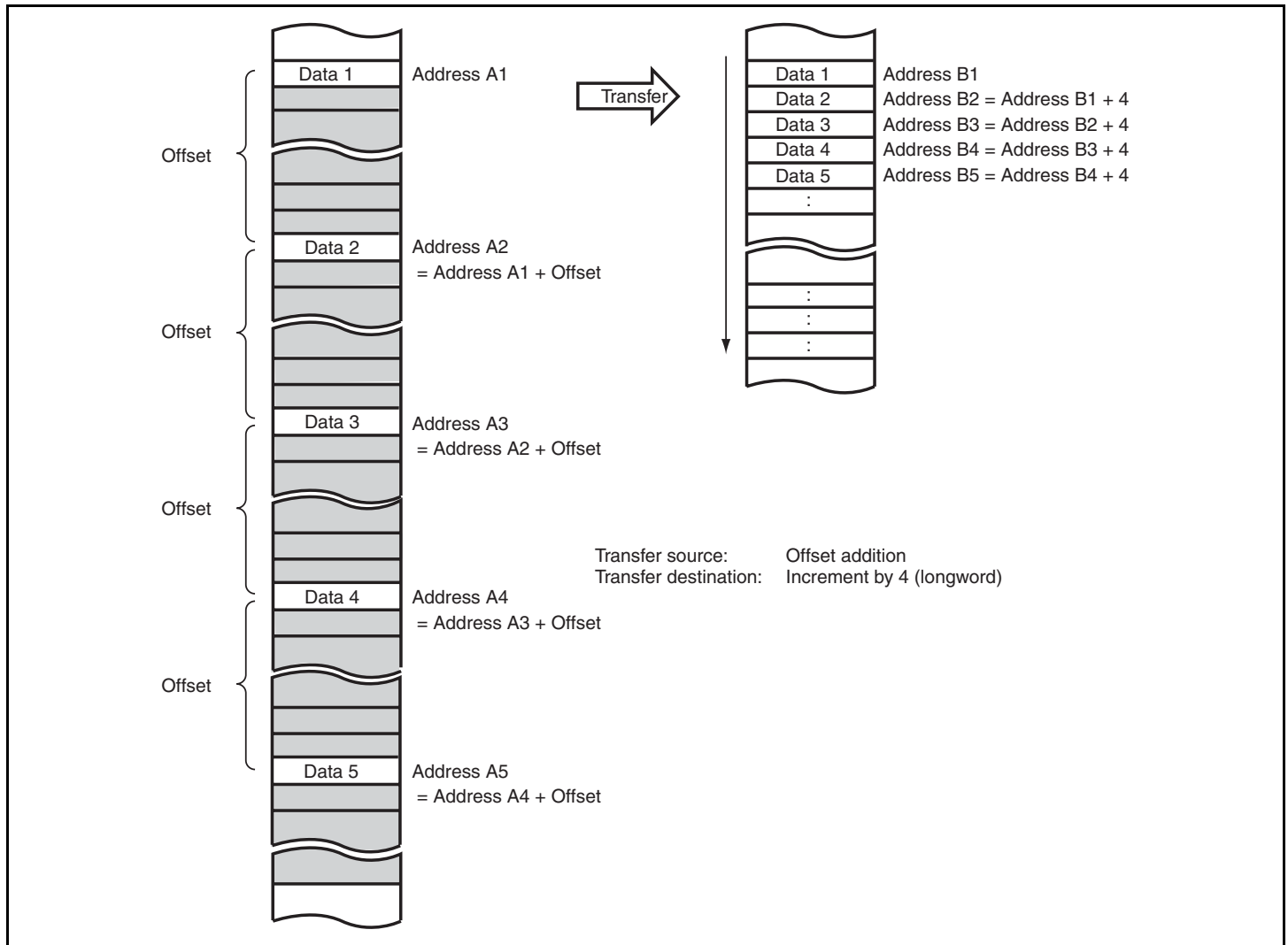
Figure 7.18 Operation of Offset Addition
