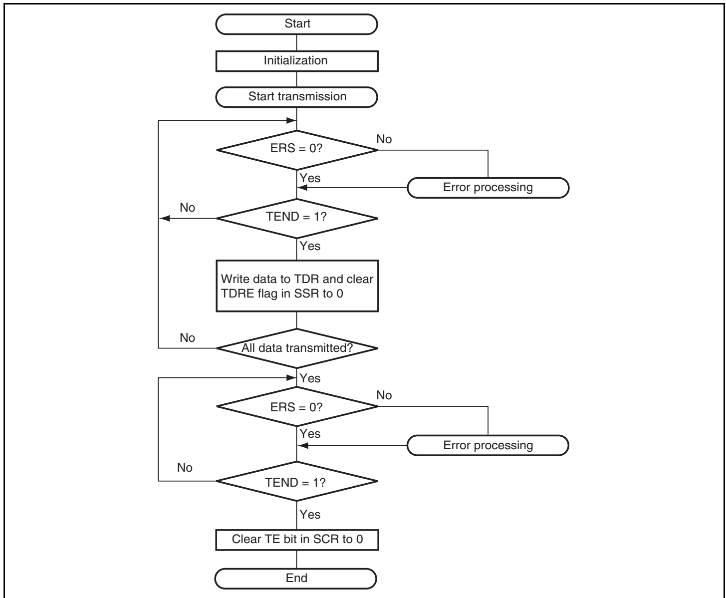
Figure 12.28 Sample Transmission Flowchart
