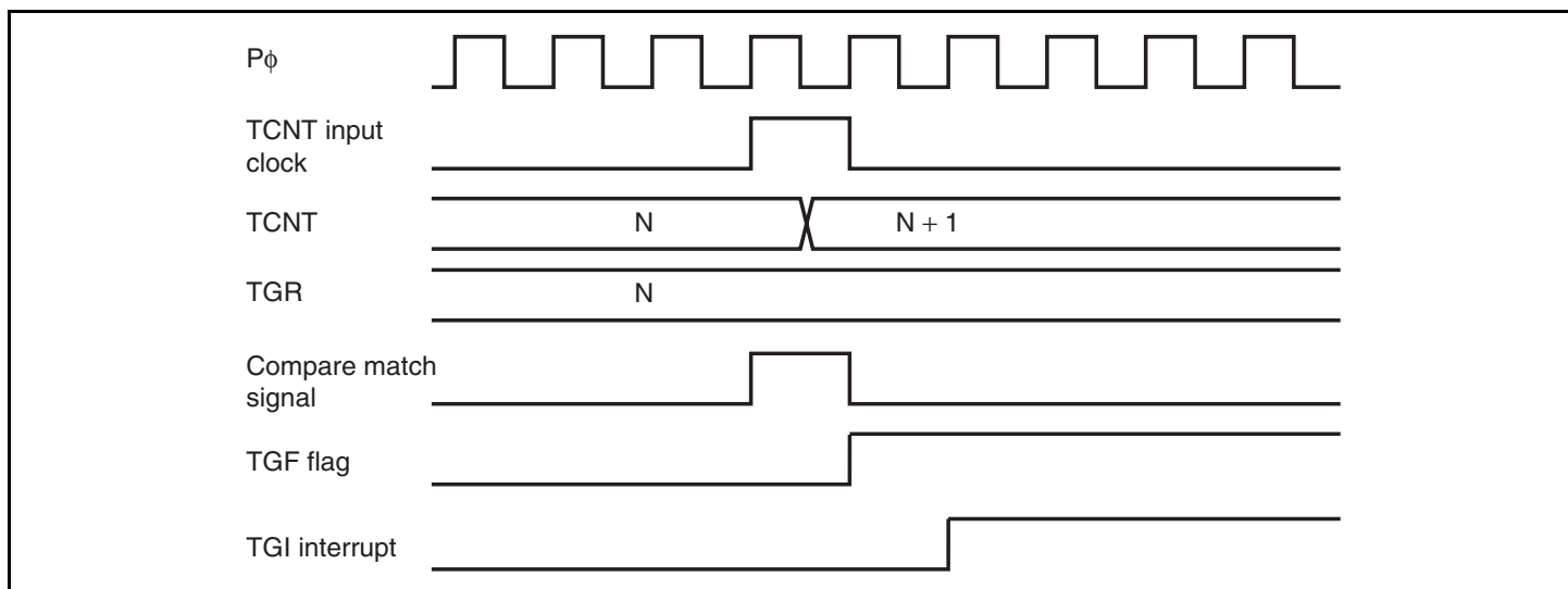
Figure 9.39 TGI Interrupt Timing (Compare Match)
