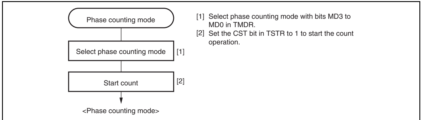
Figure 9.25 Example of Phase Counting Mode Setting Procedure
