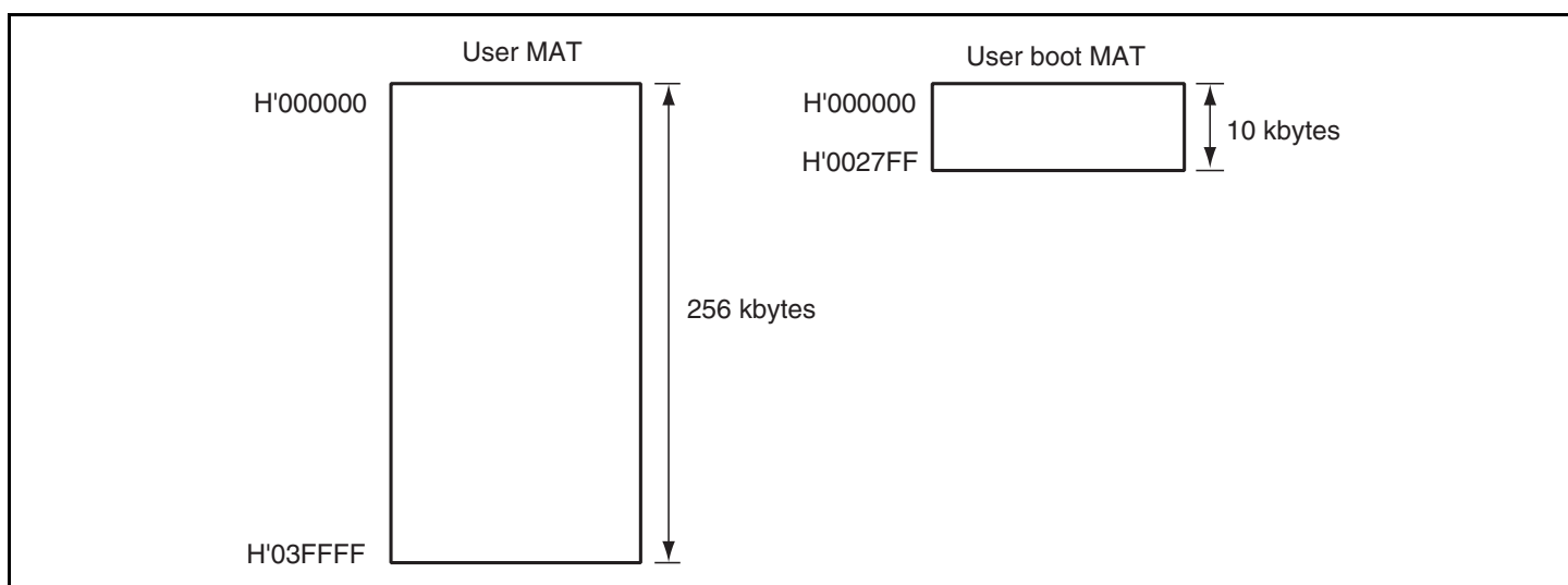
Figure 17.3 Memory MAT Configuration
