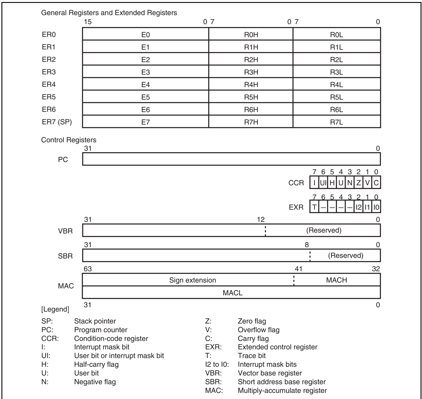
Figure 2.9 CPU Registers
