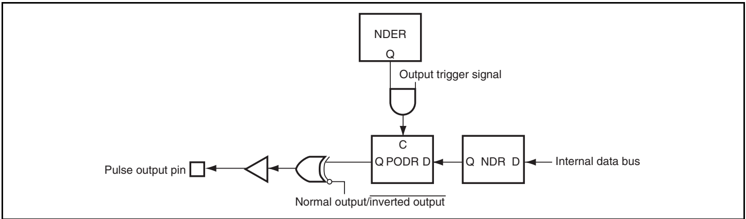
Figure 10.2 Schematic Diagram of PPG
