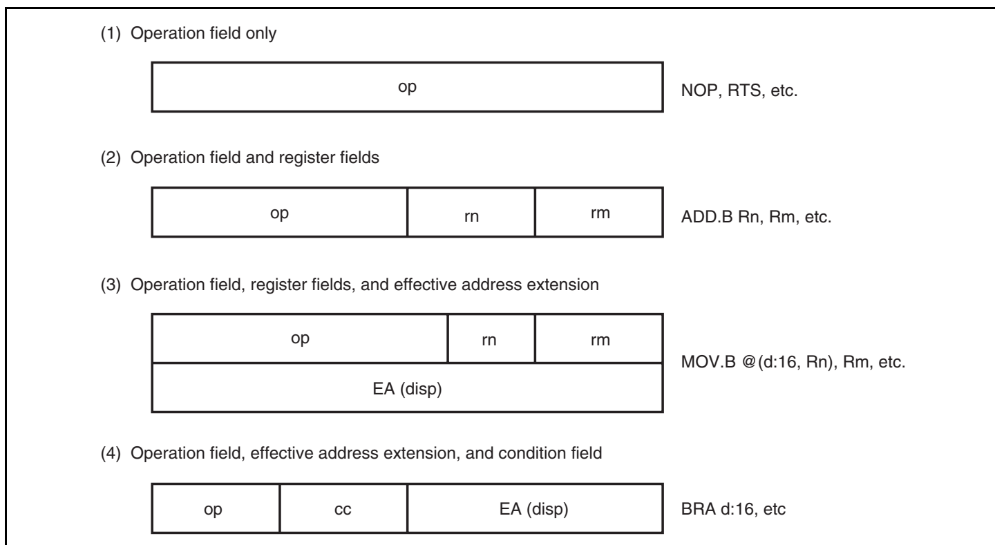
Figure 2.14 Instruction Formats
