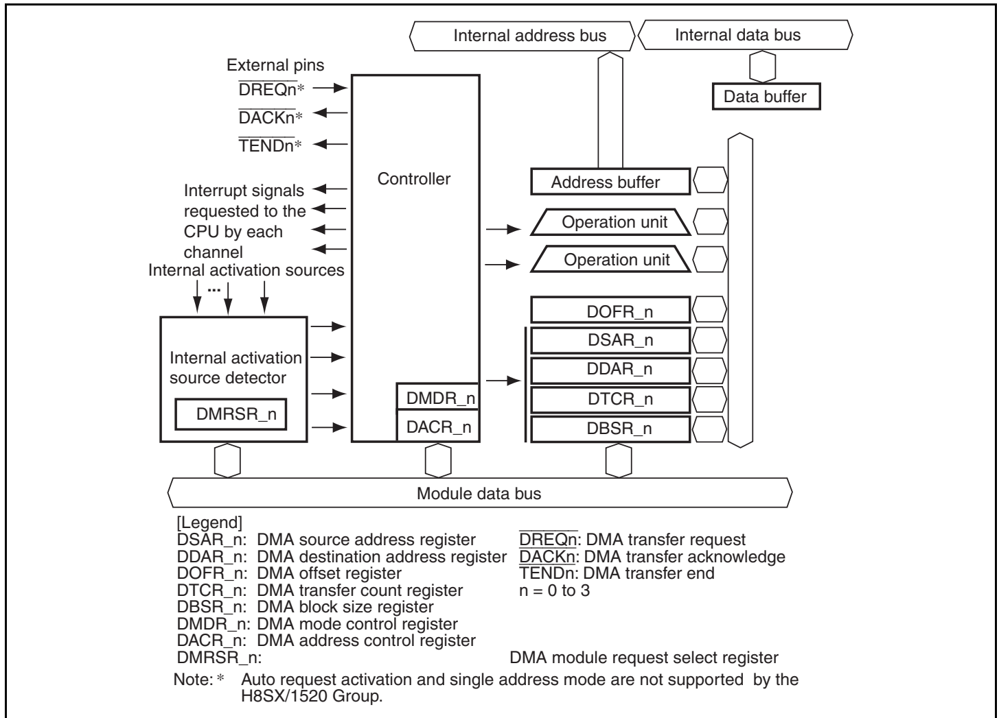
Figure 7.1 Block Diagram of DMAC
