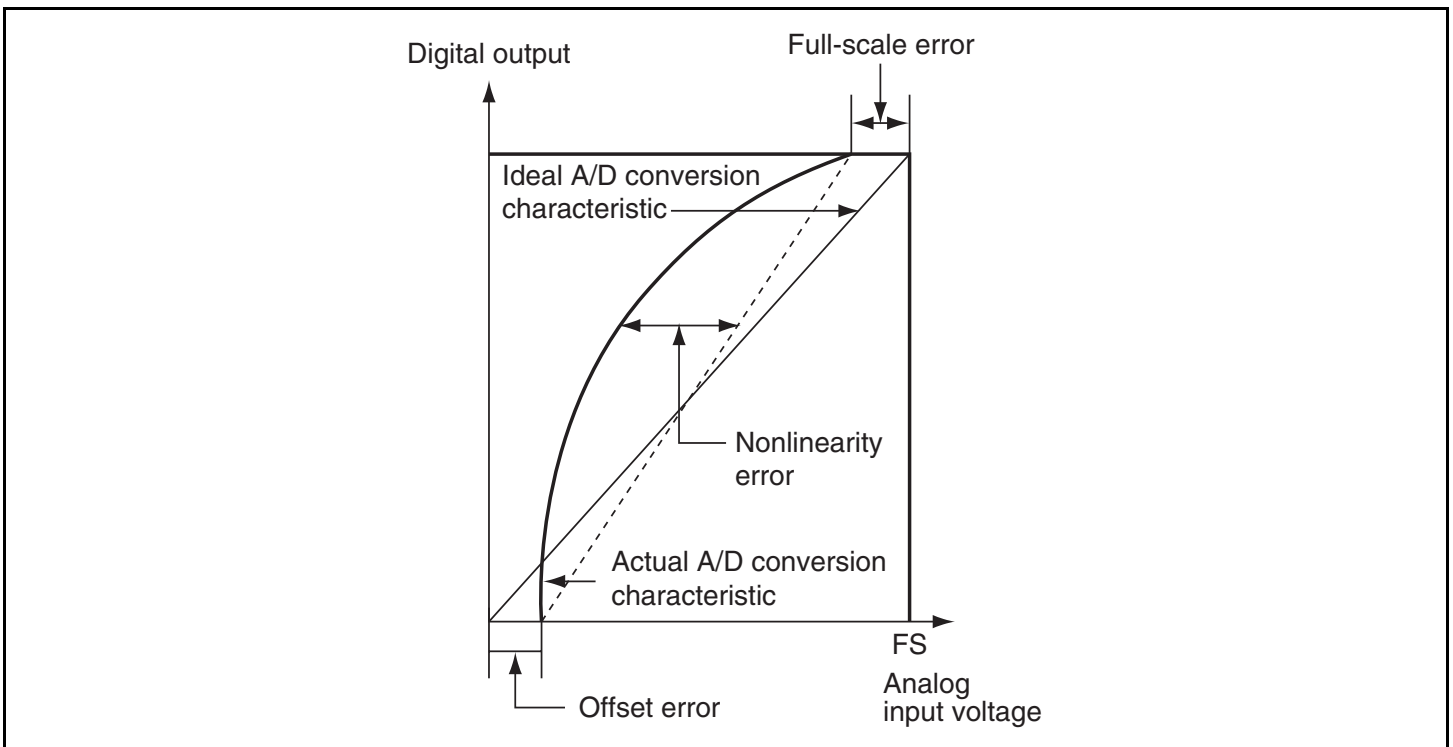
Figure 15.8 A/D Conversion Accuracy Definitions
