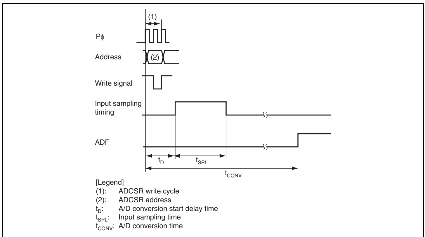
Figure 15.5 A/D Conversion Timing
