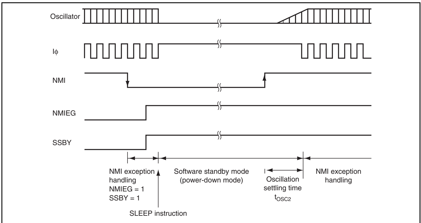
Figure 19.2 Software Standby Mode Application Example
