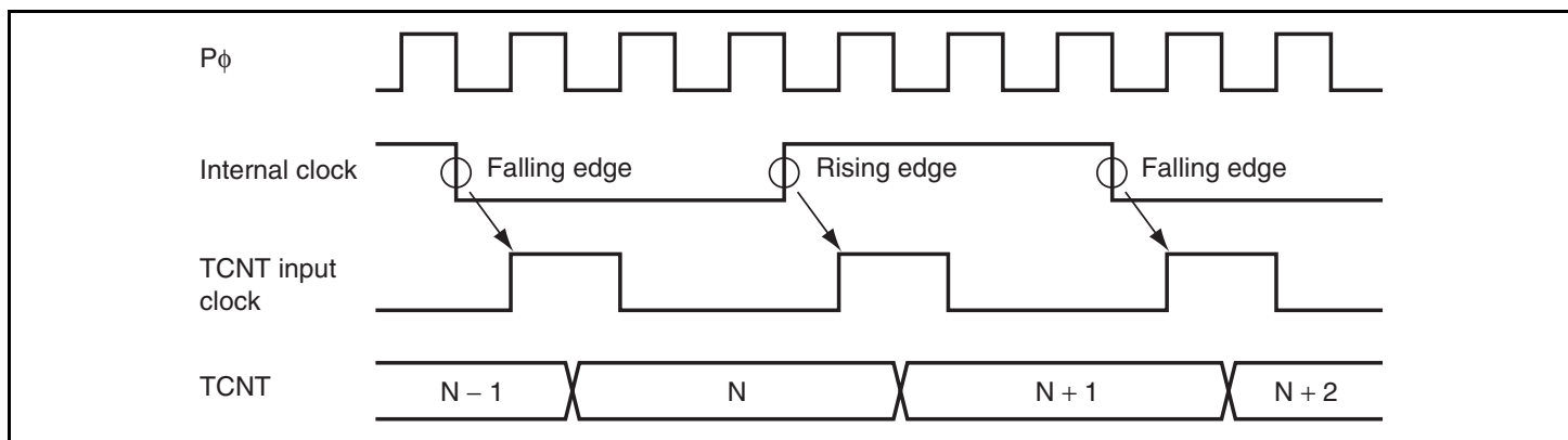
Figure 9.31 Count Timing in Internal Clock Operation
