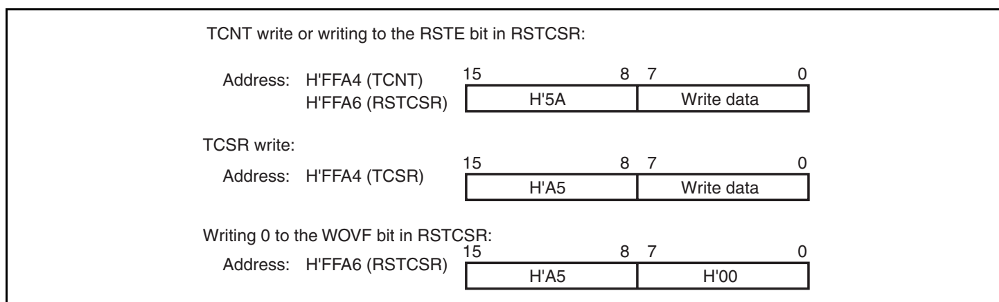
Figure 11.4 Writing to TCNT, TCSR, and RSTCSR
