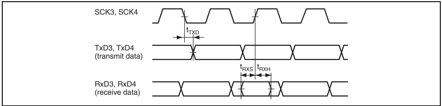
Figure 21.14 SCI Input/Output Timing: Clocked Synchronous Mode
