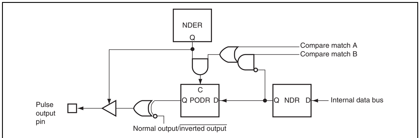
Figure 10.6 Non-Overlapping Pulse Output
