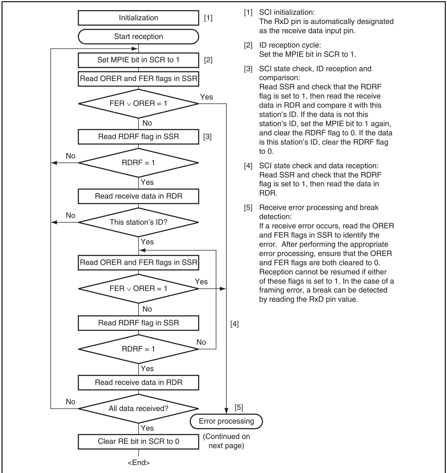
Figure 12.13 Sample Multiprocessor Serial Reception Flowchart (1)
