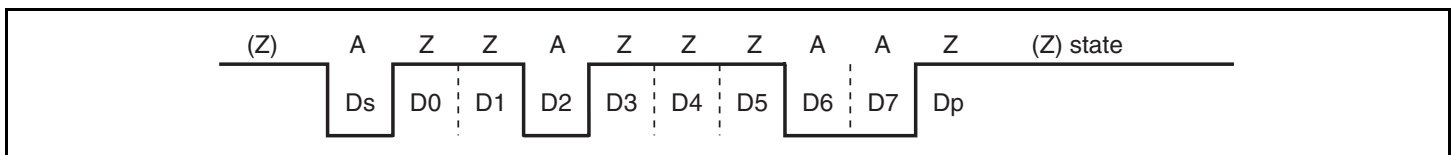
Figure 12.23 Direct Convention (SDIR = SINV = \overline{O/\overline{E}} = 0)
