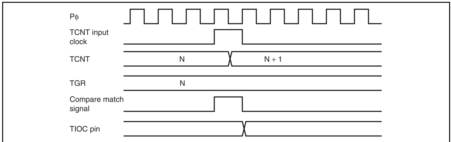
Figure 9.33 Output Compare Output Timing
