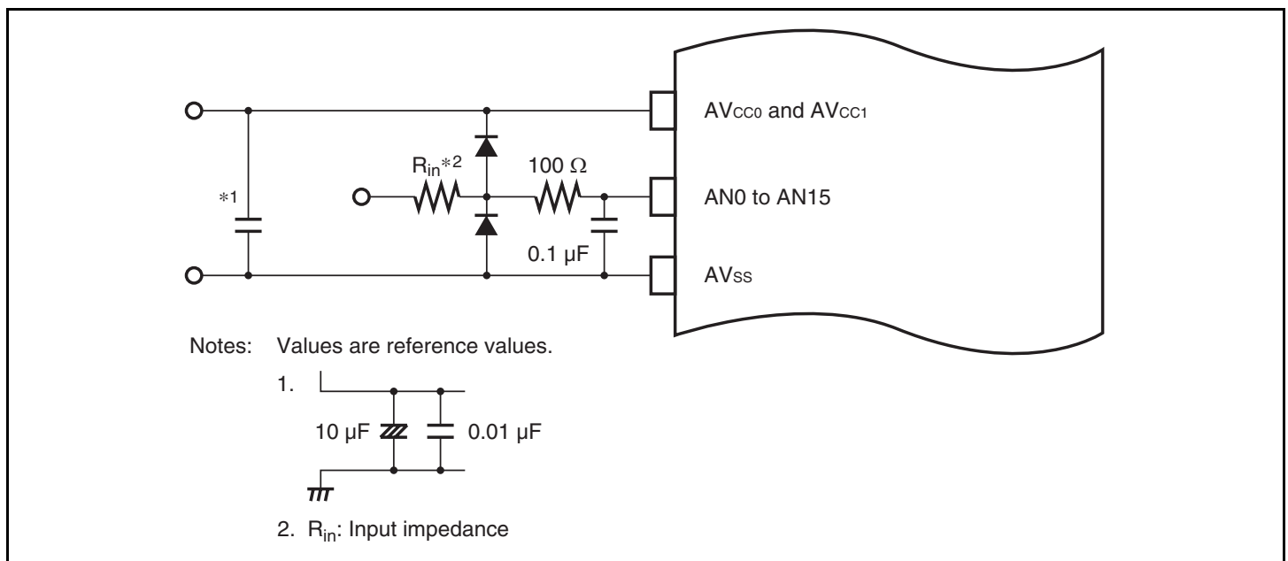
Figure 15.10 Example of Analog Input Protection Circuit
