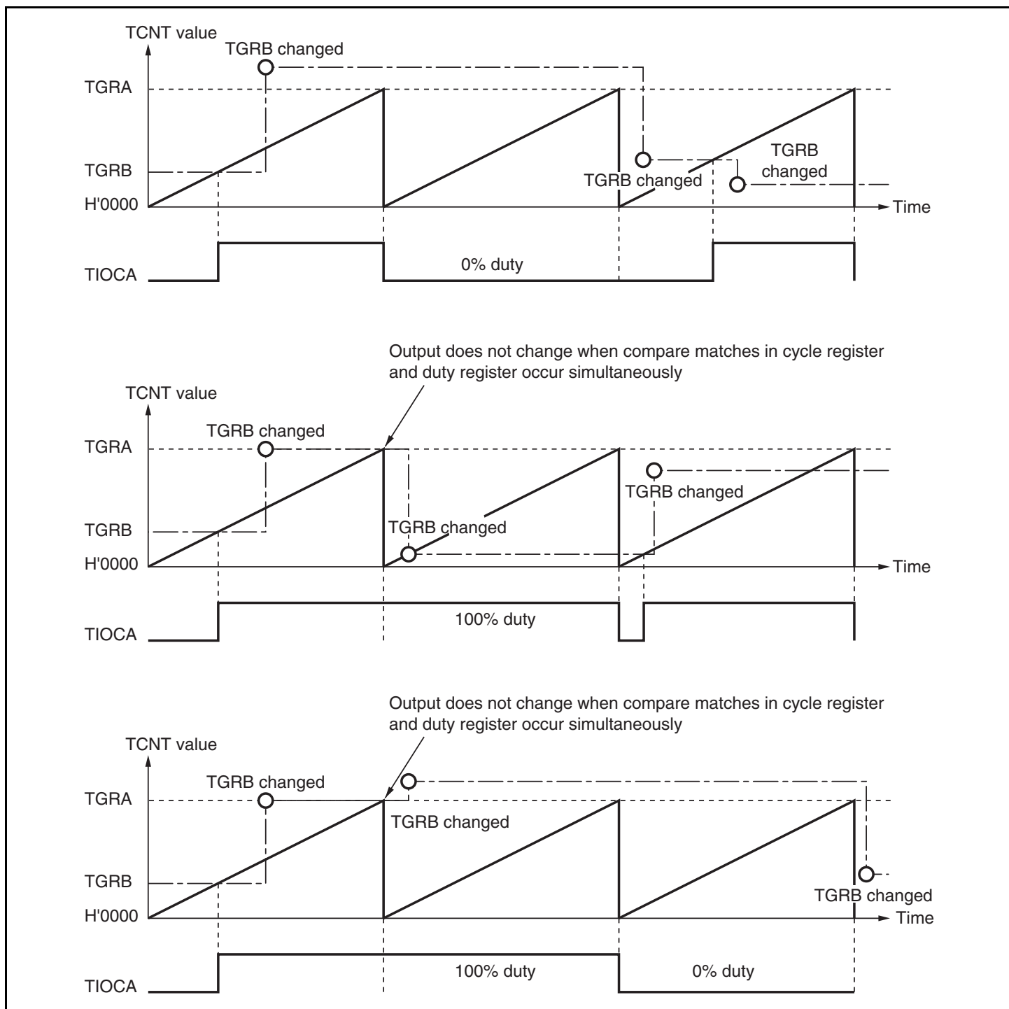
Figure 9.24 Example of PWM Mode Operation (3)
