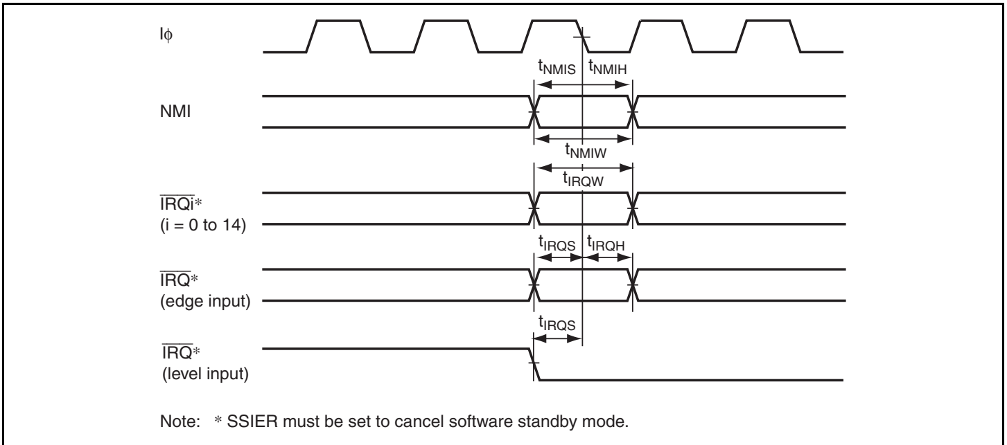
Figure 21.7 Interrupt Input Timing
