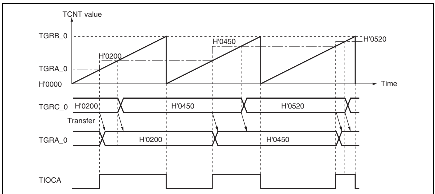
Figure 9.16 Example of Buffer Operation (1)
