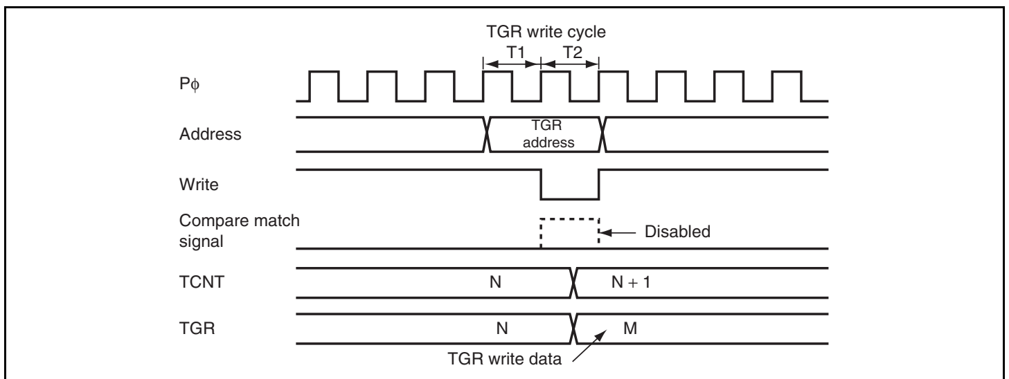
Figure 9.49 Conflict between TGR Write and Compare Match
