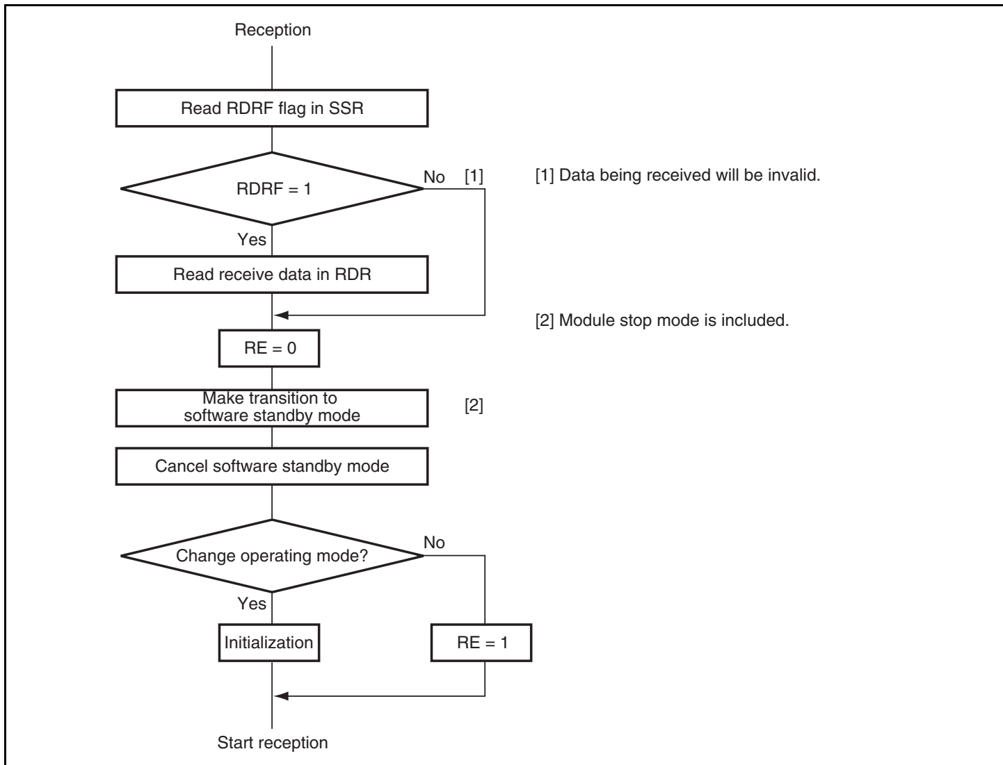
Figure 12.37 Sample Flowchart for Mode Transition during Reception
