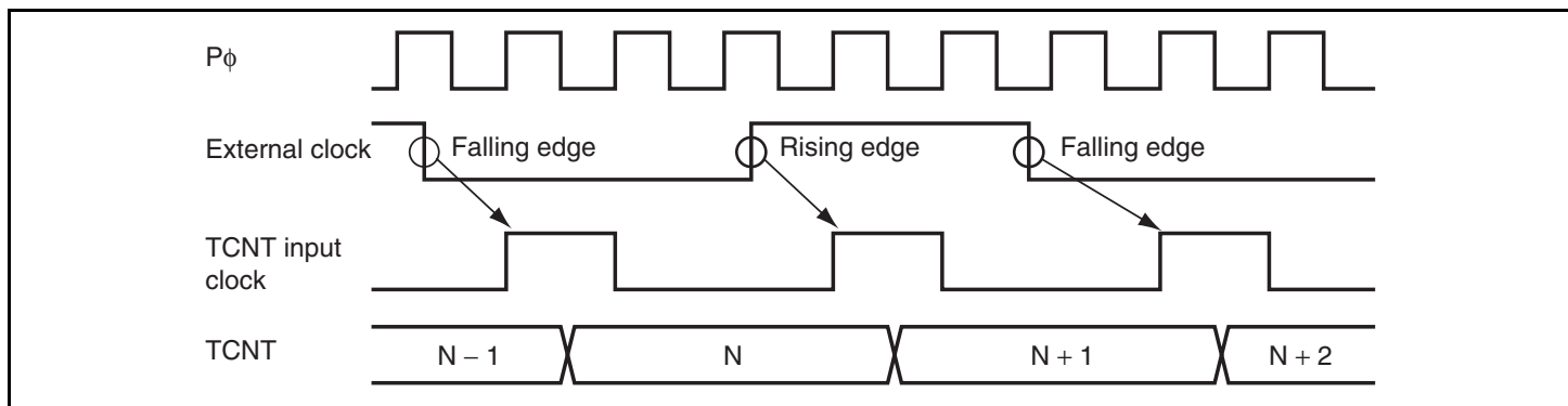
Figure 9.32 Count Timing in External Clock Operation
