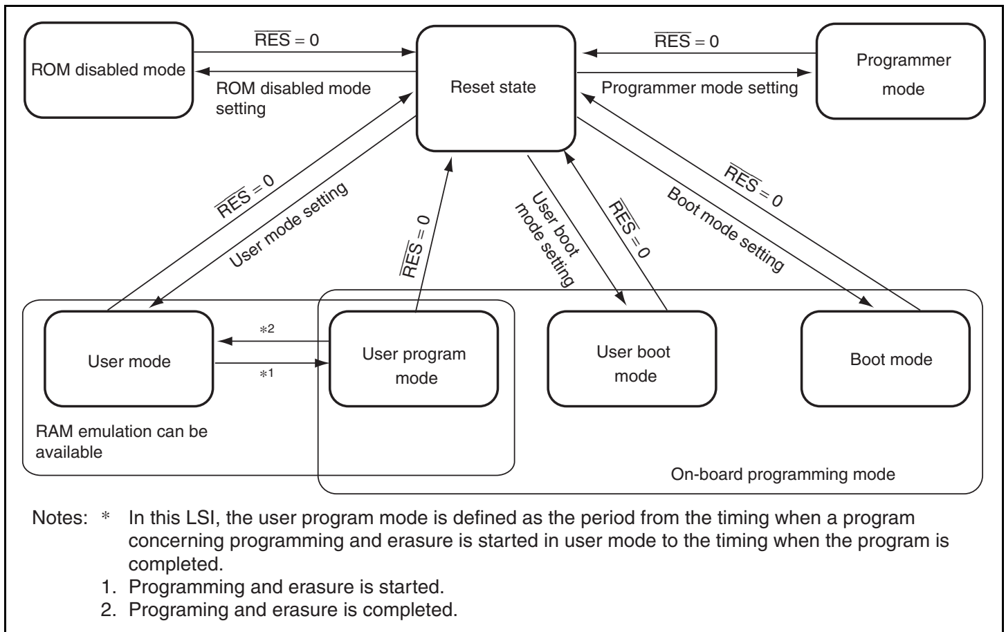
Figure 17.2 Mode Transition of Flash Memory
