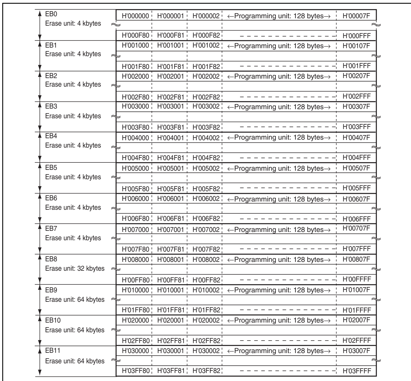
Figure 17.4 Block Structure of User MAT
