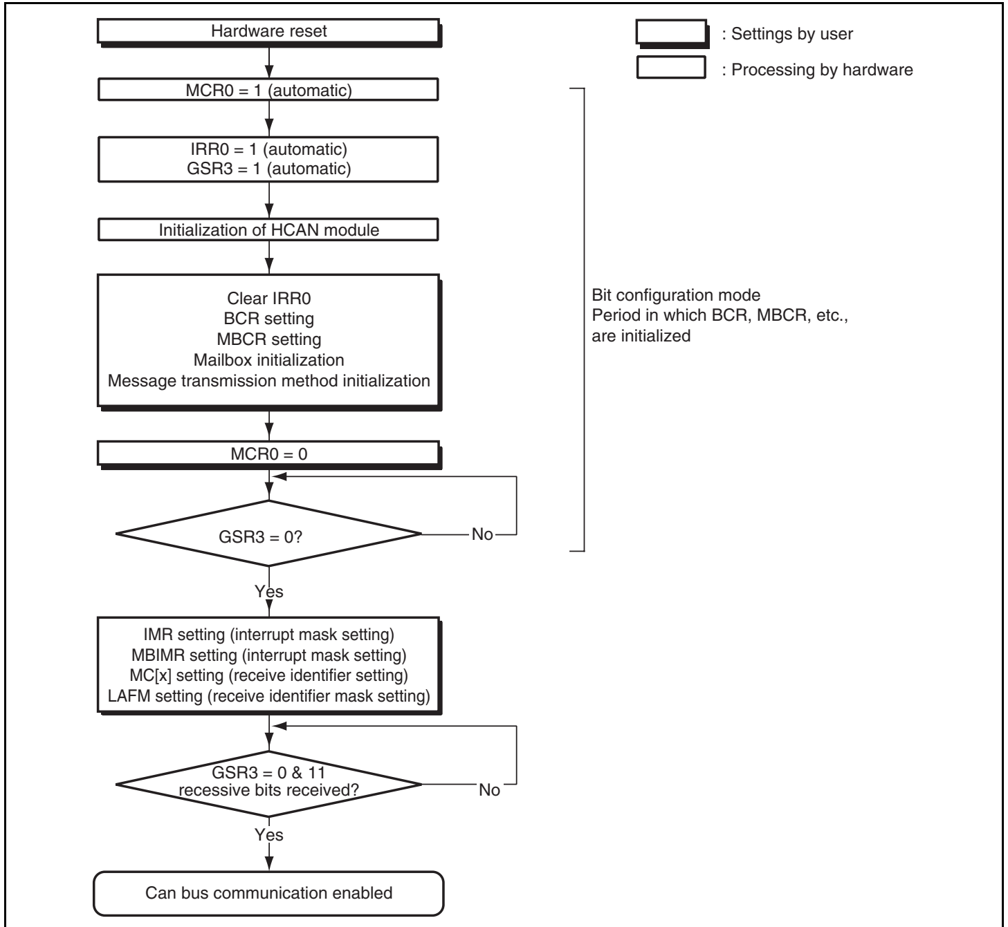
Figure 13.6 Hardware Reset Flowchart
