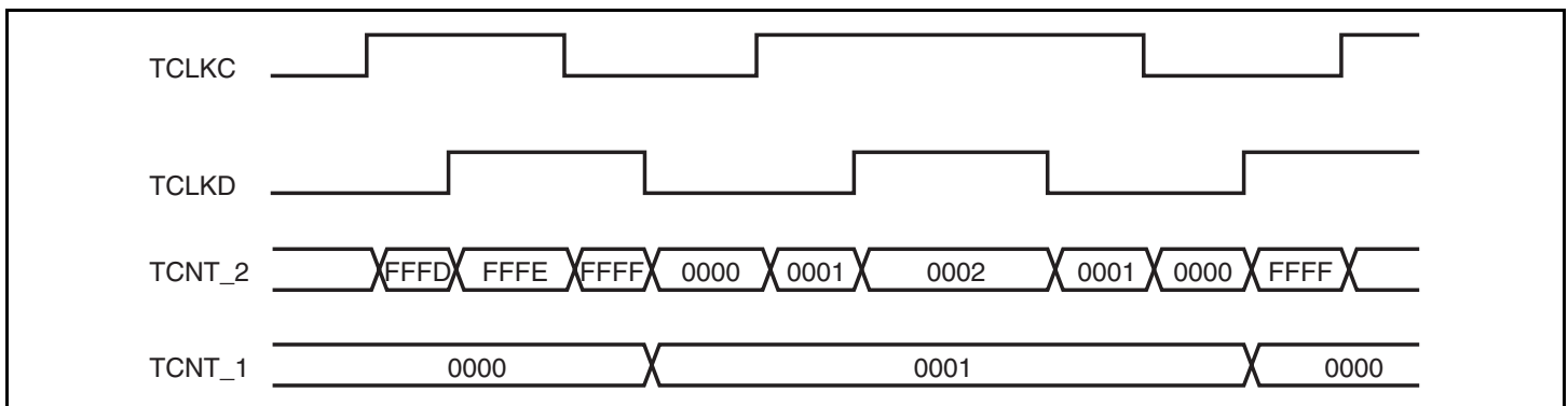
Figure 9.20 Example of Cascaded Operation (2)
