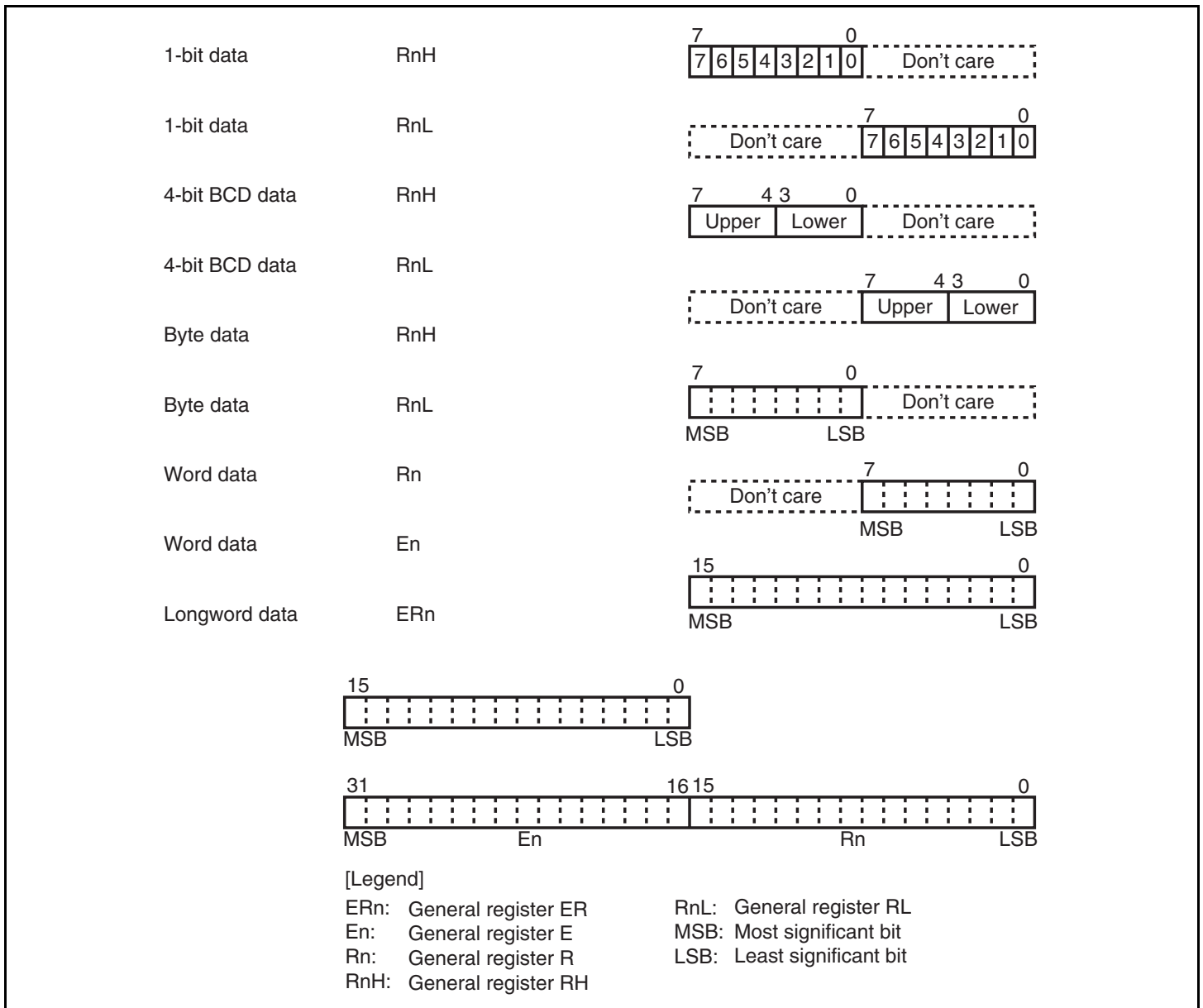
Figure 2.12 General Register Data Formats
