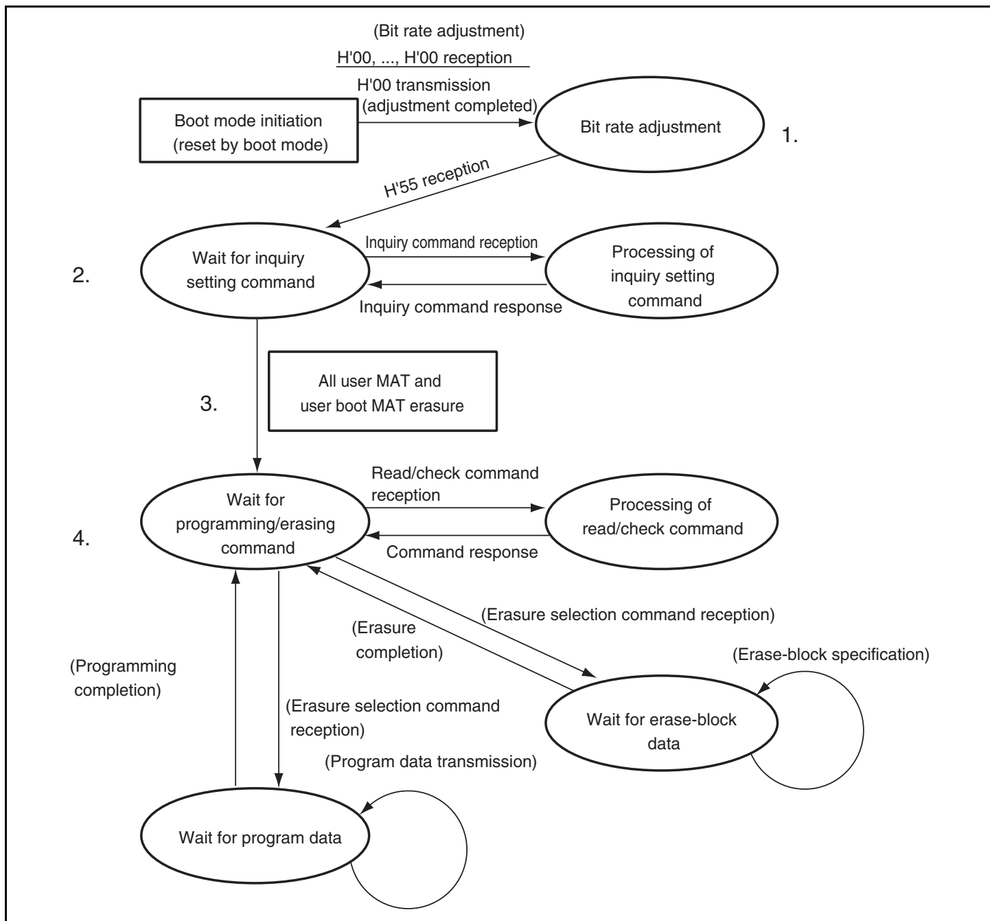
Figure 17.8 Boot Mode State Transition Diagram
