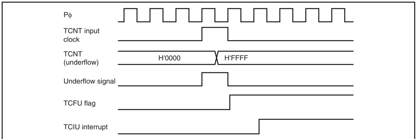
Figure 9.42 TCIU Interrupt Setting Timing
