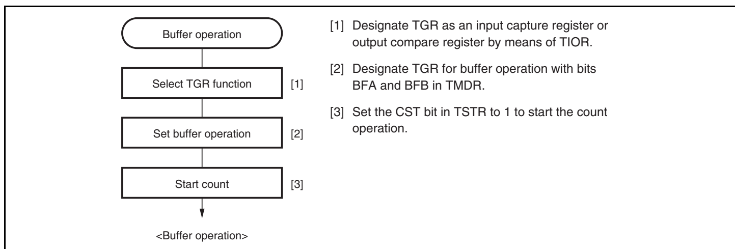
Figure 9.15 Example of Buffer Operation Setting Procedure
