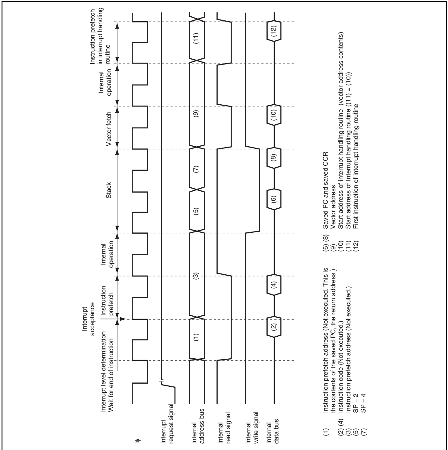
Figure 5.5 Interrupt Exception Handling
