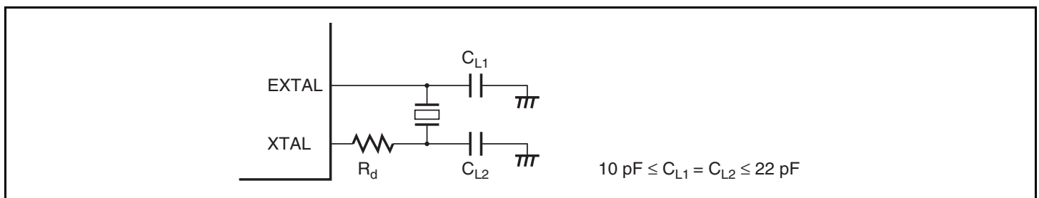
Figure 18.2 Connection of Crystal Resonator (Example)
