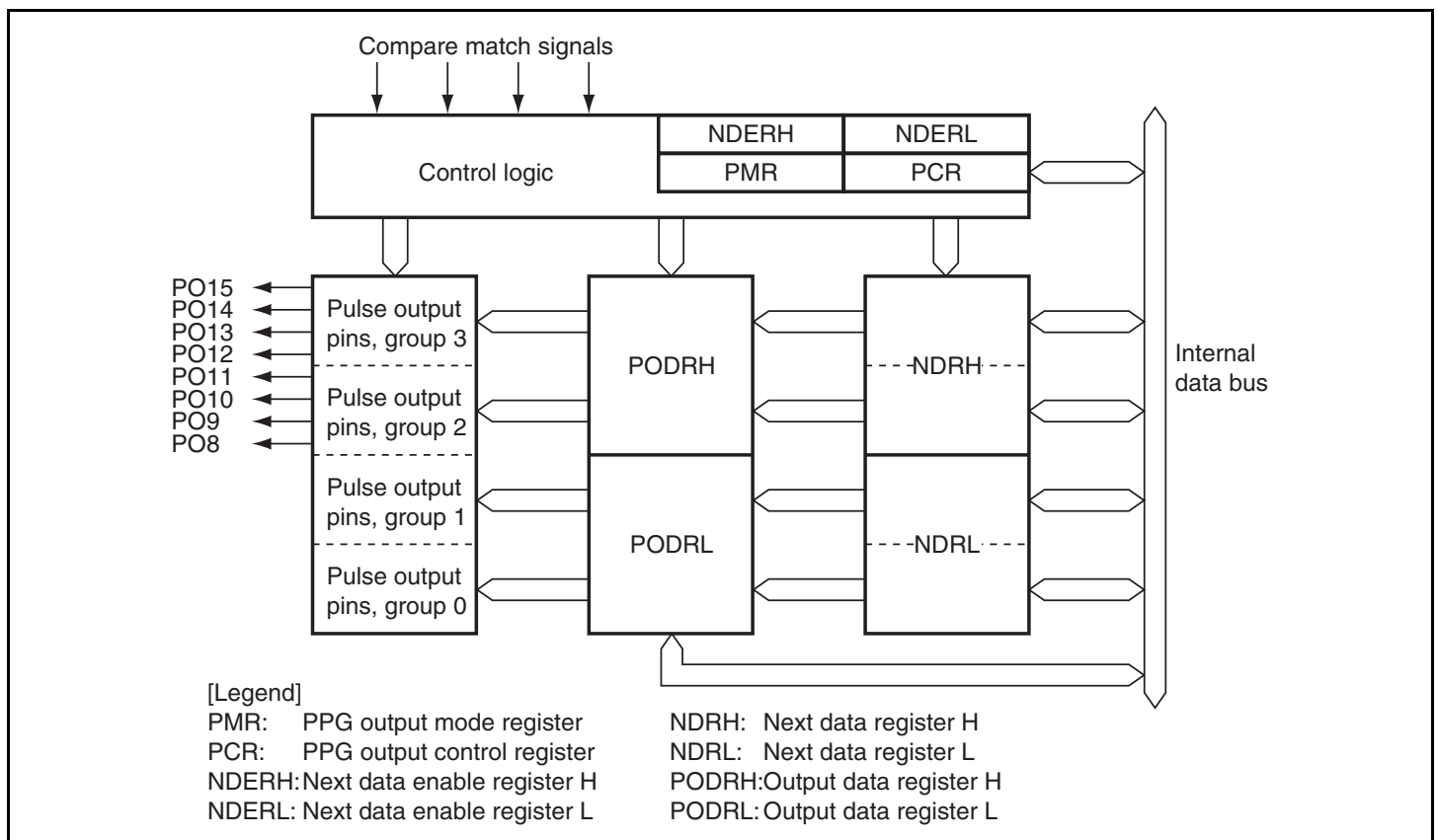
Figure 10.1 Block Diagram of PPG
