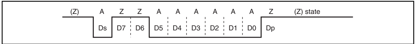
Figure 12.24 Inverse Convention (SDIR = SINV = O/\bar{E} = 1)
