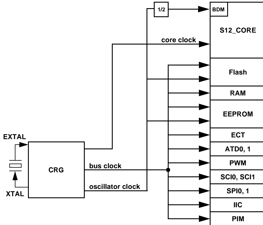
Figure 3-1 Clock Connections
