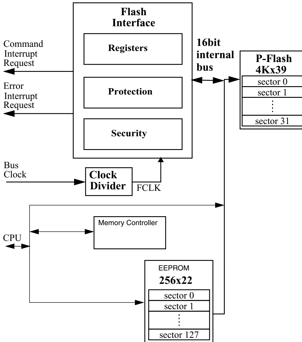
Figure 21-1. FTMRG16K1 Block Diagram
