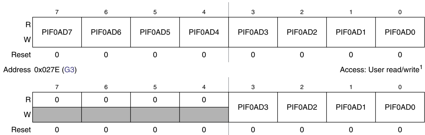
Figure 2-62. Port AD Interrupt Flag Register (PIF0AD)
