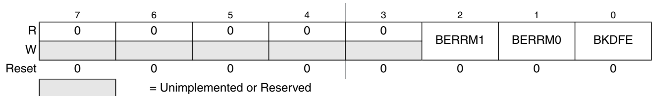
Figure 18-8. SCI Alternative Control Register 2 (SCIACR2)
