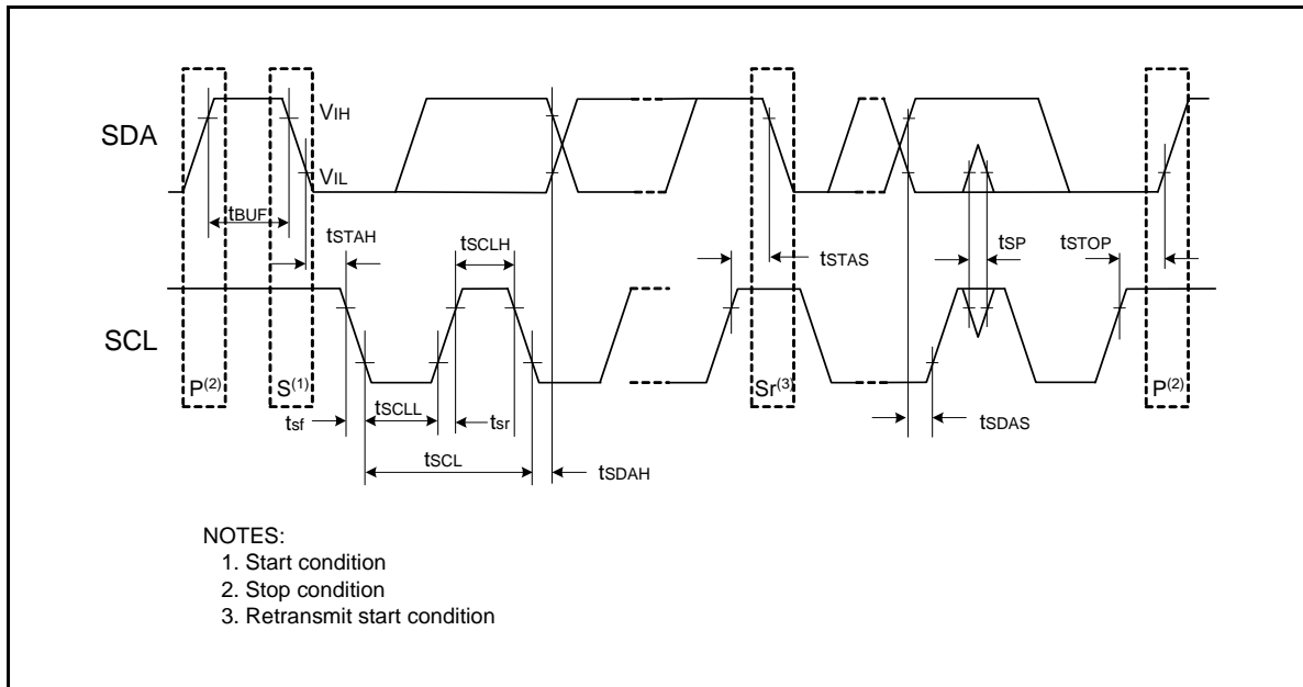
Figure 5.26 I/O Timing of I 2 C bus Interface
