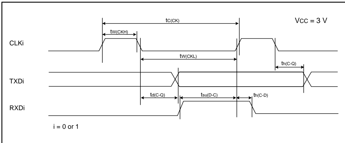
Figure 5.33 Serial Interface Timing Diagram when Vcc = 3 V
