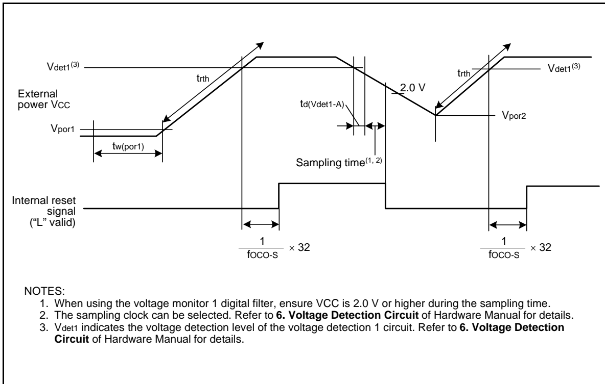
Figure 5.22 Reset Circuit Electrical Characteristics
