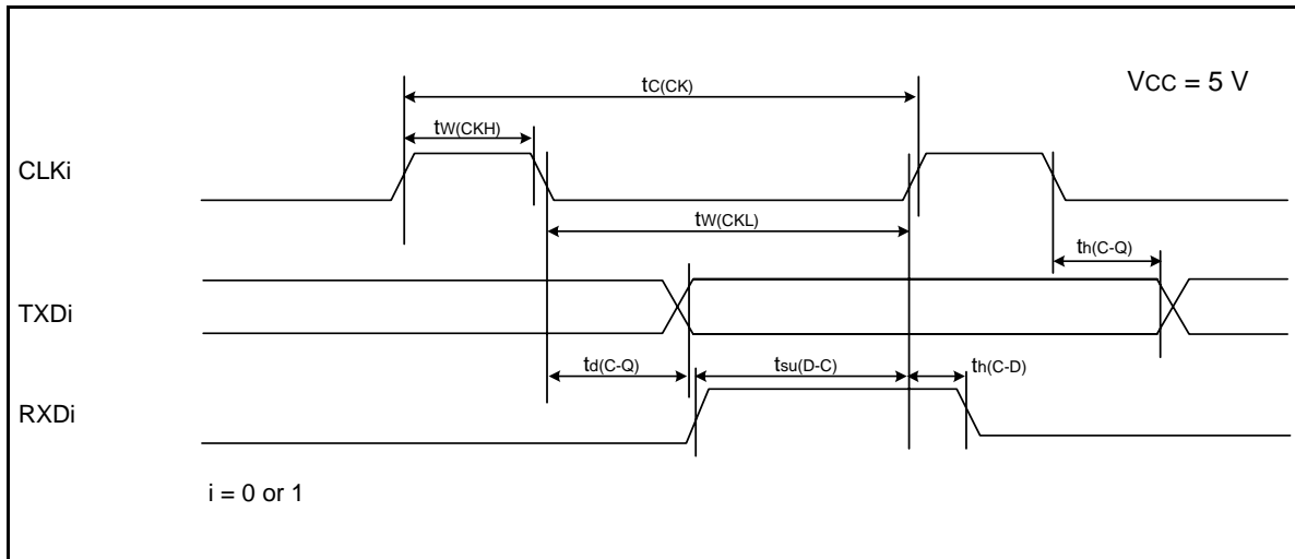
Figure 5.10 Serial Interface Timing Diagram when Vcc = 5 V
