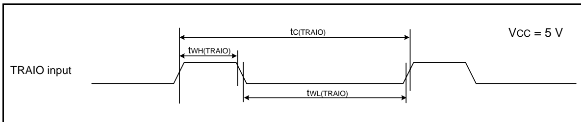
Figure 5.9 TRAI0 Input Timing Diagram when VCC = 5 V
