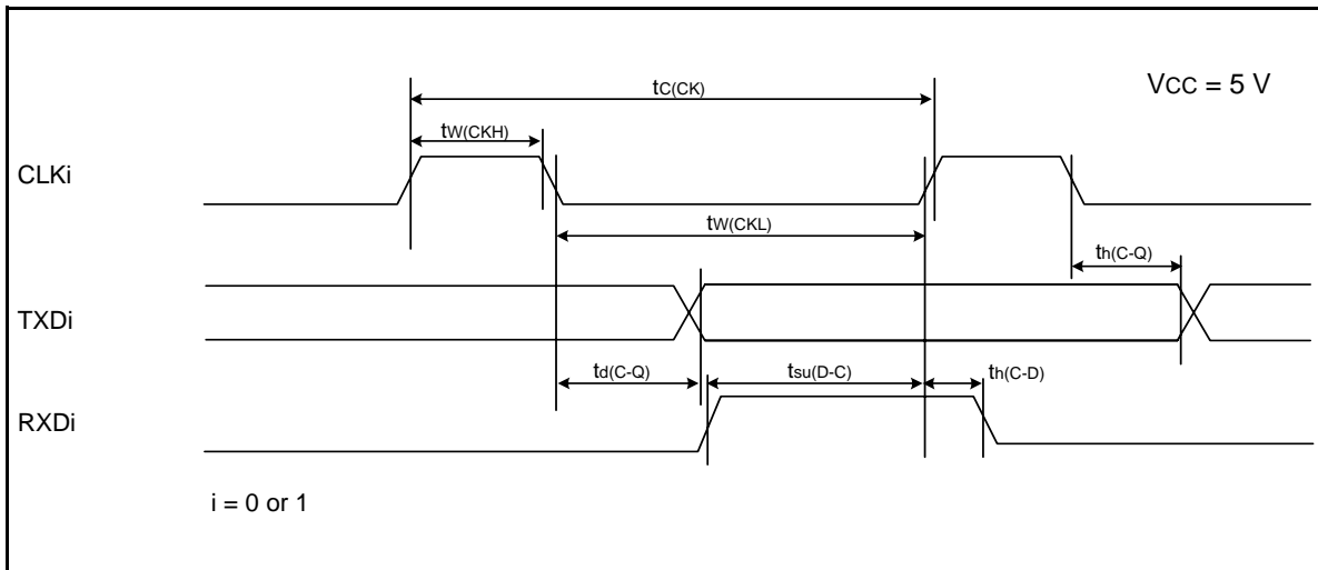
Figure 5.29 Serial Interface Timing Diagram when Vcc = 5 V
