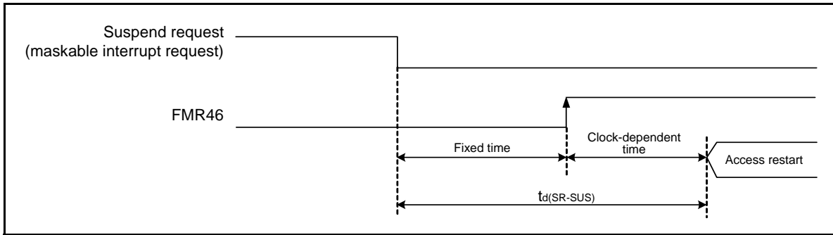
Figure 5.21 Time delay until Suspend
