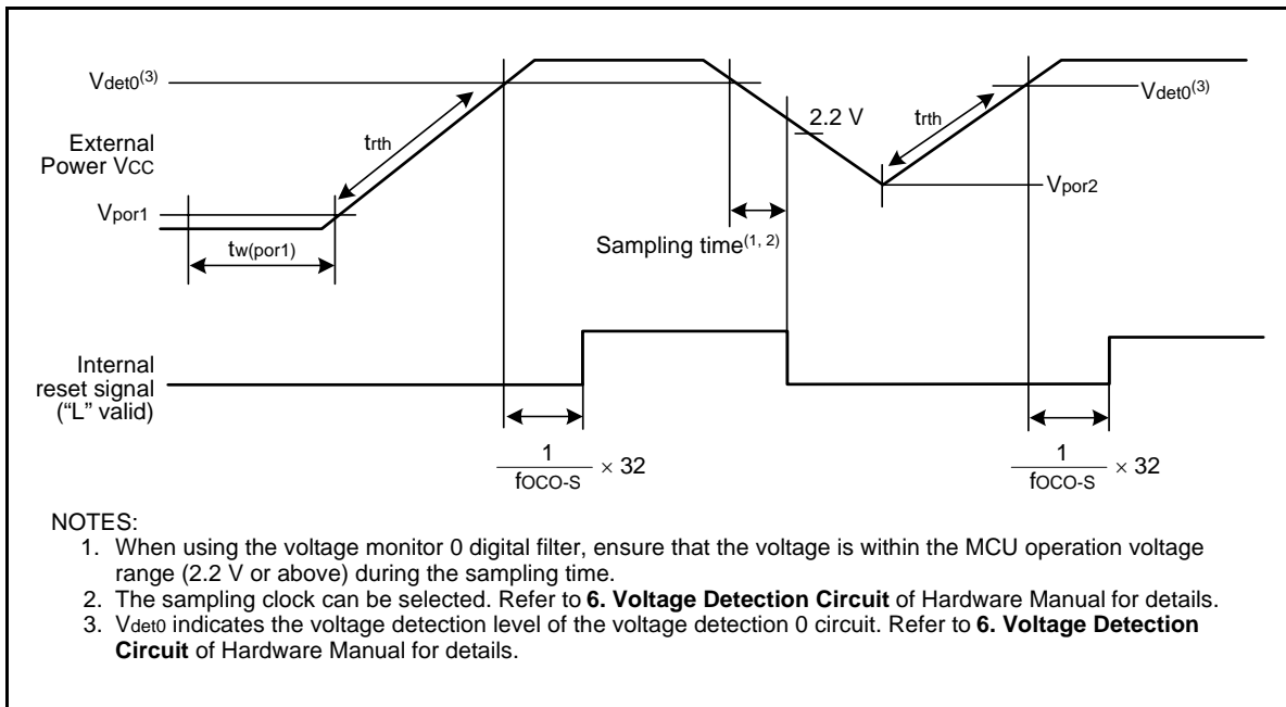
Figure 5.3 Reset Circuit Electrical Characteristics
