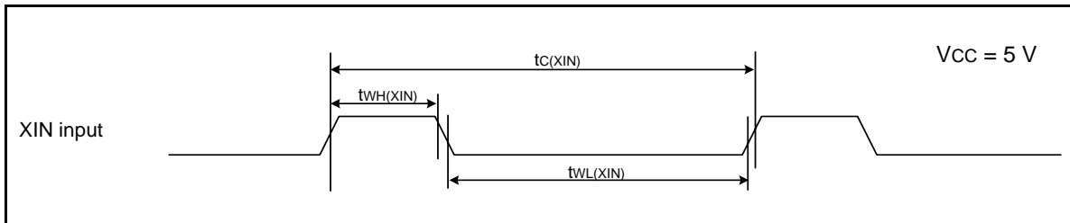
Figure 5.8 XIN Input and XCIN Input Timing Diagram when VCC = 5 V
