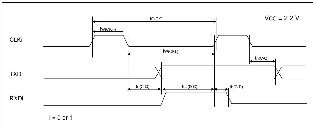
Figure 5.18 Serial Interface Timing Diagram when Vcc = 2.2 V
