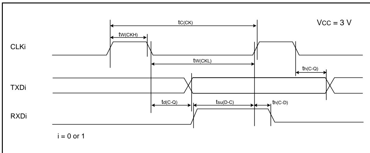
Figure 5.14 Serial Interface Timing Diagram when Vcc = 3 V
