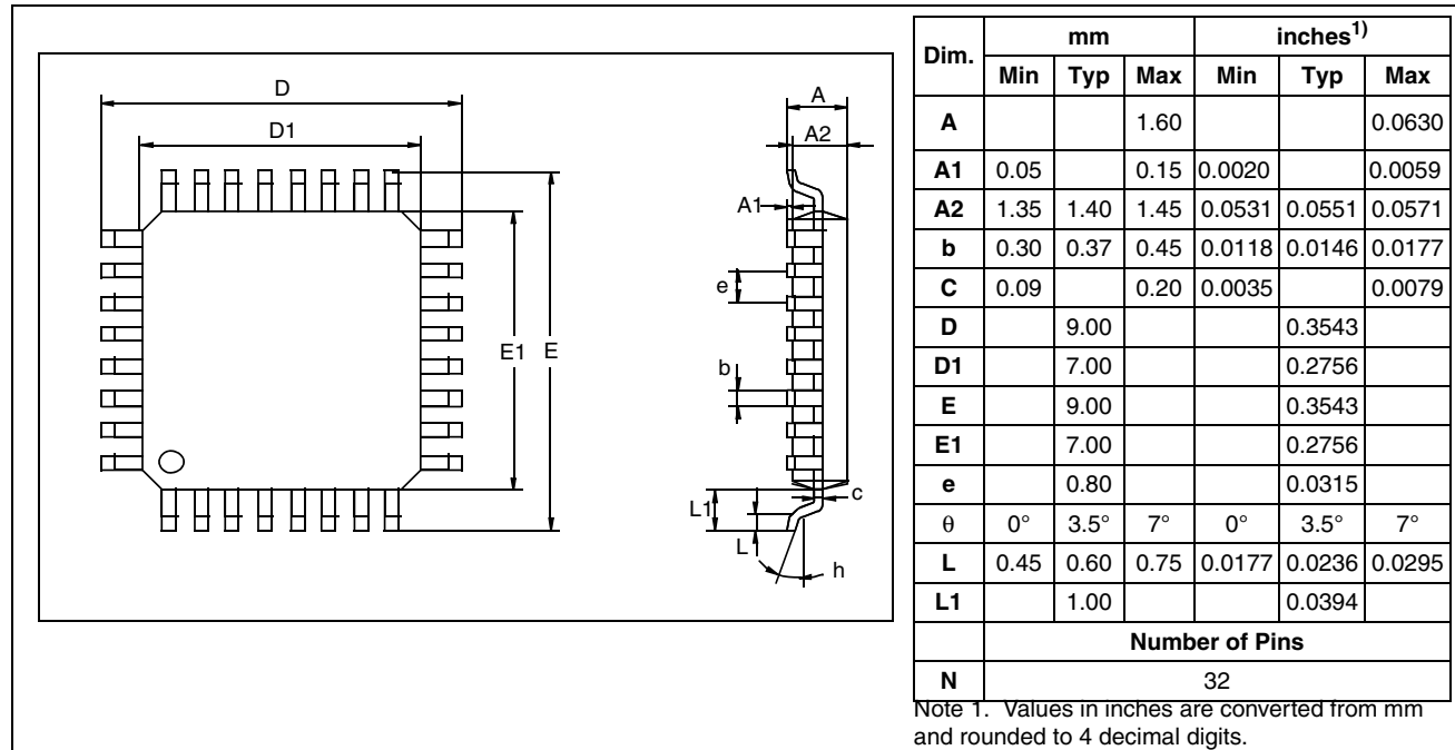
Figure 165. 32-Pin Low Profile Quad Flat Package
