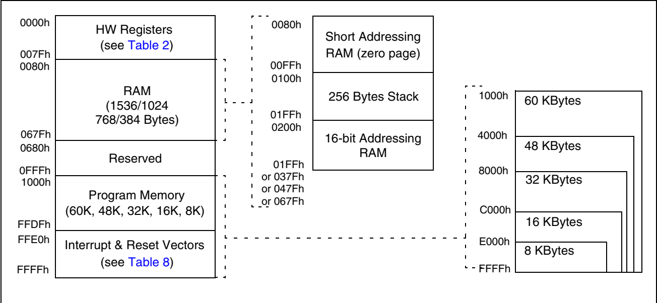
Figure 8. Memory Map
