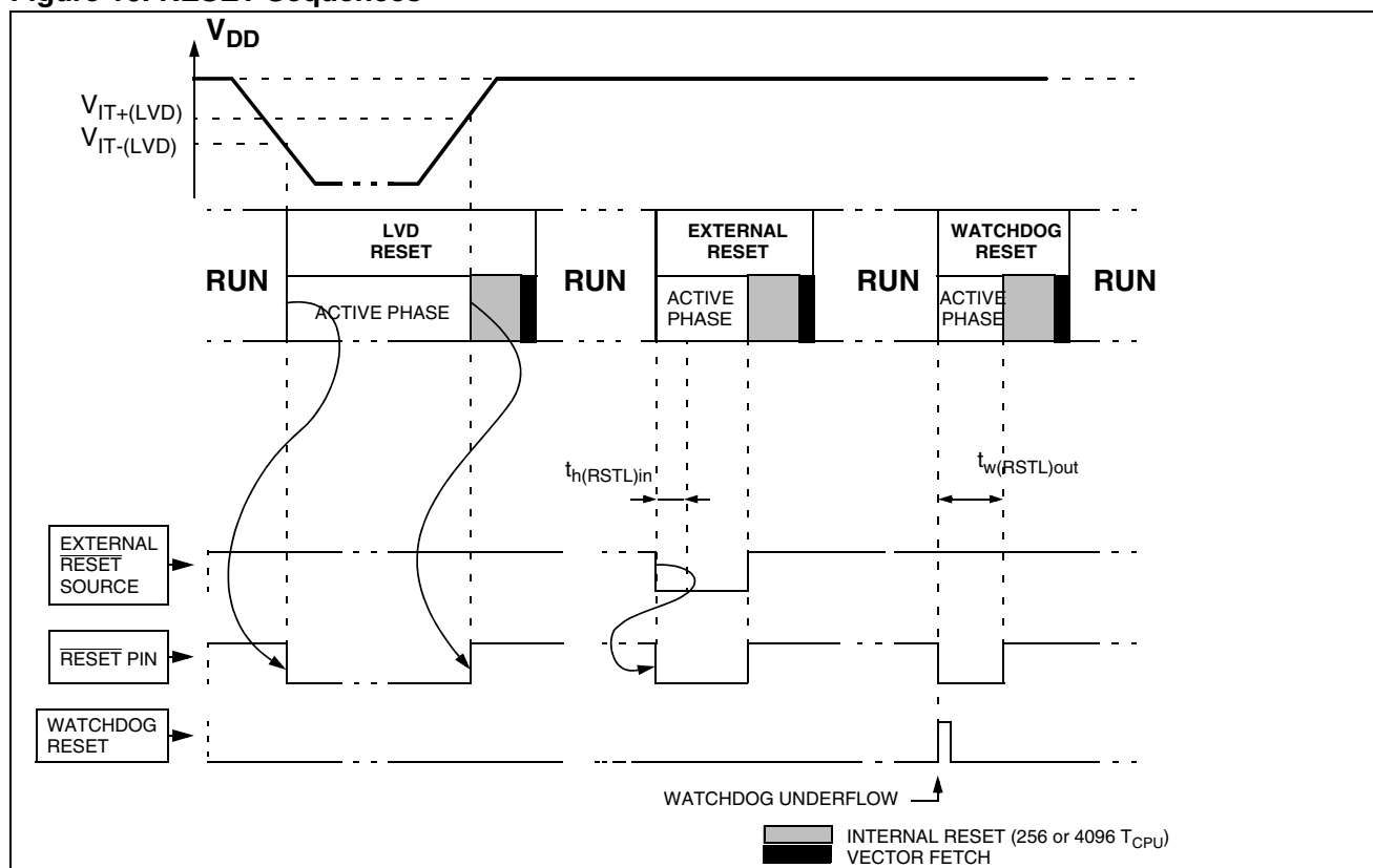
Figure 16. RESET Sequences
