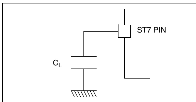
Figure 128. Pin loading conditions
