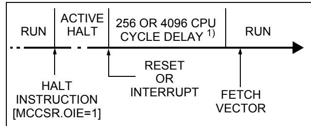
Figure 29. Active-halt Mode Flow-chart
