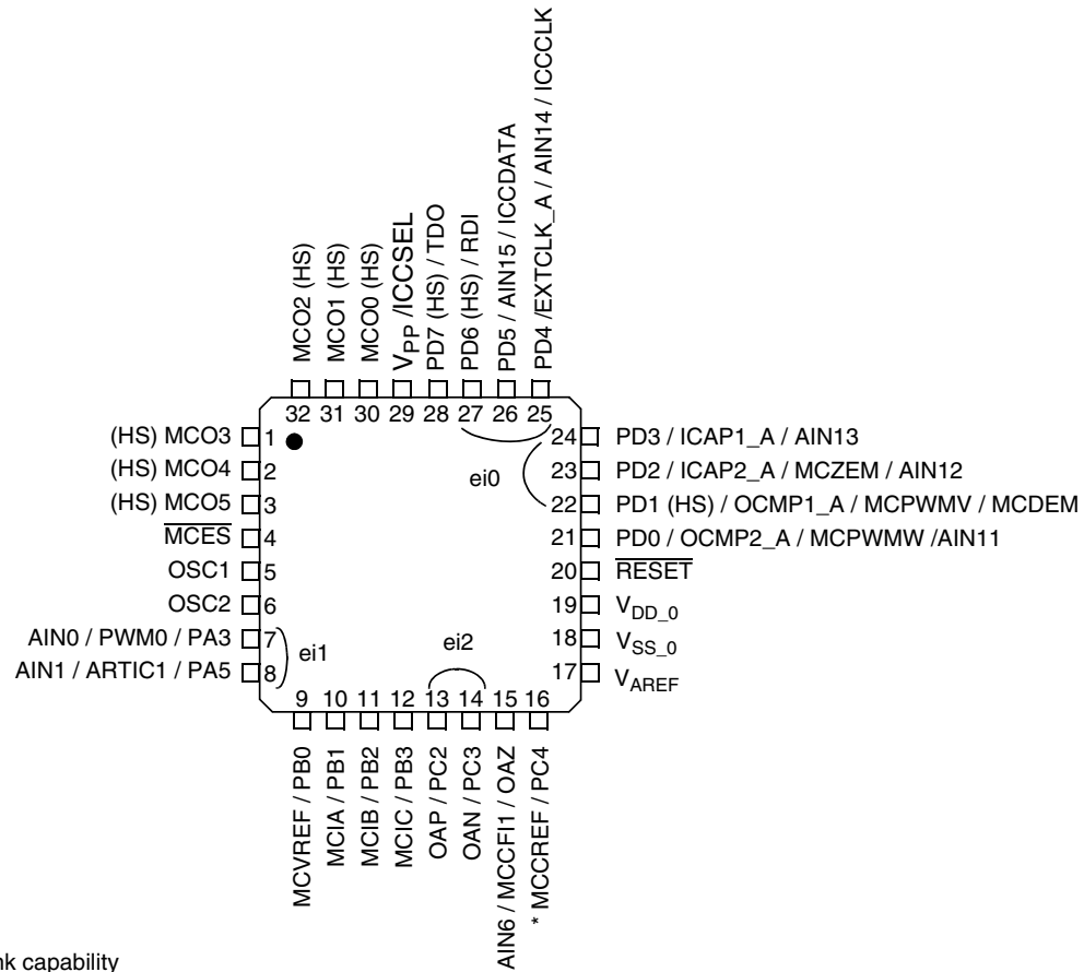
Figure 7. 32-Pin LQFP 7x7 Package Pinout
