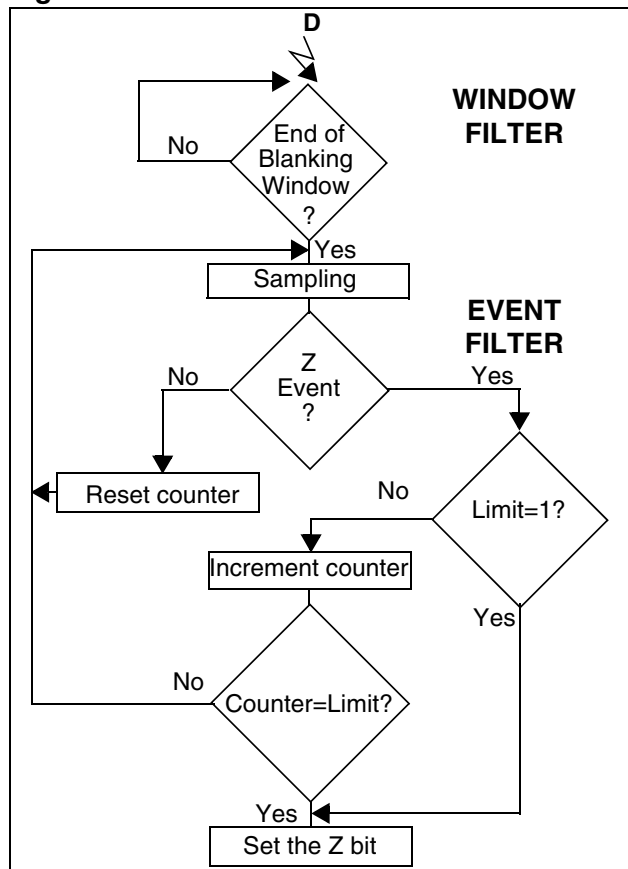
Figure 80. Z Window and Event Filter Flowchart
