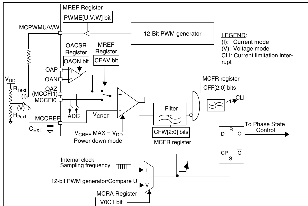
Figure 106. Current Feedback
