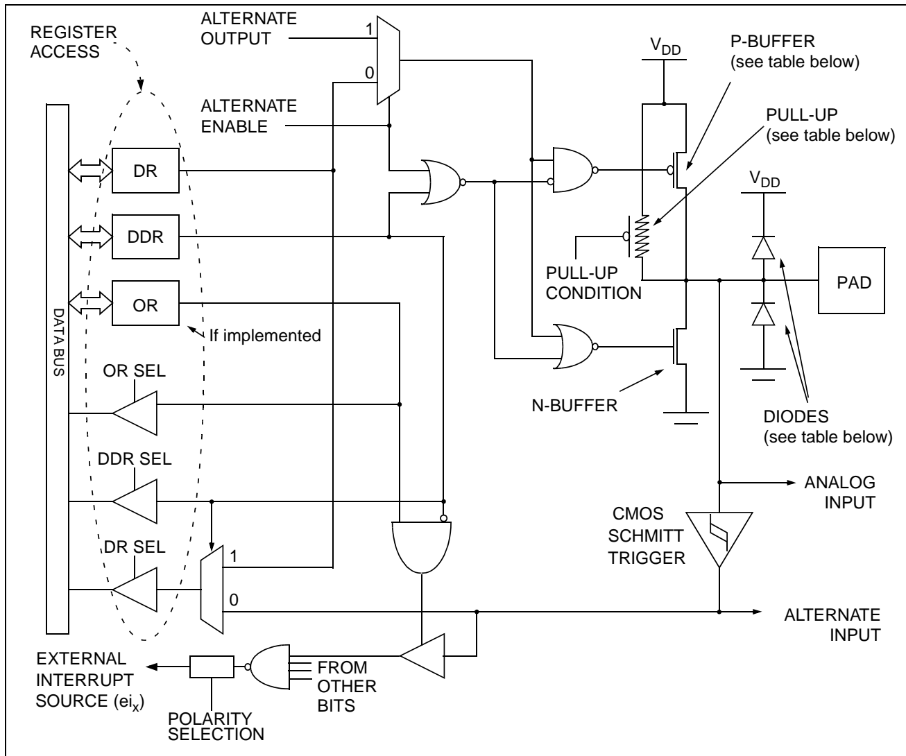
Figure 32. I/O Port General Block Diagram
