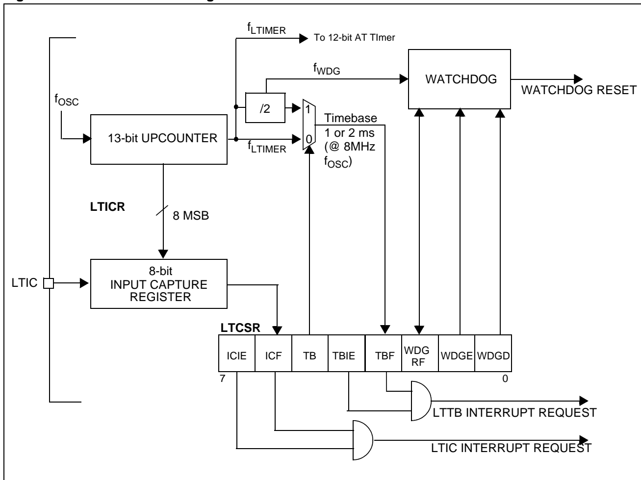
Figure 34. Lite Timer Block Diagram
