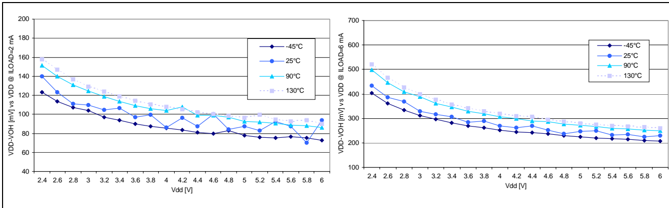
Figure 65. Typical V_{DD}-V_{OH} vs. V_{DD} (HS pins)
