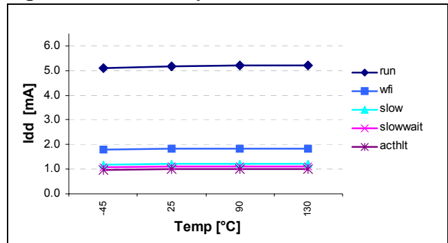
Figure 50. I_{DD} vs temp @Vdd 5V & int RC=4MHz
