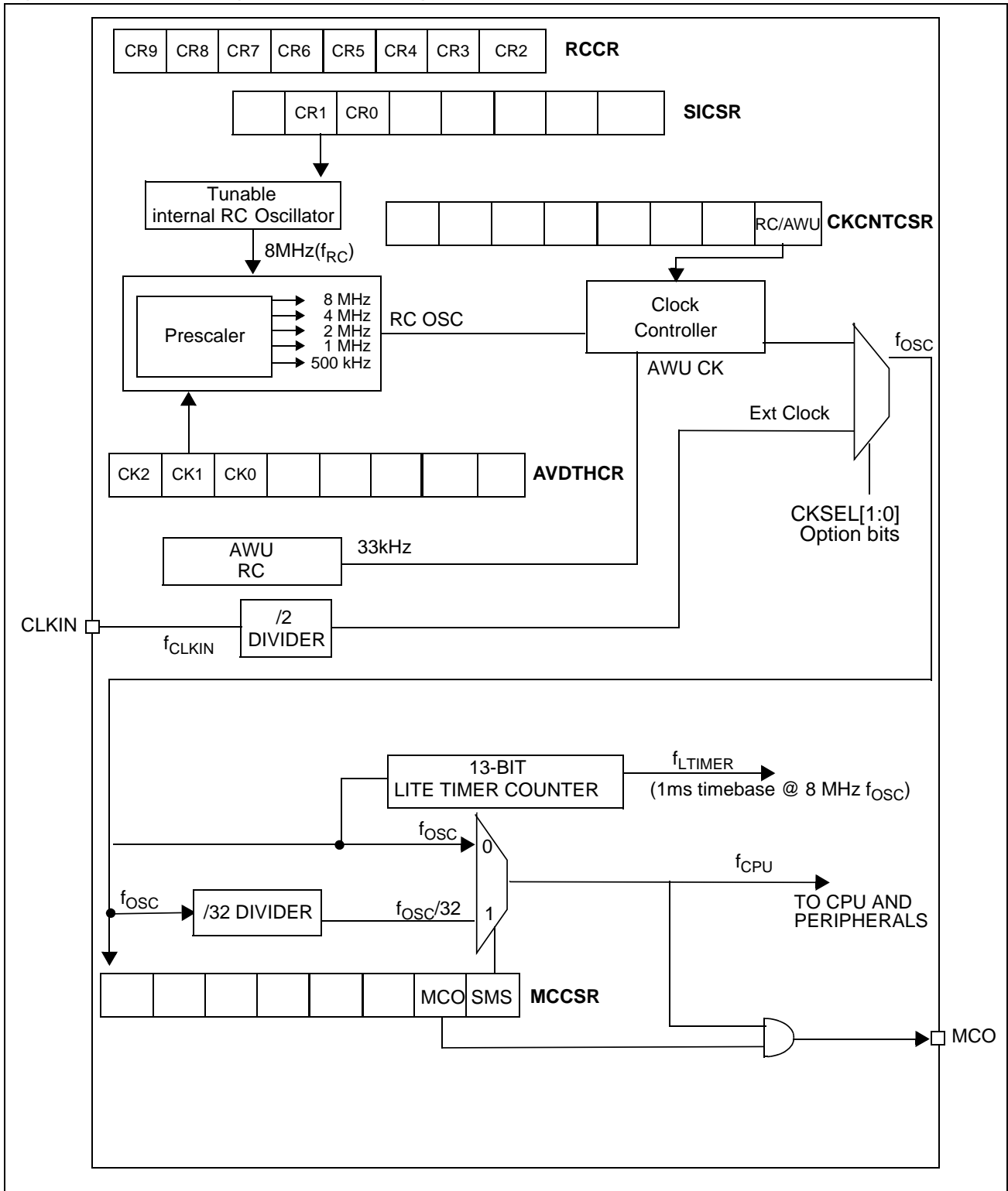
Figure 14. Clock Management Block Diagram
