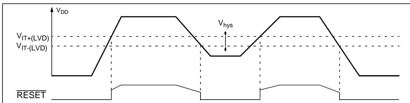
Figure 19. Low Voltage Detector vs Reset
