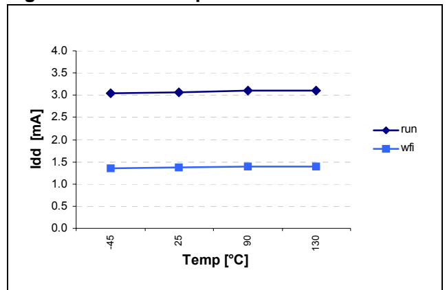
Figure 51. I_{DD} vs temp @Vdd 5V & int RC=2MHz
