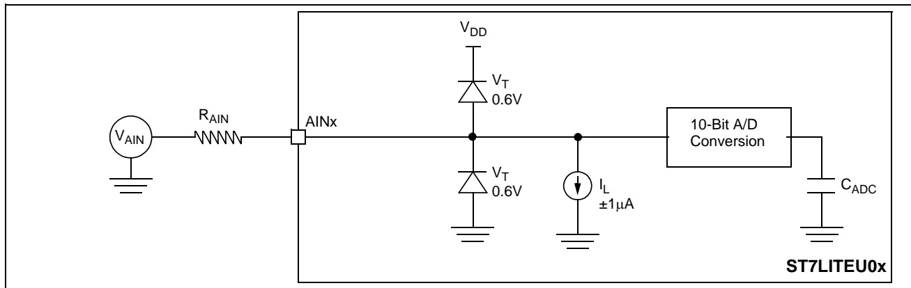
Figure 68. Typical Application with ADC
