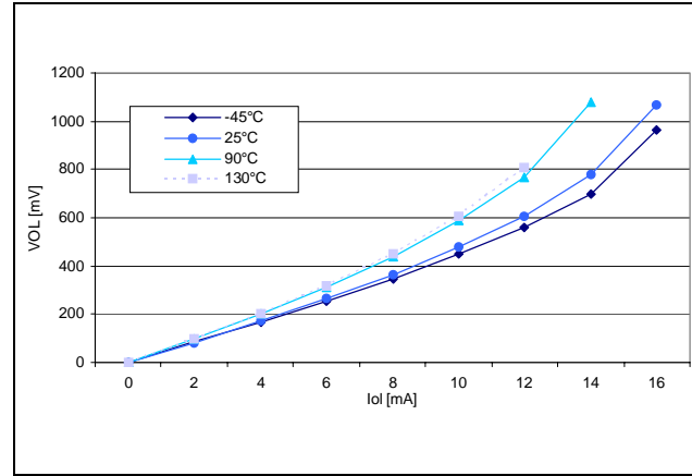
Figure 58. Typical V_{OL} at V_{DD} = 2.4V (HS pins)
