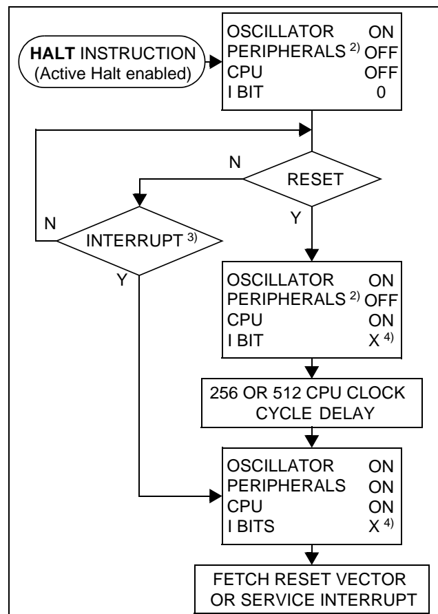
Figure 26. ACTIVE-HALT Mode Flow-chart
