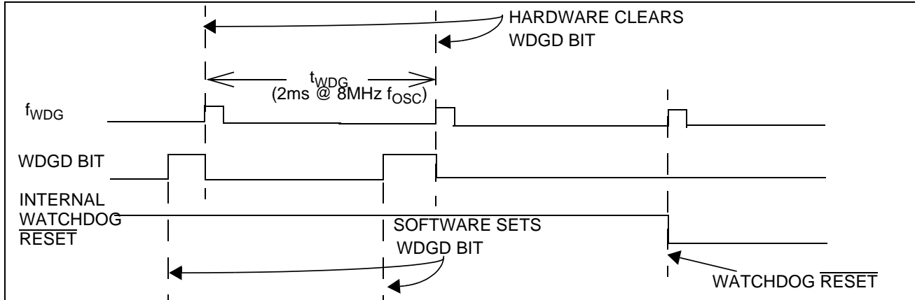
Figure 35. Watchdog Timing Diagram
