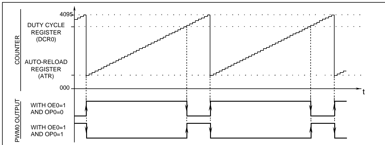
Figure 38. PWM Function
