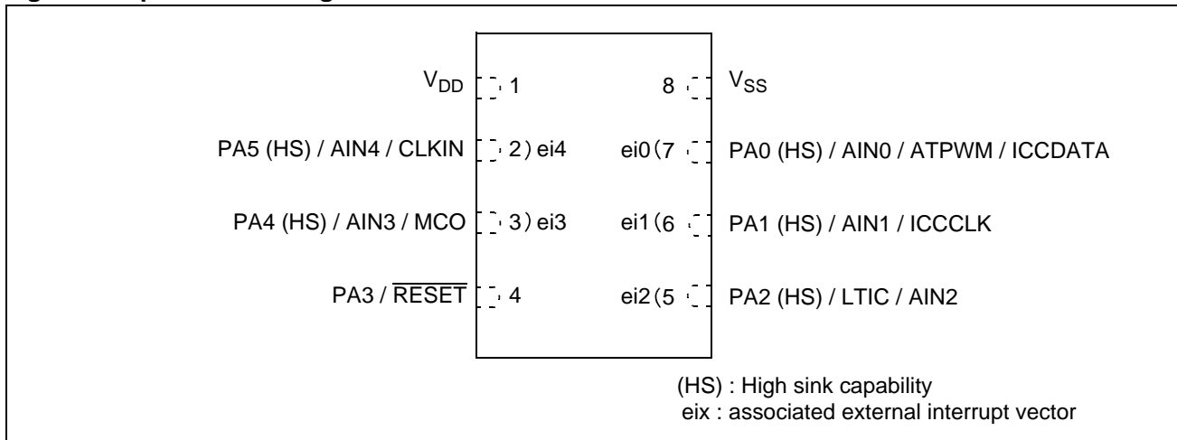
Figure 3. 8-pin DFN Package Pinout
