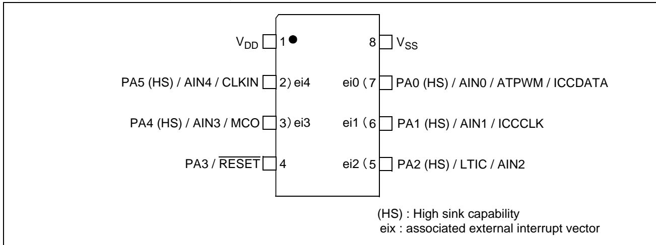
Figure 2. 8-pin SO and DIP Package Pinout
