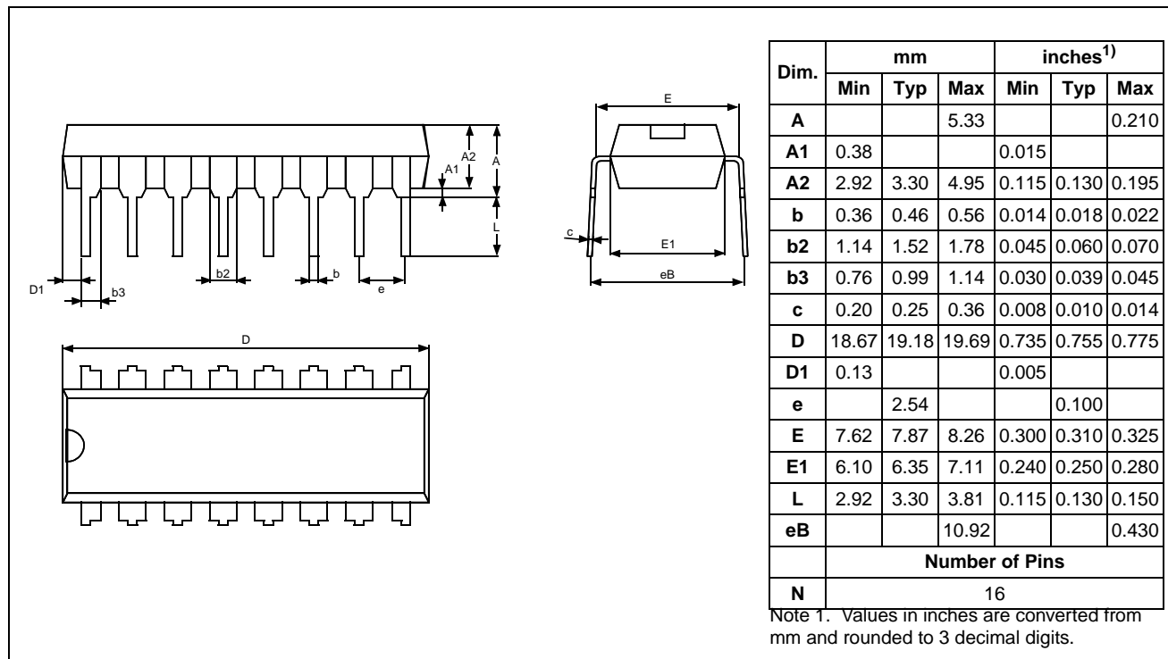
Figure 73. 16-Pin Plastic Dual In-Line Package, 300-mil Width
