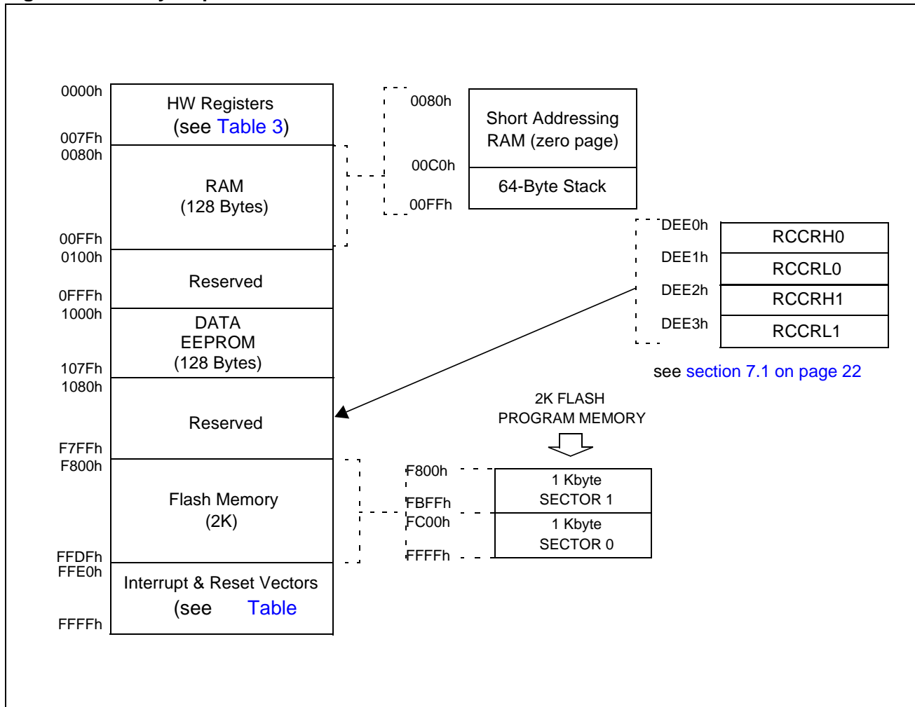
Figure 5. Memory Map
