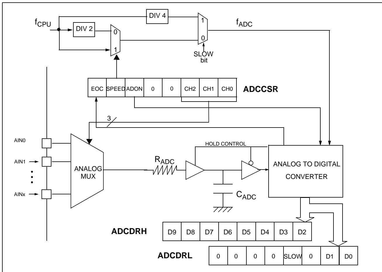
Figure 40. ADC Block Diagram
