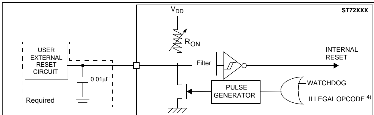
Figure 67. \overline{\text{RESET}} pin protection when LVD is disabled. 1)
