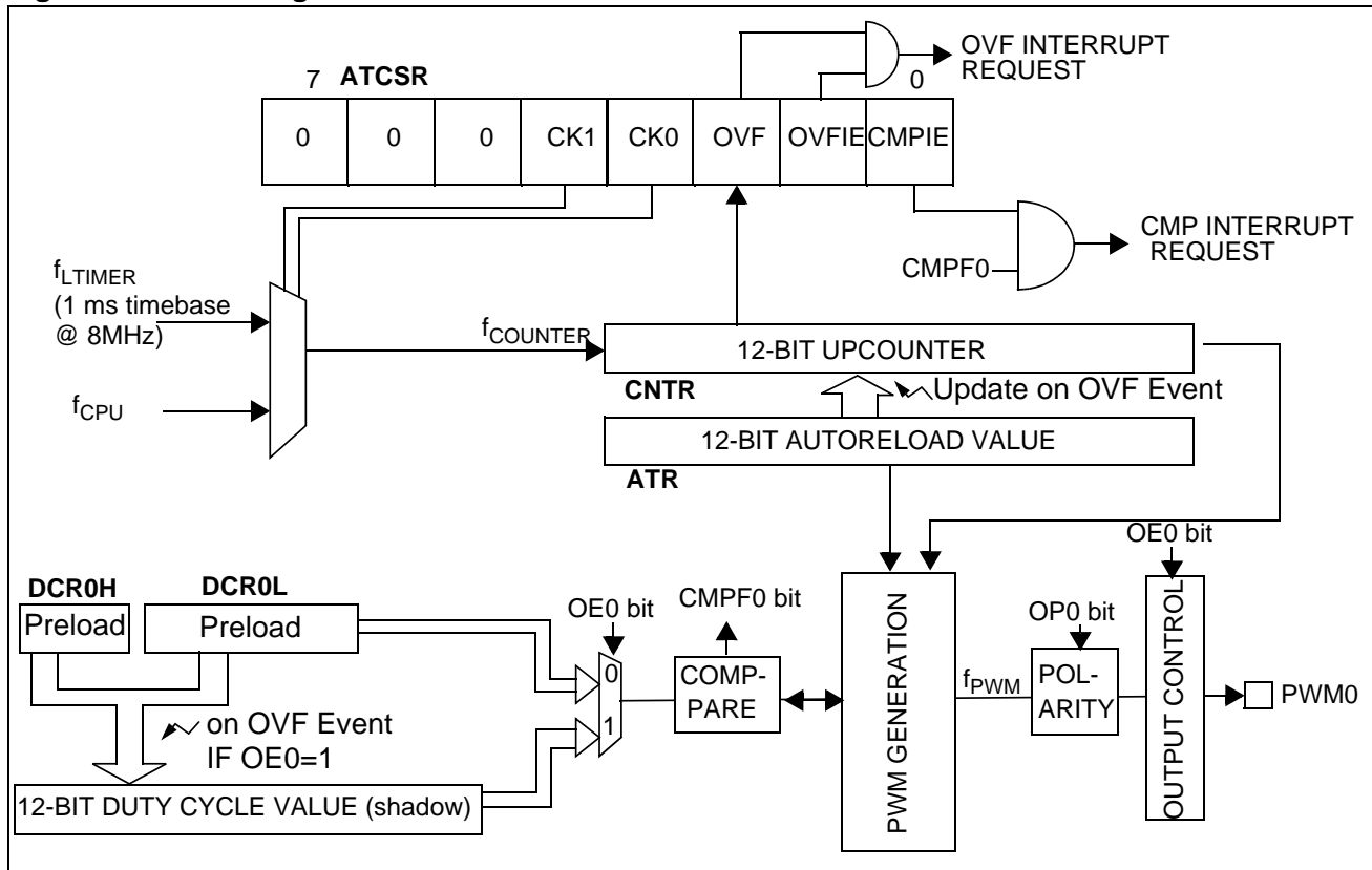
Figure 37. Block Diagram
