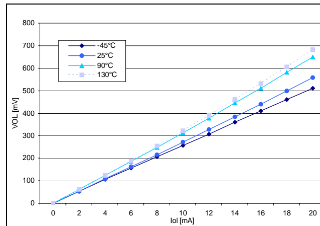
Figure 60. Typical V_{OL} at V_{DD} = 5V (HS pins)
