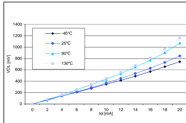
Figure 59. Typical V_{OL} at V_{DD} = 3V (HS pins)
