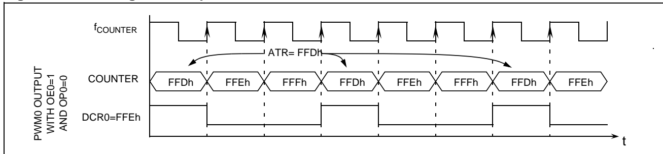
Figure 39. PWM Signal Example
