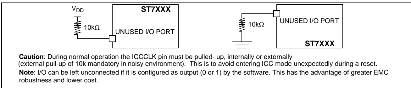
Figure 52. Two typical Applications with unused I/O Pin
