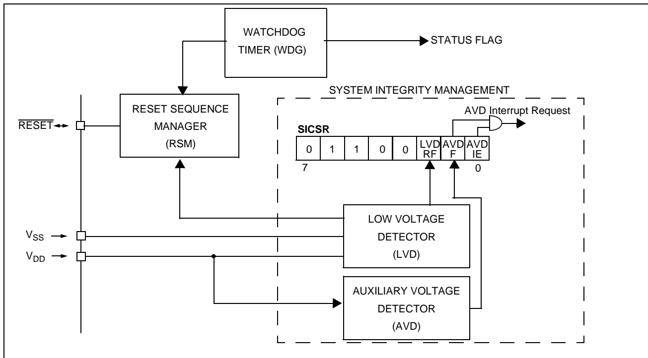
Figure 20. Reset and Supply Management Block Diagram
