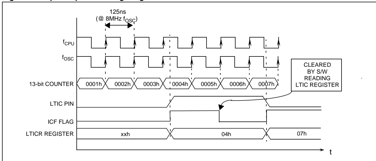
Figure 36. Input Capture Timing Diagram
