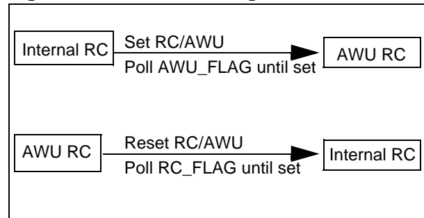
Figure 13. Clock Switching
