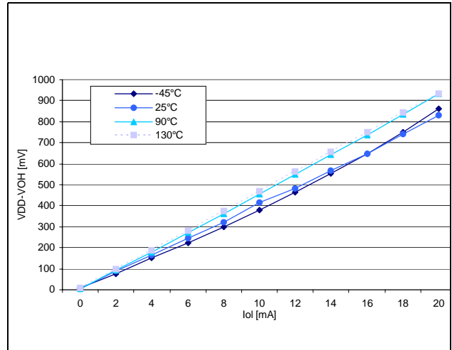
Figure 63. Typical V_{DD}-V_{OH} at V_{DD} = 5V (HS pins)
