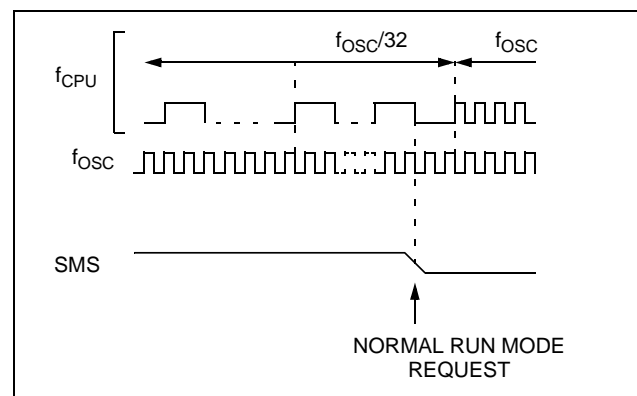
Figure 23. SLOW Mode Clock Transition
