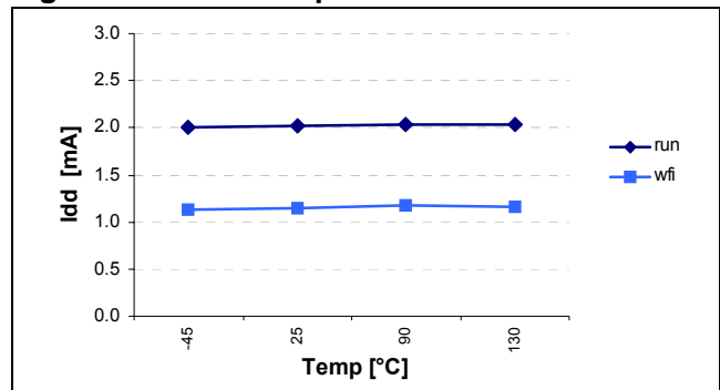
Figure 51. I_{DD} vs temp @Vdd 5V & int RC=2MHz
