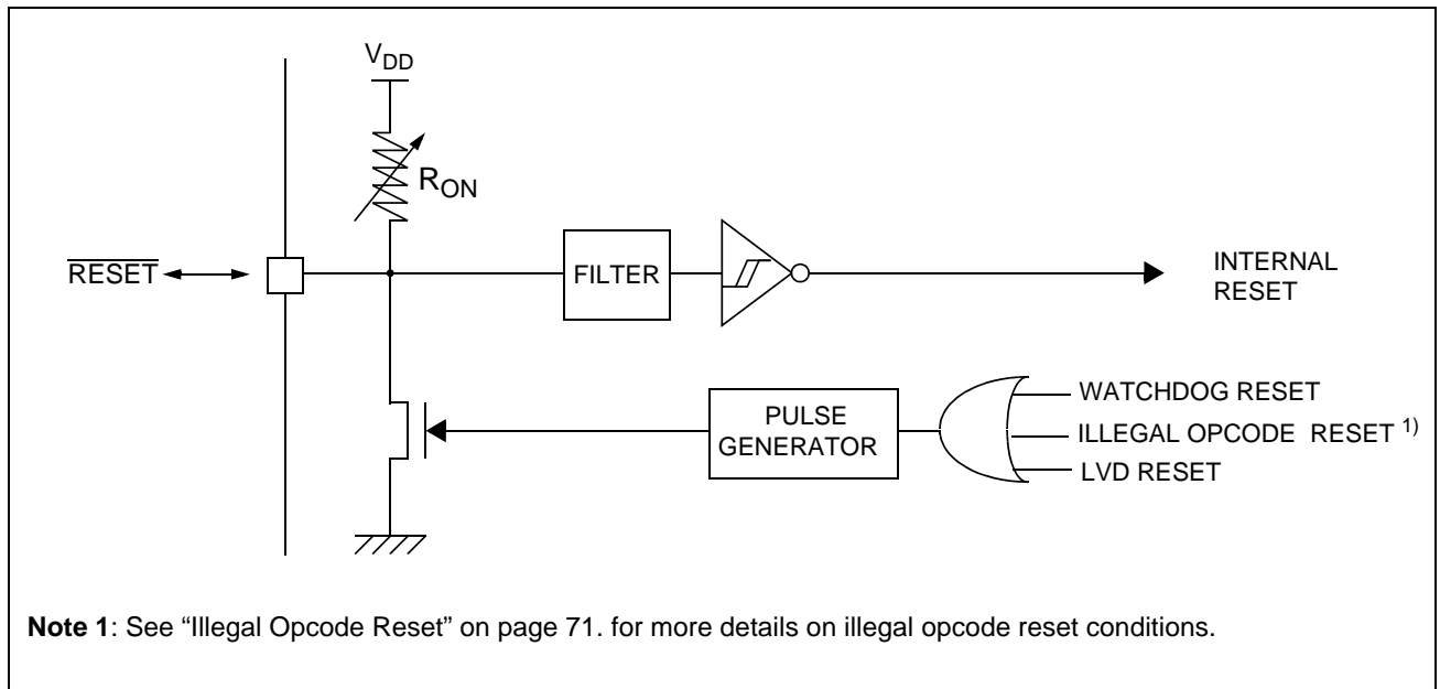
Figure 16. Reset Block Diagram
