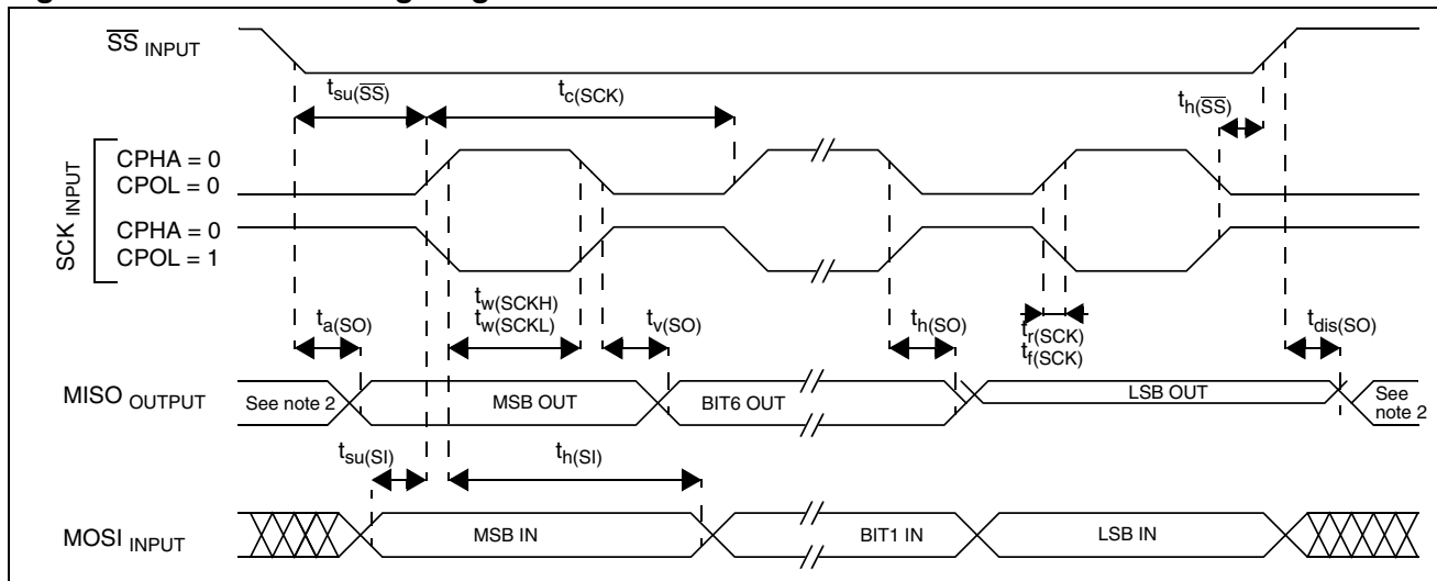
Figure 96. SPI Slave Timing Diagram with CPHA = 0^3)
