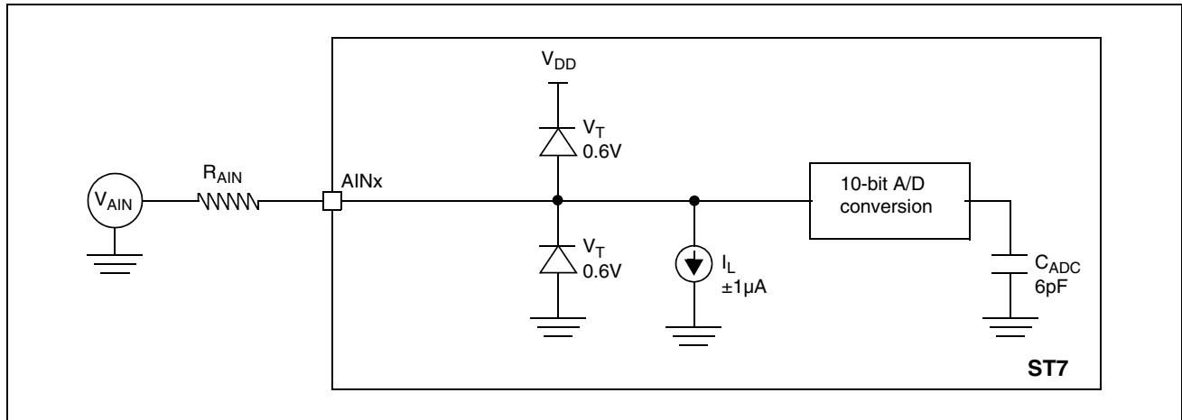
Figure 99. Typical Application with ADC
