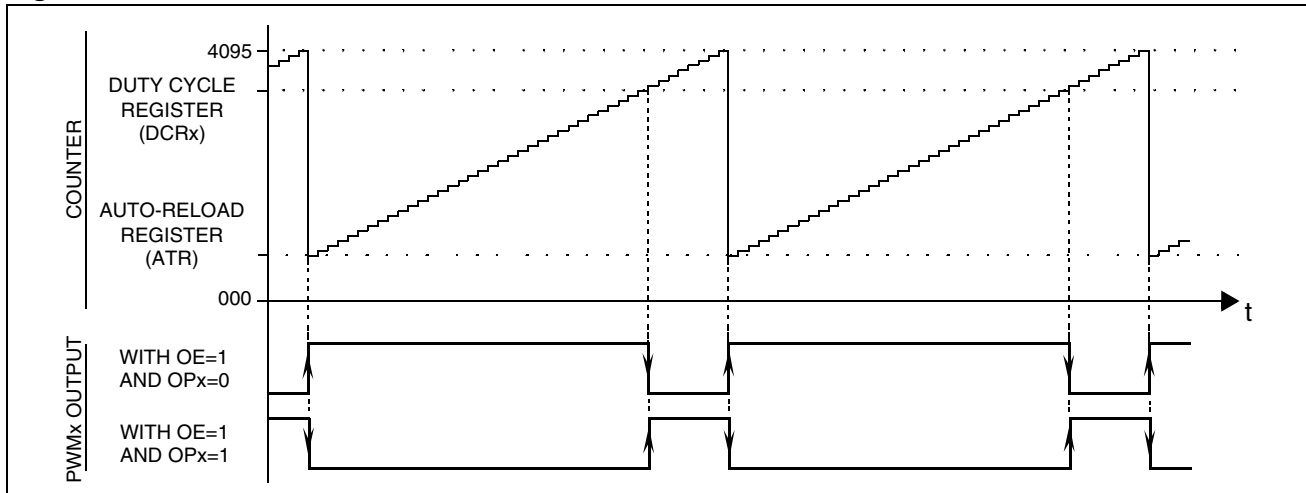
Figure 35. PWM Function
