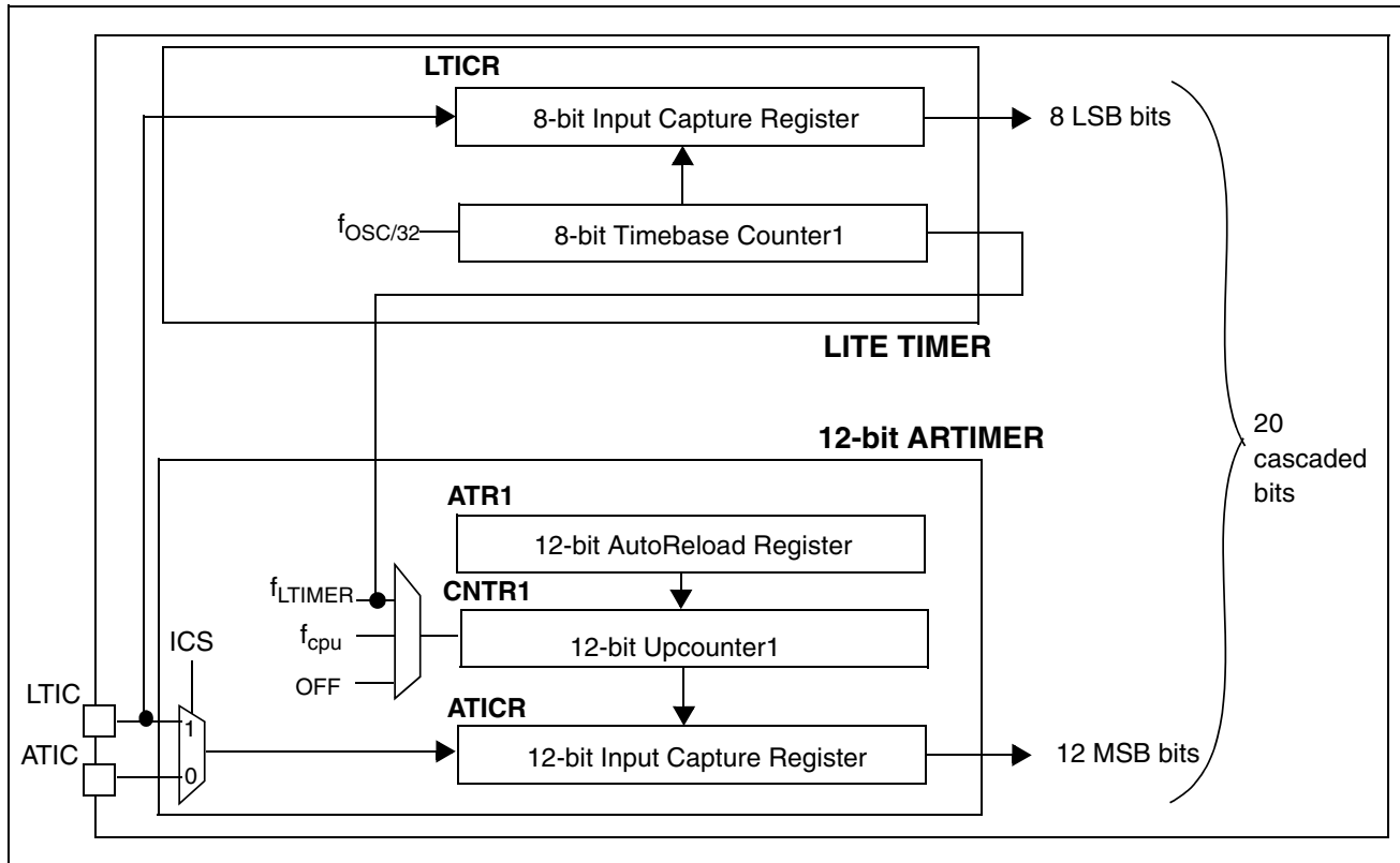
Figure 42. Long Range Input Capture Block Diagram
