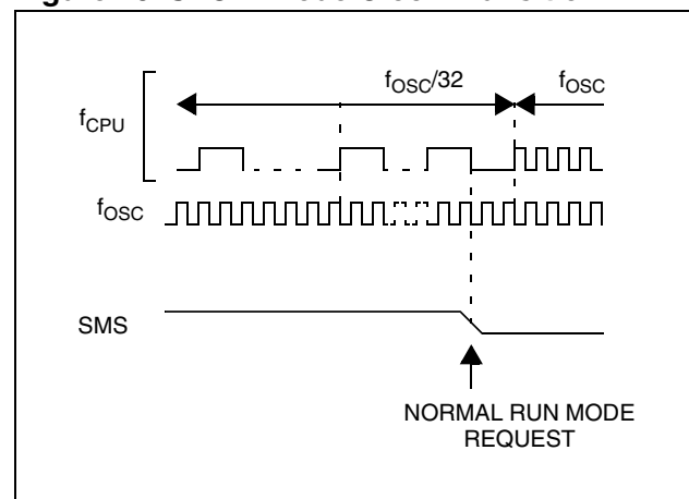
Figure 20. SLOW Mode Clock Transition
