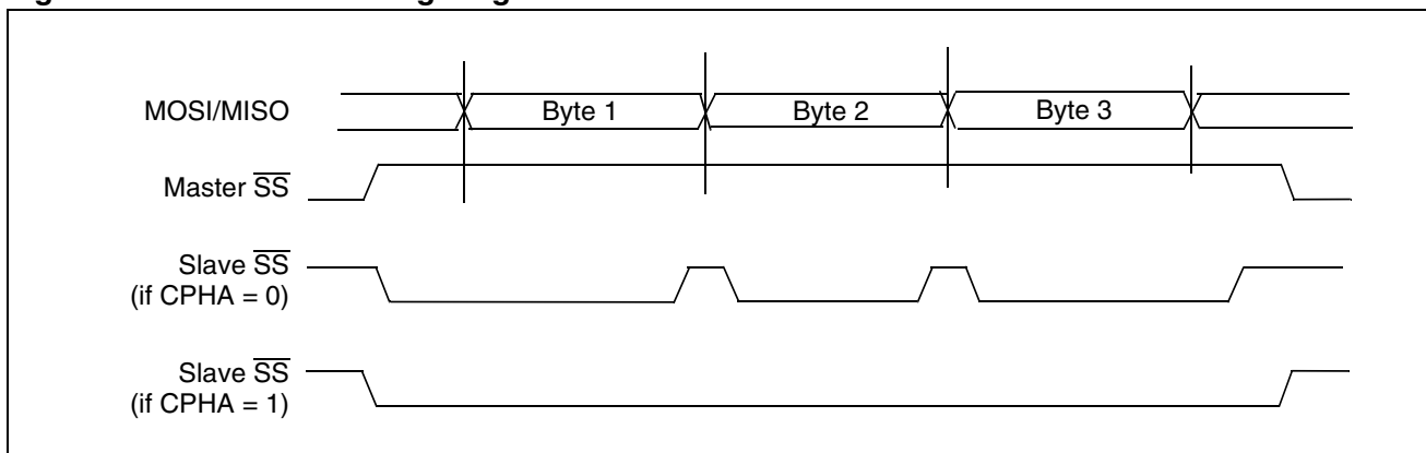
Figure 52. Generic \overline{SS} Timing Diagram
