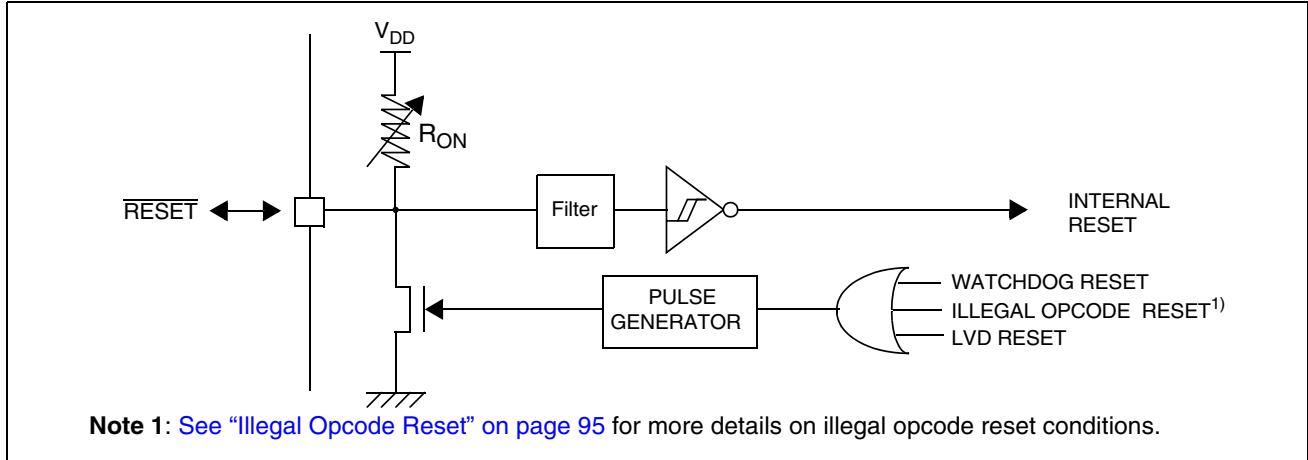
Figure 14. Reset Block Diagram
