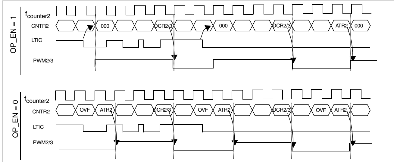
Figure 45. One Pulse Mode Timing Diagram
