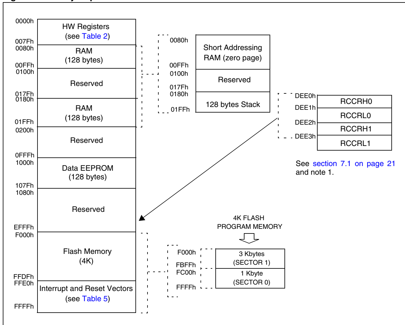
Figure 3. Memory Map
