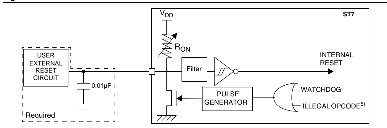
Figure 95. \overline{\text{RESET}} Pin Protection When LVD Is Disabled 1)
