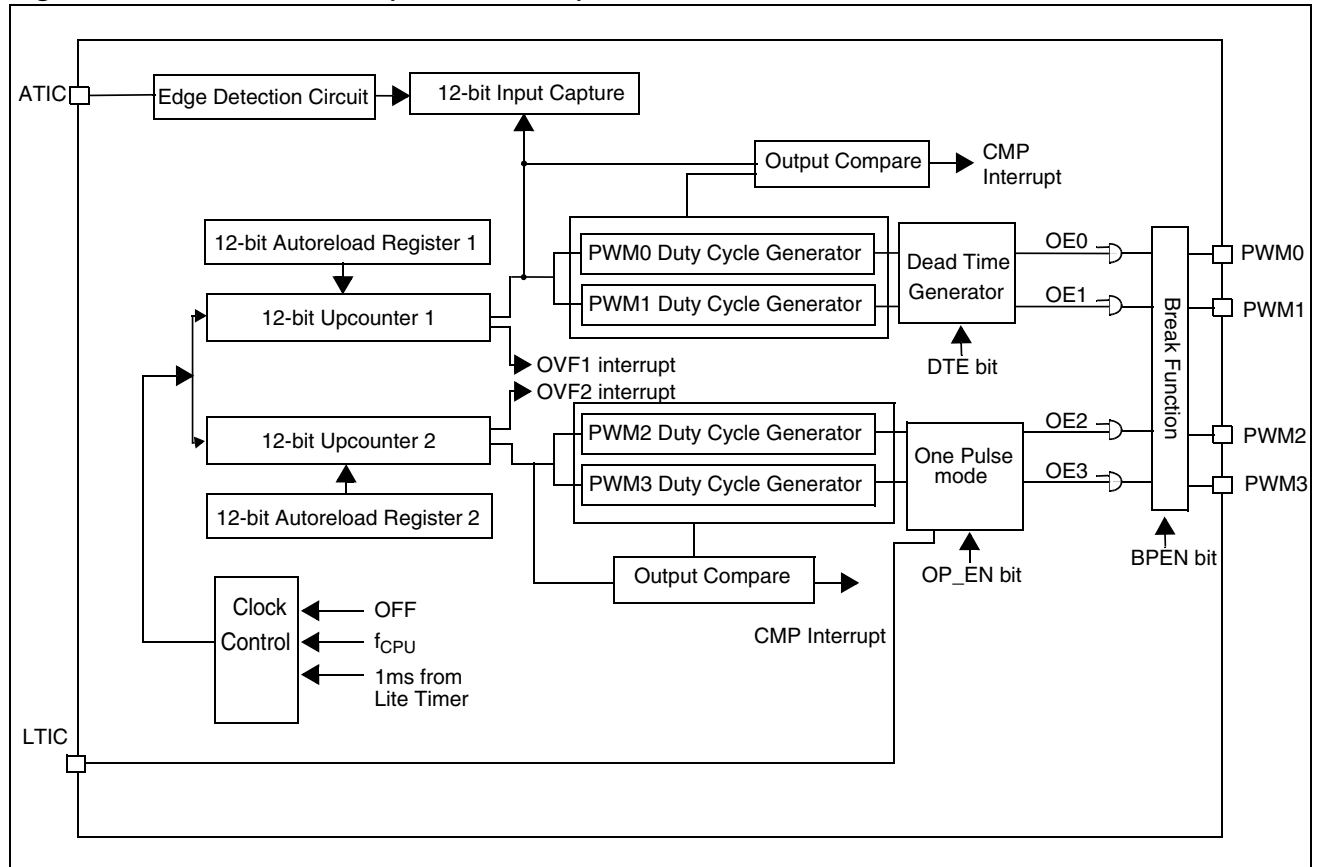
Figure 33. Dual Timer Mode (ENCNTR2 = 1)
