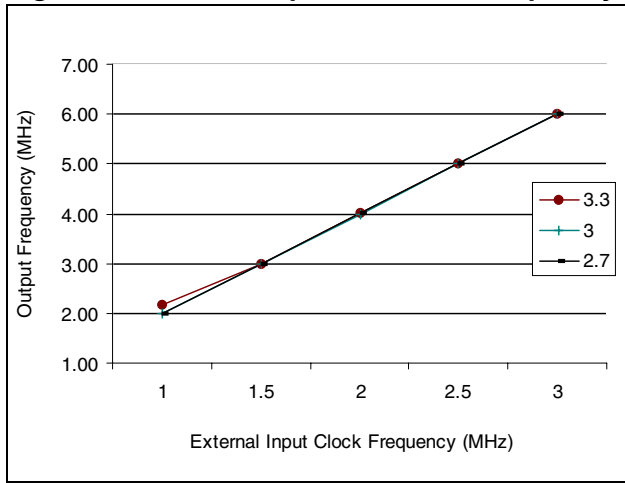
Figure 65. PLLx4 Output vs CLKIN Frequency
