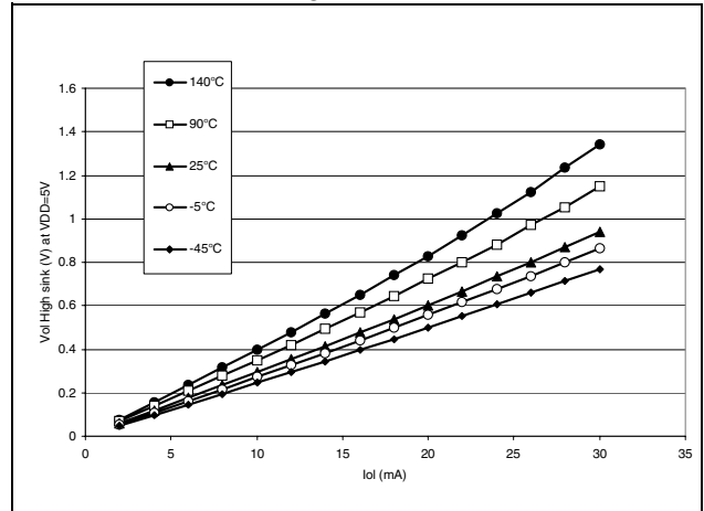
Figure 81. Typical V_{OL} at V_{DD} = 5V (High-sink)
