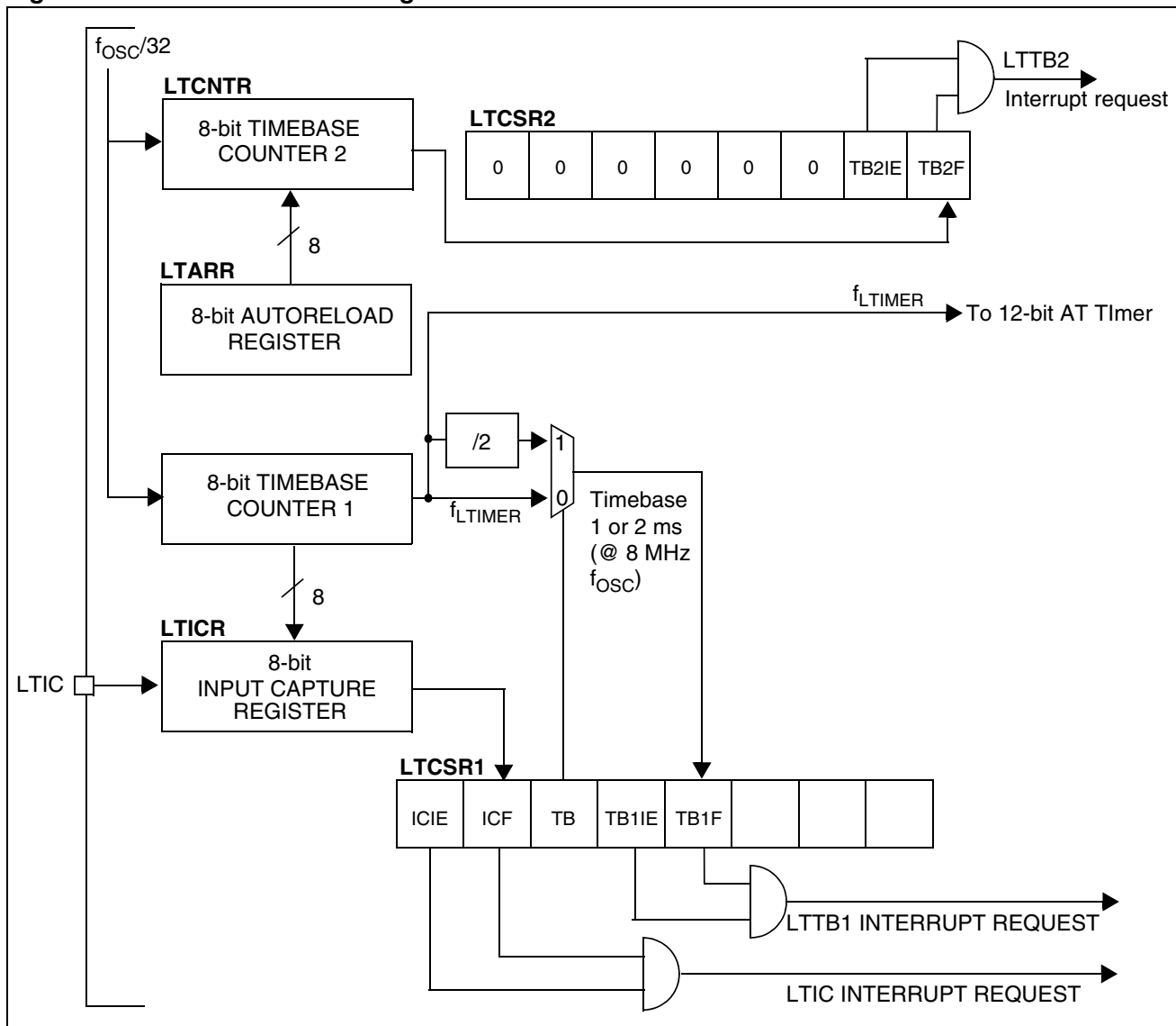
Figure 48. Lite Timer 2 Block Diagram
