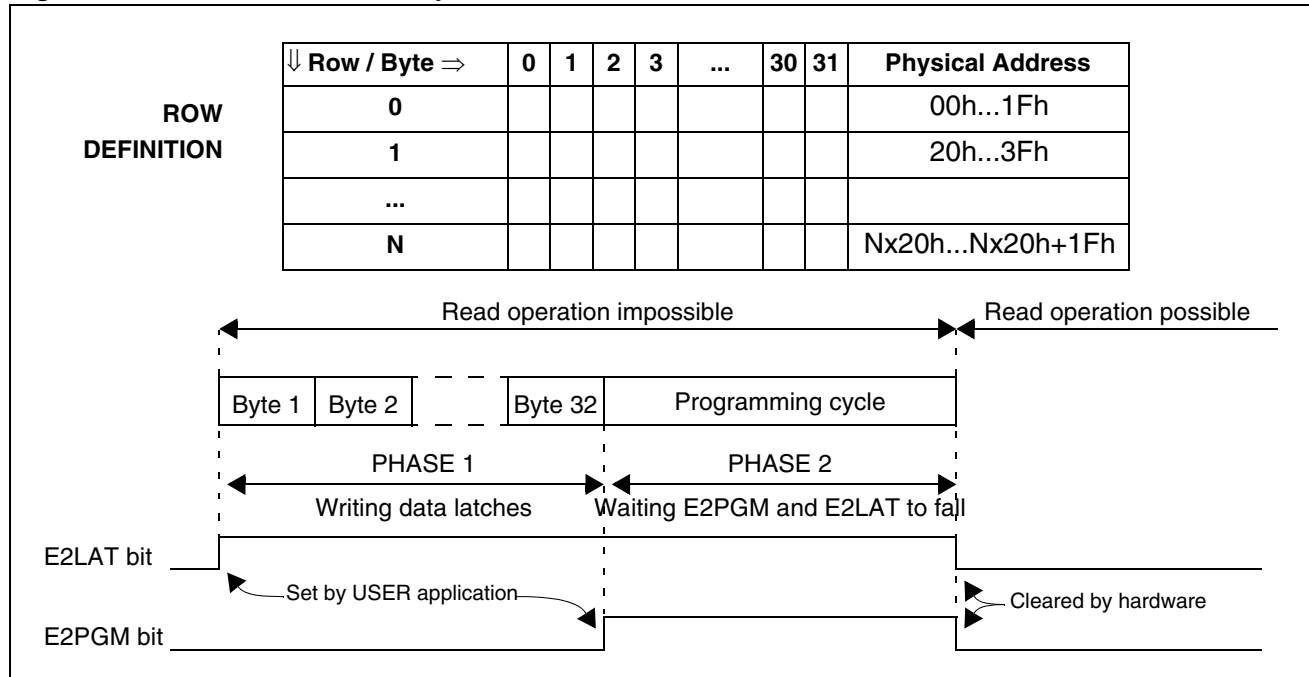
Figure 7. Data EEPROM Write Operation
