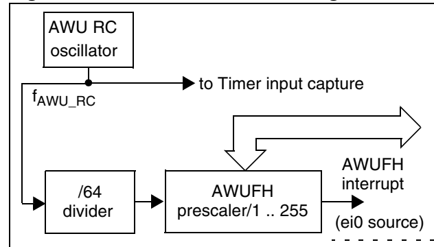
Figure 26. AWUFH Mode Block Diagram
