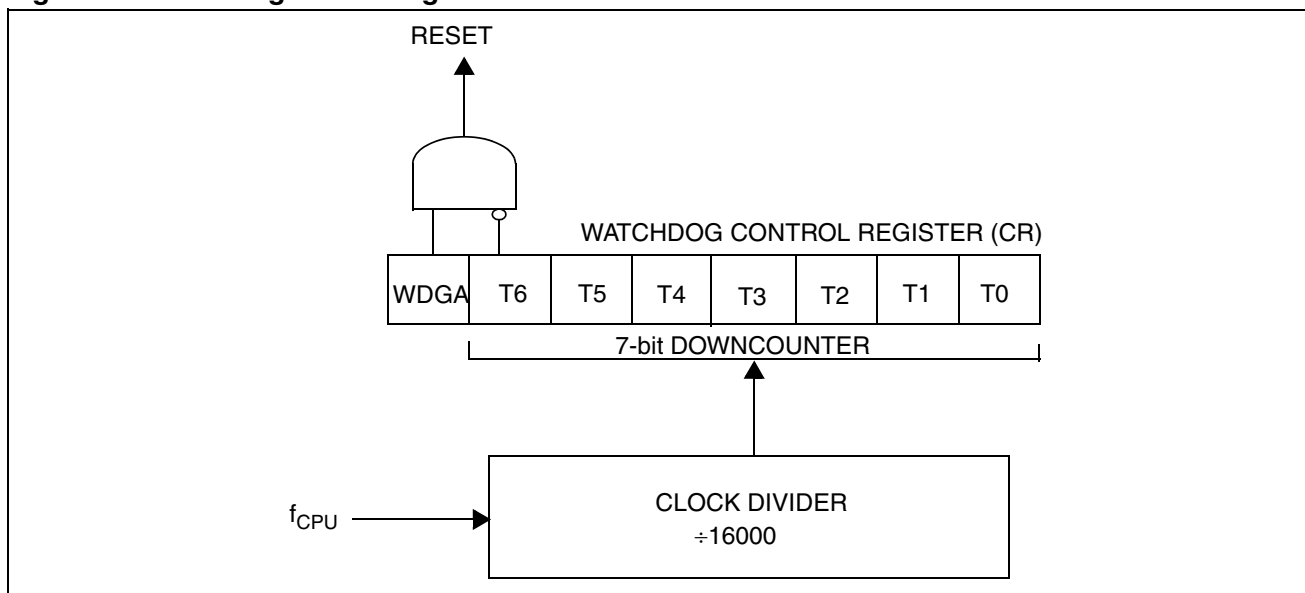
Figure 31. Watchdog Block Diagram
