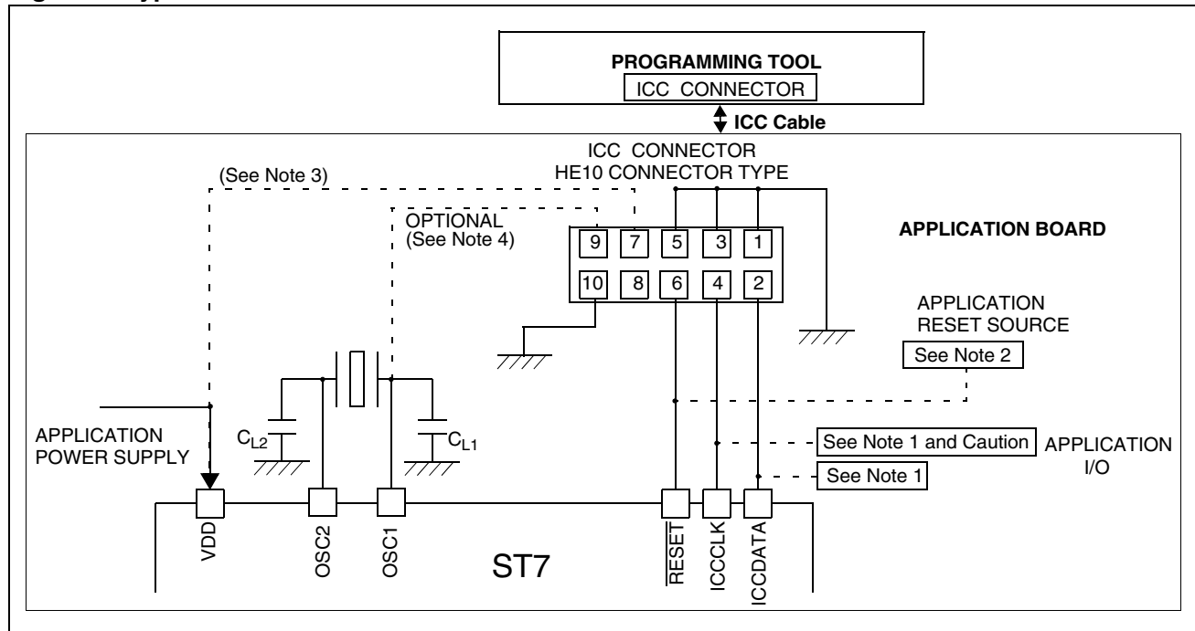
Figure 4. Typical ICC Interface
