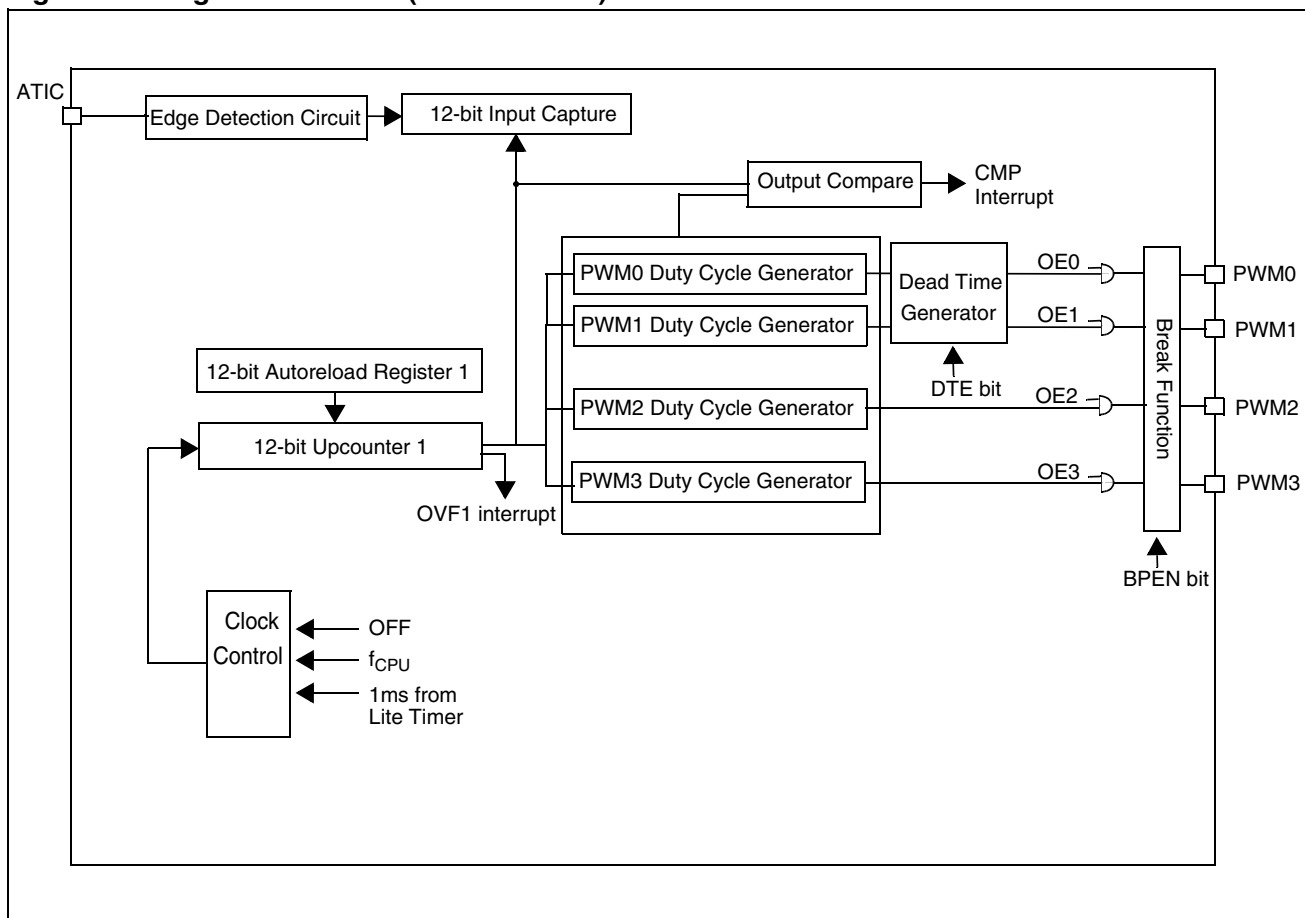
Figure 32. Single Timer Mode (ENCNTR2 = 0)
