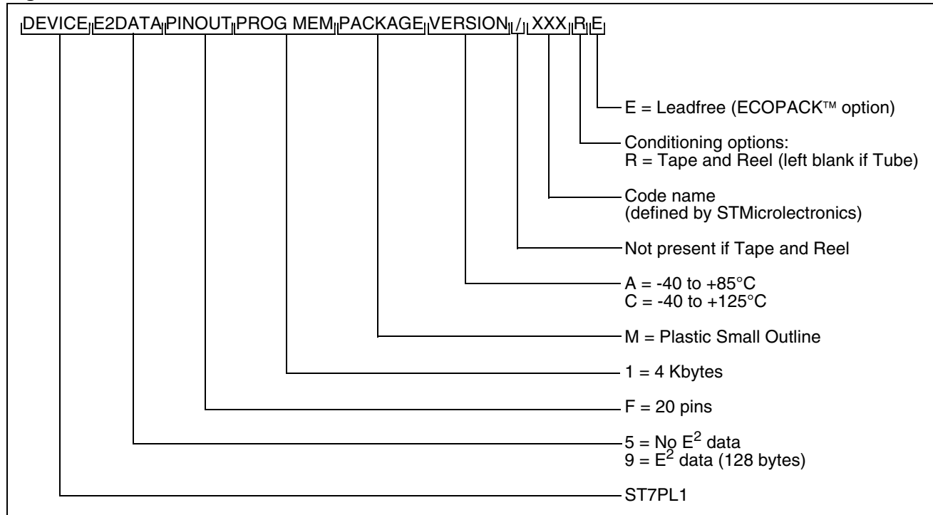
Figure 103. FASTROM Commercial Product Code Structure
