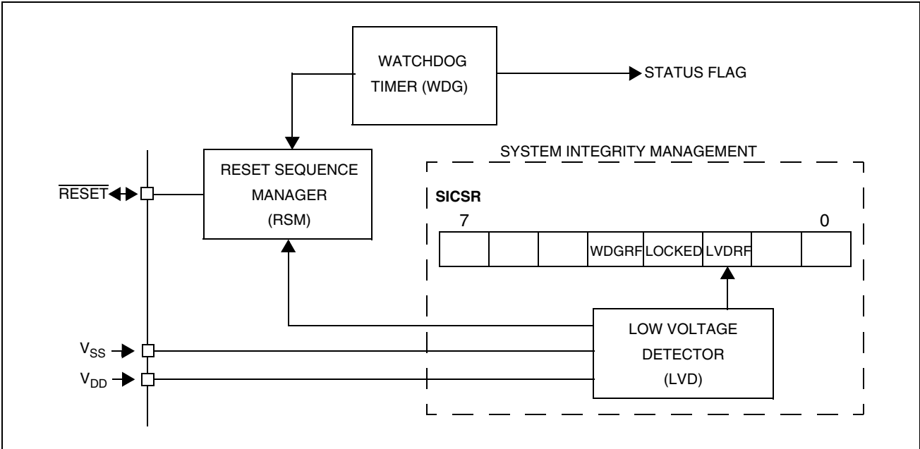
Figure 17. Reset and Supply Management Block Diagram
