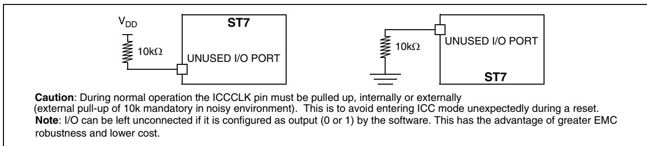
Figure 75. Two Typical Applications with Unused I/O Pin
