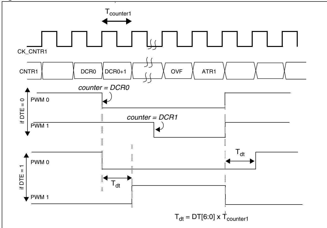
Figure 37. Dead Time Generation
