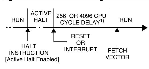
Figure 24. ACTIVE HALT Timing Overview
