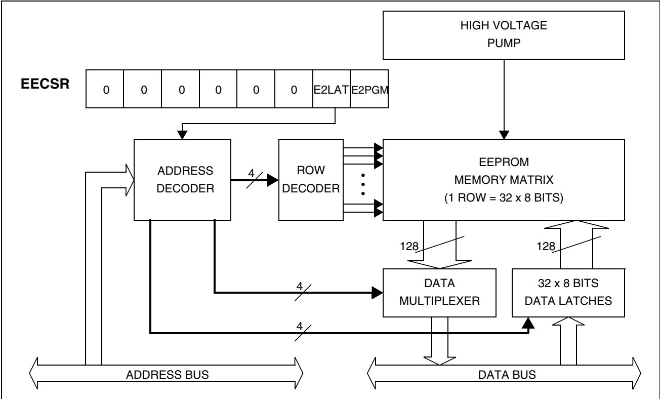
Figure 5. EEPROM Block Diagram
