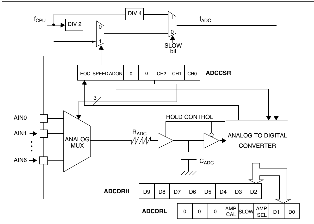
Figure 57. ADC Block Diagram
