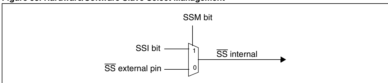
Figure 53. Hardware/Software Slave Select Management
