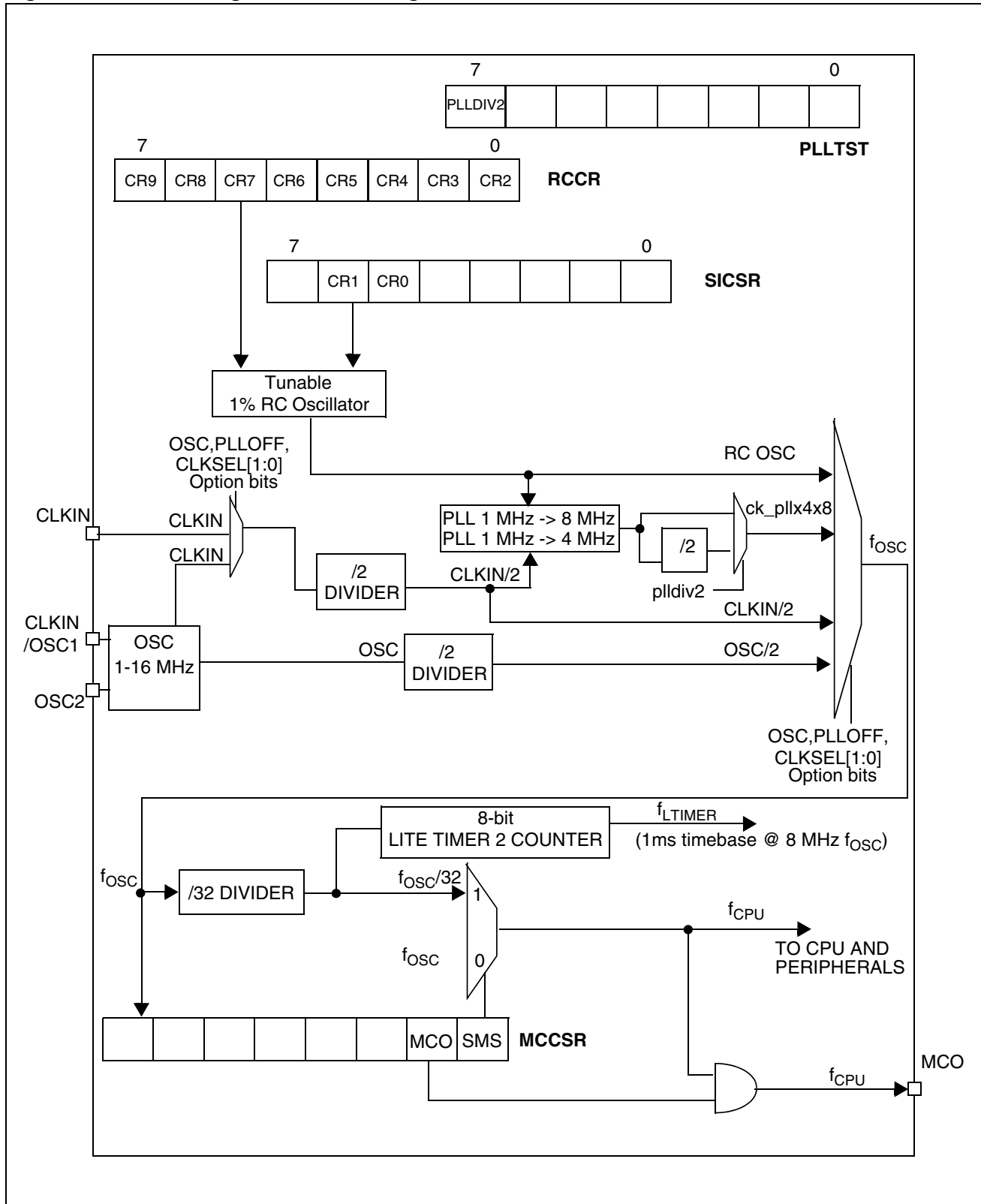
Figure 12. Clock Management Block Diagram
