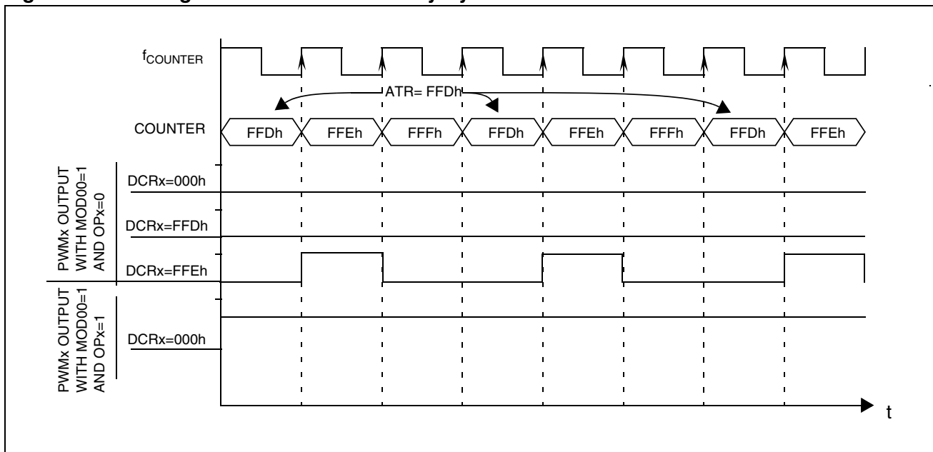
Figure 36. PWM Signal from 0% to 100% Duty Cycle
