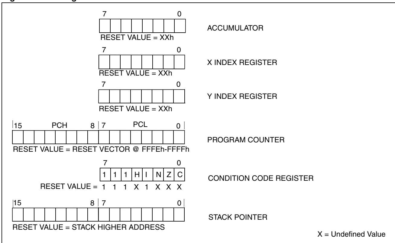
Figure 9. CPU Registers
