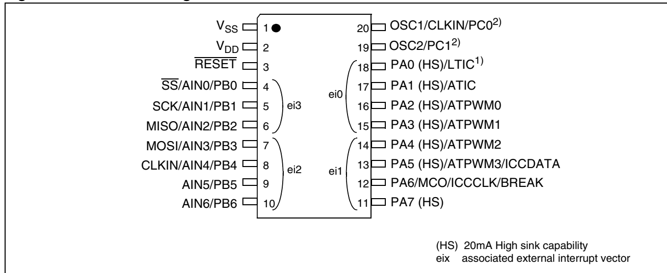
Figure 2. 20-Pin SO Package Pinout
