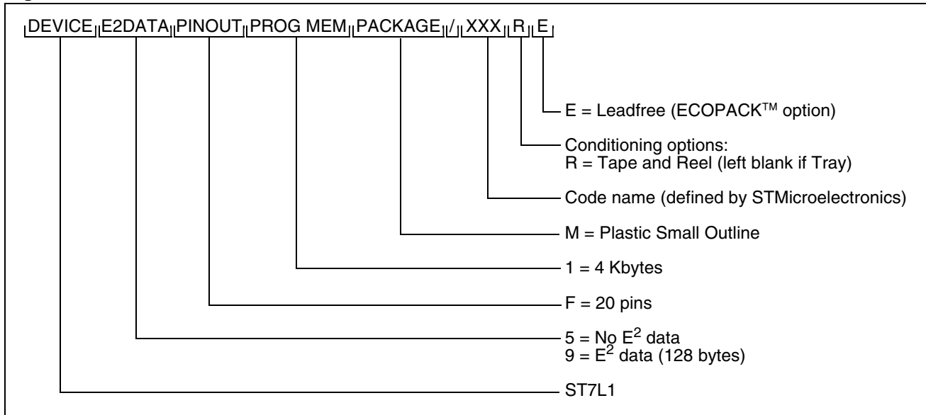
Figure 104. ROM Commercial Product Code Structure
