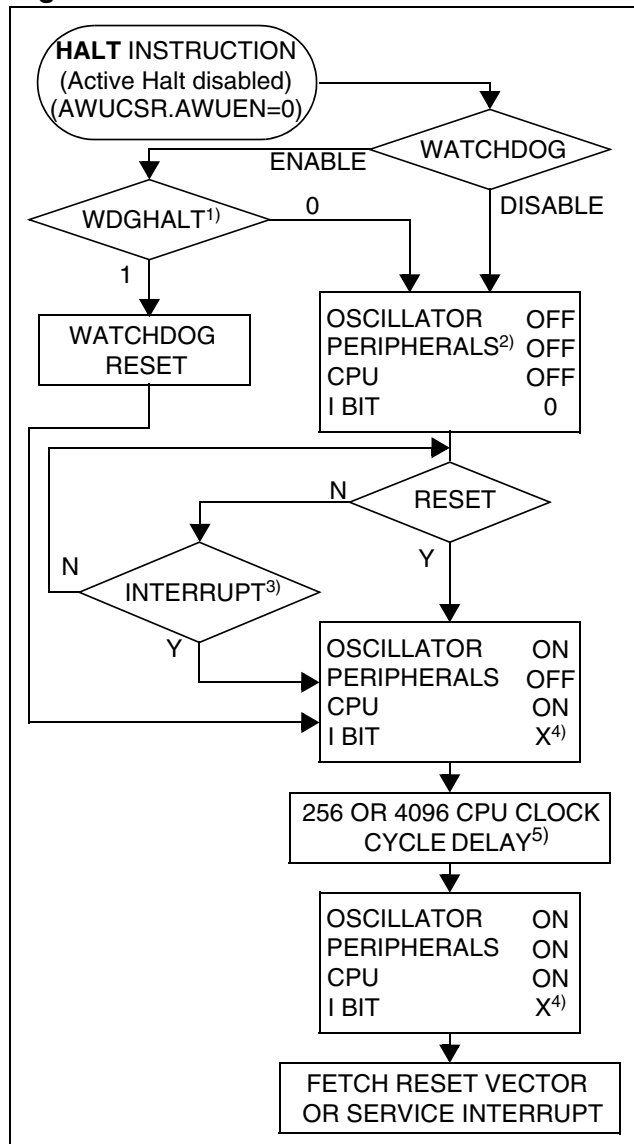
Figure 23. HALT Mode Flowchart
