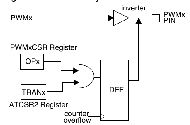
Figure 34. PWM Polarity Inversion
