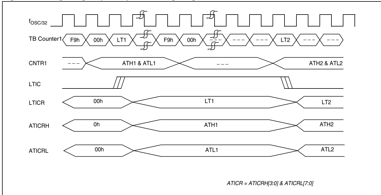
Figure 43. Long Range Input Capture Timing Diagram
