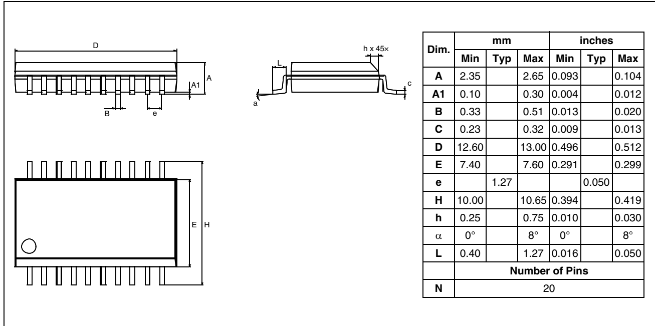
Figure 101. 20-Pin Plastic Small Outline Package, 300-mil Width
