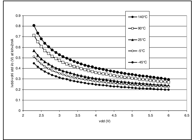
Figure 91. Typical V_{DD} - V_{OH} vs V_{DD} (Standard)
