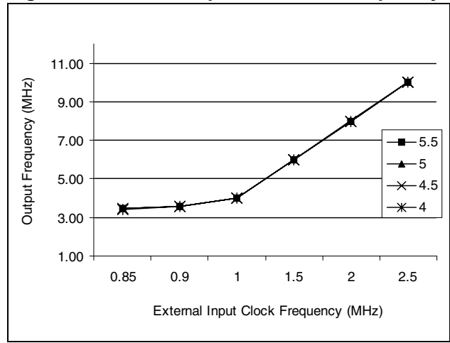
Figure 66. PLLx8 Output vs CLKIN Frequency
