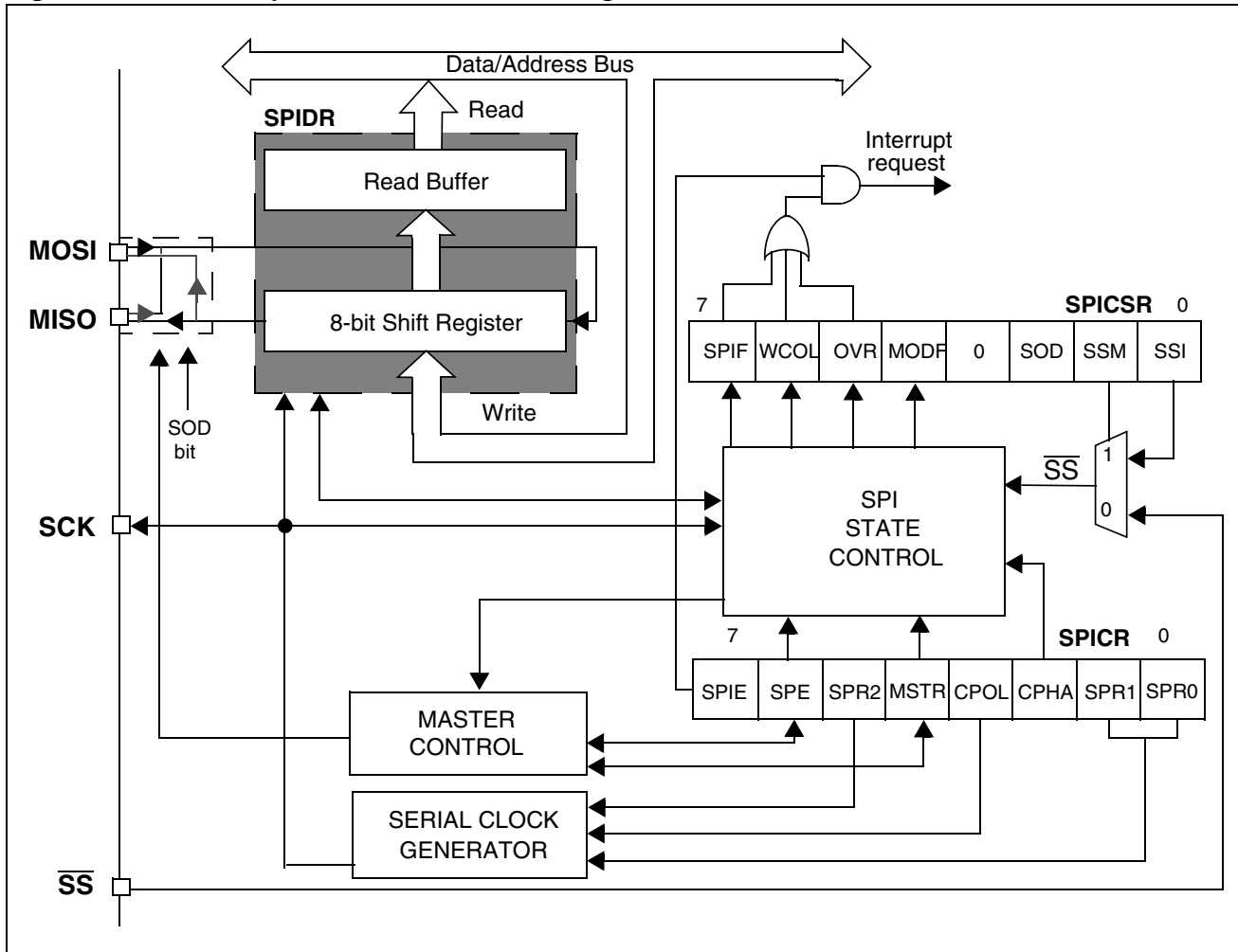
Figure 50. Serial Peripheral Interface Block Diagram
