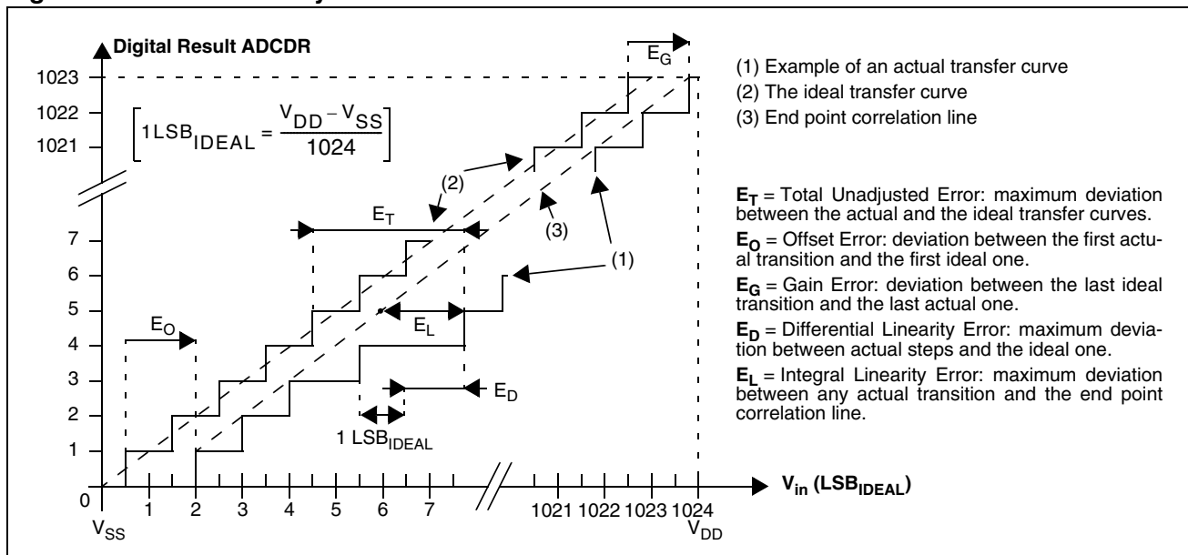
Figure 100. ADC Accuracy Characteristics
