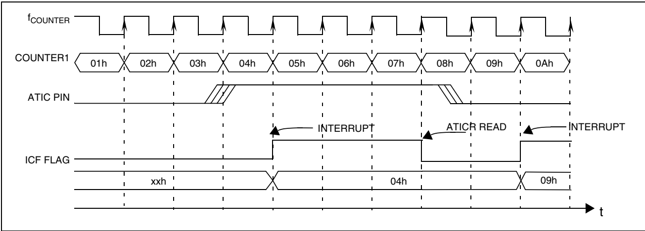
Figure 41. Input Capture Timing Diagram
