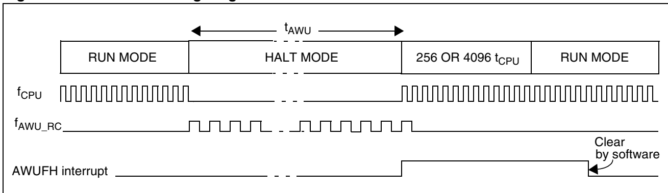
Figure 27. AWUF Halt Timing Diagram
