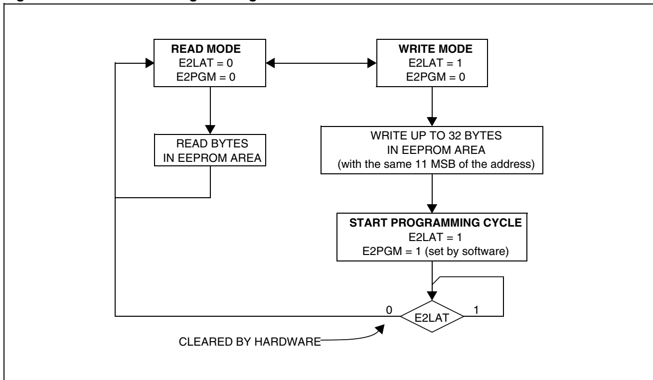
Figure 6. Data EEPROM Programming Flowchart
