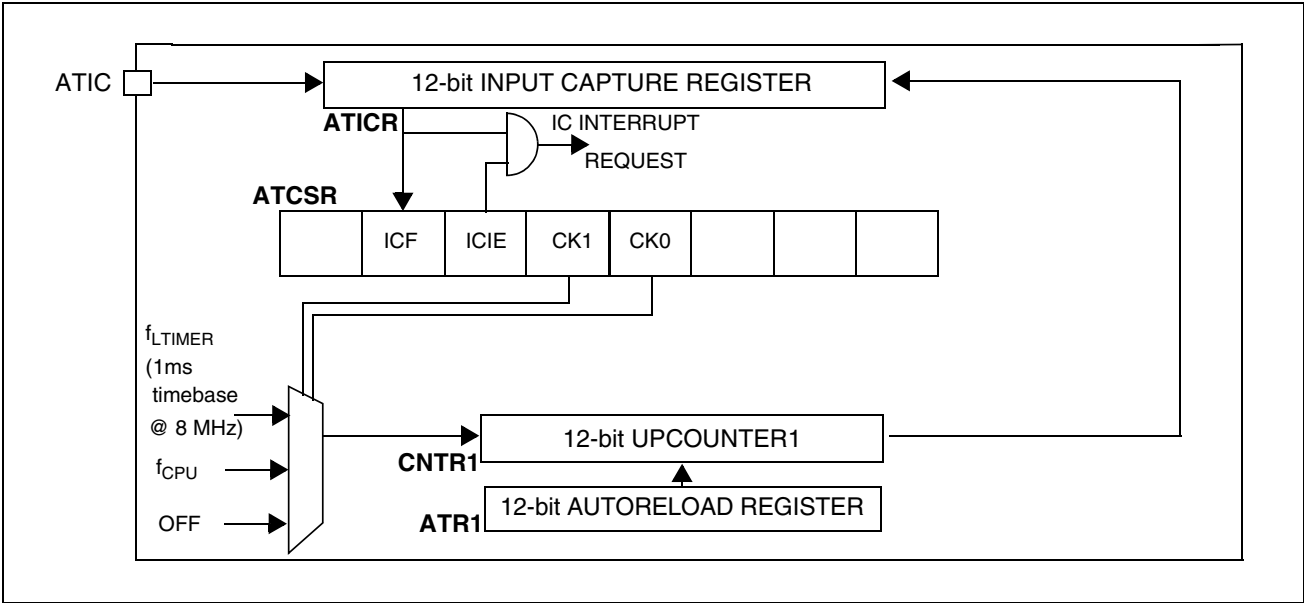
Figure 40. Block Diagram of Input Capture Mode
