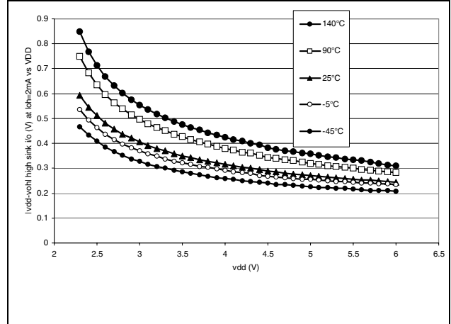
Figure 93. Typical V_{DD} - V_{OH} vs V_{DD} (Port C)
