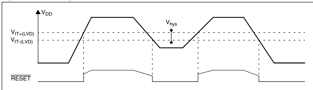
Figure 16. Low Voltage Detector vs Reset
