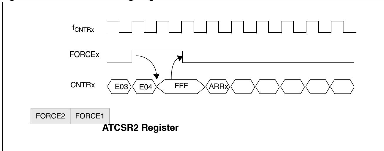
Figure 47. Force Overflow Timing Diagram
