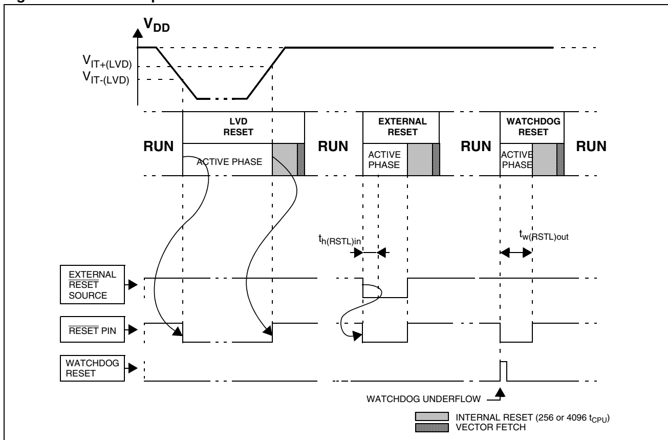
Figure 15. RESET Sequences
