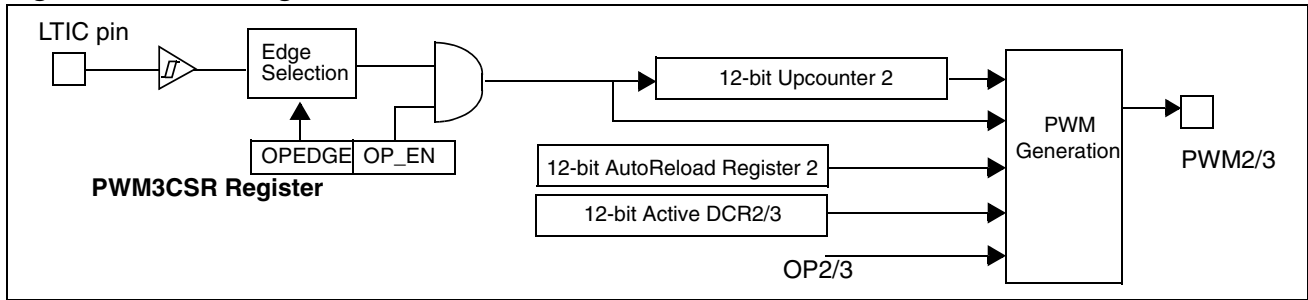
Figure 44. Block Diagram of One Pulse Mode
