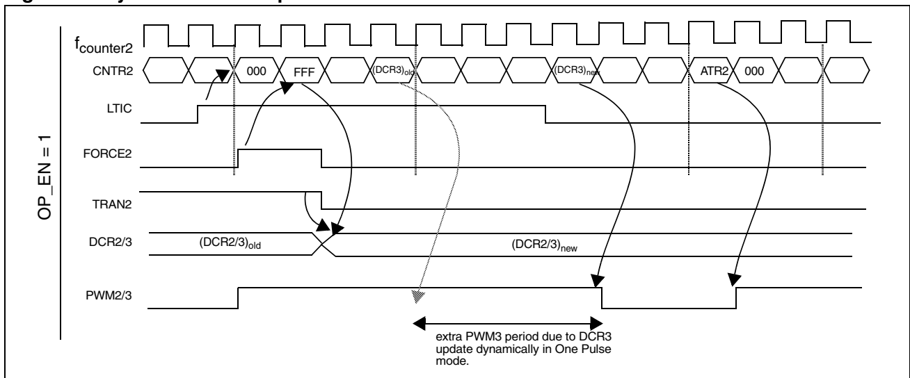
Figure 46. Dynamic DCR2/3 update in One Pulse Mode
