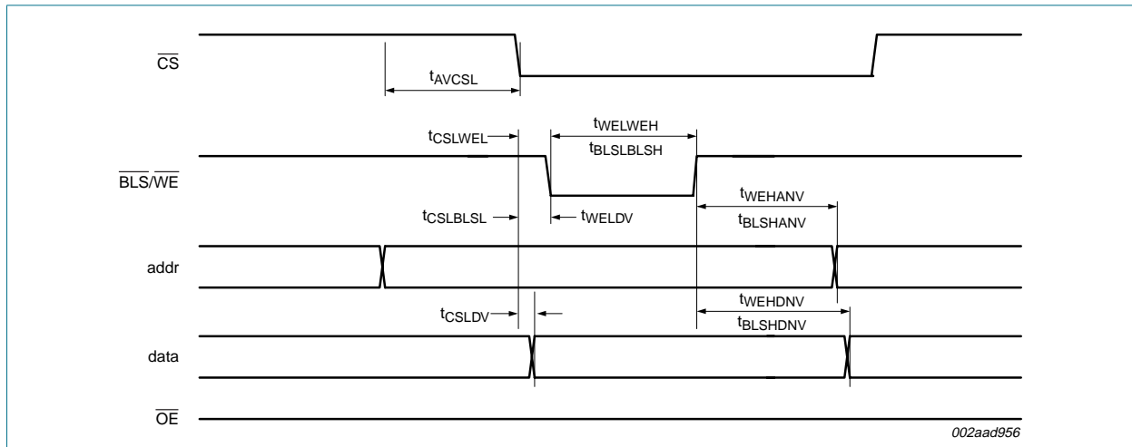
Fig 9. External memory write access
