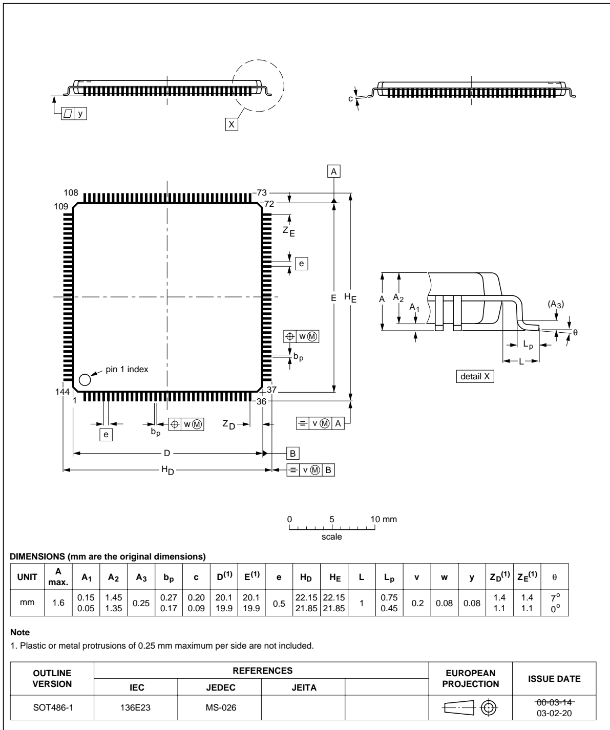
Fig 17. Package outline SOT486-1 (LQFP144)
