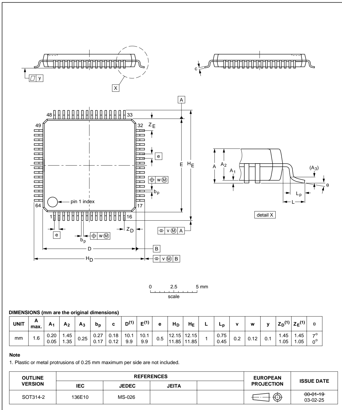
Fig 13. Package outline SOT314-2 (LQFP64)
