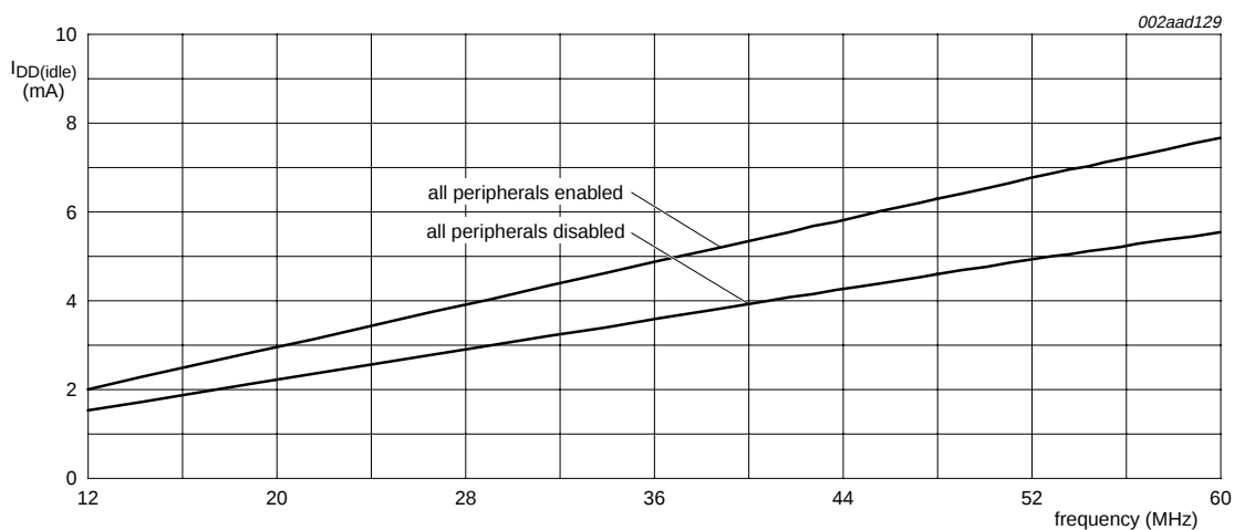
Fig 7. Typical LPC2109/01 I_{DD(idle)} measured at different frequencies
