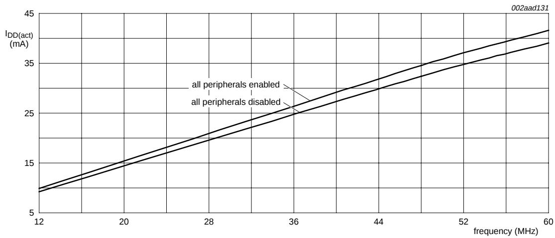
Fig 9. Typical LPC2119/01 and LPC2129/01 I_{DD(act)} measured at different frequencies
