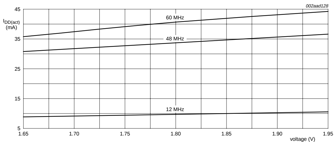
Fig 5. Typical LPC2109/01 I_{DD(act)} measured at different frequencies
