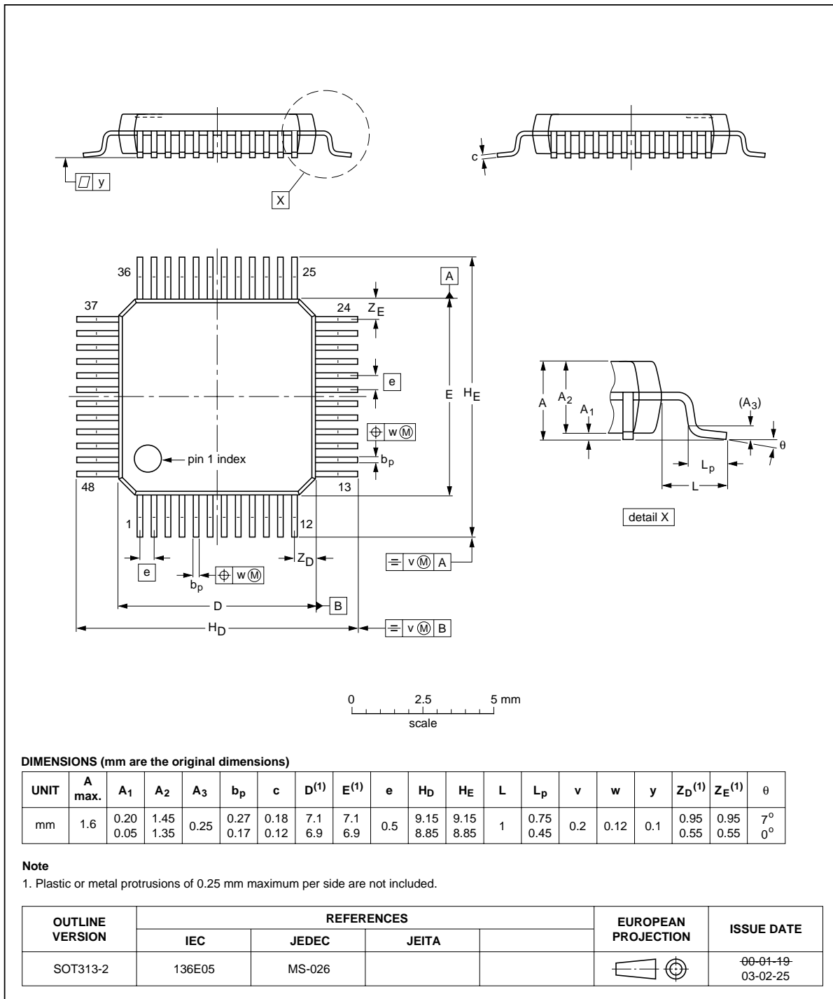
Fig 13. Package outline SOT313-2 (LQFP48)
