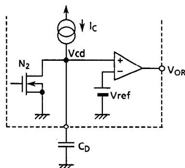
Figure 9 Delay circuit
