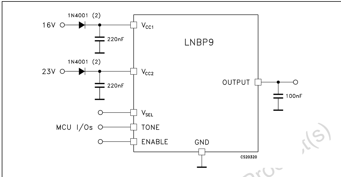
Figure 3. LNBP9 with 22KHz Tone control pin
