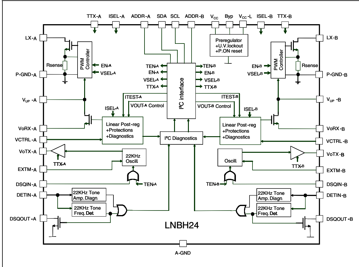
Figure 1. Block diagram
