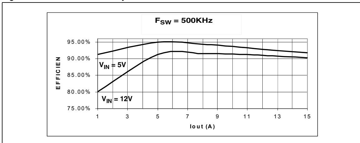
Figure 17. Demoboard efficiency
