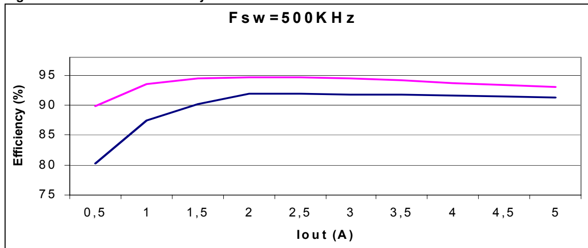
Figure 21. Demoboard efficiency
