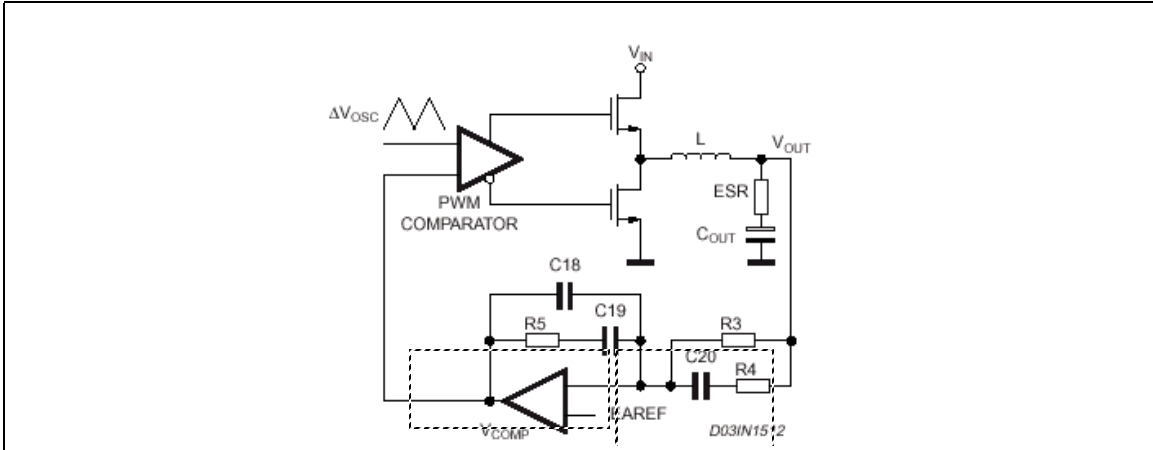
Figure 14. Compensation Network
