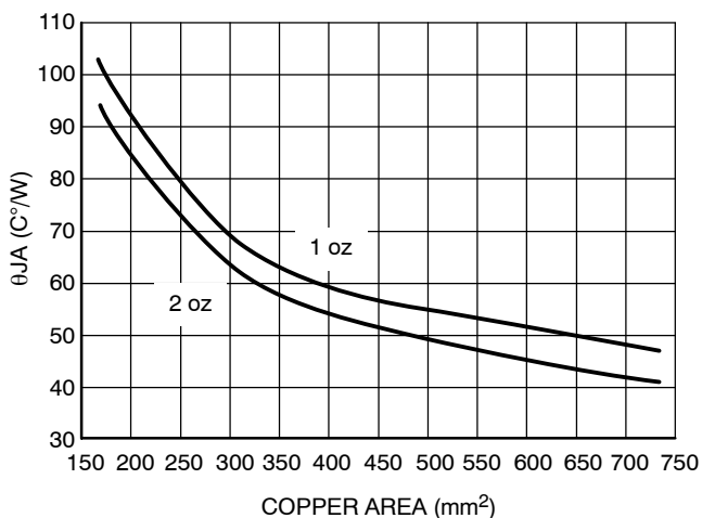
Figure 51. \theta_{JA} vs. Copper Spreader Area, DPAK 5-Lead
