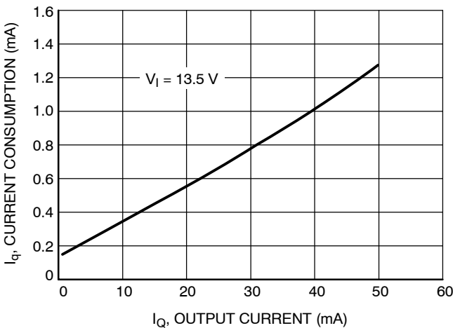
Figure 39. Current Consumption I_q vs. Output Current I_q (Low Load)
