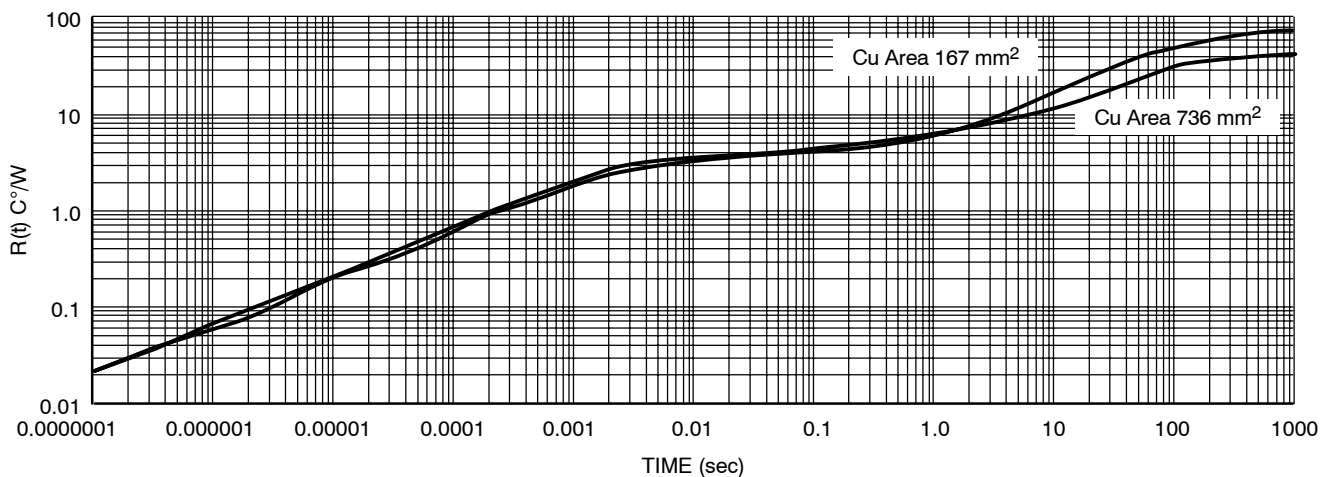
Figure 54. Single-Pulse Heating Curves, D 2 PAK 5-Lead
