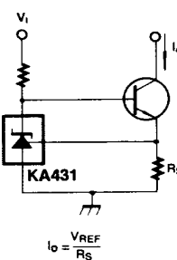
Figure 15. Constant-Current Sink
