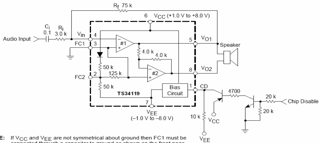
Figure 26. Split Supply Operation
