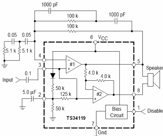
Figure 24. Audio Amplifier with Bandpass
