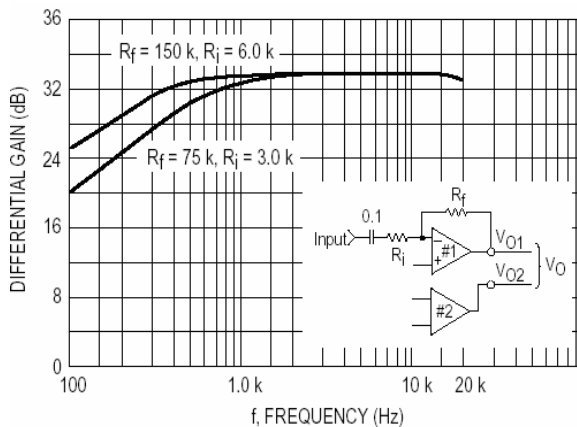
Figure 3. Differential Gain versus Frequency
