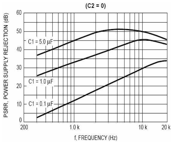
Figure 7. Power Supply Rejection versus Frequency
