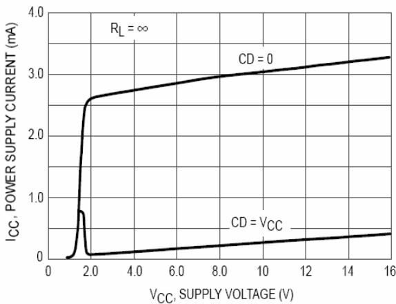
Figure 15. Power Supply Current
