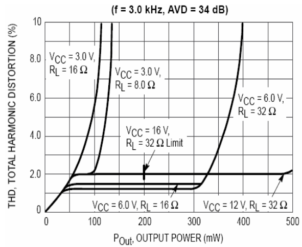
Figure 12. Distortion versus Power
