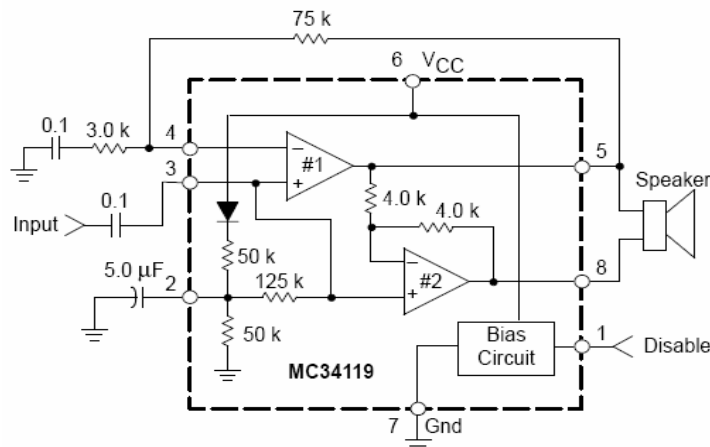
Figure 21. Audio Amplifier with High Input Impedance
