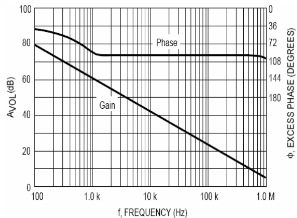
Figure 2. Amplifier #1 Open Loop Gain and Phase
