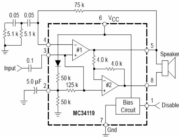
Figure 22. Audio Amplifier with Bass Suppression
