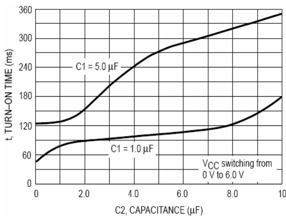
Figure 1. Turn-On Time versus C1, C2 at Power-On
