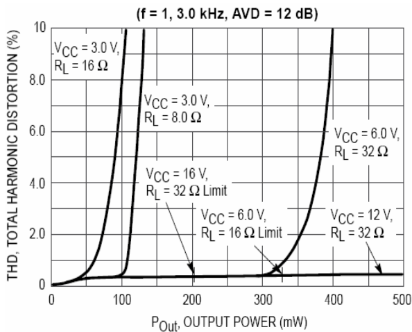
Figure 13. Distortion versus Power
