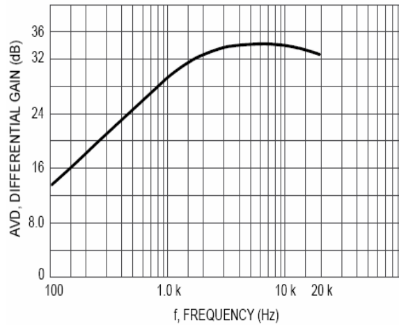
Figure 23. Frequency Response of Figure 22
