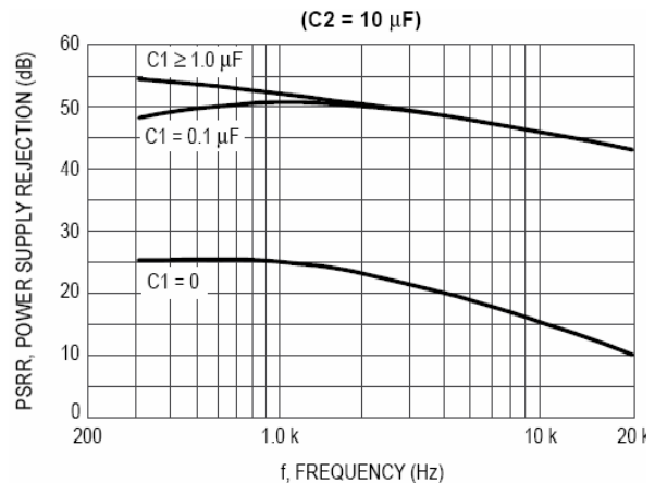
Figure 4. Power Supply Rejection versus Frequency
