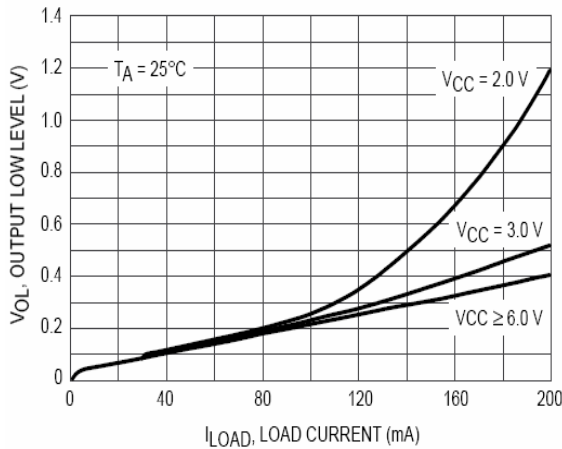
Figure 19. V_{OL} @ VO_1, VO_2 versus Load Current
