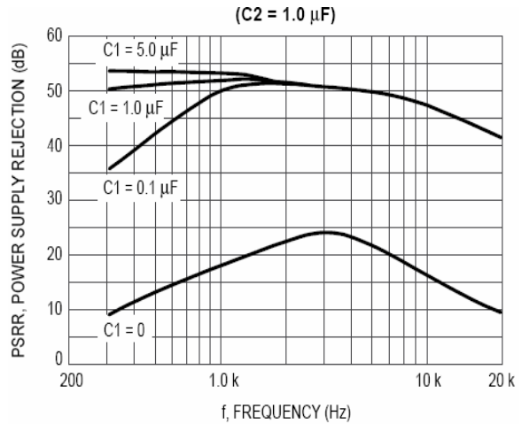
Figure 6. Power Supply Rejection versus Frequency
