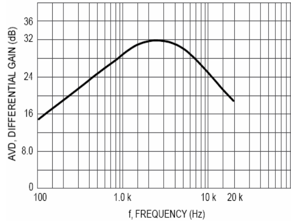
Figure 25. Frequency Response of Figure 24
