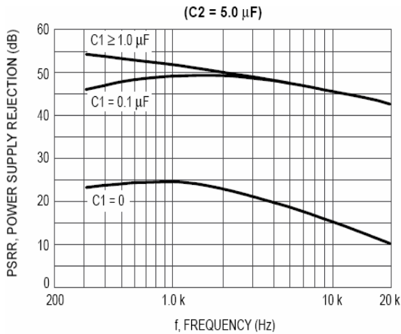
Figure 5. Power Supply Rejection versus Frequency
