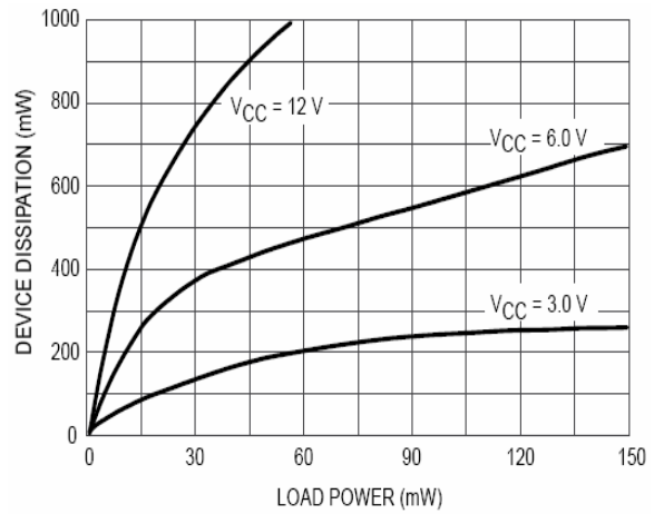
Figure 8. Device Dissipation, 8.0 Ω Load
