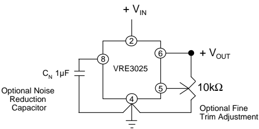
Figure 3 External Connections
