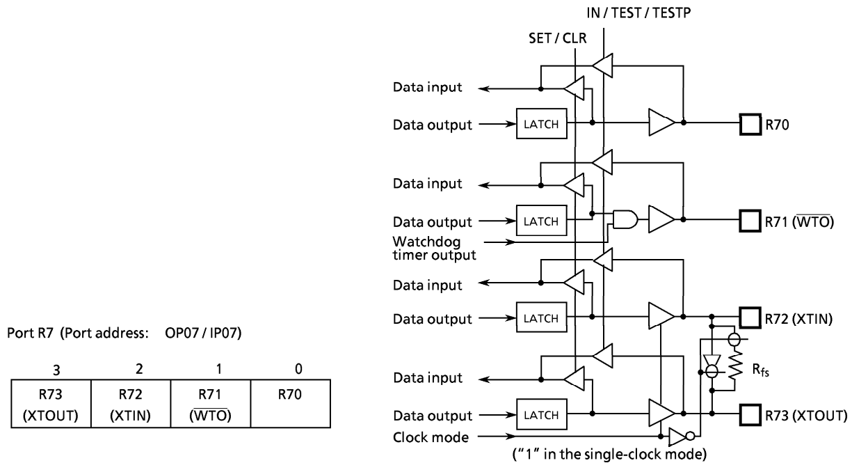
Figure 3-8. Port R7
