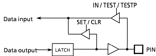
Figure 3-7. Port R6
