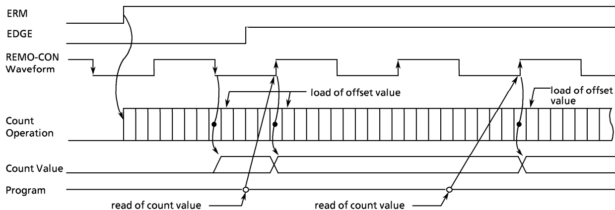
Figure 3-24. Timing chart
