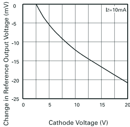
Change in Vref v Cathode Voltage
