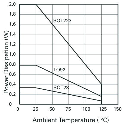
Power Dissipation Derating
