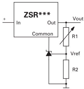
Shunt regulator
