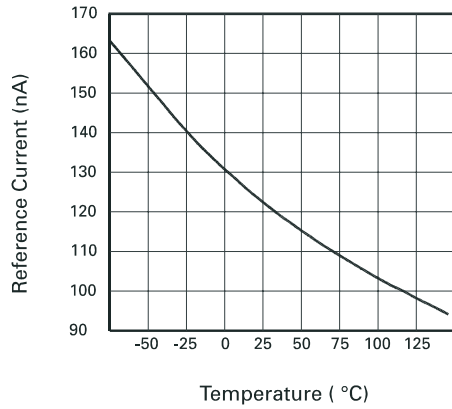
Iref vs. Temperature
