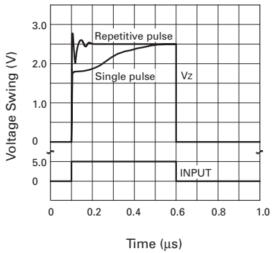
Pulse Response
