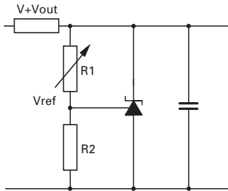
Shunt regulator
