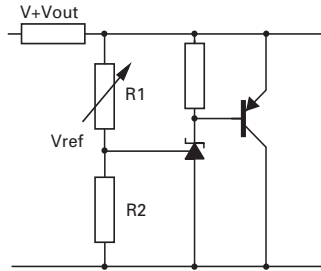
Higher current shunt regulator
