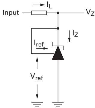
Fig 1 - Test circuit for V_Z = V_{ref}
