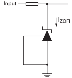
Fig 3 - Test circuit for for OI state current †
