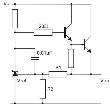
Higher current shunt regulator
