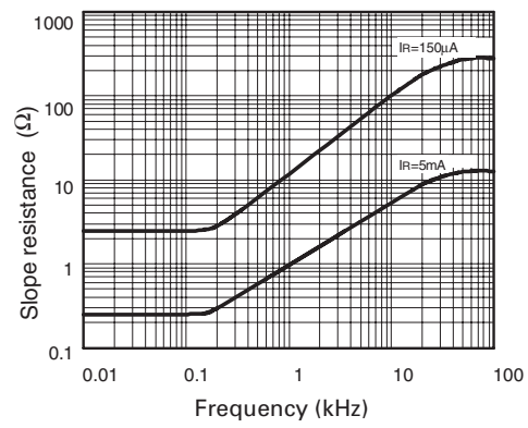
Slope Resistance v Frequency
