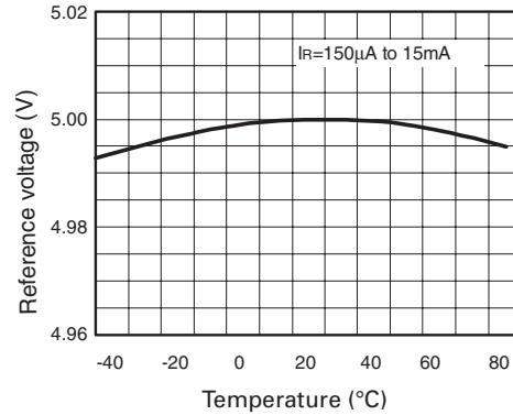
Temperature Drift
