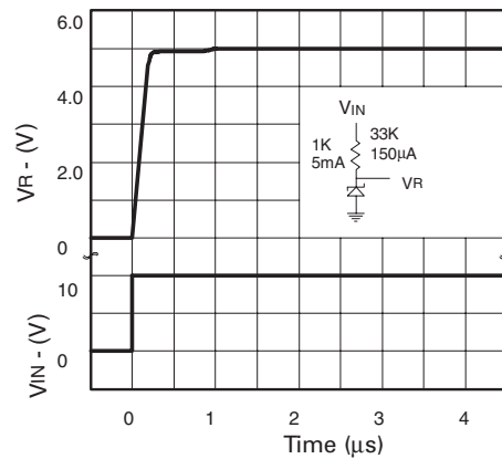
Transient Response (Repetitive Pulse)
