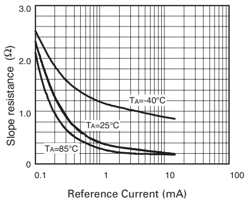
Slope Resistance v Current
