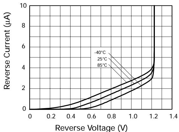
Reverse Characteristics
