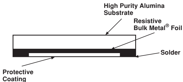
FIGURE 3 - CHIP CONFIGURATION
