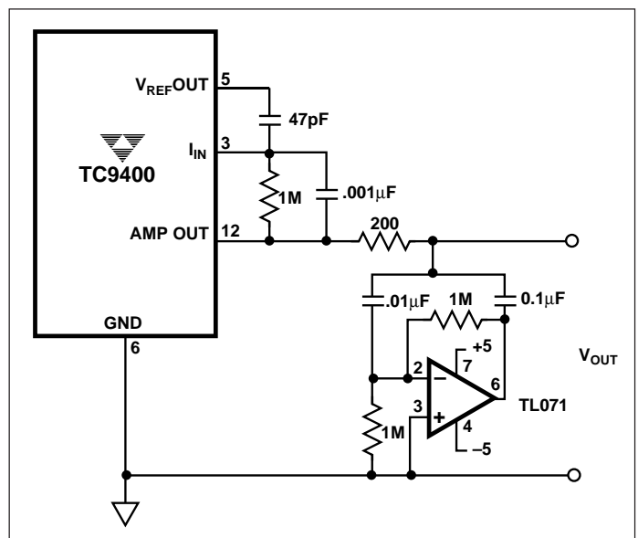
Figure 10. Ripple Filter
