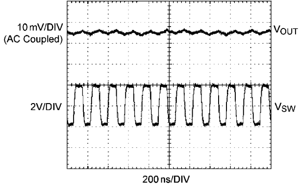
Typical Switching Waveform (PWM Mode, I_{OUT} = 300\text{ mA} )
