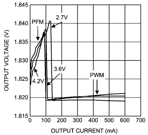
Output Voltage vs. Output Current (Auto Mode)
