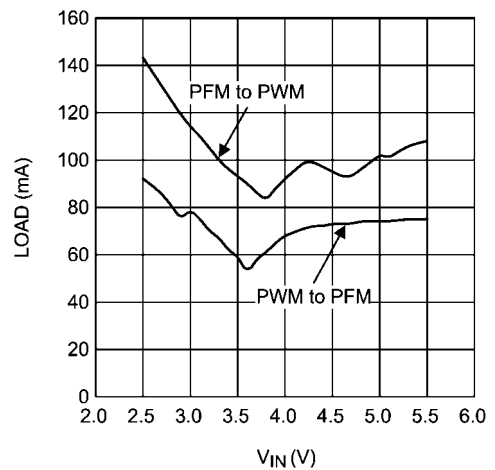
PFM ↔ PWM Mode Change Point
