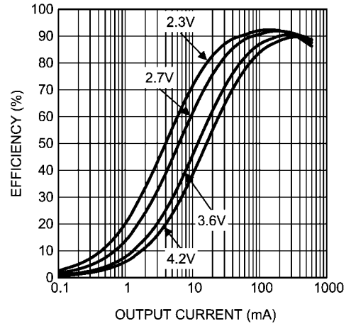
Efficiency vs. Output Current (PWM Mode)
