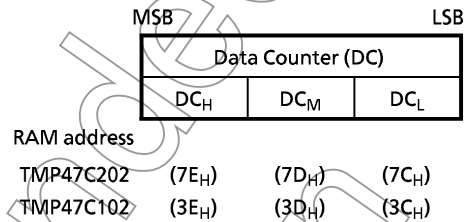
Figure 2-7. Data Counter
