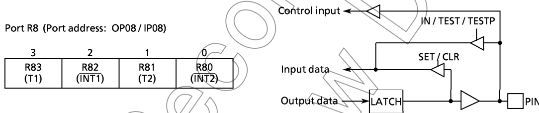
Figure 3-5. Port R8
