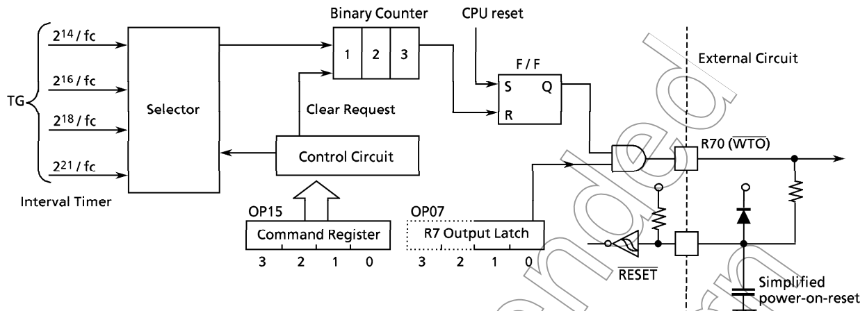
Figure 3-14. Watchdog Timer
