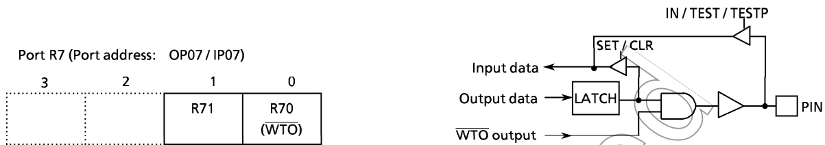
Figure 3-4. Ports R7
