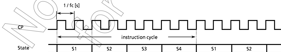
Figure 2-17. Instruction Cycle
