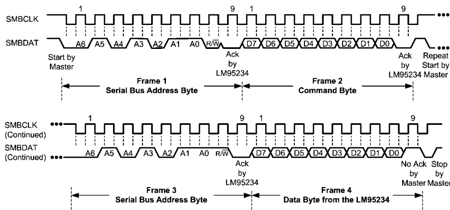
(d) Serial Bus Write followed by a Repeat Start and Immediate Read 20106314
