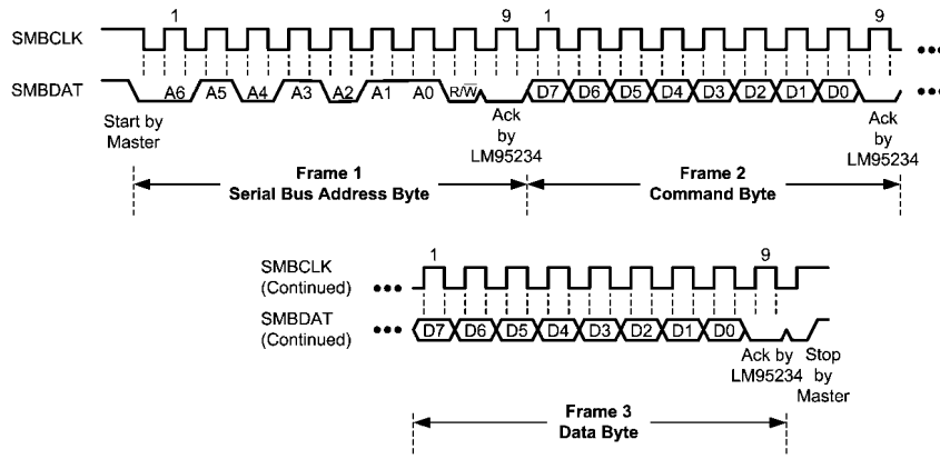
(a) Serial Bus Write to the internal Command Register followed by a the Data Byte 20106310
