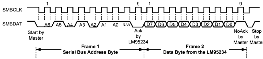
(c) Serial Bus Read from a Register with the Internal Command Register preset to desired value. 20106312
