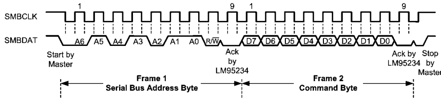
(b) Serial Bus Write to the Internal Command Register 20106311
